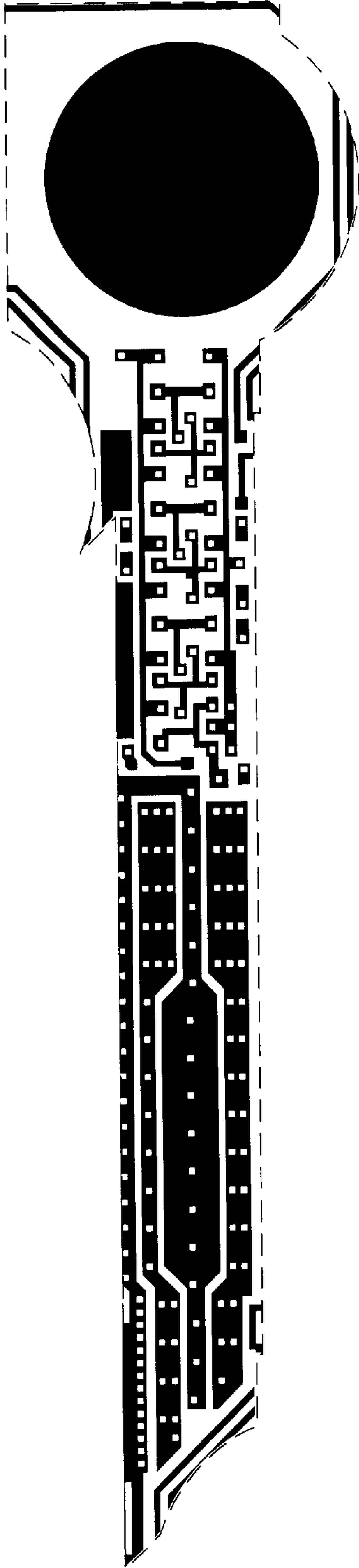
Metal 1 mask
