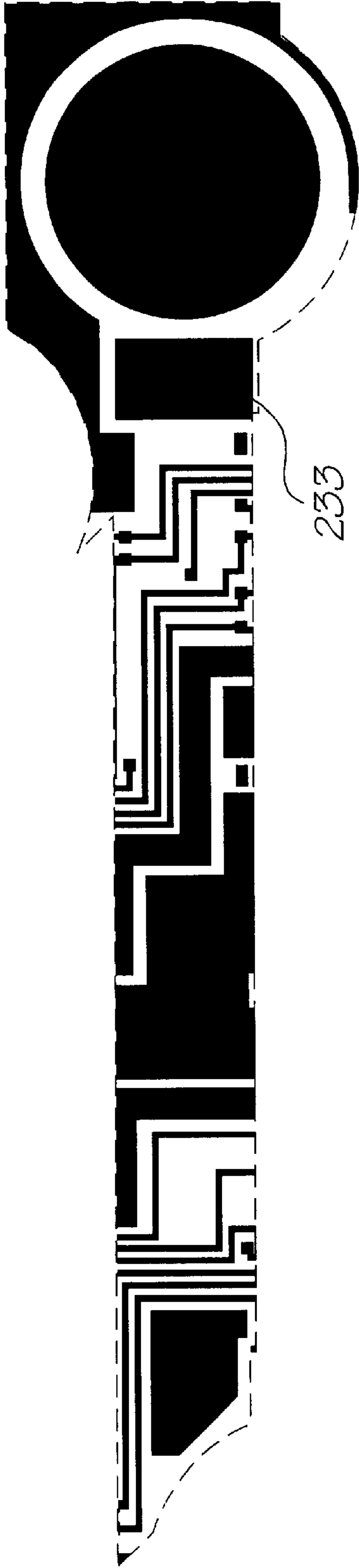
Metal 2 mask
