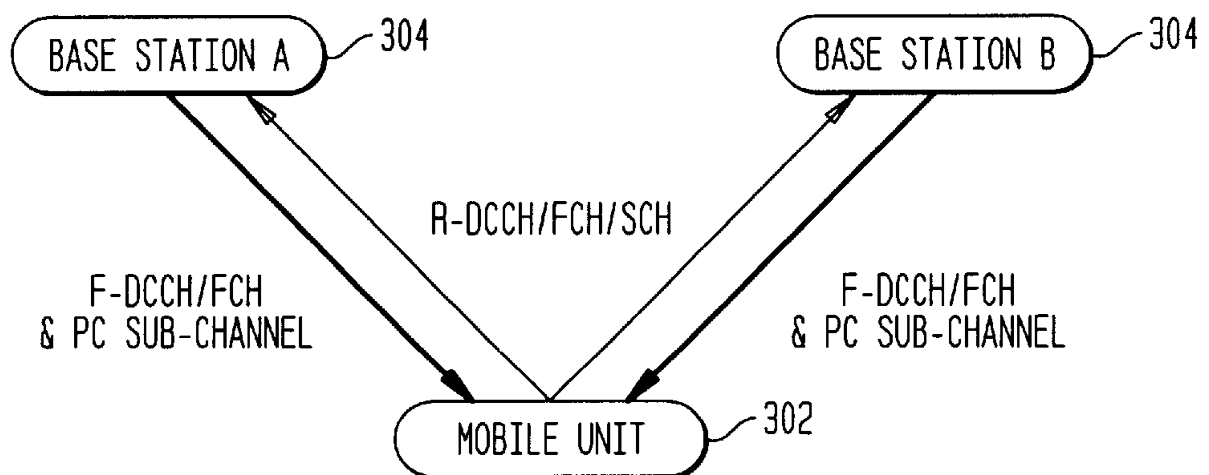
FIG. 3 (PRIOR ART)
