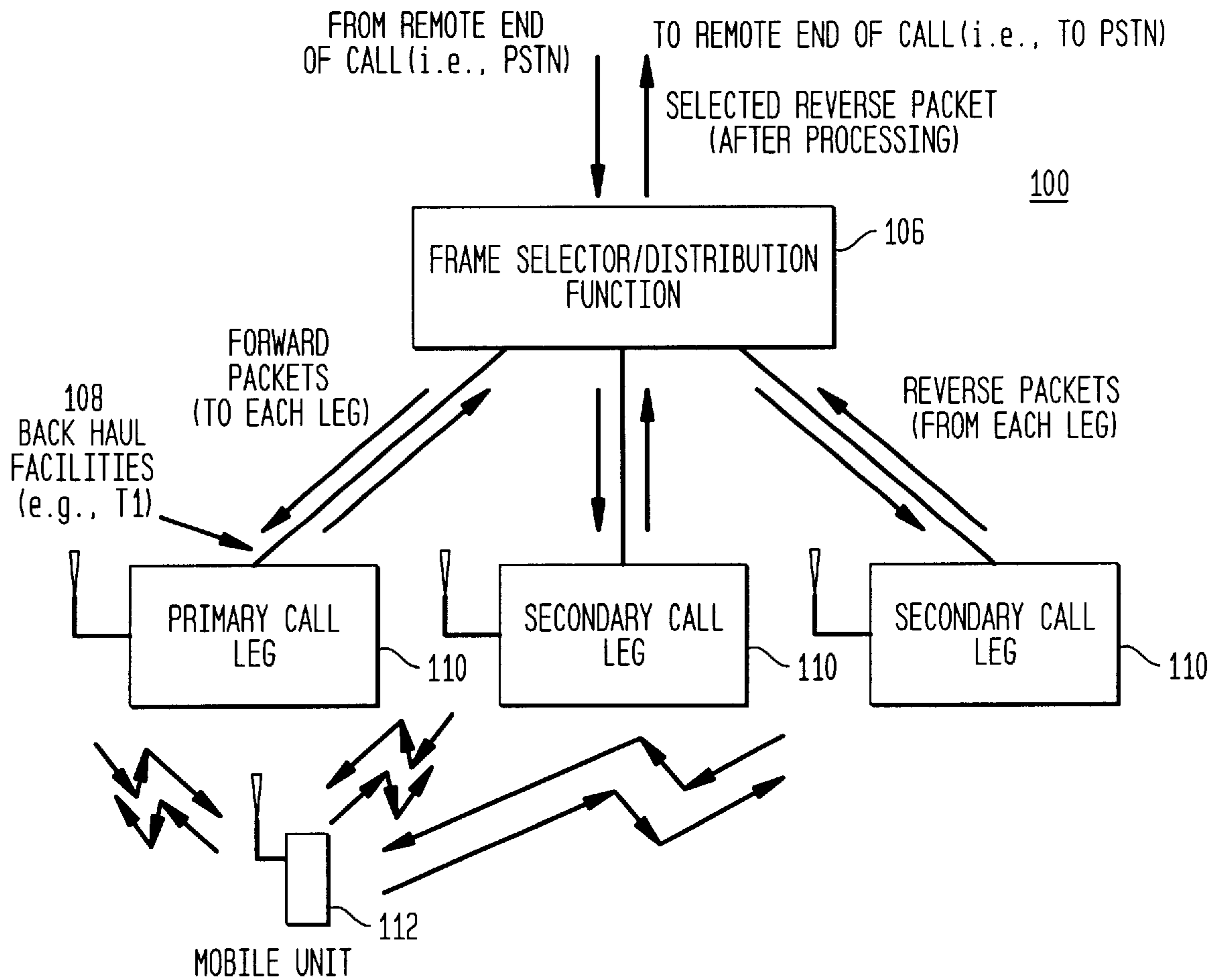
FIG. 2 (PRIOR ART)
