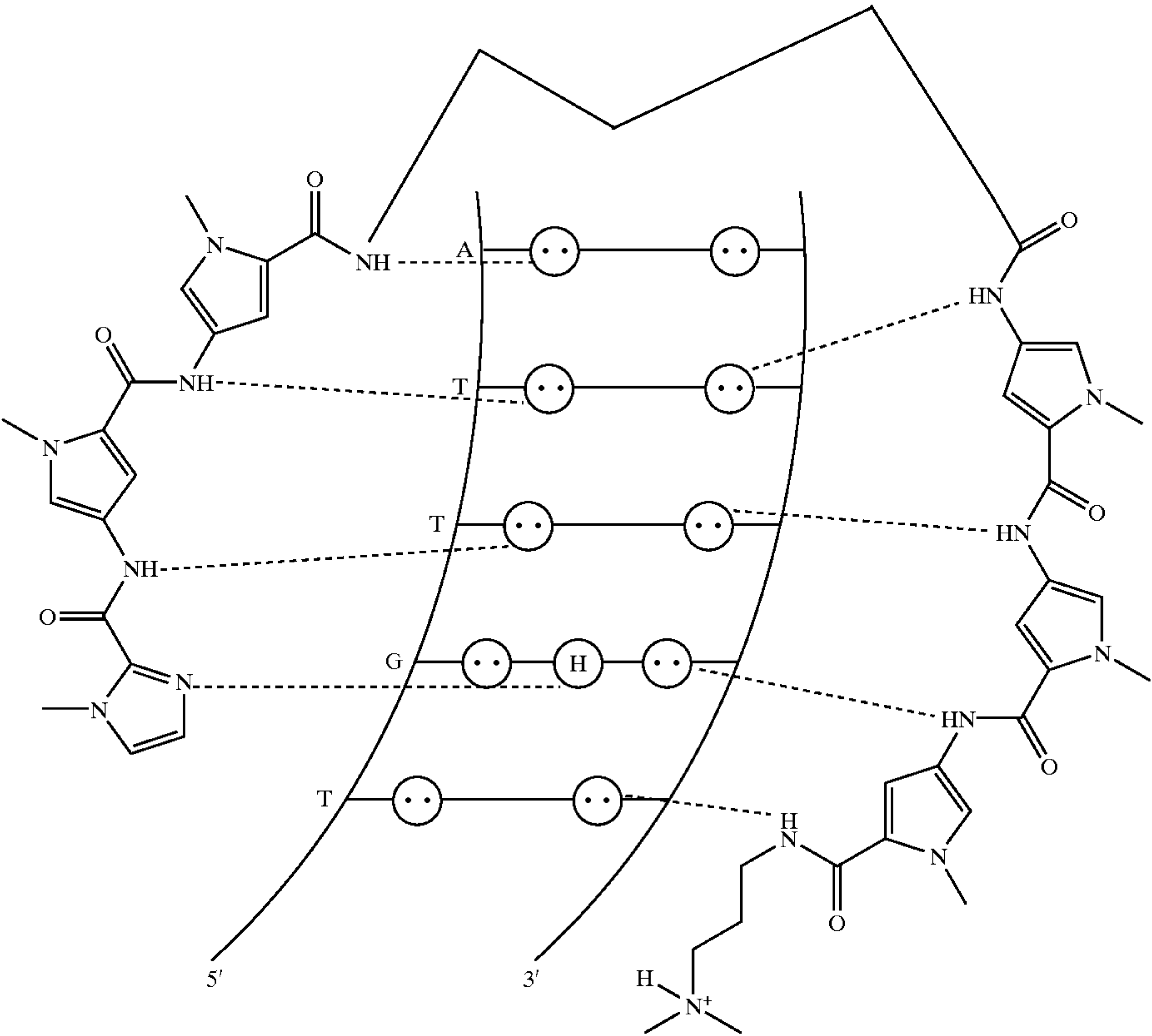
ImPyPy-γ-PyPyPy-Dp•TGTТА K_a = 8 \times 10^7 M^{-1}
