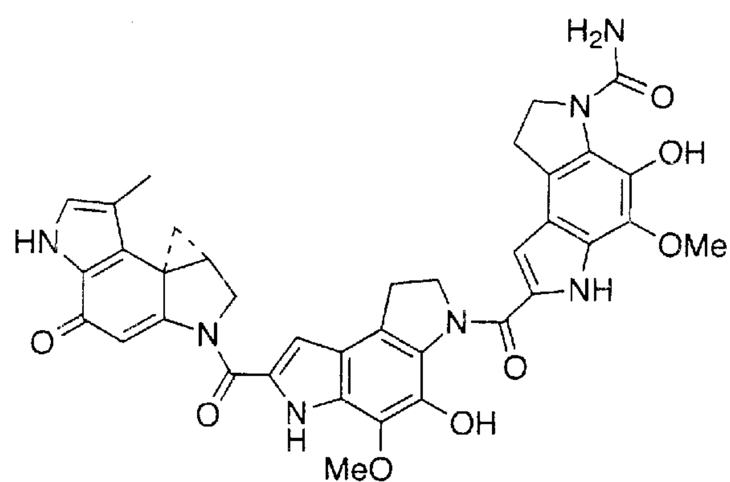
(+)- CC-1065
