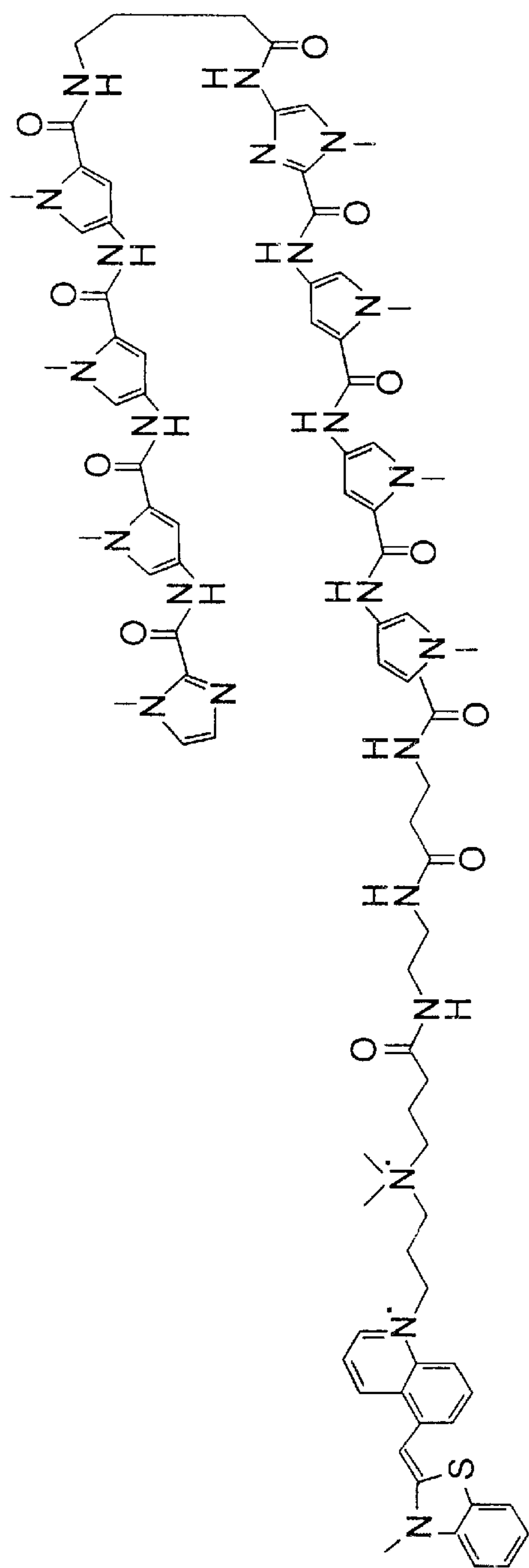
ImPyPyPy-β-ImPyPyPy-β-ED-TO
