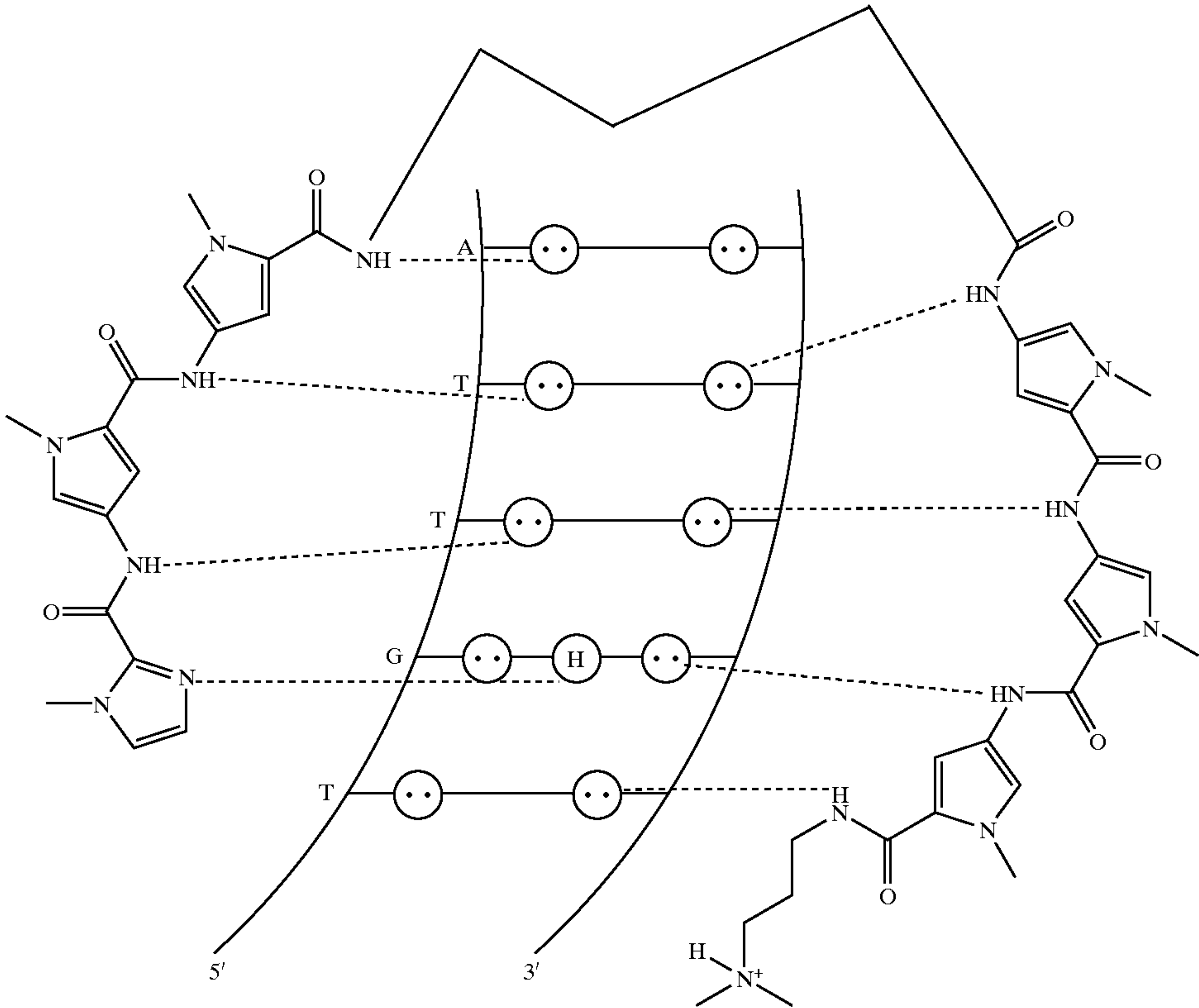
ImPyPy- \gamma -PyPyPy-Dp•5'-TGTTA-3' K_a = 7 \times 10^7 \text{M}^{-1} specificity: 30-fold
