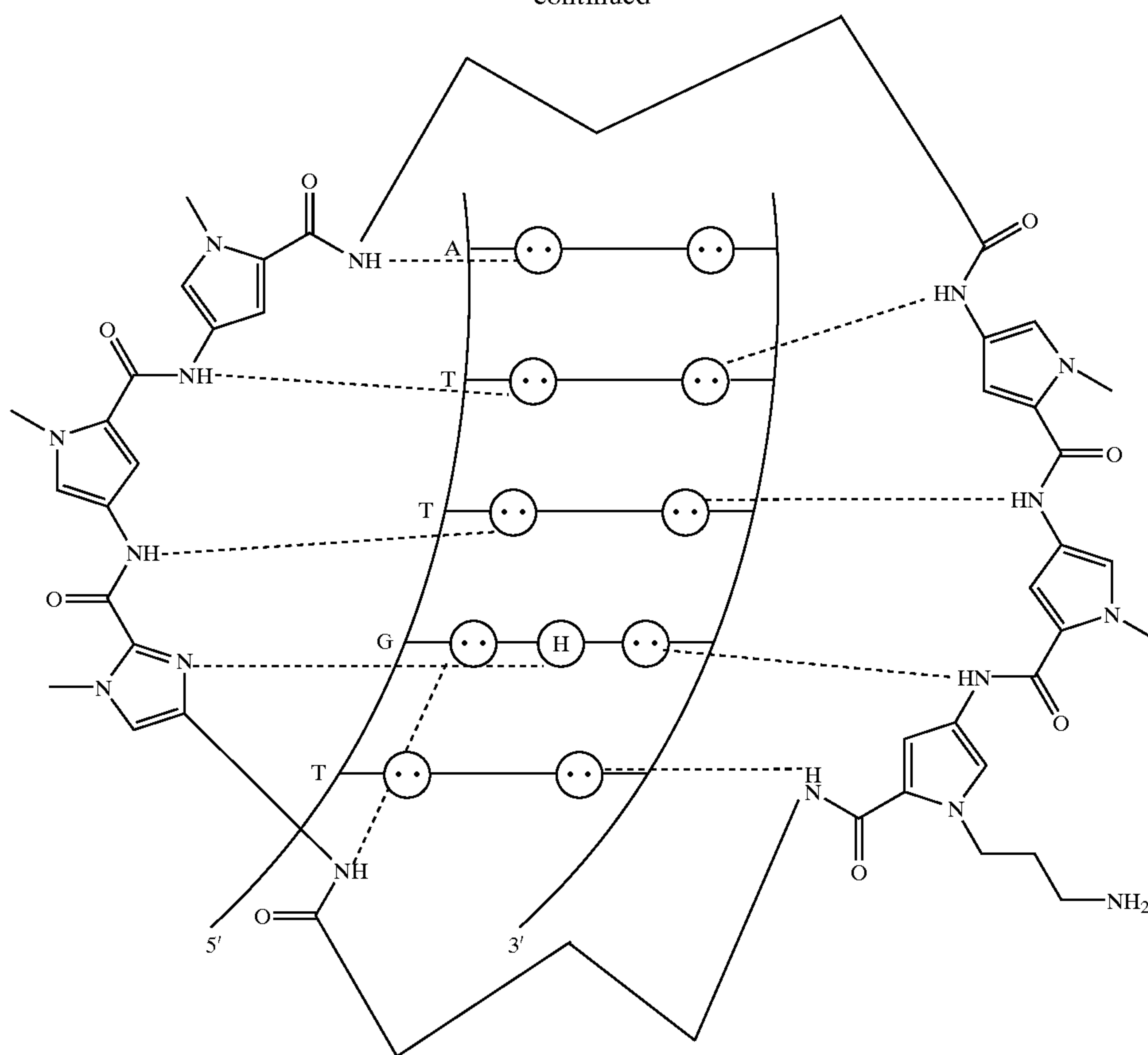
cyclo-(ImPyPy- \gamma -PyPyPy- \gamma )-5'-TGTTA-3' K_a = 2 \times 10^9 M^{-1} specificity: 2-fold
