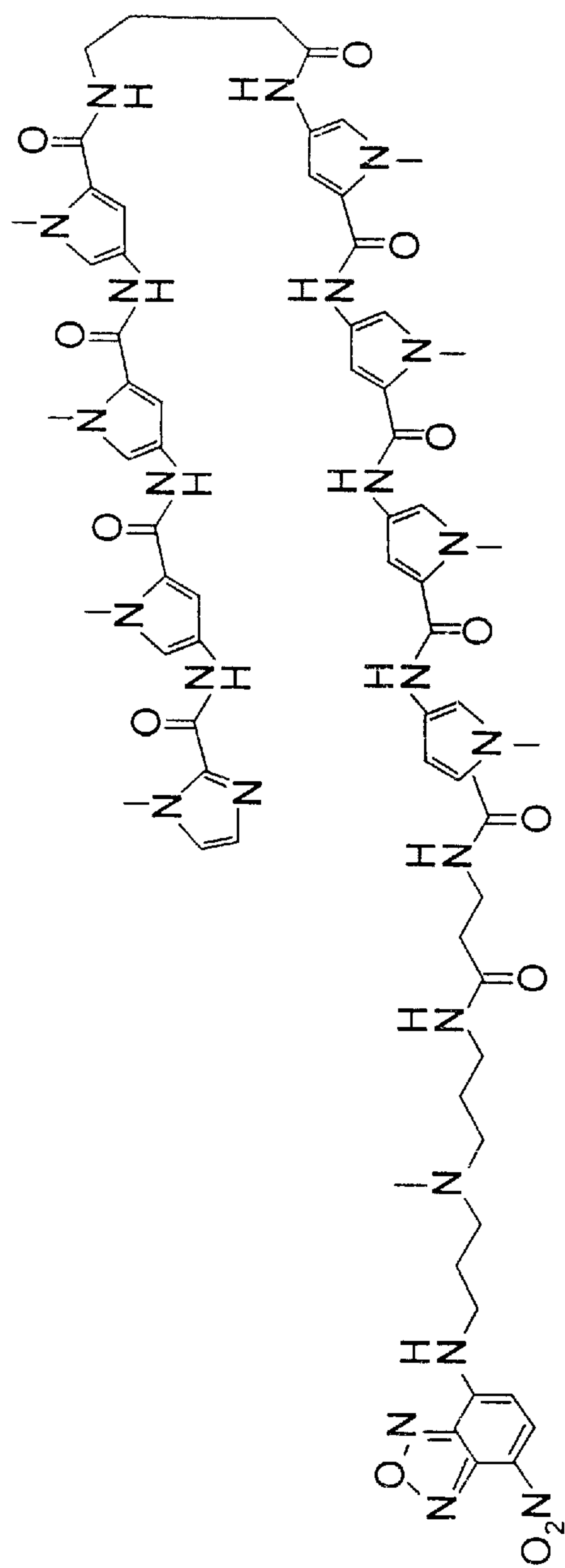
ImPyPyPy-γ-PyPyPyPy-β-Dp-NBD
