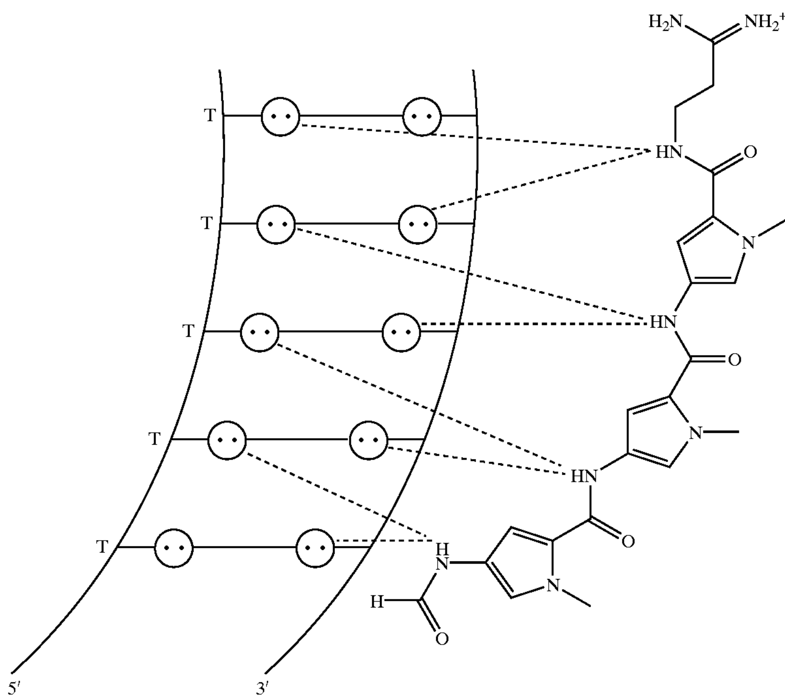
1:1 Distamycin•DNA Complex
