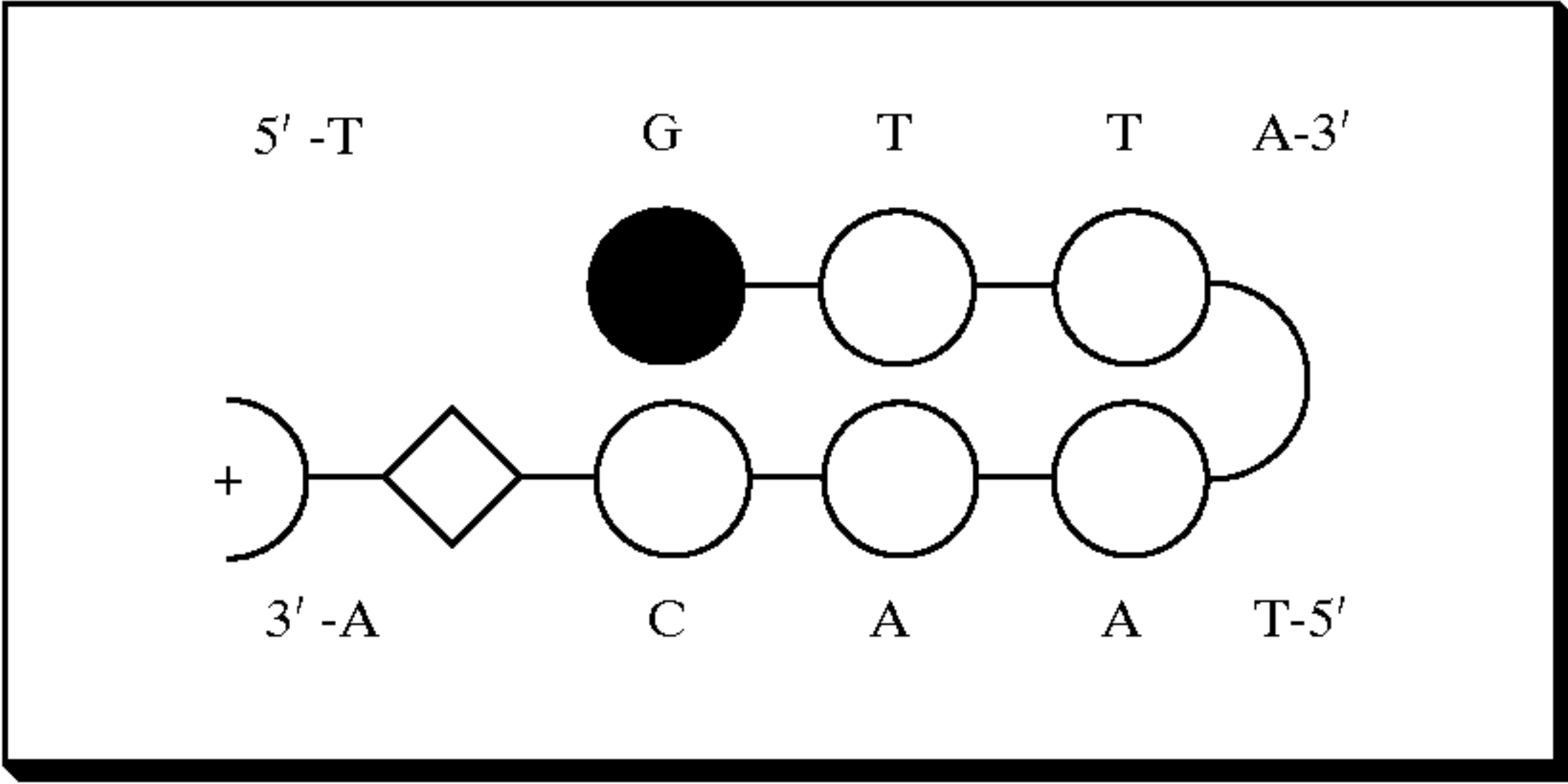
ImPyPy- \gamma -PyPyPy- \beta -Dp•5'-TGTTA-3'
