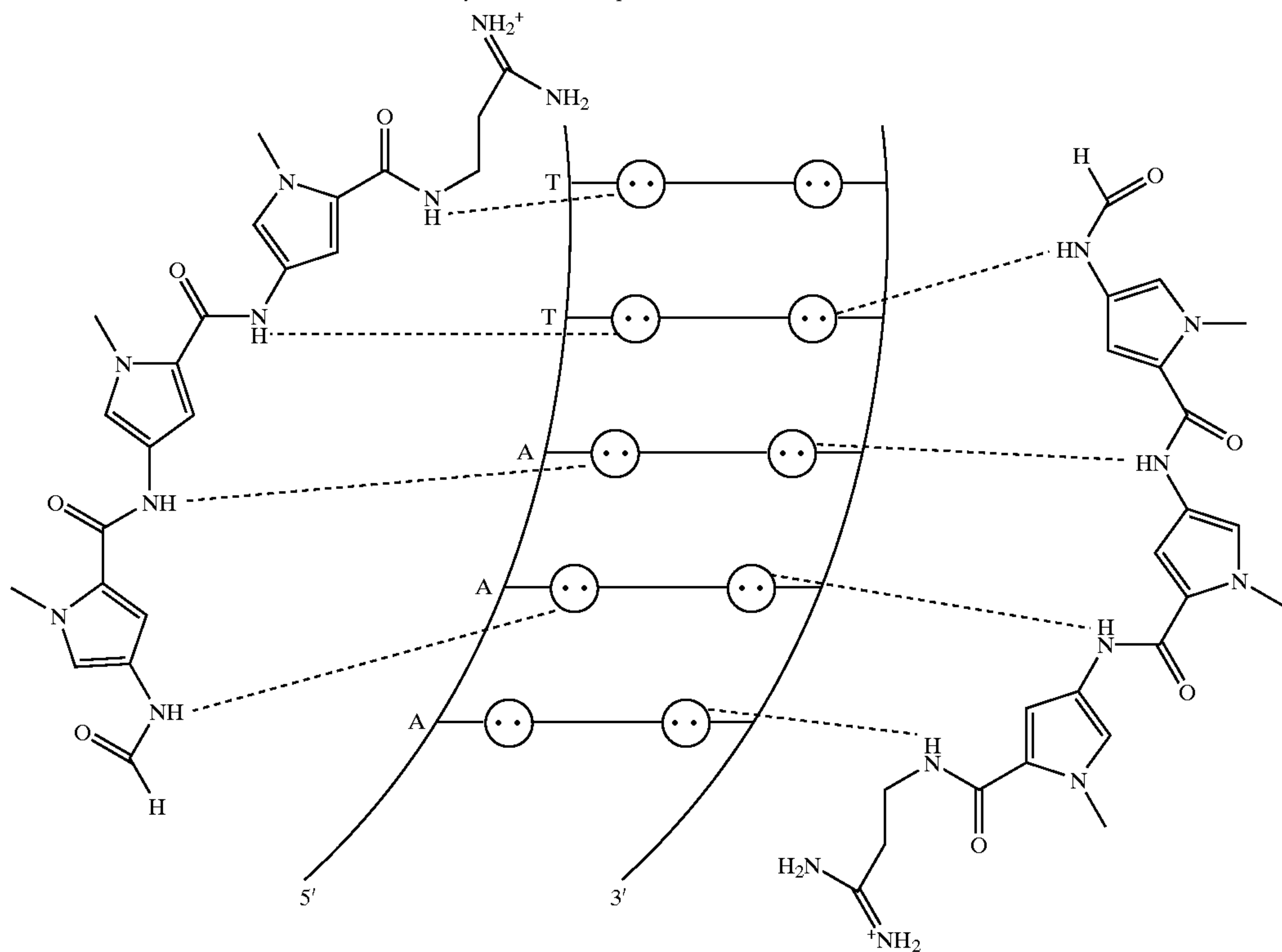
1:1 Distamycin•DNA Complex
