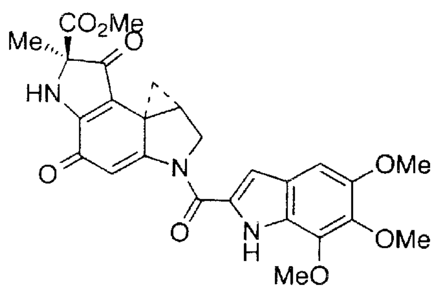
(+)- Duocarmycin A
