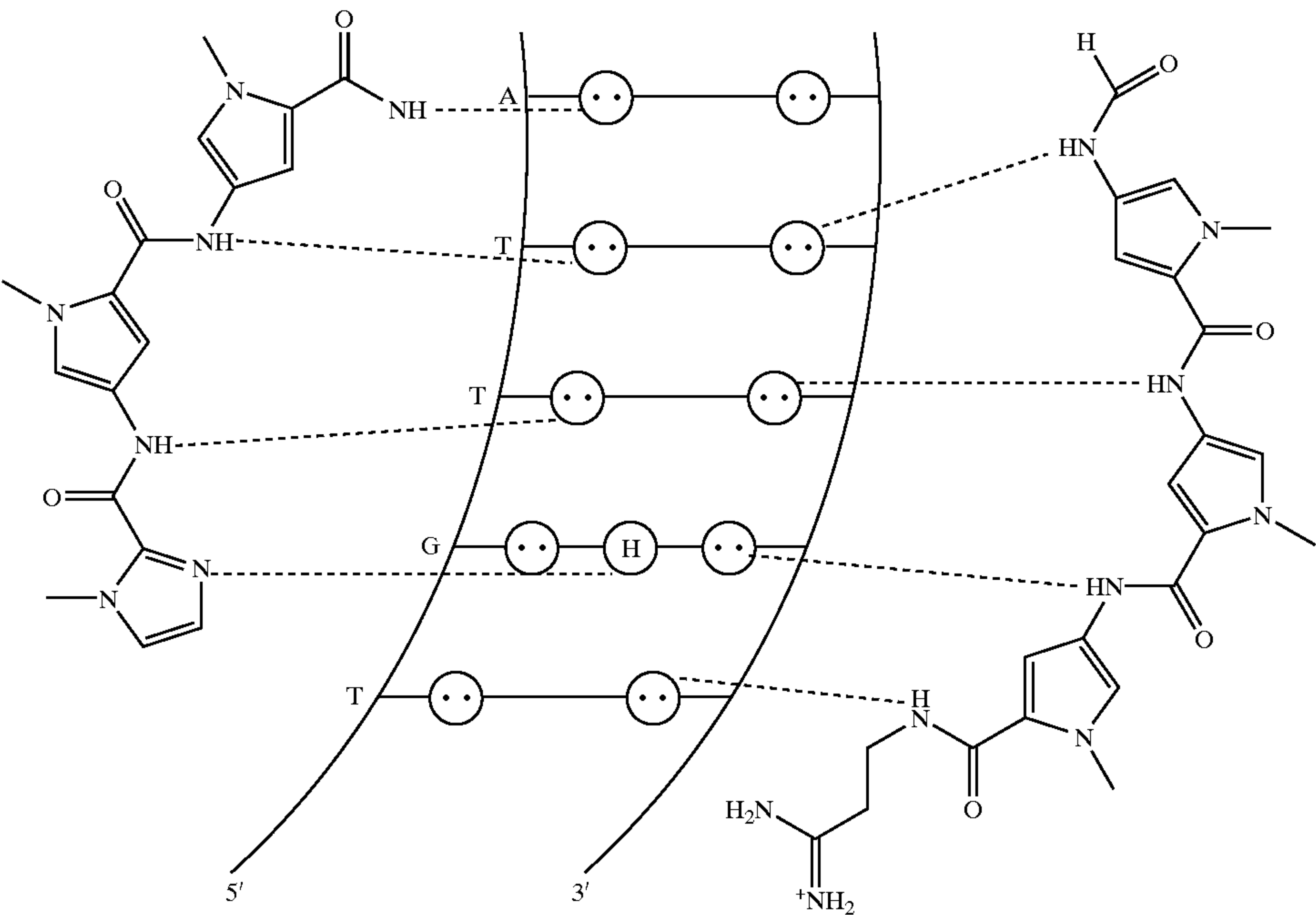
ImPyPy-Dp/PyPyPy•TGTТА K_a \sim 2 \times 10^5 M^{-1}
