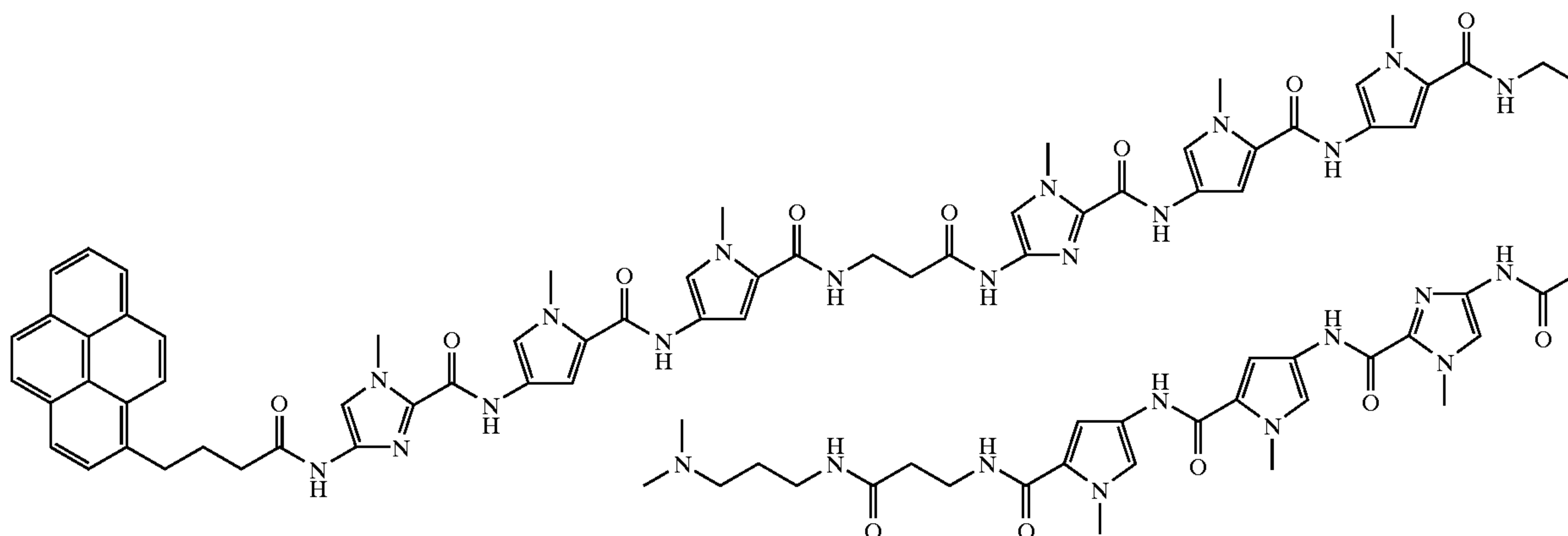
Pyrene-PyPyPy-β-ImPyPy-γ-ImPyPy-β-Dp
