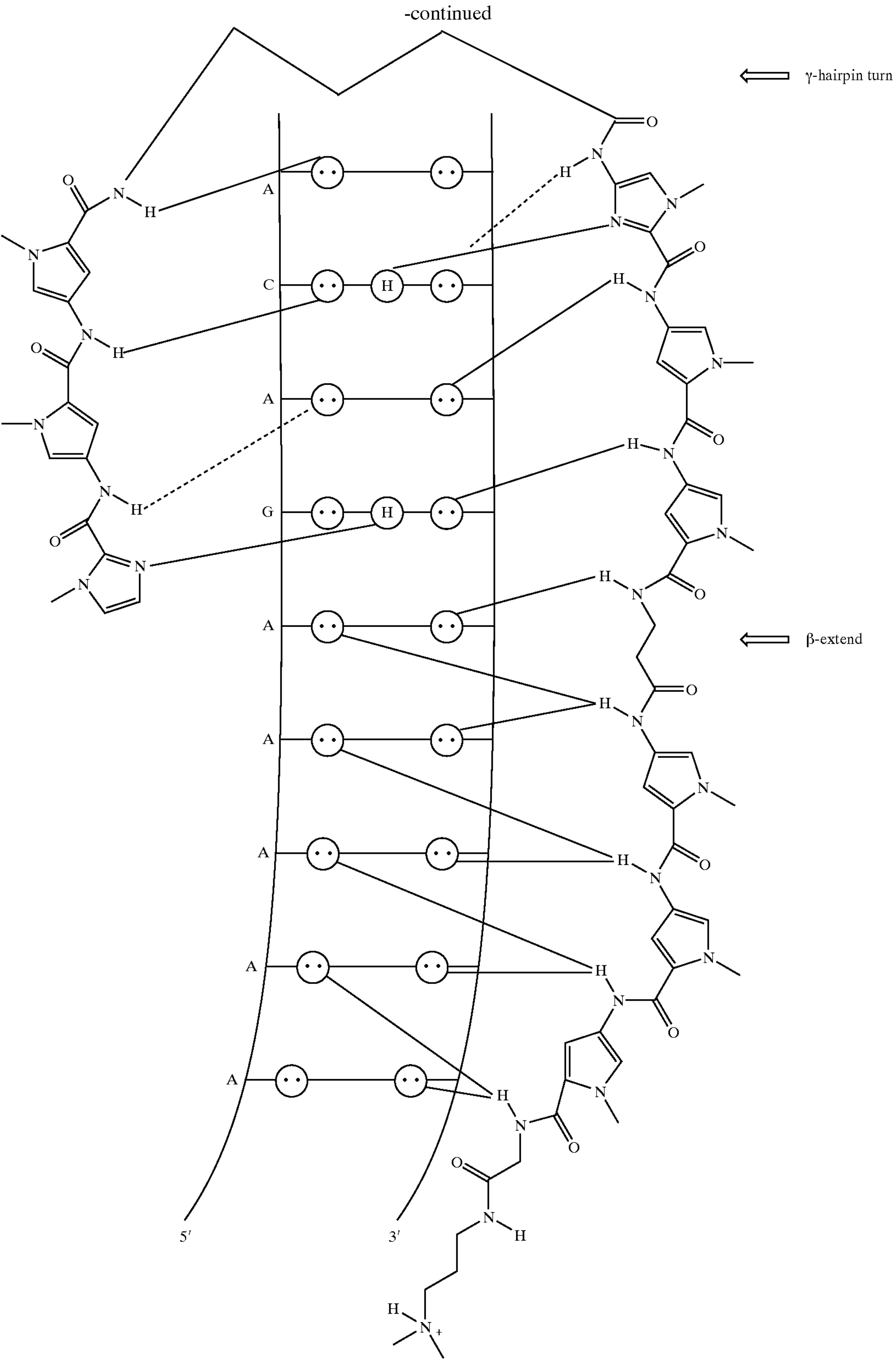
ImPyPy- \gamma -ImPyPy- \beta -PyPyPy-G-Dp K_a = 2 \times 10^{10} \text{ M}^{-1}
