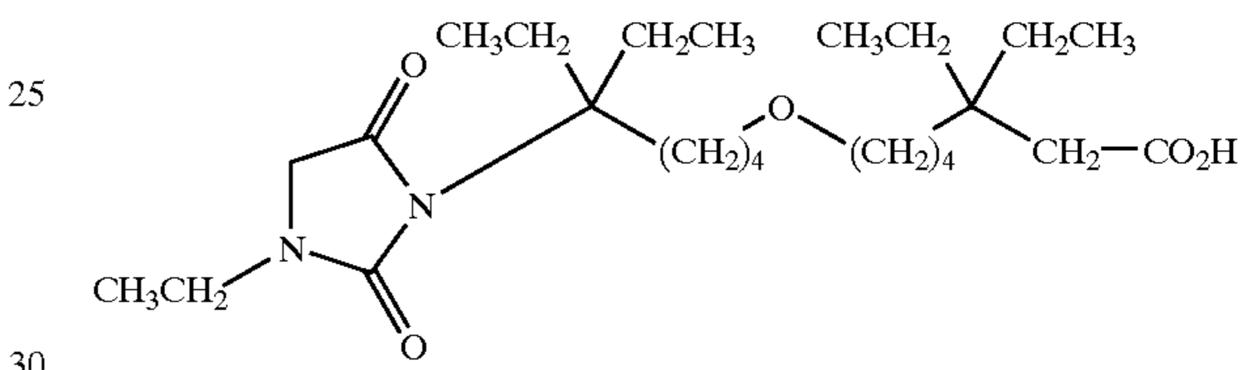
3,3-diethyl-7-[5-ethyl-5-(3-ethyl-2,5-dioxo-imidazolidine-1-yl)-heptyloxy]-heptanoic acid;
