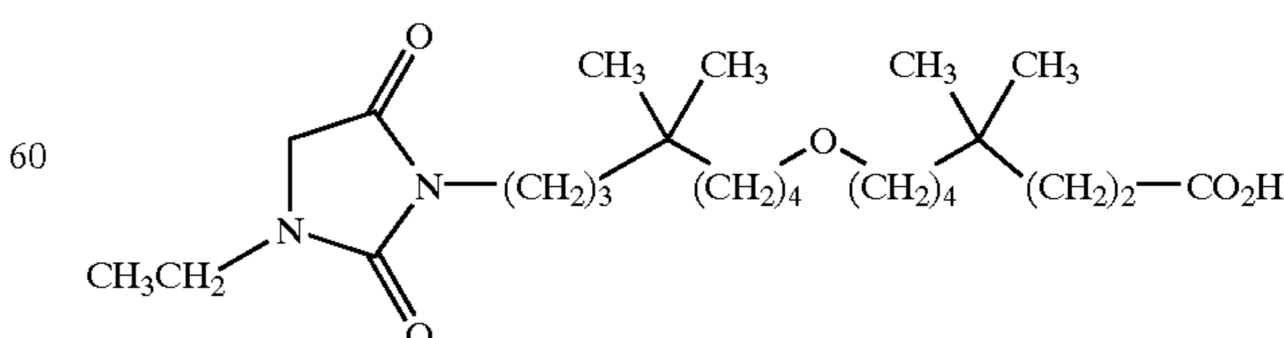
8-[8-(3-ethyl-2,5-dioxo-imidazolidin-1-yl)-5,5-dimethyl-octyloxy]-4,4-dimethyl-octanoic acid;
