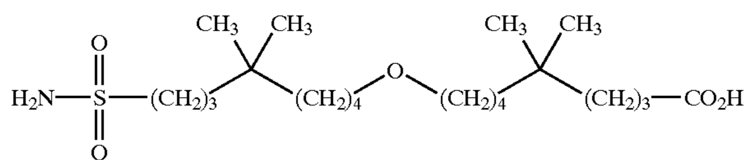
9-(5,5-dimethyl-8-sulfamoyl-octyloxy)-5,5-dimethylnonanoic acid;
