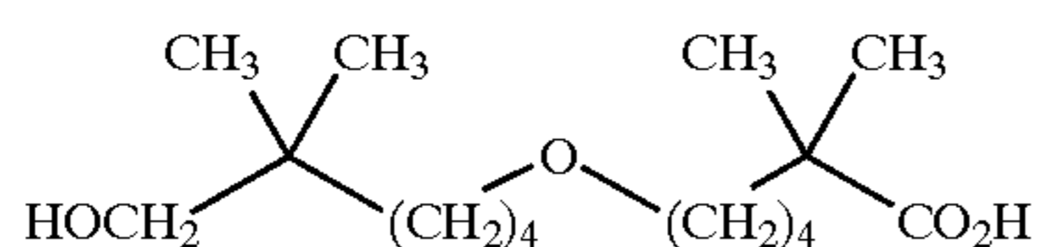
6-(6-hydroxy-5,5-dimethyl-hexyloxy)-2,2-dimethyl-hexanoic acid;
