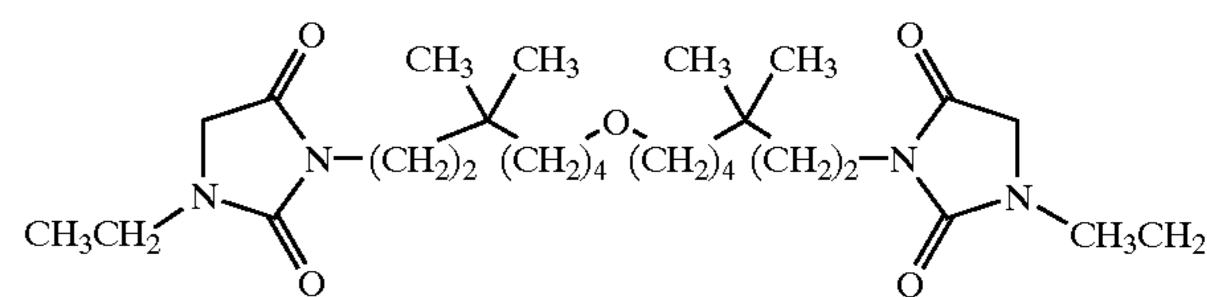
3-[7-(7-(3-ethyl-2,5-dioxo-imidazolidin-1-yl)-5,5-dimethyl-heptyloxy)-3,3-dimethyl-heptyl]-1-ethyl-imidazolidine-2,4-dione;
