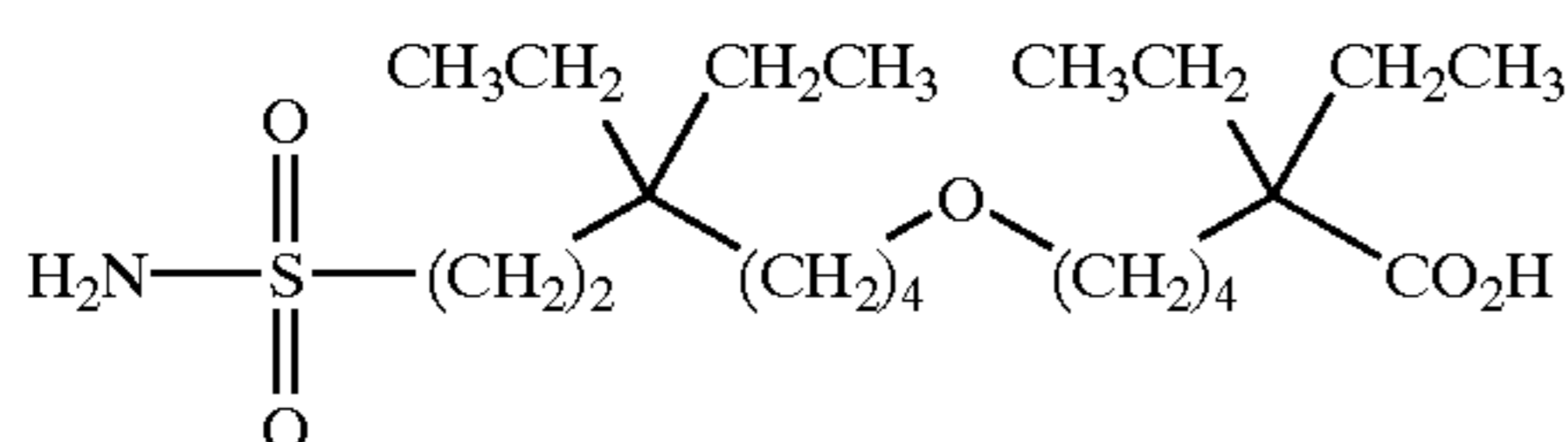
6-(5,5-diethyl-7-sulfamoyl-heptyloxy)-2,2-diethyl-hexanoic acid;
