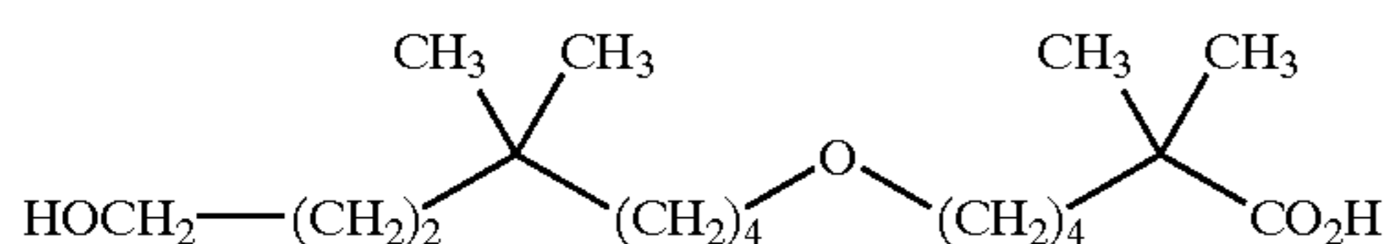
7-(7-hydroxy-5,5-dimethyl-heptyloxy)-3,3-dimethyl-heptanoic acid;
