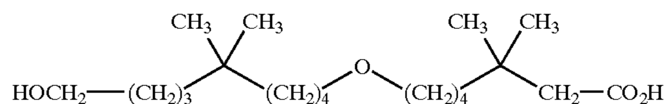
20-(9-hydroxy-5,5-dimethyl-nonyloxy)-3,3-dimethyl-heptanoic acid;
