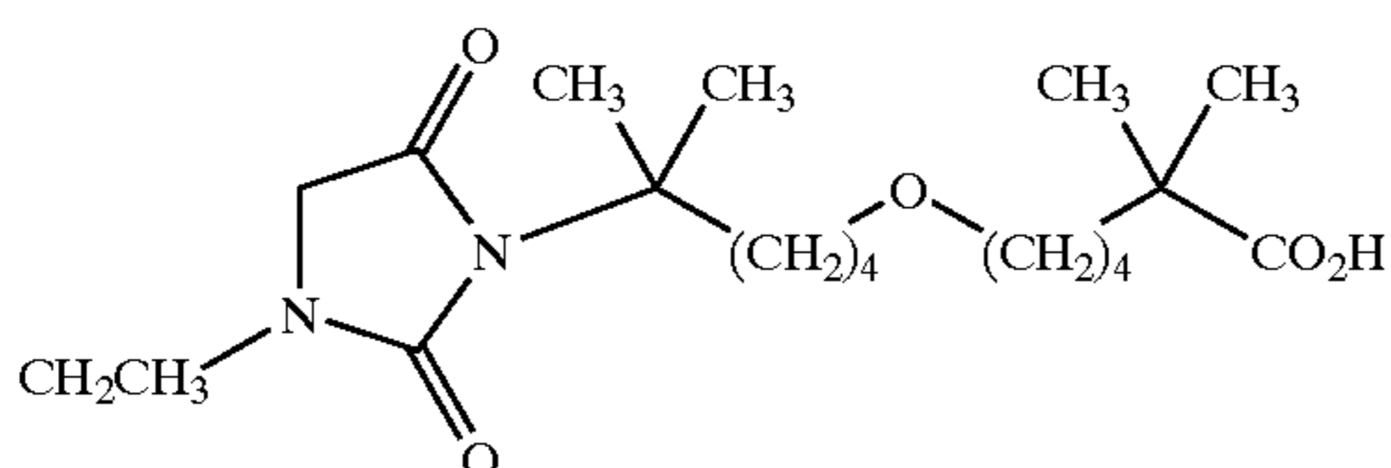
6-[5-(3-ethyl-2,5-dioxo-imidazolidin-1-yl)-5-methyl-hexyloxy]-2,2-dimethyl-hexanoic acid;
