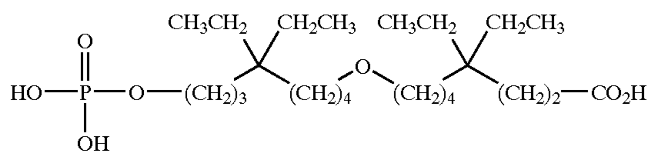
8-(5,5-diethyl-8-phosphonoxy-octyloxy)-4,4-diethyloctanoic acid;
