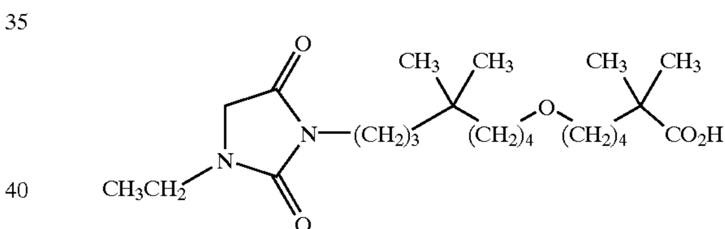
8-[7-(3-ethyl-2,5-dioxo-imidazolidin-1-yl)-5,5-dimethyl-heptyloxy]-4,4-dimethyl-octanoic acid;
