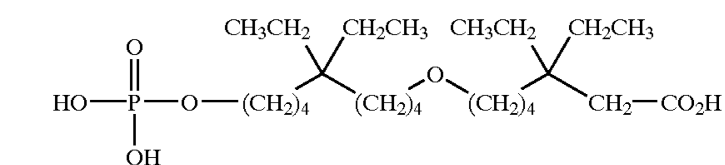
7-(5,5-diethyl-9-phosphonoxy-nonyloxy)-3,3-diethylheptanoic acid;
