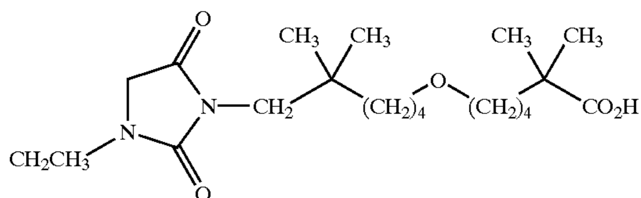
6-[6-(3-ethyl-2,5-dioxo-imidazolidin-1-yl)-5,5-dimethyl-hexyloxy]-2,2-dimethyl-hexanoic acid;
