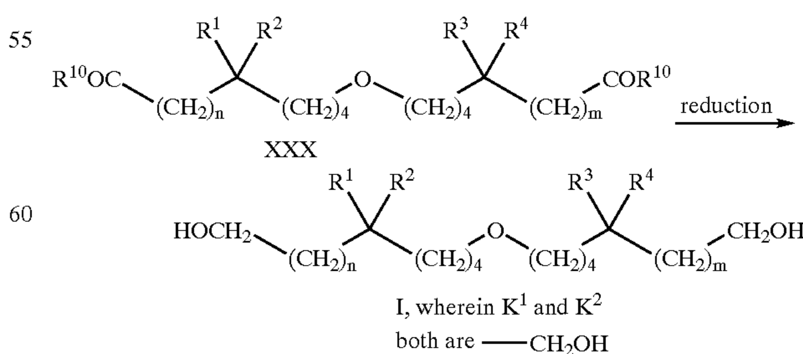
SCHEME 9: Synthesis of compounds of formula I, wherein K 1 and K 2 are both —CH 2 OH
