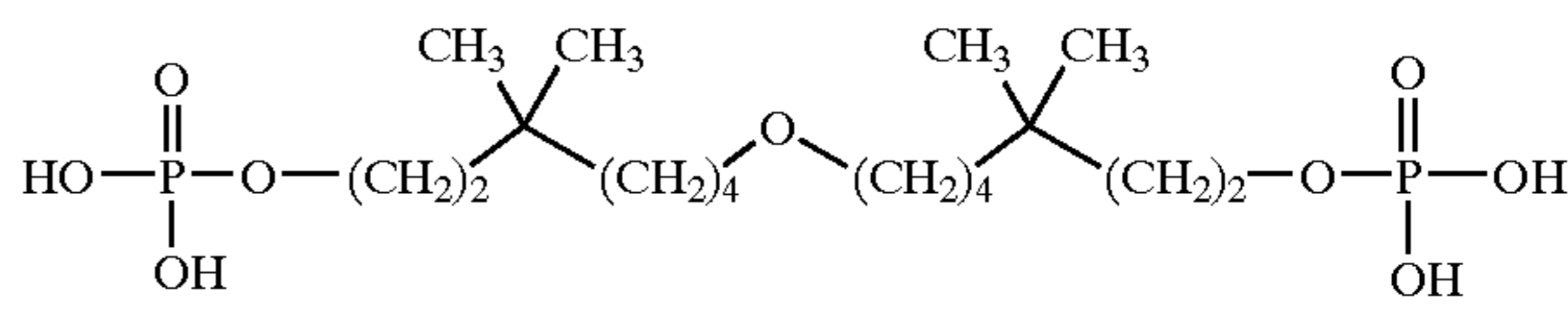
phosphoric acid mono-[7-(5,5-dimethyl-7-phosphonoxy-heptyloxy)-3,3-dimethyl-heptyl]ester;
