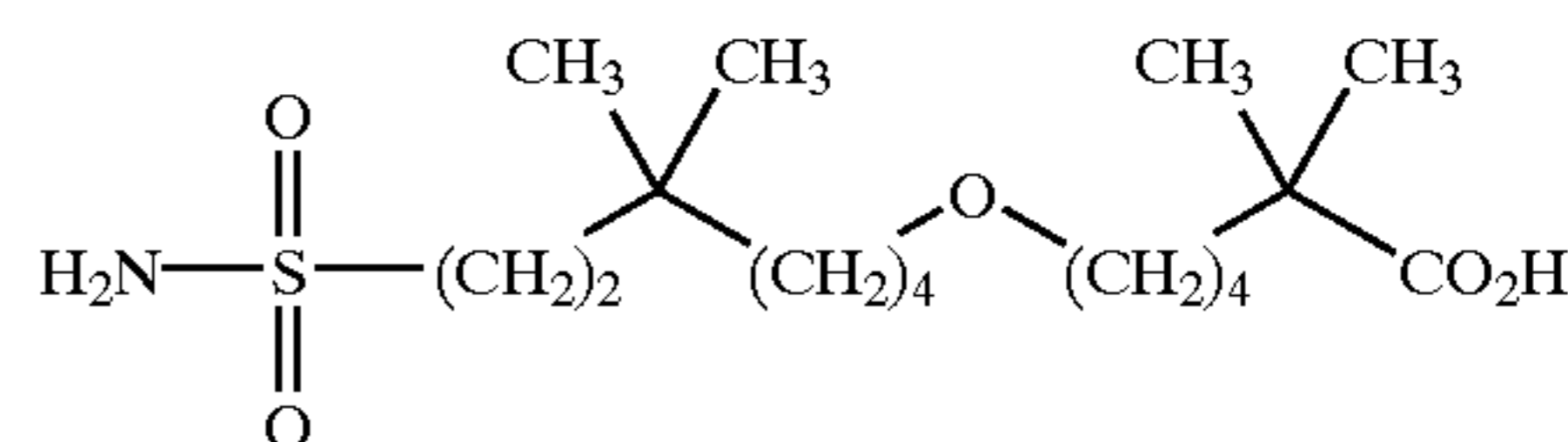
6-(5,5-dimethyl-7-sulfamoyl-heptyloxy)-2,2-dimethyl-hexanoic acid;
