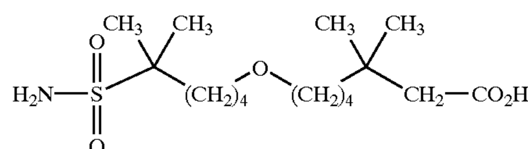
3,3-dimethyl-7-(5-methyl-5-sulfamoyl-hexyloxy)-heptanoic acid;
