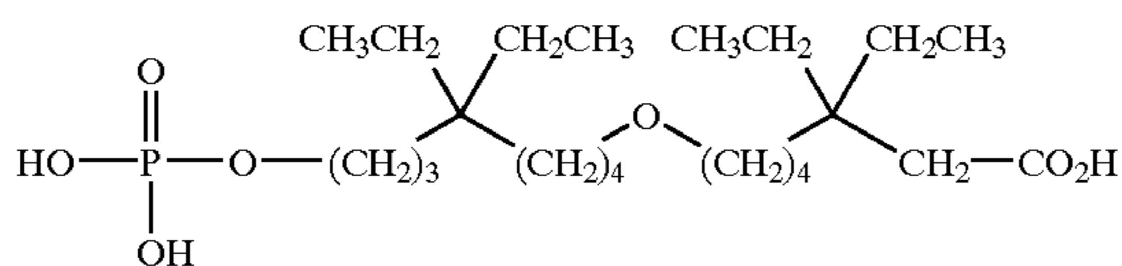
7-(5,5-diethyl-8-phosphonoxy-octyloxy)-3,3-diethylheptanoic acid;
