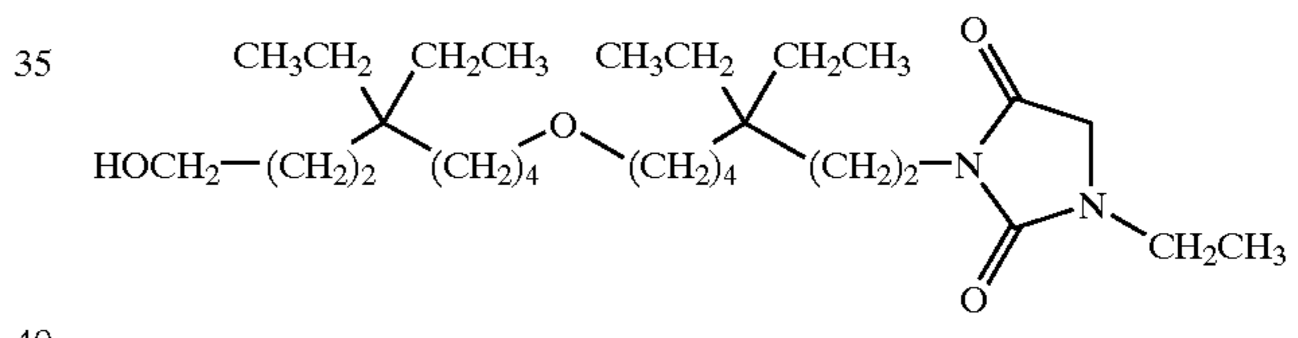
3-[6-(5,5-diethyl-8-hydroxy-octyloxy)-2,2-diethyl-hexyl]-1-ethyl-imidazolidine-2,4-dione;
