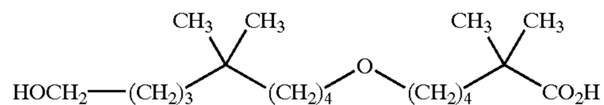
10-(9-hydroxy-5,5-dimethyl-nonyloxy)-2,2-dimethyl-hexanoic acid;
