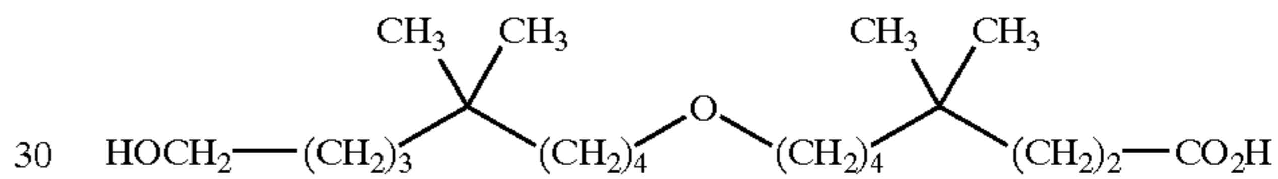
30-(6-hydroxy-5,5-dimethyl-hexyloxy)-4,4-dimethyl-octanoic acid;
