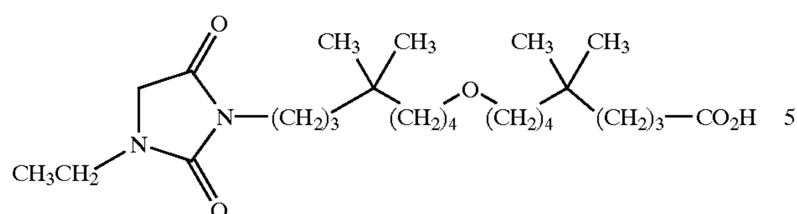
9-[8-(3-ethyl-2,5-dioxo-imidazolidin-1-yl)-5,5-dimethyl-octyloxy]-5,5-dimethyl-nonanoic acid;
