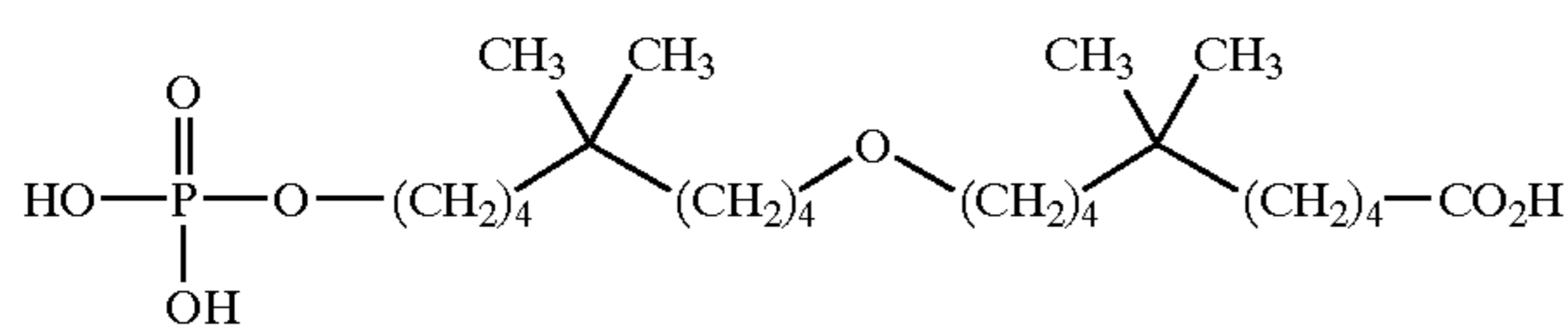
10-(5,5-dimethyl-9-phosphonoxy-nonyloxy)-6,6-dimethyl-decanoic acid;
