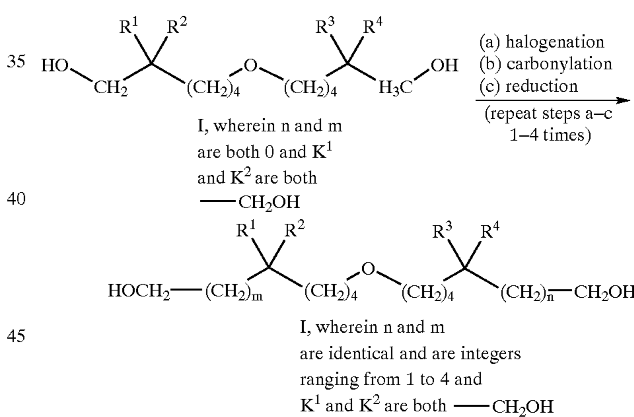
SCHEME 8: Synthesis of compounds of Formula I, wherein n and m are identical integers ranging from 1 to 4 and K 1 and K 2 are both —CH 2 OH
