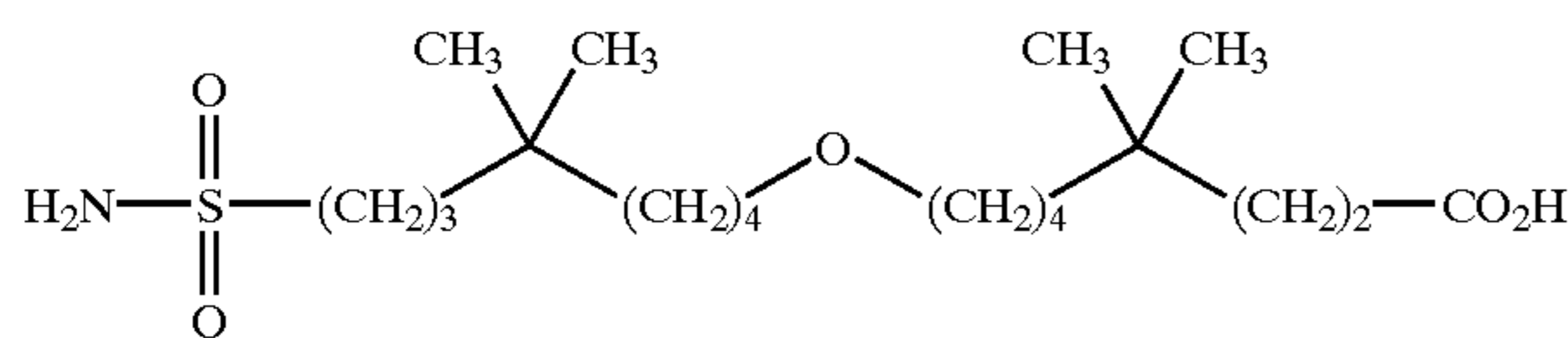
8-(5,5-dimethyl-8-sulfamoyl-octyloxy)-4,4-dimethyloctanoic acid;
