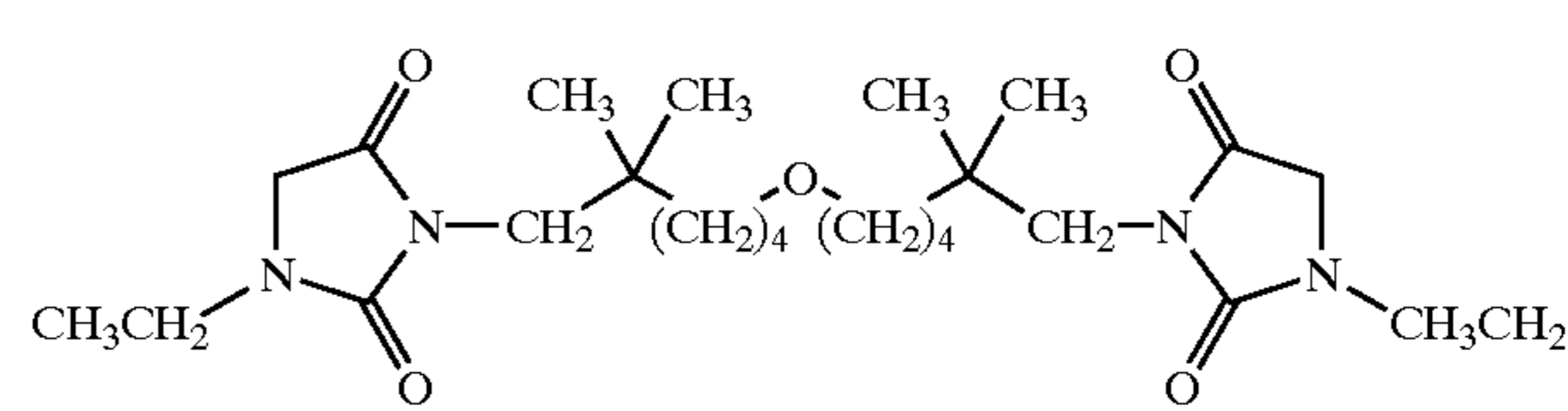
3-[6-(6-(3-ethyl-2,5-dioxo-imidazolidin-1-yl)-5,5-dimethyl-hexyloxy)-2,2-dimethyl-hexyl]-1-ethyl-imidazolidine-2,4-dione;
