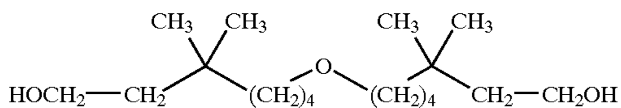
7-(7-hydroxy-5,5-dimethyl-heptyloxy)-3,3-dimethyl-heptan-1-ol;
