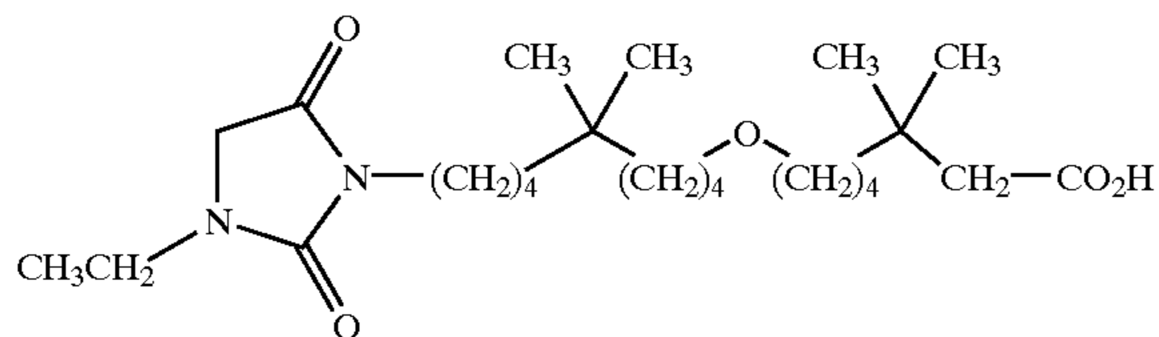
7-[9-(3-ethyl-2,5-dioxo-imidazolidin-1-yl)-5,5-dimethyl-nonyloxy]-3,3-dimethyl-heptanoic acid;
