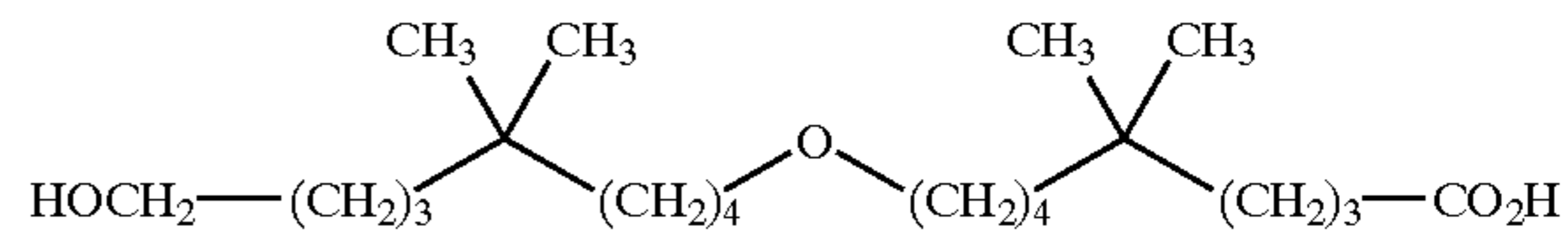
40-(7-hydroxy-5,5-dimethyl-heptyloxy)-5,5-dimethyl-nonanoic acid;
