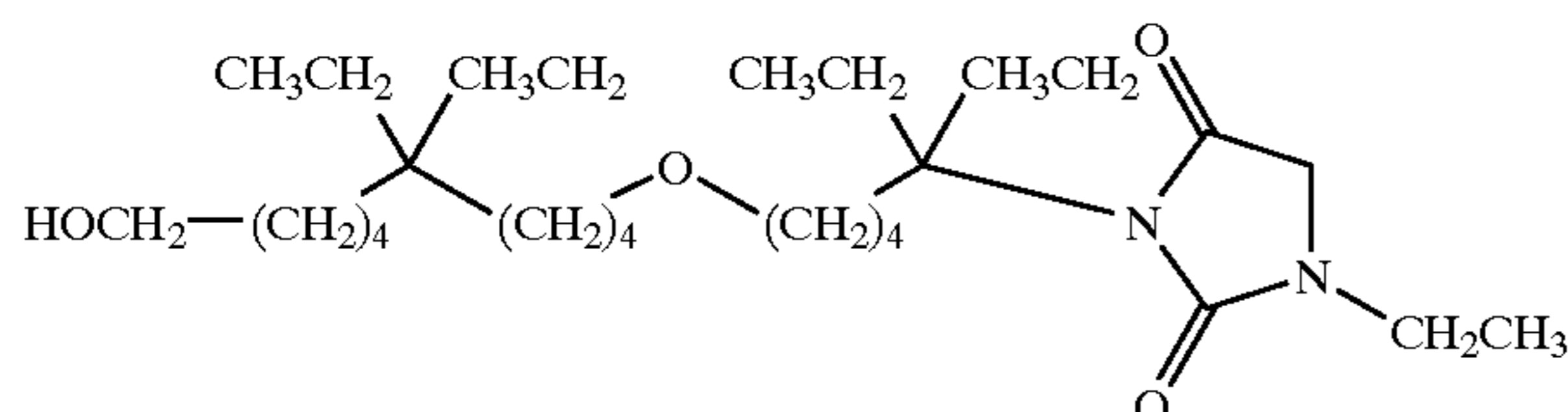
3-[5-(5,5-diethyl-10-hydroxy-decyloxy)-1,1-diethyl-pentyl]-1-ethyl-imidazolidine-2,4-dione;
