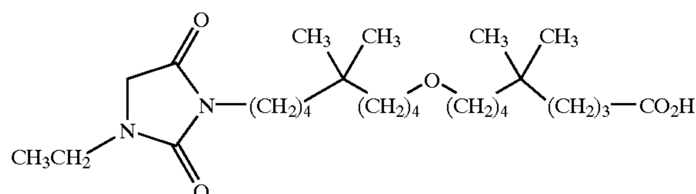
8-[9-(3-ethyl-2,5-dioxo-imidazolidin-1-yl)-5,5-dimethyl-nonyloxy]-4,4-dimethyl-octanoic acid;
