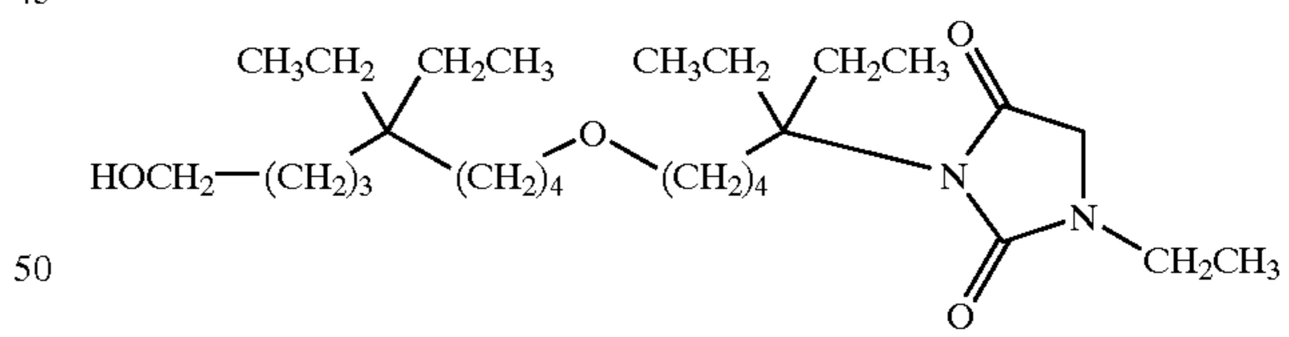
3-[7-(5,5-diethyl-8-hydroxy-octyloxy)-3,3-diethyl-heptyl]-1-ethyl-imidazolidine-2,4-dione;
