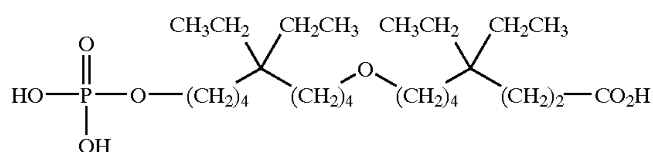
7-(5,5-diethyl-9-phosphonoxy-nonyloxy)-3,3-diethylheptanoic acid;
