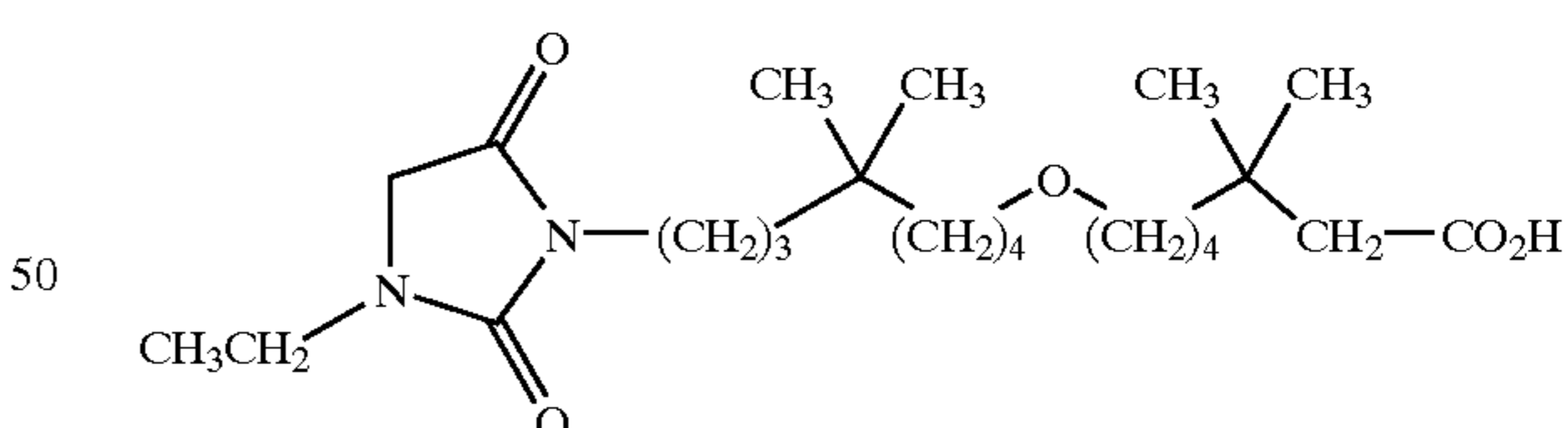
6-[8-(3-ethyl-2,5-dioxo-imidazolidin-1-yl)-5,5-dimethyl-octyloxy]-2,2-dimethyl-hexanoic acid;
