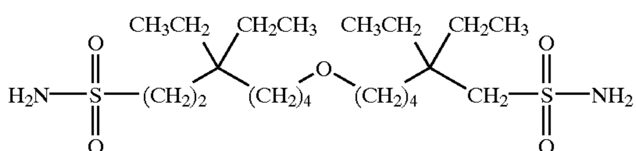
3,3-diethyl-7-(5-ethyl-5-sulfamoylmethyl-heptyloxy)-heptane-1-sulfonic acid amide;
