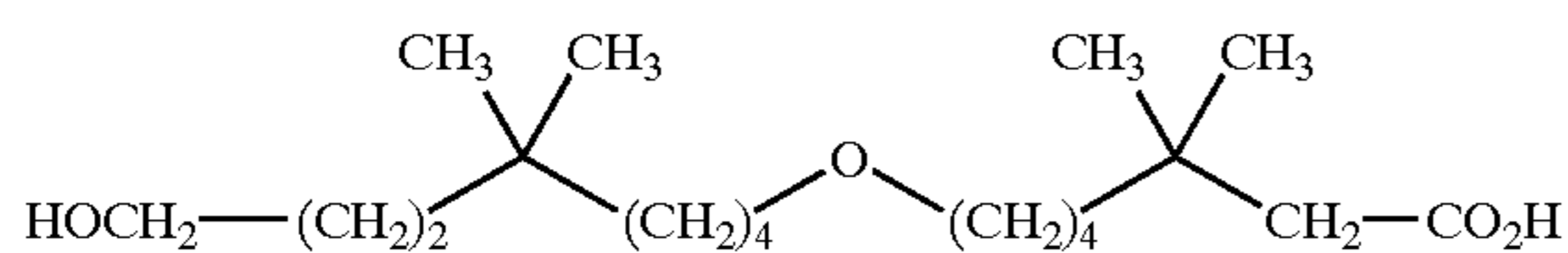
7-(8-hydroxy-5,5-dimethyl-octyloxy)-3,3-dimethyl-heptanoic acid;
