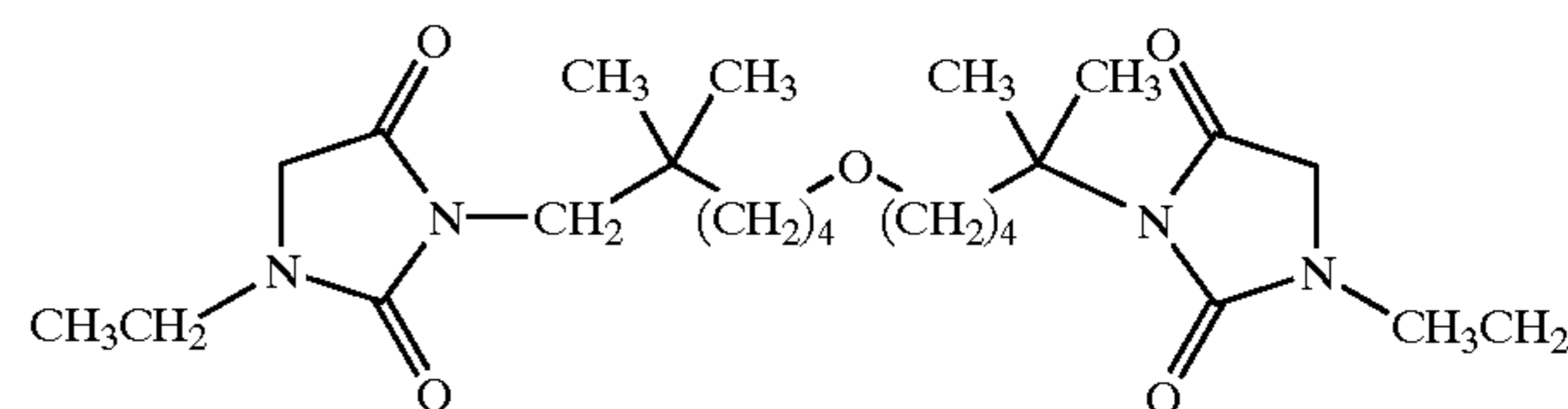
3-[5-(6-(3-ethyl-2,5-dioxo-imidazolidin-1-yl)-5,5-dimethyl-hexyloxy)-1,1-dimethyl-pentyl]-1-ethyl-imidazolidine-2,4-dione;
