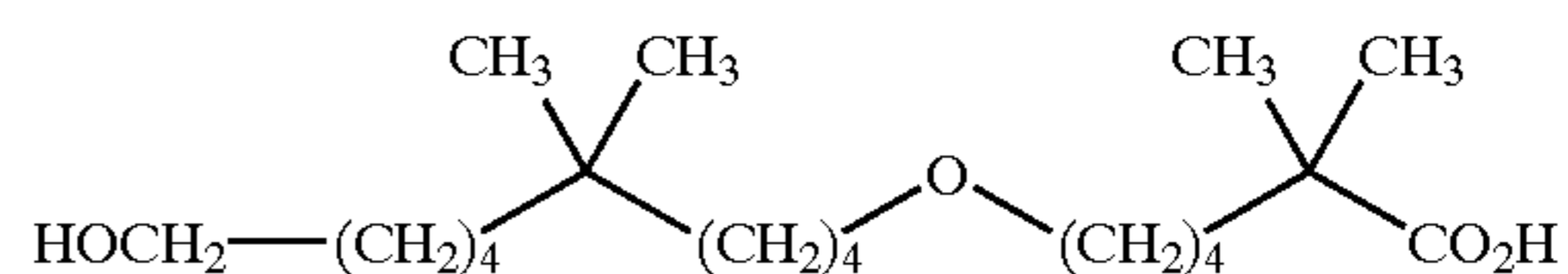
45-(10-hydroxy-5,5-dimethyl-decyloxy)-2,2-dimethyl-hexanoic acid;
