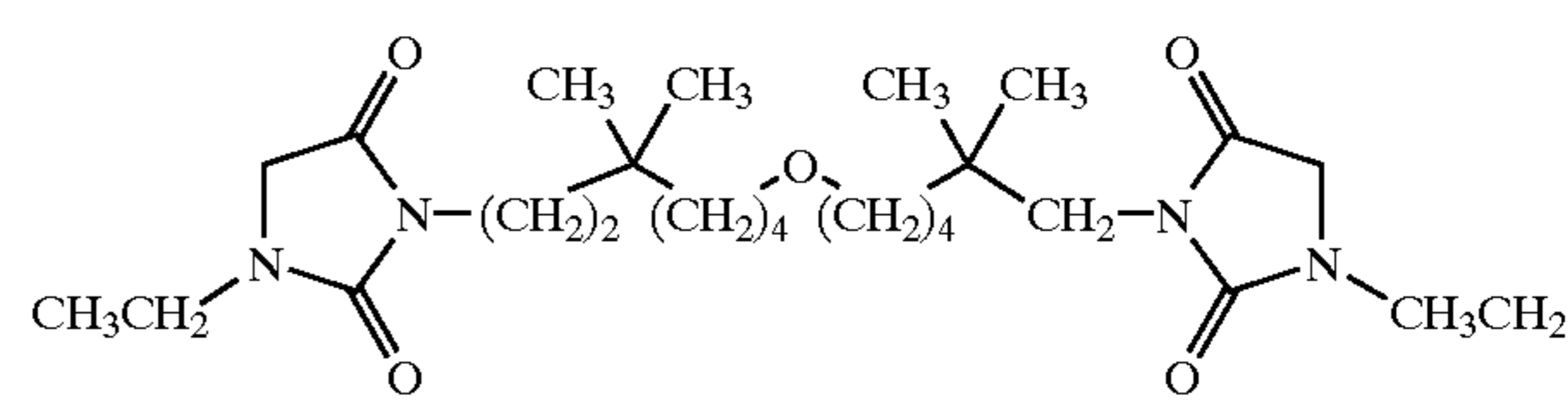
3-[6-(7-(3-ethyl-2,5-dioxo-imidazolidin-1-yl)-5,5-dimethyl-heptyloxy)-2,2-dimethyl-hexyl]-1-ethyl-imidazolidine-2,4-dione;
