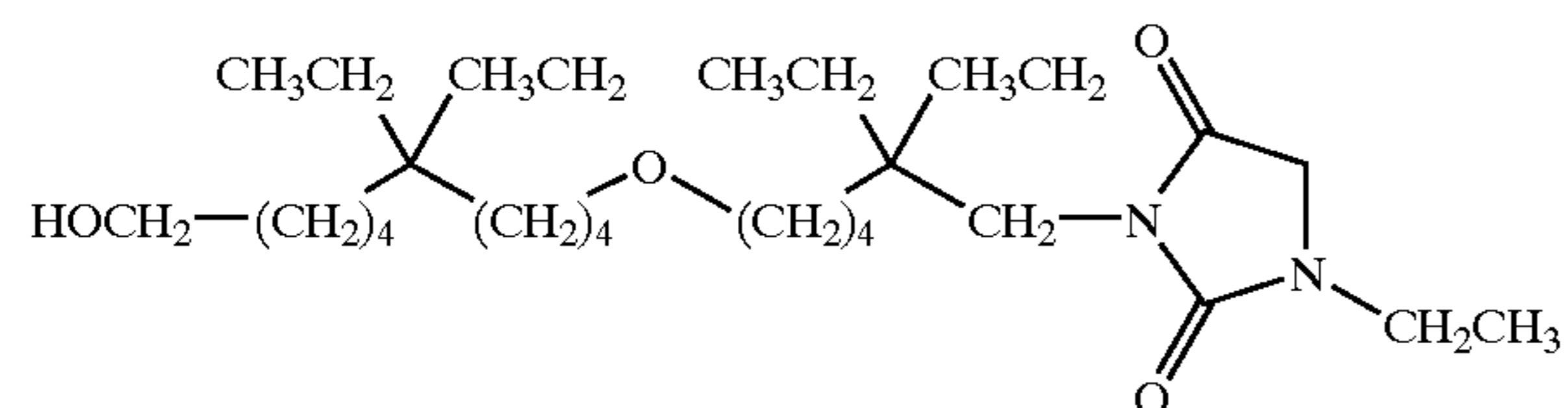
3-[6-(5,5-diethyl-10-hydroxy-decyloxy)-2,2-diethyl-hexyl]-1-ethyl-imidazolidine-2,4-dione;
