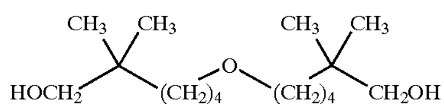
6-(6-hydroxy-5,5-dimethyl-hexyloxy)-2,2-dimethyl-hexan-1-ol;
