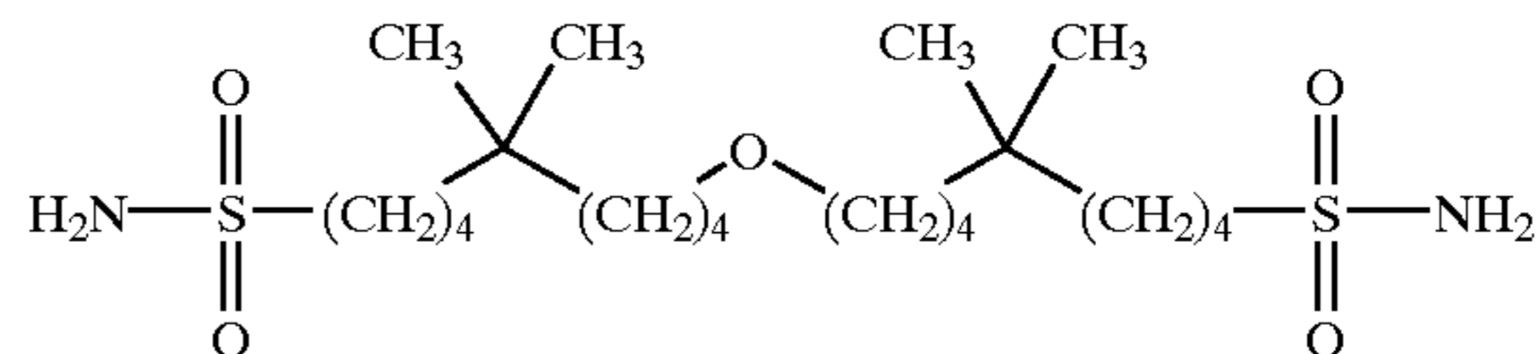
9-(5,5-dimethyl-9-sulfamoyl-octyloxy)-5,5-dimethylnonane-1-sulfonic acid amide;
