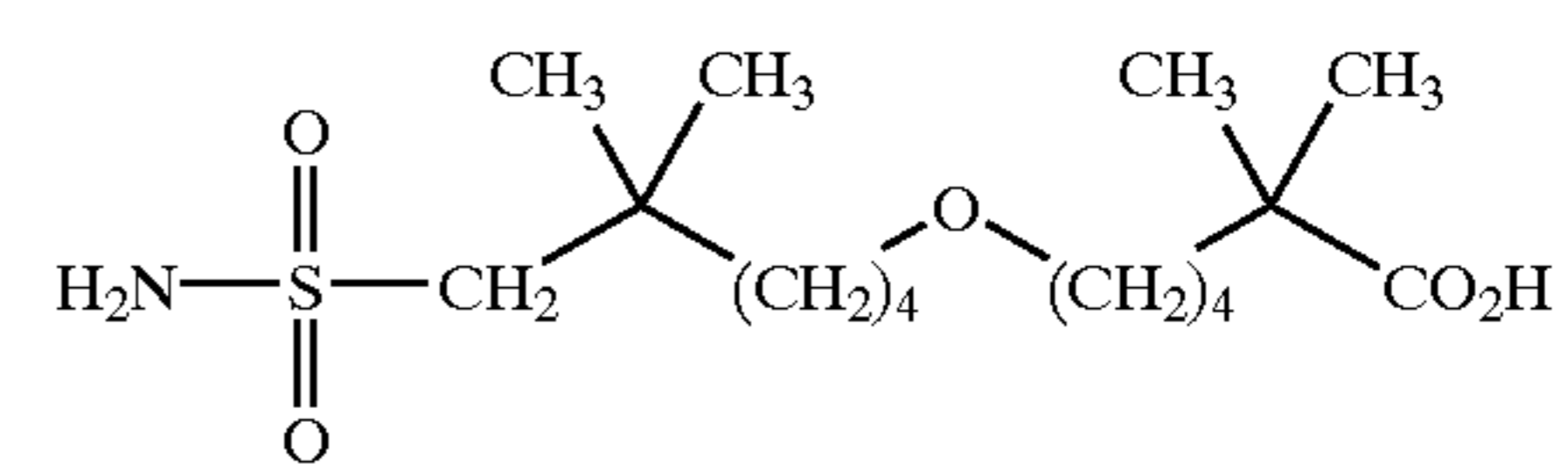
6-(5,5-dimethyl-6-sulfamoyl-hexyloxy)-2,2-dimethyl-hexanoic acid;
