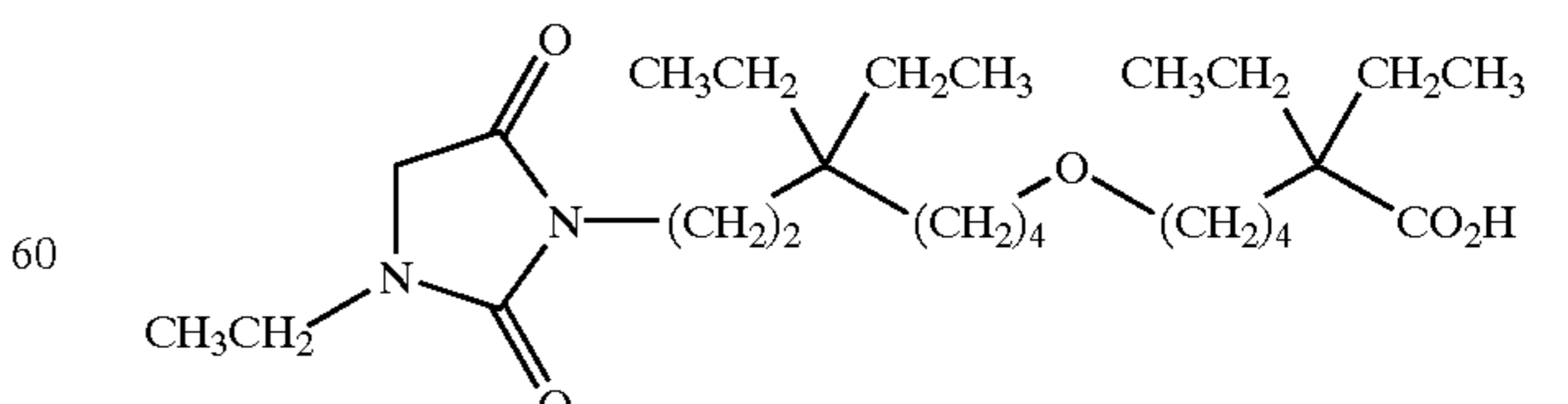
3,3-diethyl-7-[5-ethyl-5-(3-ethyl-2,5-dioxo-imidazolidine-1-ylmethyl)-heptyloxy]-heptanoic acid;
