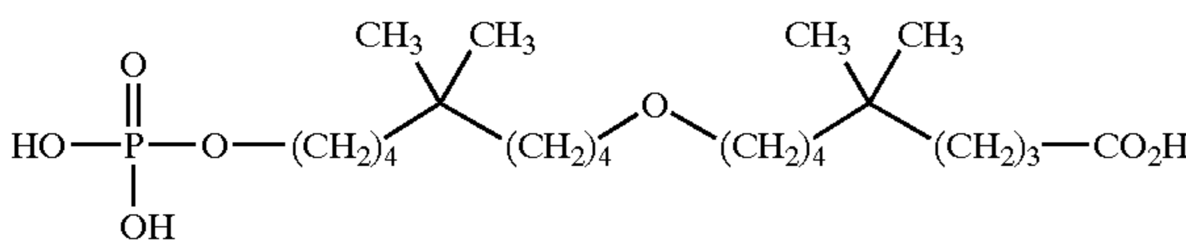
9-(5,5-dimethyl-9-phosphonoxy-nonyloxy)-5,5-dimethylnonanoic acid;
