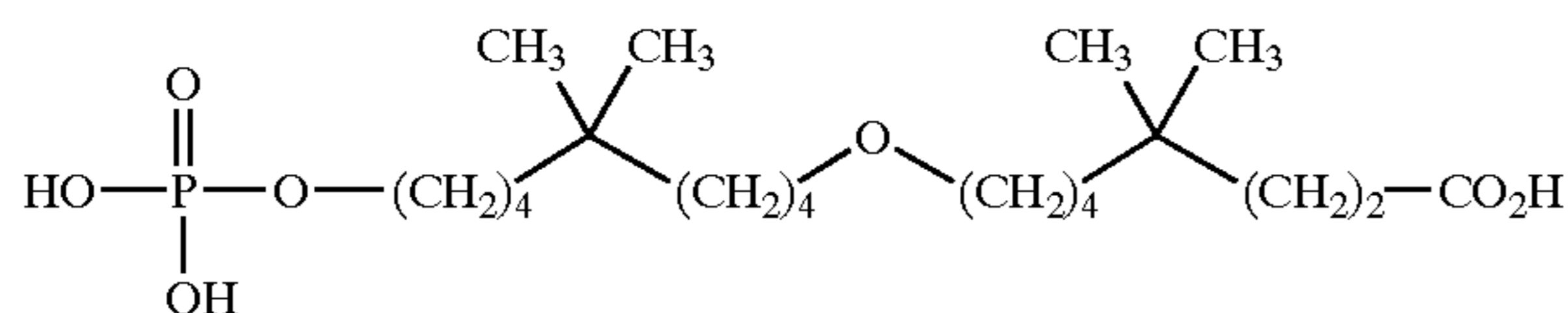
8-(5,5-dimethyl-9-phosphonoxy-nonyloxy)-4,4-dimethyloctanoic acid;
