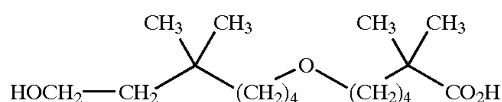
6-(7-hydroxy-5,5-dimethyl-heptyloxy)-2,2-dimethyl-hexanoic acid;
