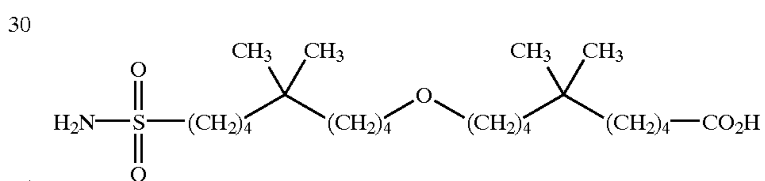
9-(5,5-dimethyl-9-sulfamoyl-nonyloxy)-5,5-dimethylnonanoic acid;
