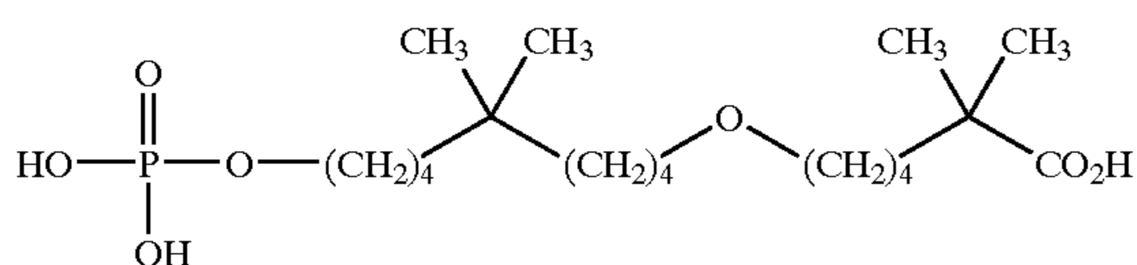
6-(5,5-dimethyl-9-phosphonoxy-nonyloxy)-2,2-dimethylhexanoic acid;
