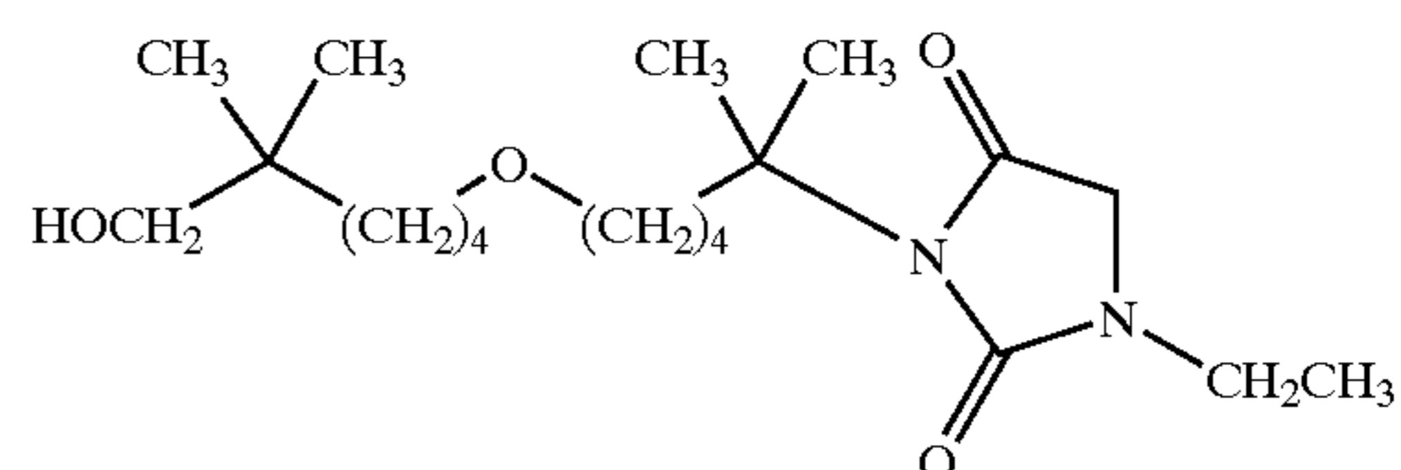
1-ethyl-3-[5-(6-hydroxy-5,5-dimethyl-hexyloxy)-1,1-dimethyl-pentyl]-imidazolidine-2,4-dione;
