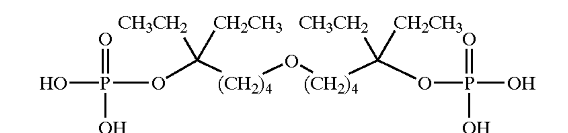
10-(5,5-diethyl-9-phosphonoxy-nonyloxy)-6,6-diethyldecanoic acid;
