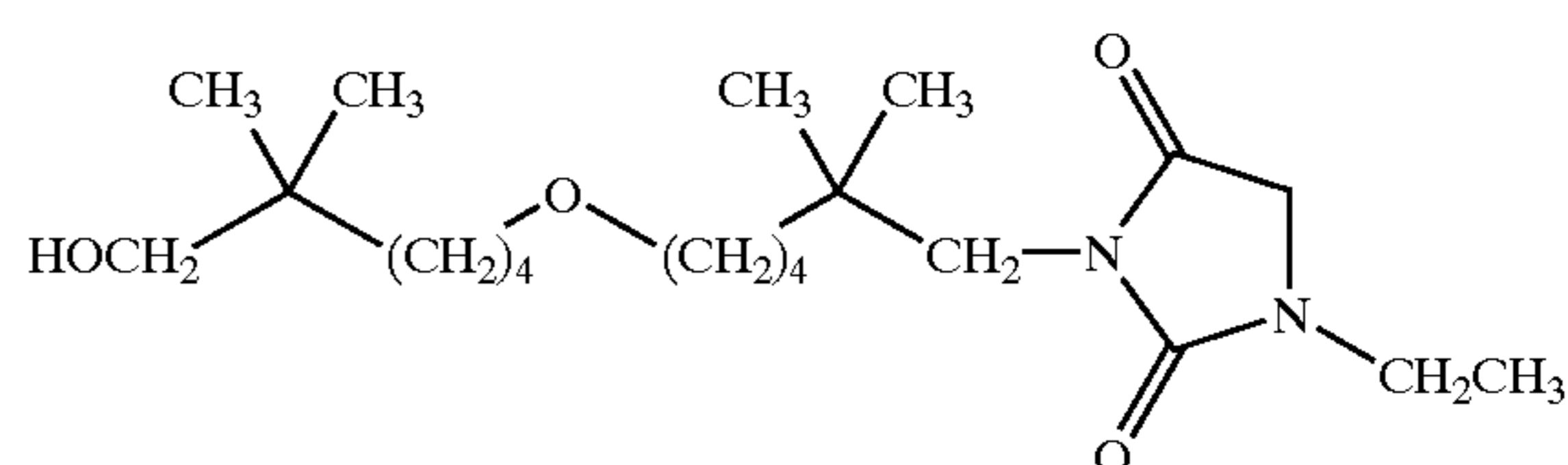
1-ethyl-3-[6-(6-hydroxy-5,5-dimethyl-hexyloxy)-2,2-dimethyl-hexyl]-imidazolidine-2,4-dione;
