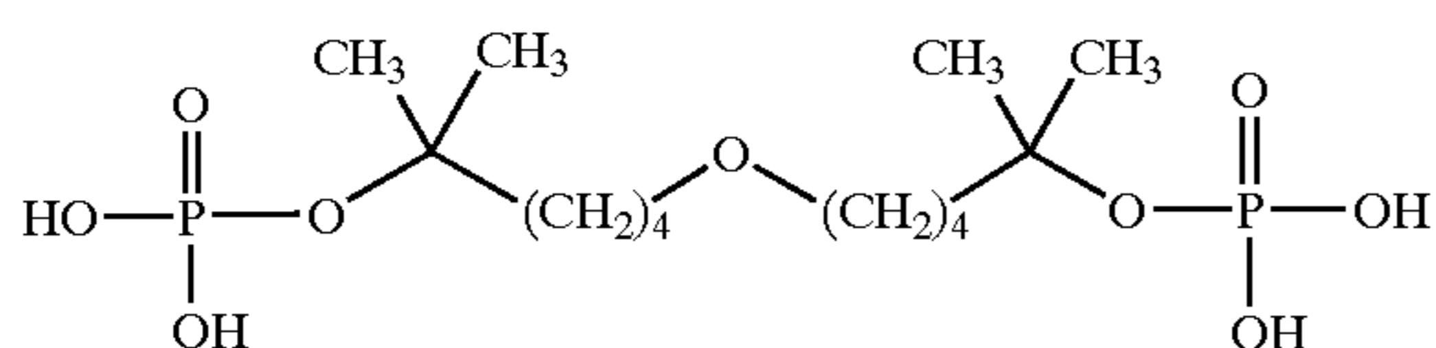
10-(5,5-dimethyl-9-phosphonoxy-nonyloxy)-6,6-dimethyl-decanoic acid;
