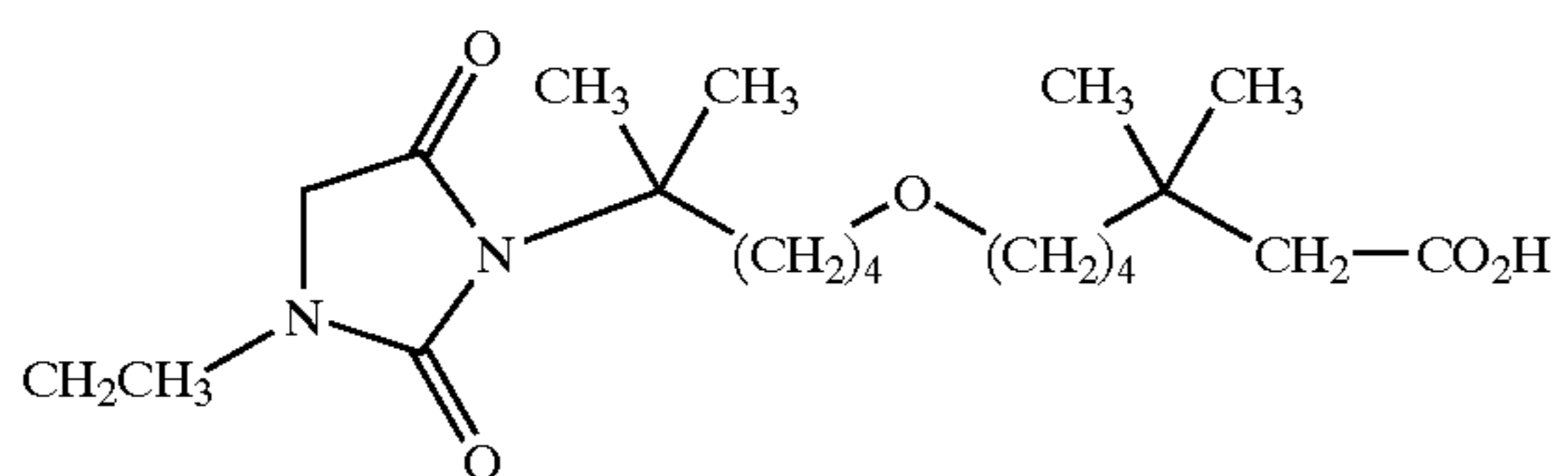
7-[5-(3-ethyl-2,5-dioxo-imidazolidin-1-yl)-5-methyl-hexyloxy]-3,3-dimethyl-heptanoic acid;
