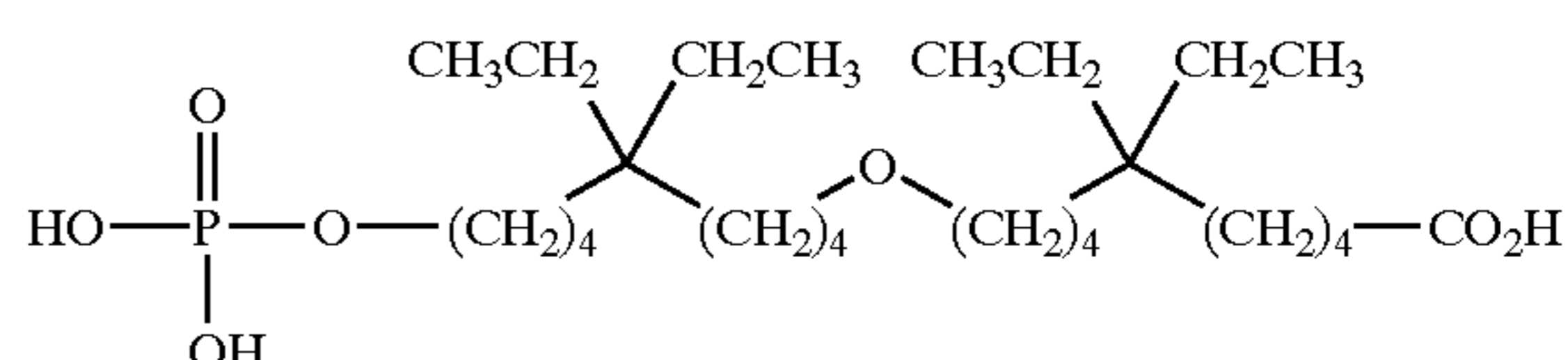
9-(5,5-diethyl-9-phosphonoxy-nonyloxy)-5,5-diethylnonanoic acid;
