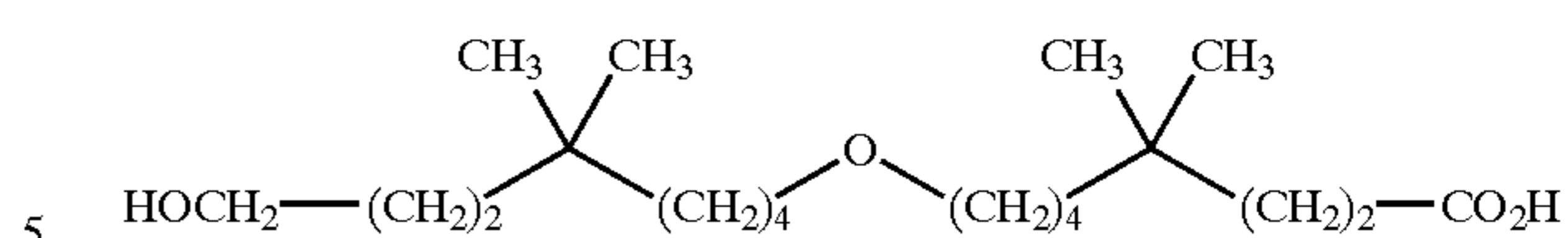
8-(8-hydroxy-5,5-dimethyl-octyloxy)-4,4-dimethyl-octanoic acid;
