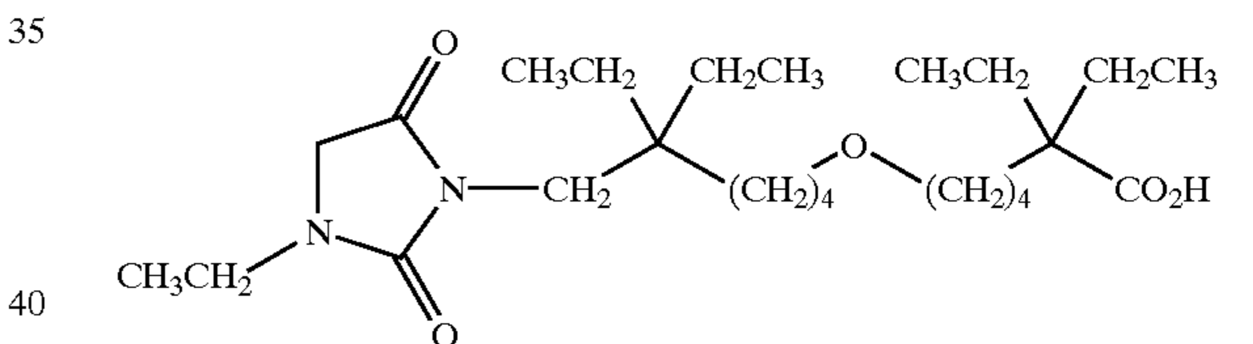
3,3-diethyl-7-[5-ethyl-5-(3-ethyl-2,5-dioxo-imidazolidine-1-yl)-heptyloxy]-heptanoic acid;
