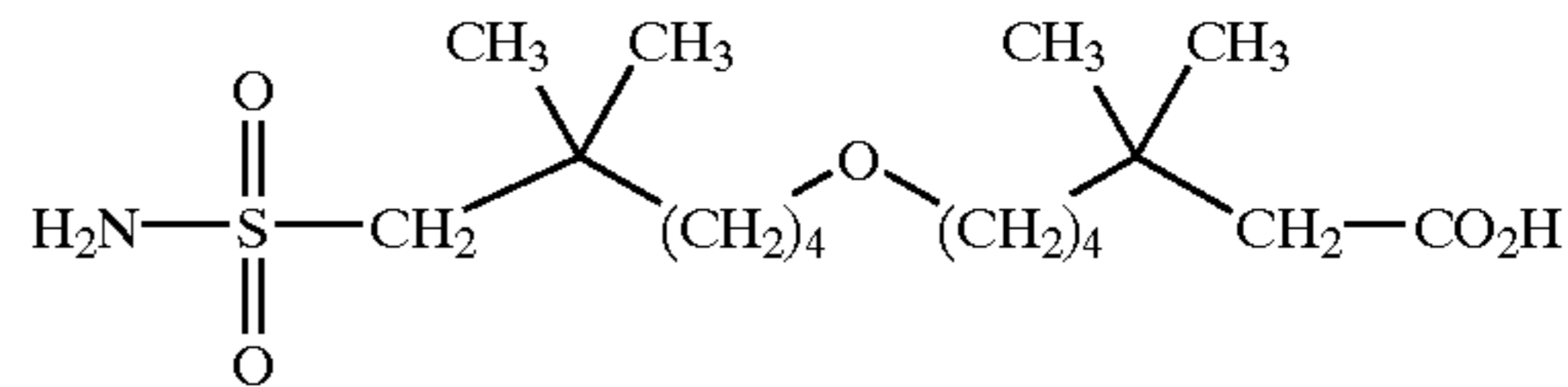
7-(5,5-dimethyl-6-sulfamoyl-hexyloxy)-3,3-dimethyl-heptanoic acid;
