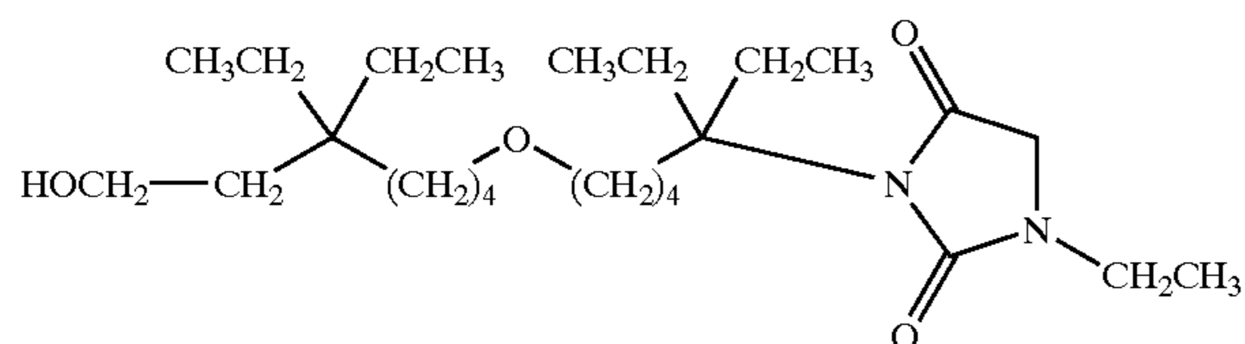
3-[2,2-diethyl-6-(5-ethyl-5-hydroxymethyl-heptyloxy)-hexyl]-1-ethyl-imidazolidine-2,4-dione;
