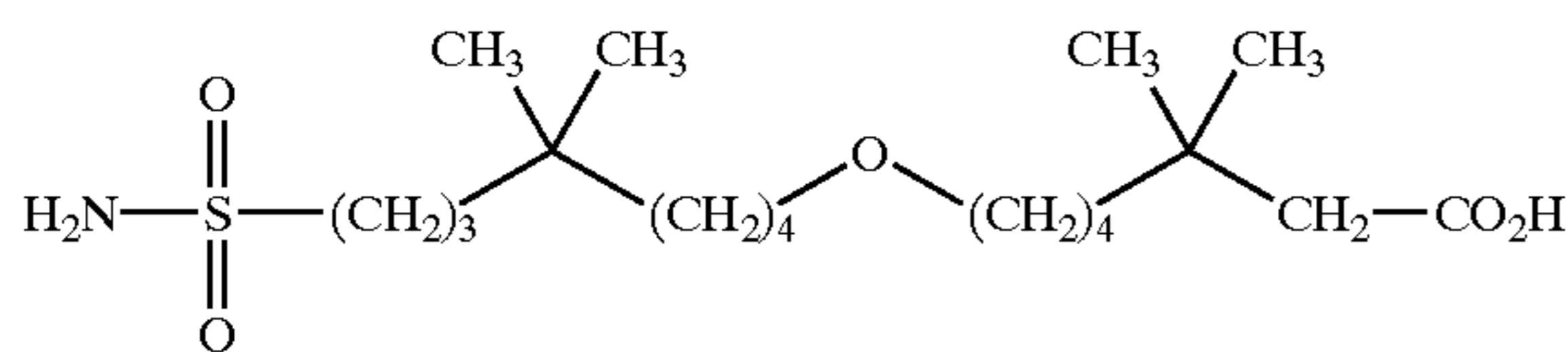
7-(5,5-dimethyl-8-sulfamoyl-octyloxy)-3,3-dimethylheptanoic acid;
