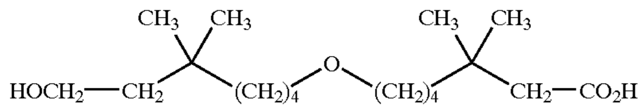
7-(7-hydroxy-5,5-dimethyl-heptyloxy)-3,3-dimethyl-heptanoic acid;
