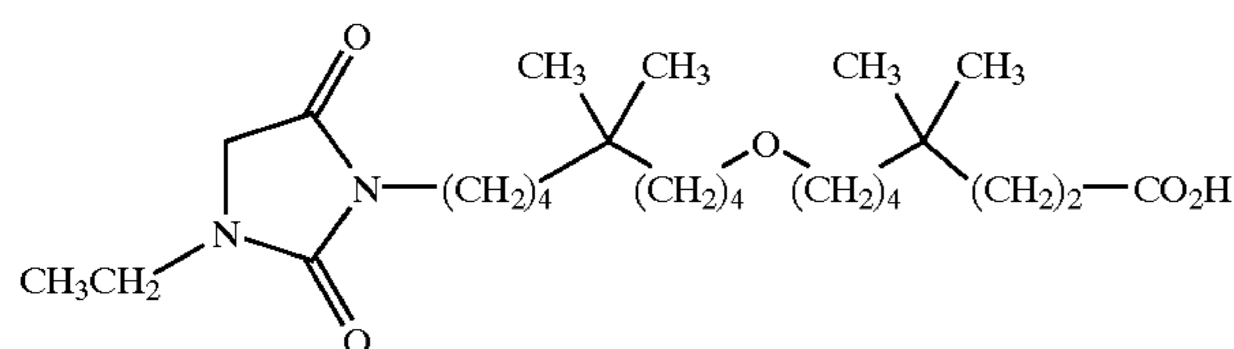
8-[9-(3-ethyl-2,5-dioxo-imidazolidin-1-yl)-5,5-dimethyl-nonyloxy]-4,4-dimethyl-octanoic acid;
