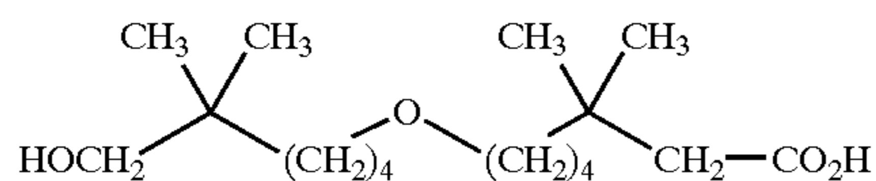
7-(6-hydroxy-5,5-dimethyl-hexyloxy)-3,3-dimethyl-heptanoic acid;
