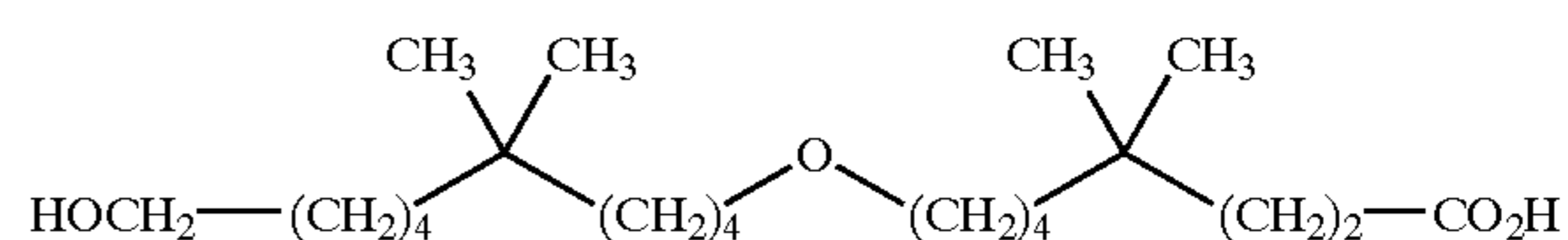
60-(8-hydroxy-5,5-dimethyl-octyloxy)-4,4-dimethyl-octanoic acid;
