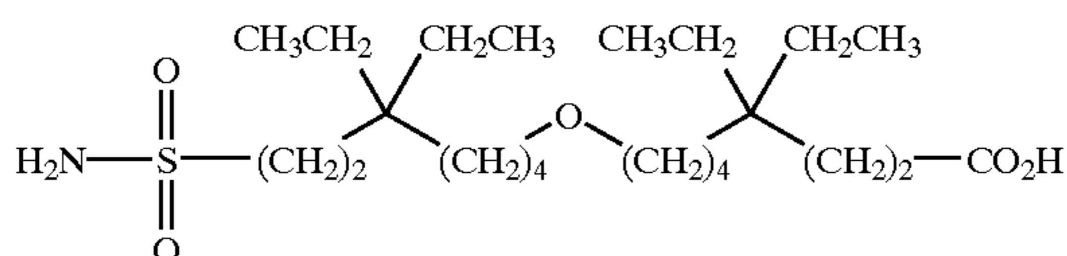
7-(5,5-diethyl-7-sulfamoyl-heptyloxy)-3,3-diethyl-heptanoic acid;
