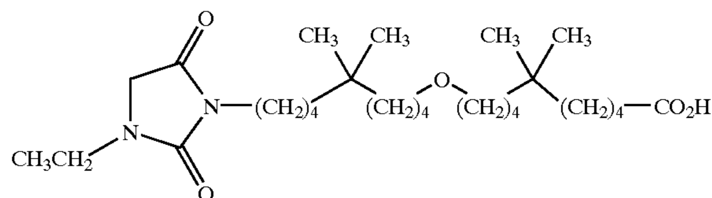
10-[9-(3-ethyl-2,5-dioxo-imidazolidin-1-yl)-5,5-dimethyl-nonyloxy]-6,6-dimethyl-decanoic acid;
