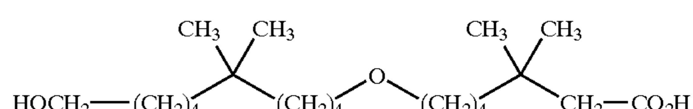
45-(10-hydroxy-5,5-dimethyl-decyloxy)-2,2-dimethyl-hexanoic acid;
