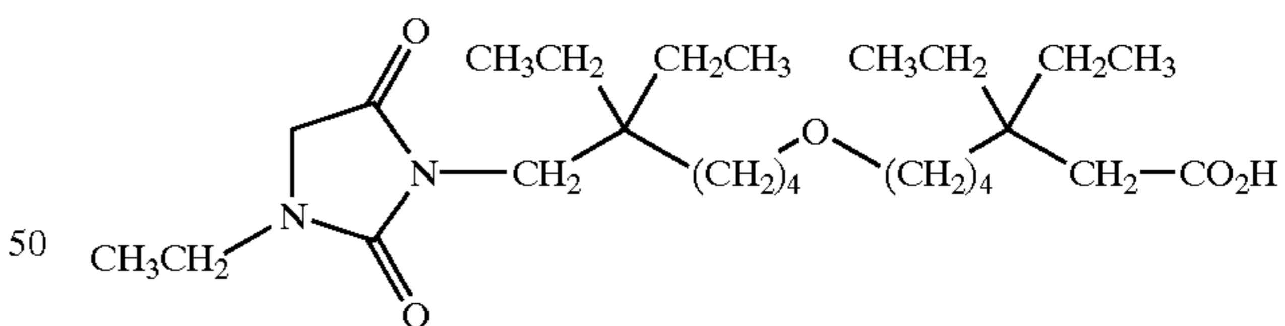
3,3-diethyl-7-[5-ethyl-5-(3-ethyl-2,5-dioxo-imidazolidine-1-ylmethyl)-heptyloxy]-heptanoic acid;
