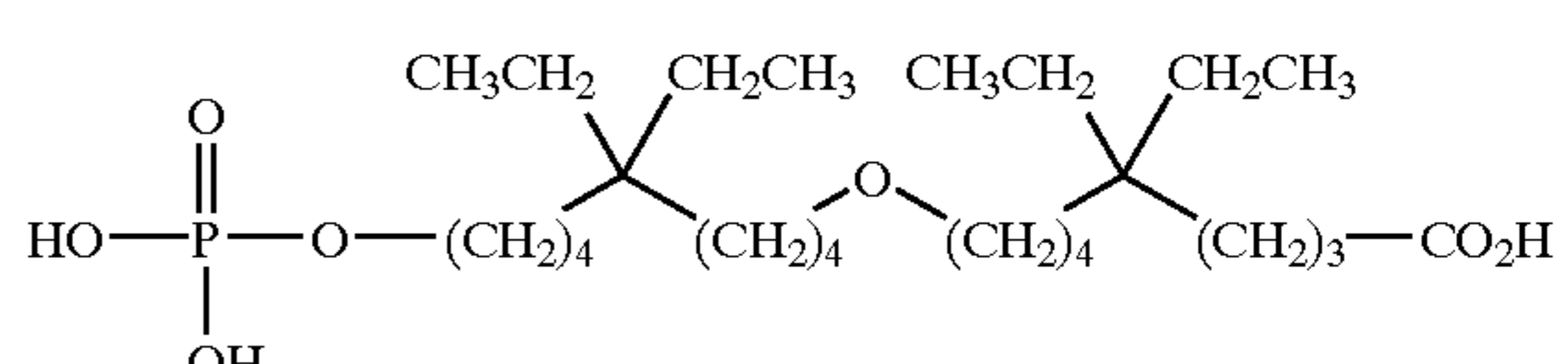
8-(5,5-diethyl-9-phosphonoxy-nonyloxy)-4,4-diethyloctanoic acid;
