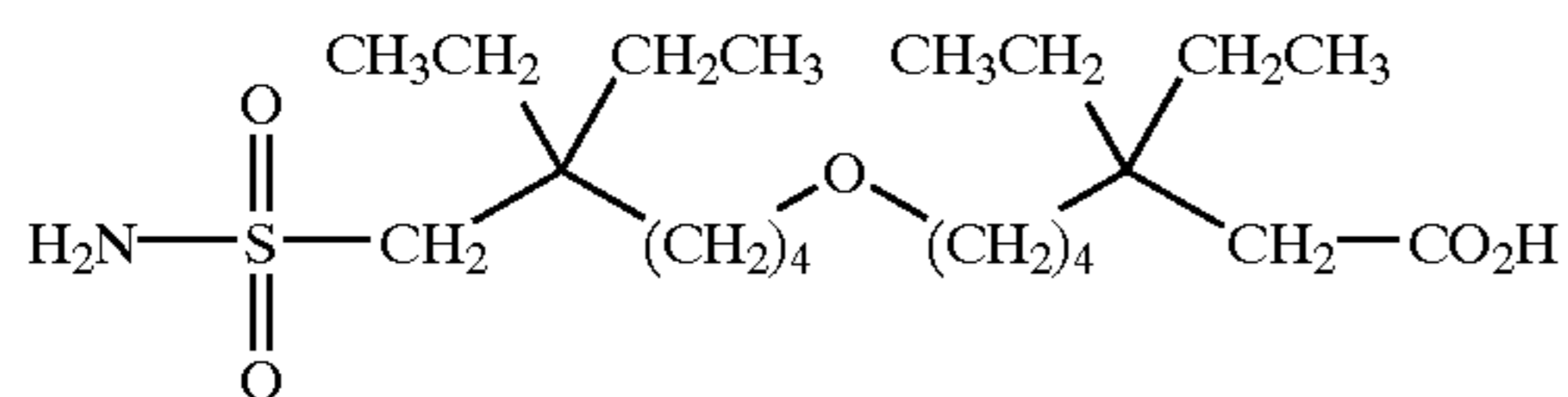
3,3-diethyl-7-(5-ethyl-5-sulfamoylmethyl-heptyloxy)-heptanoic acid;
