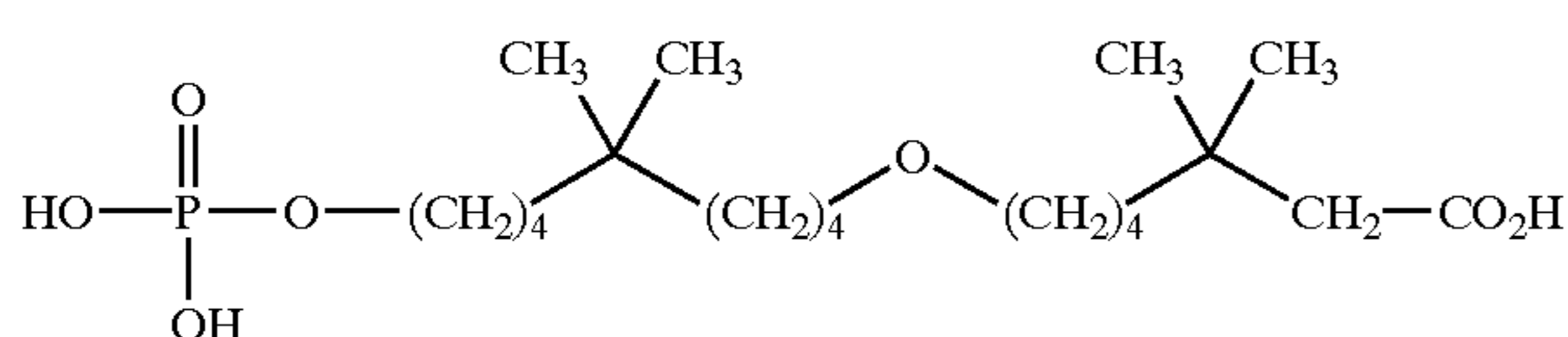
7-(5,5-dimethyl-9-phosphonoxy-nonyloxy)-3,3-dimethylheptanoic acid;
