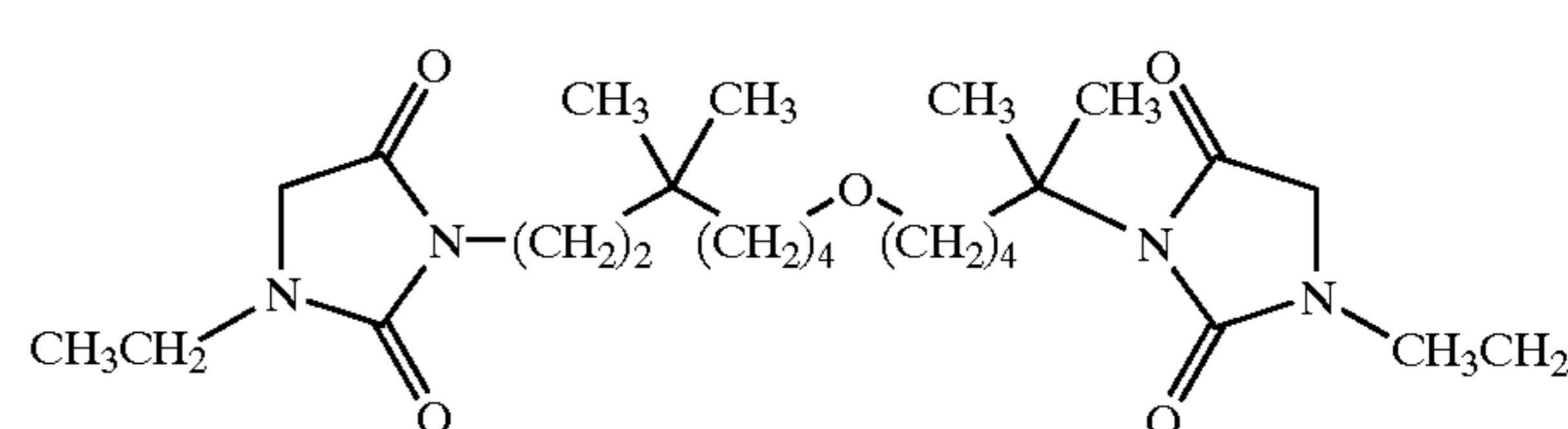
3-[5-(7-cyclopentyl-5,5-dimethyl-heptyloxy)-1,1-dimethyl-pentyl]-1-ethyl-imadazolidine-2,4-dione;
