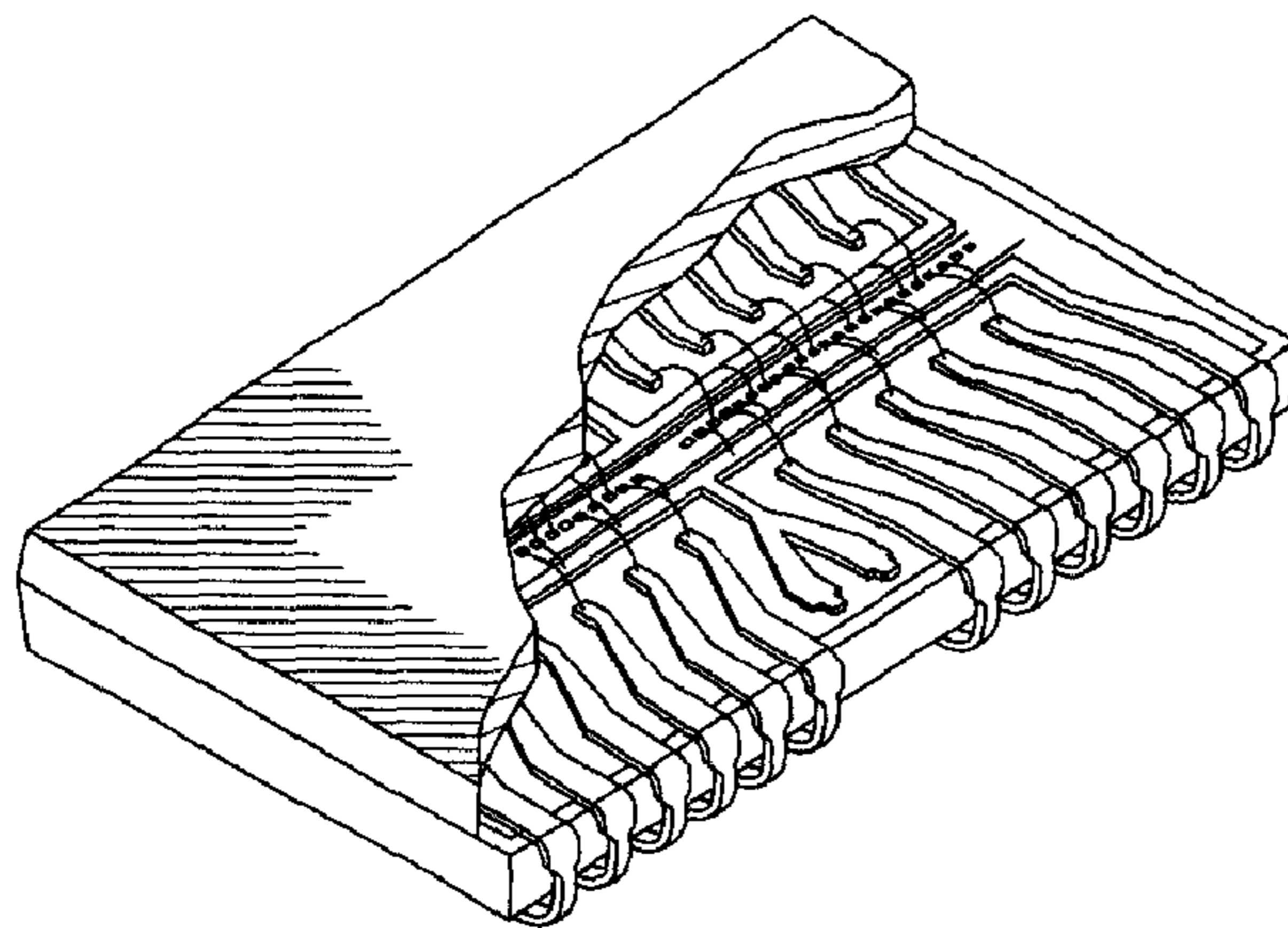
Fig. 5 (PRIOR ART)
