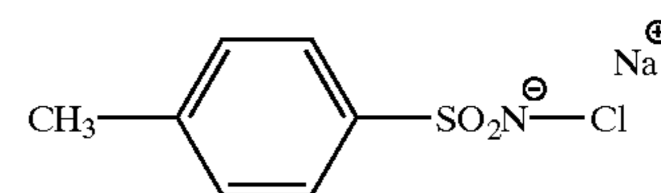
Chloramine-T
