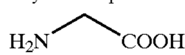
Glycine
