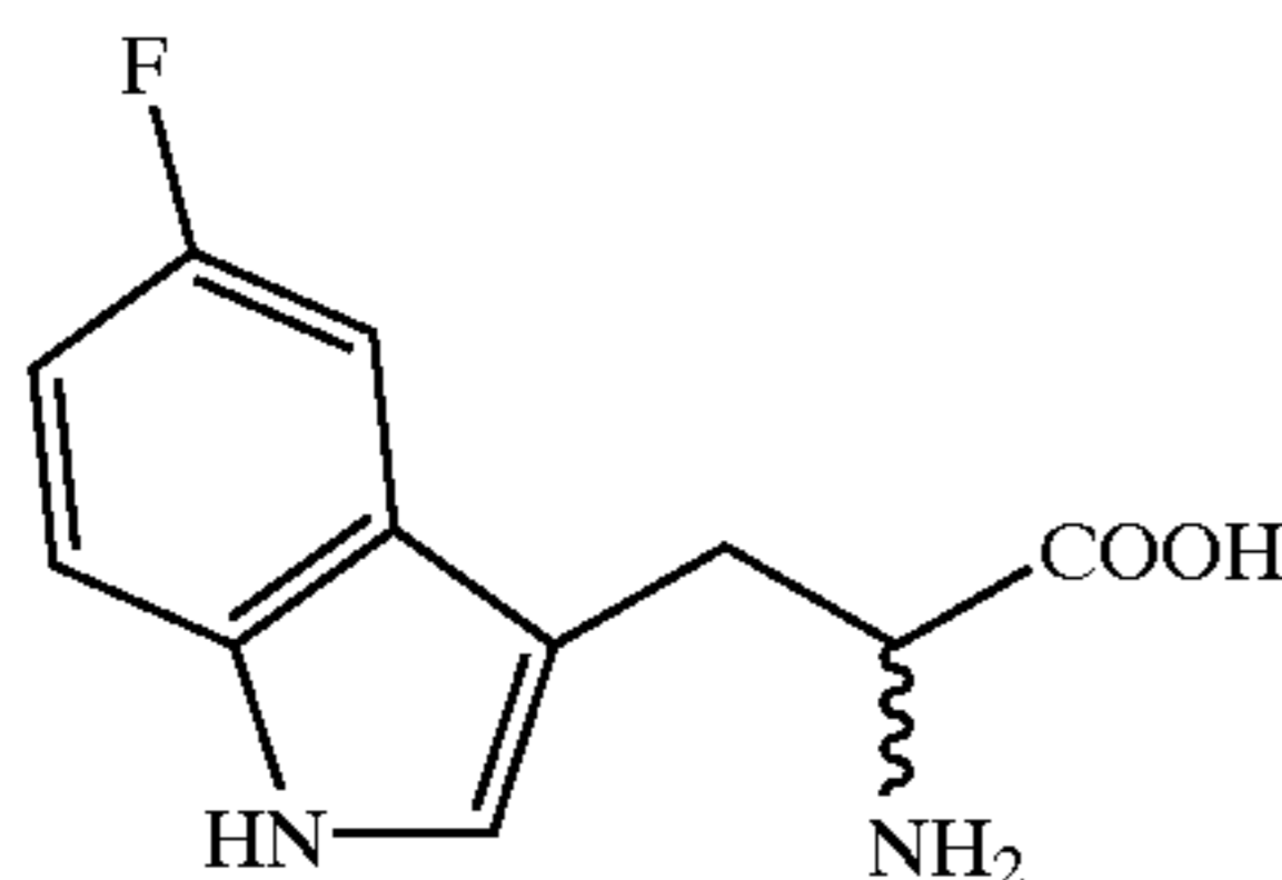
DL-5-F-Trp
