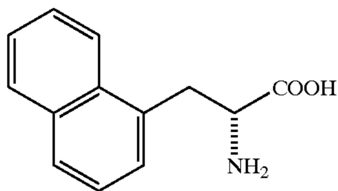
D-1-Nal
