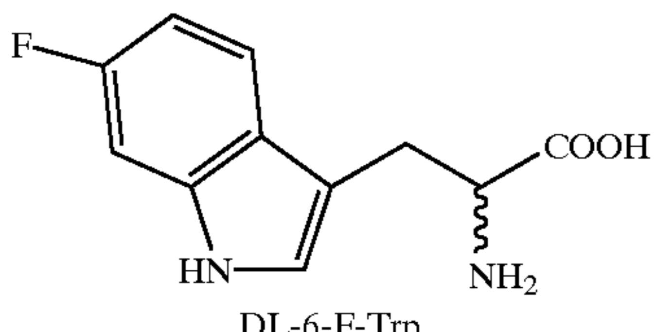
DL-6-F-Trp
