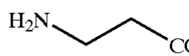
\beta -alanine
