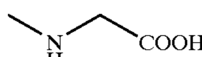
Sarcosine
