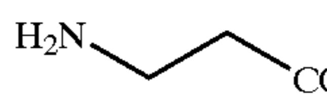
\beta -alanine
