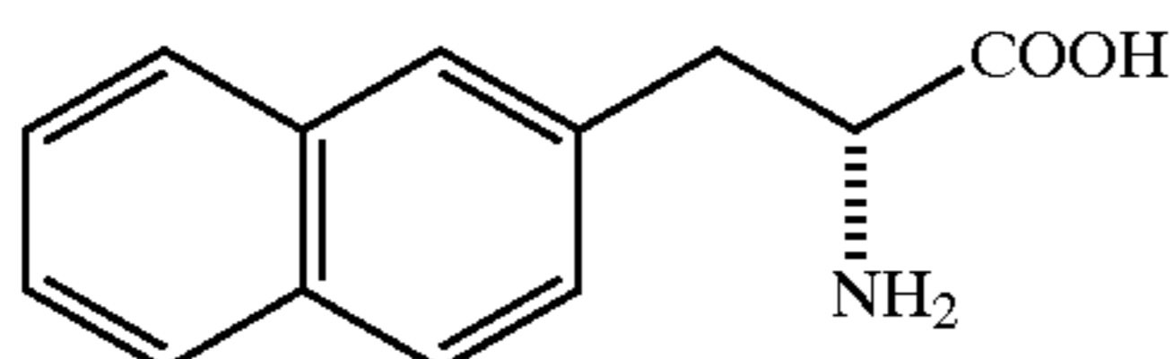
D-2-Nal
