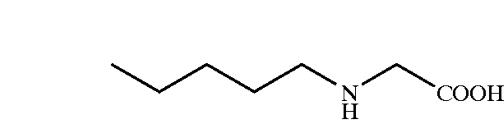
N-Pentyl glycine
