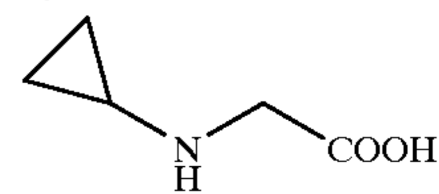
N-Cyclopropyl glycine
