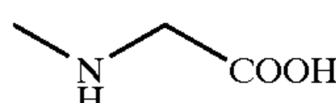
Sarcosine
