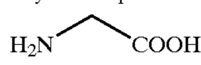
Glycine
