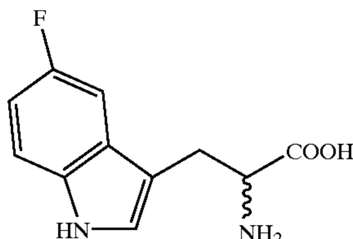
DL-5-F-Trp
