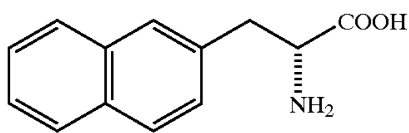
D-2-Nal
