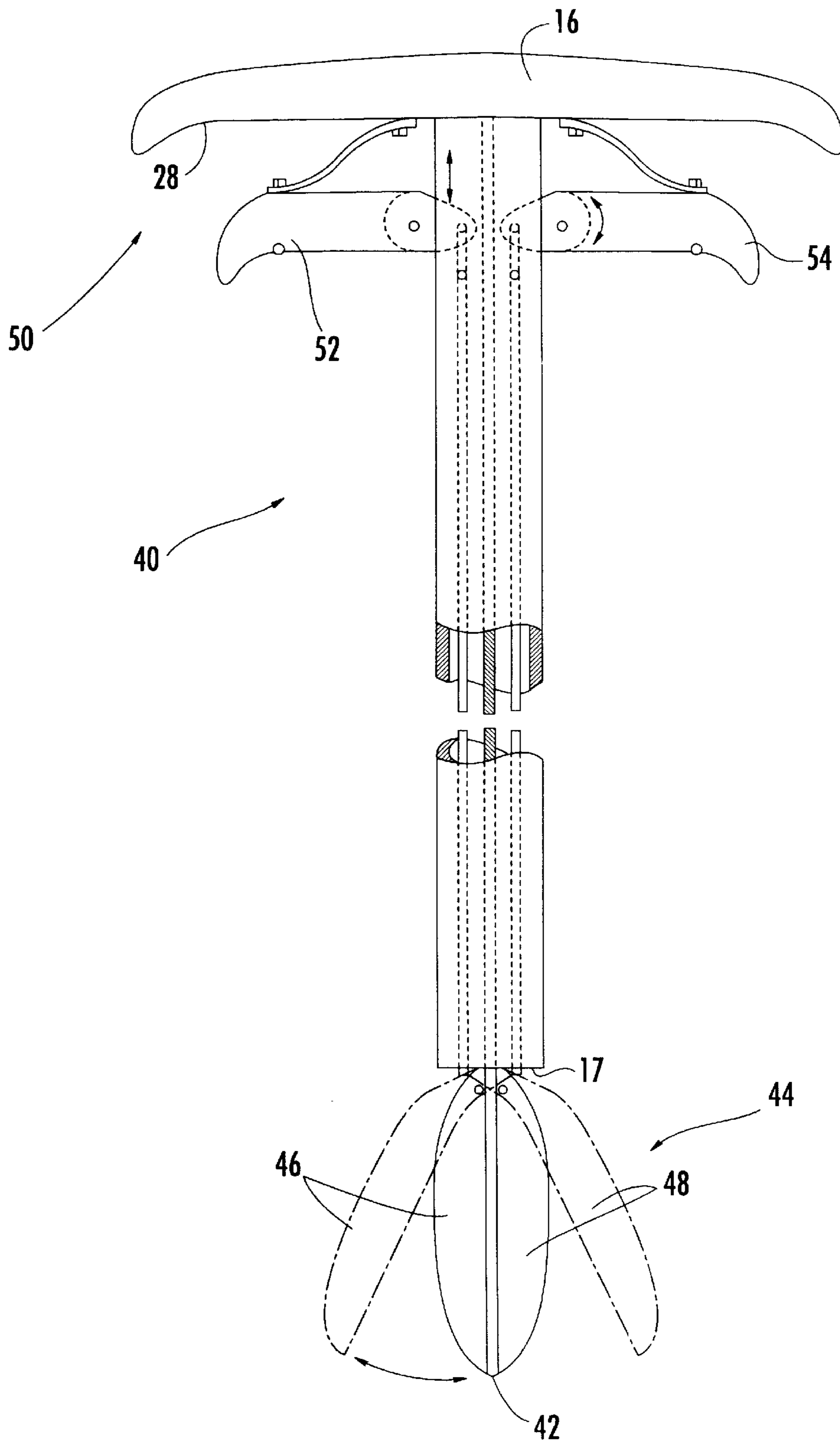
FIG. 2. PRIOR ART
