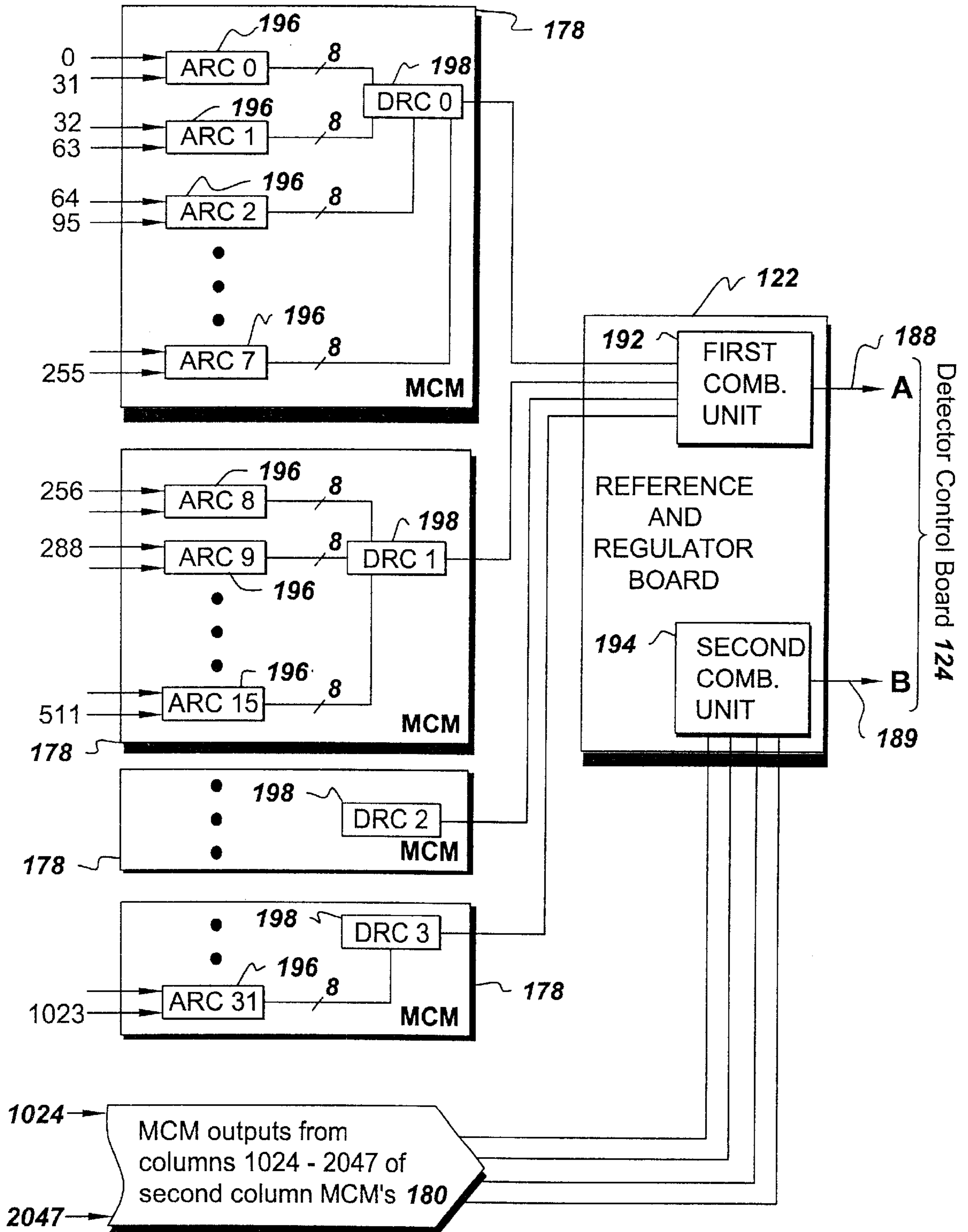
fig. 9 (PRIOR ART)
