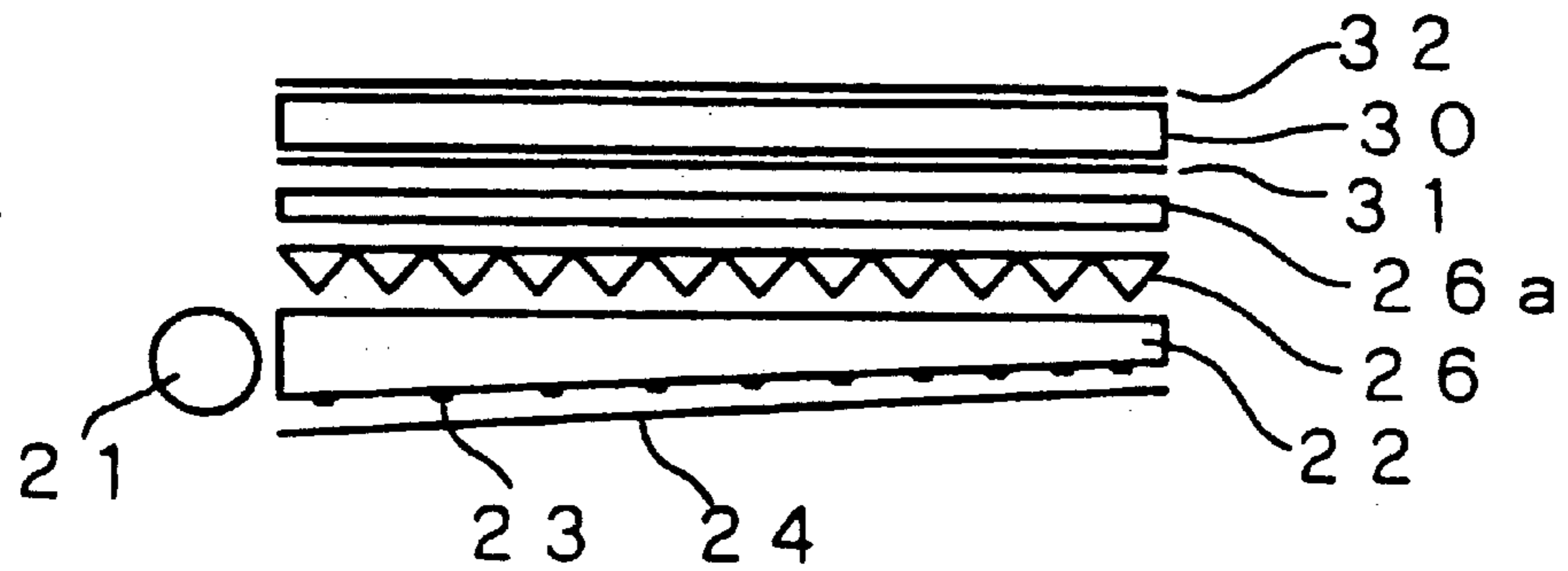
FIG. 13 PRIOR ART
