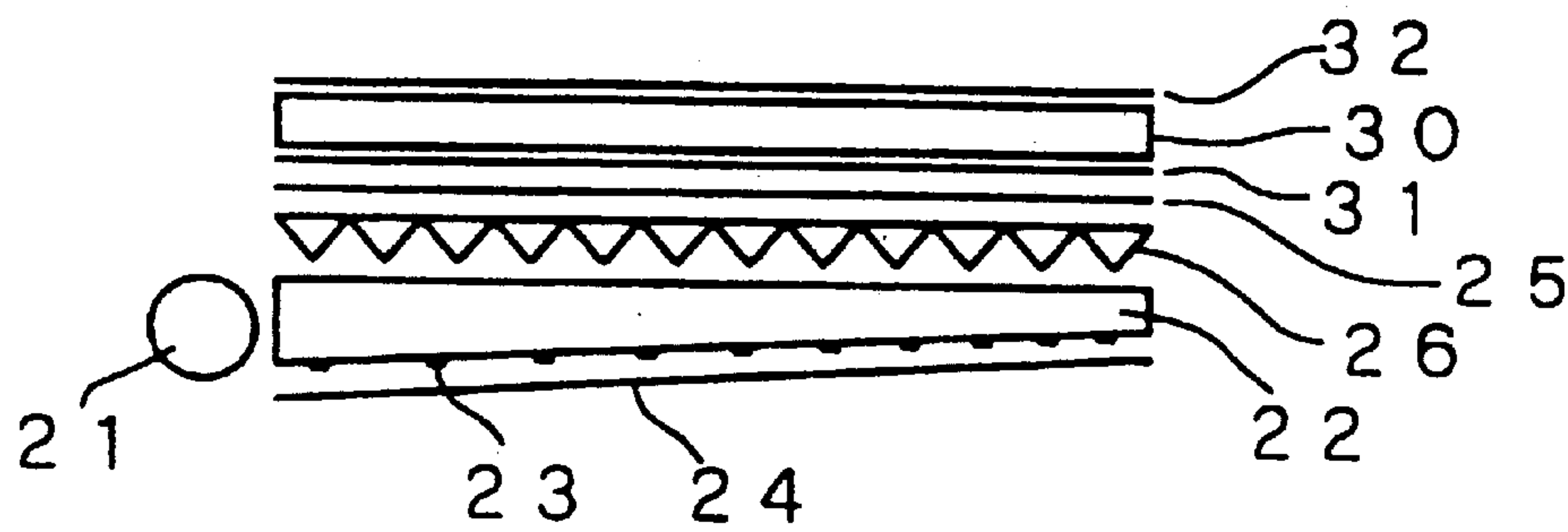
FIG. 12 PRIOR ART
