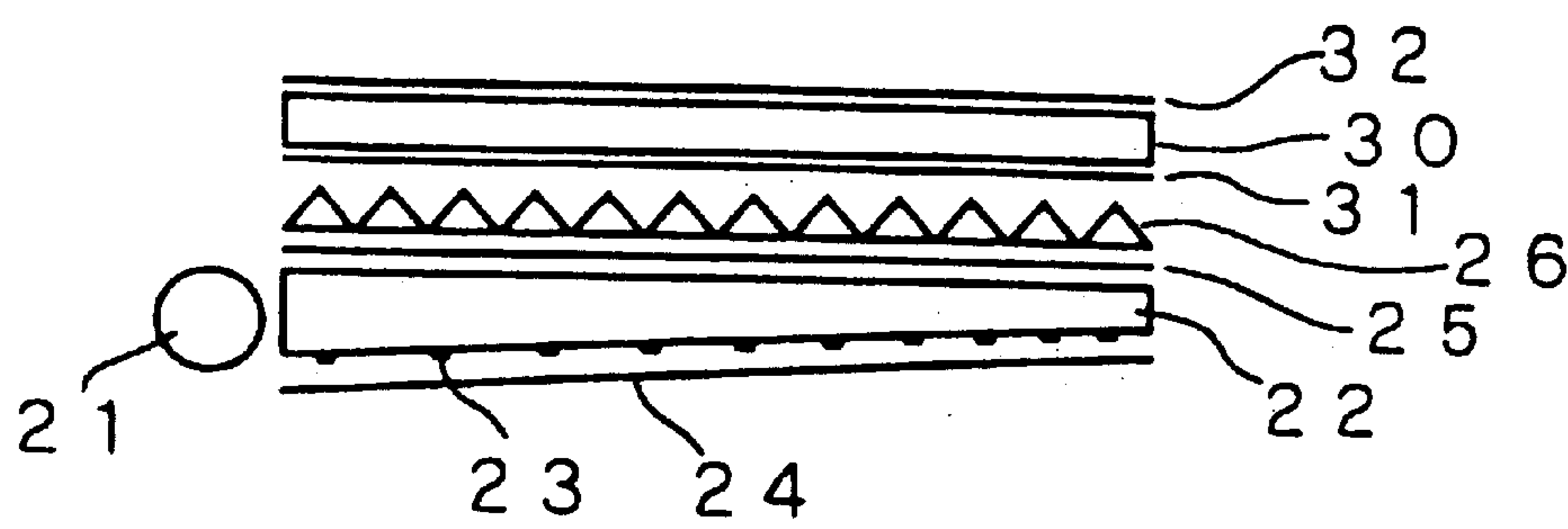
FIG. 11 PRIOR ART
