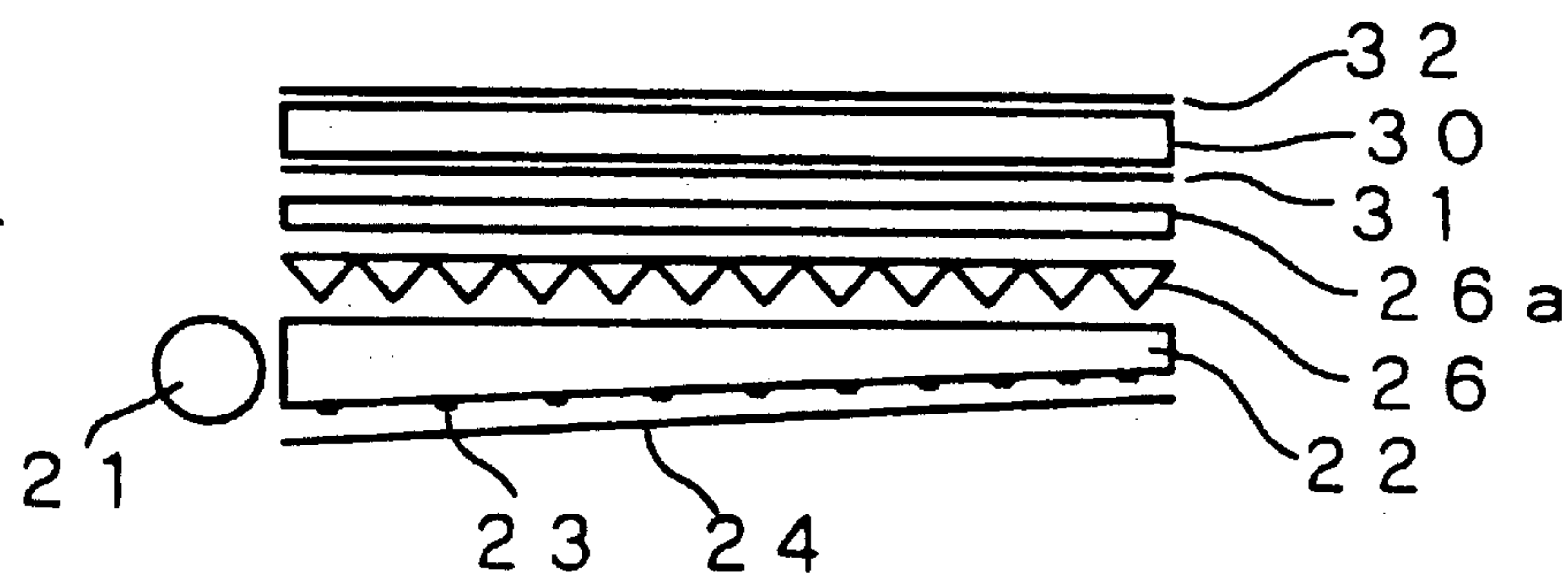
FIG. 13 PRIOR ART
