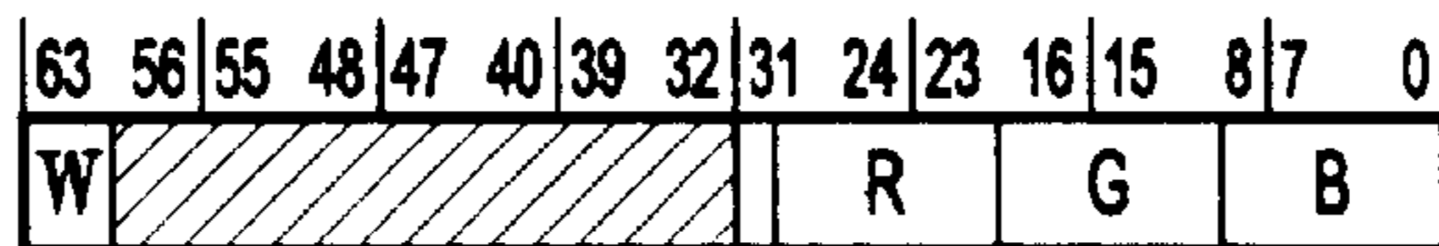
64 BPP PIXEL FORMAT 2:10:10:10
