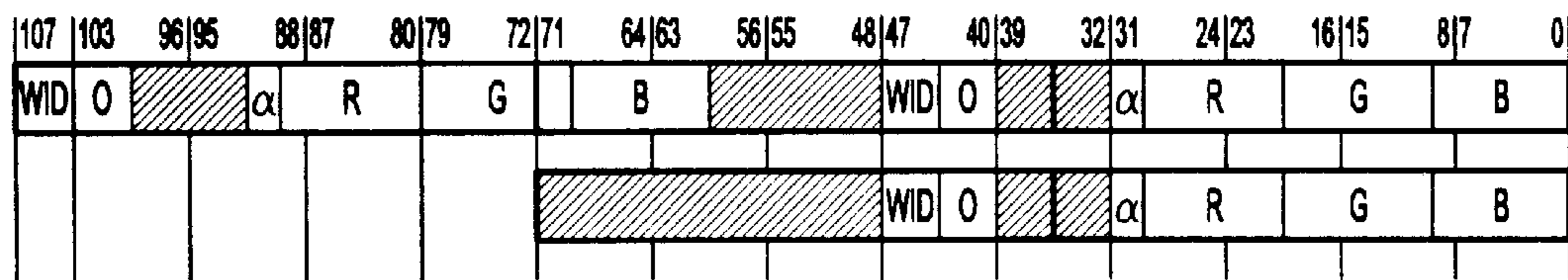
96 bpp Display Refresh 4:4:24:2*(10:10:10)
