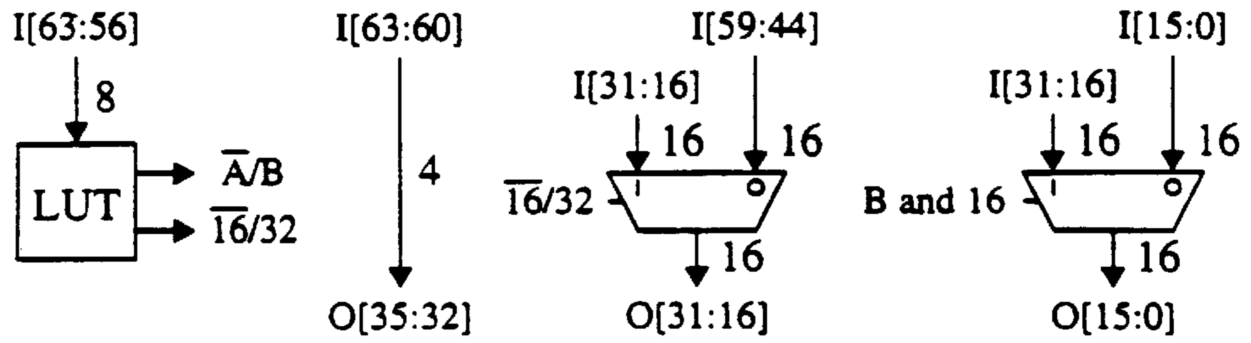
SRAM-to-DQ Routing
