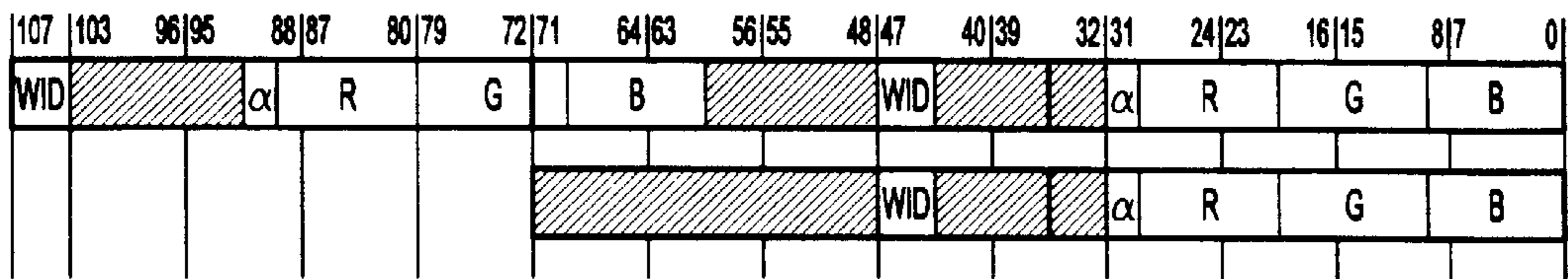
96 bpp Display Refresh 4:28:2*(2:10:10:10)
