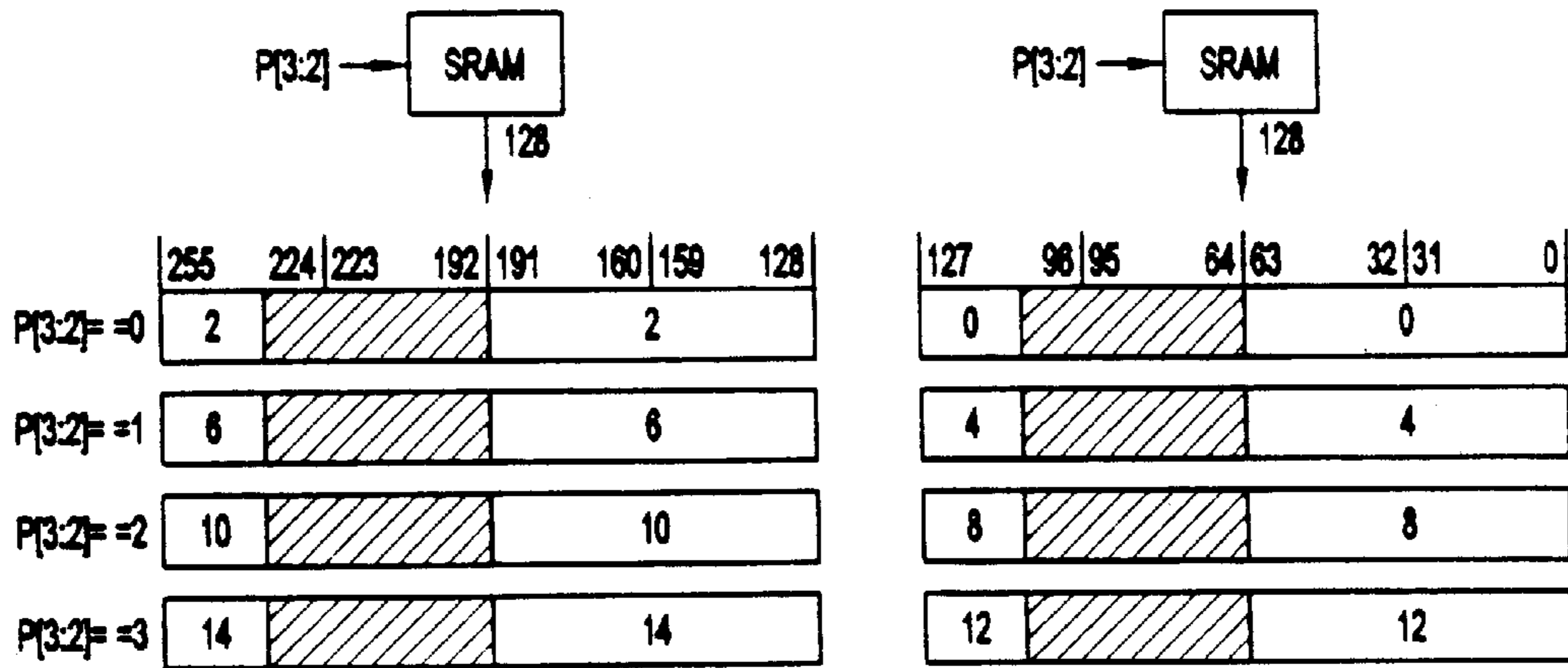
SRAM-TO-DQ ROUTING
