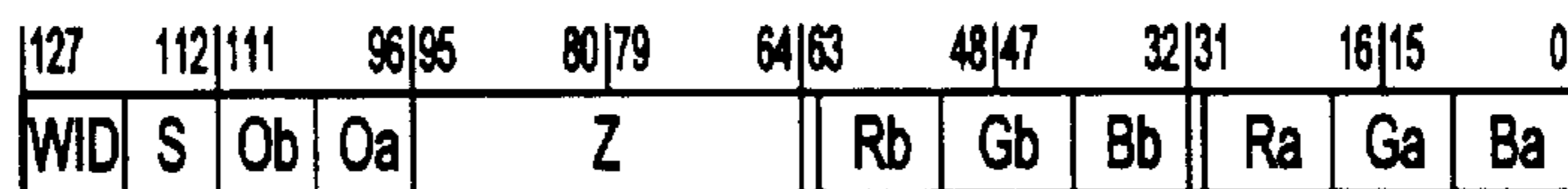
128 bpp Pixel Format 8:32:8:2*(8:2:10:10:10)
