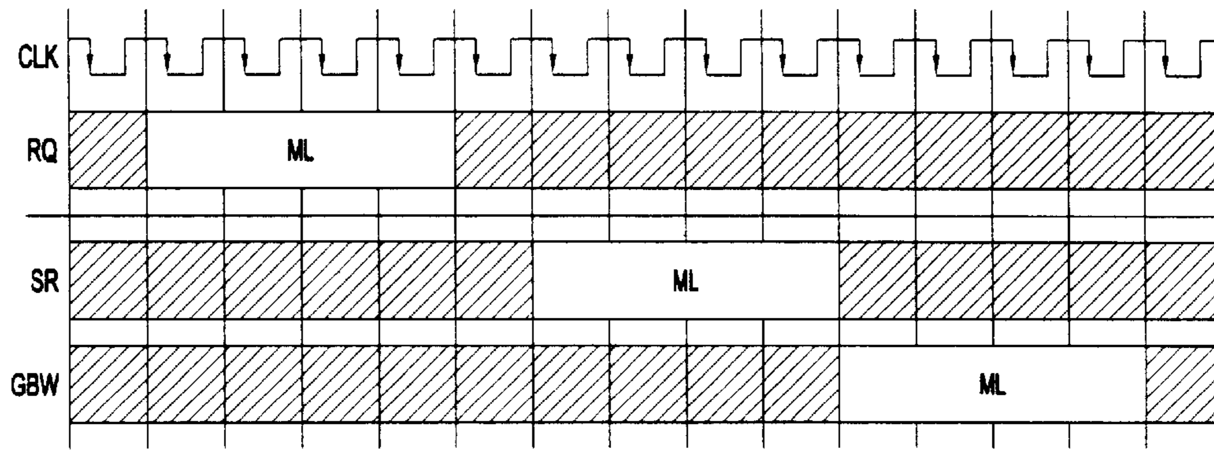
ML OPERATION
