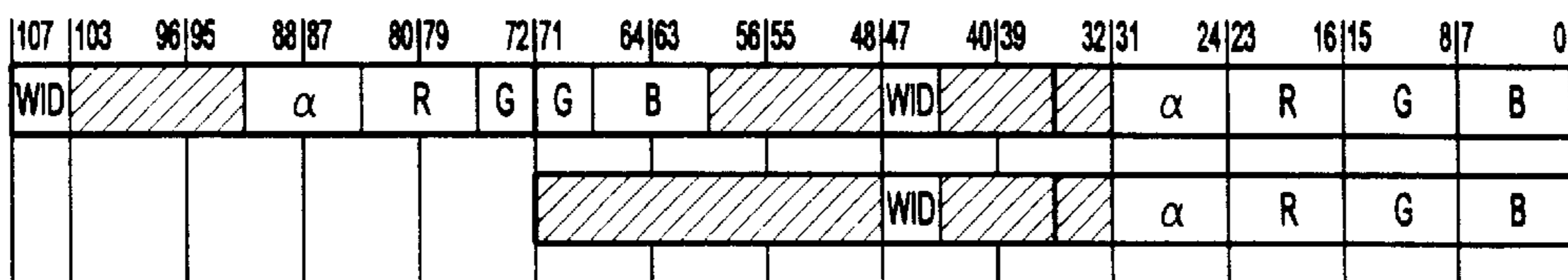
96 bpp Display Refresh 4:28:2*(8:8:8:8)
