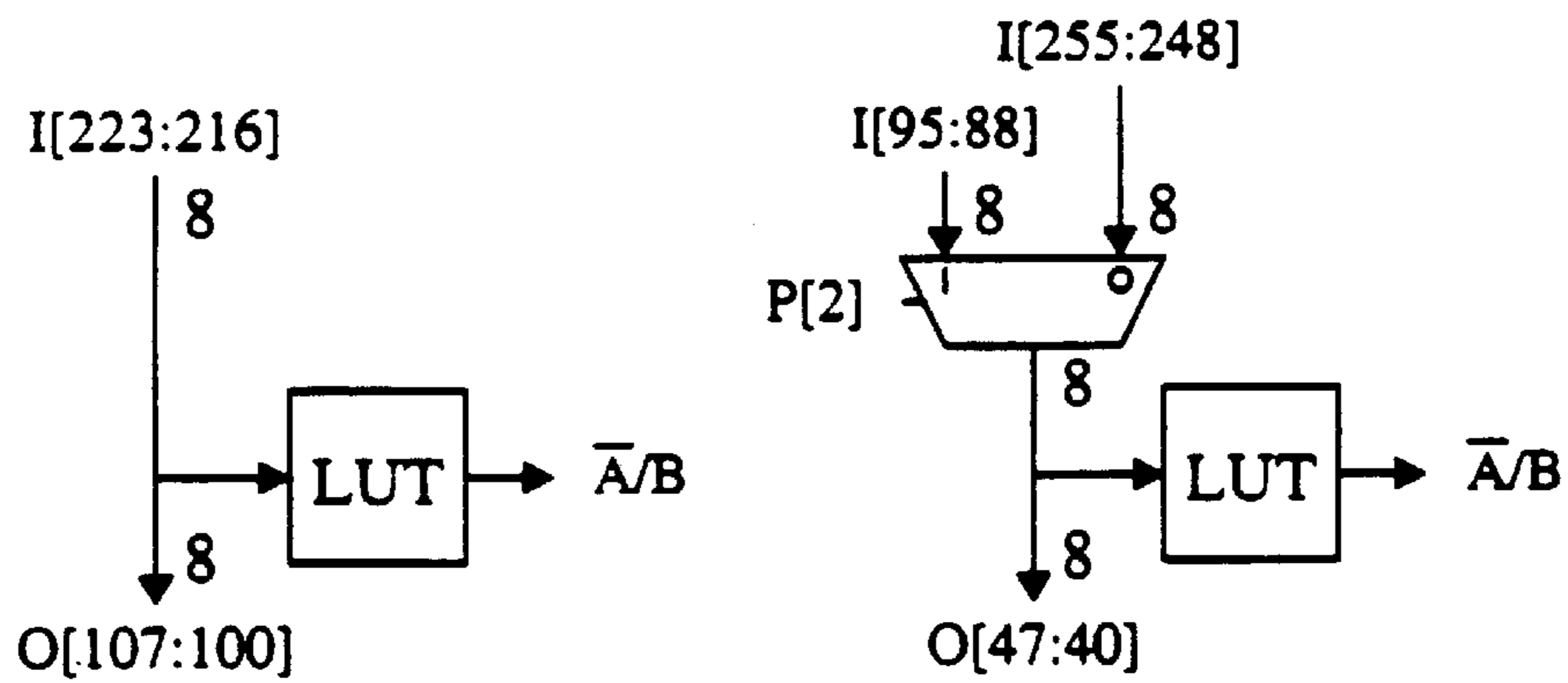
SRAM-to-DQ Routing
