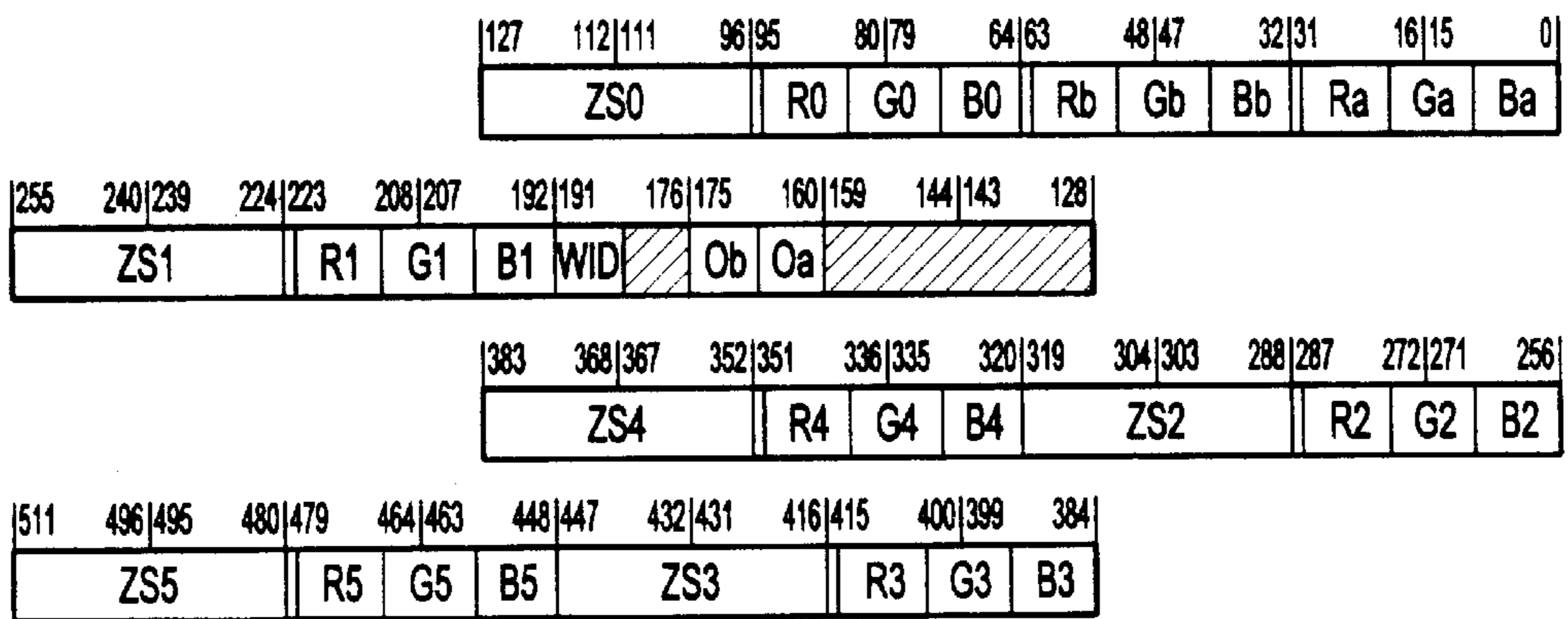
512 bpp Pixel Format 8:2*(8:10:10:10):6*(10:10:10:32)
