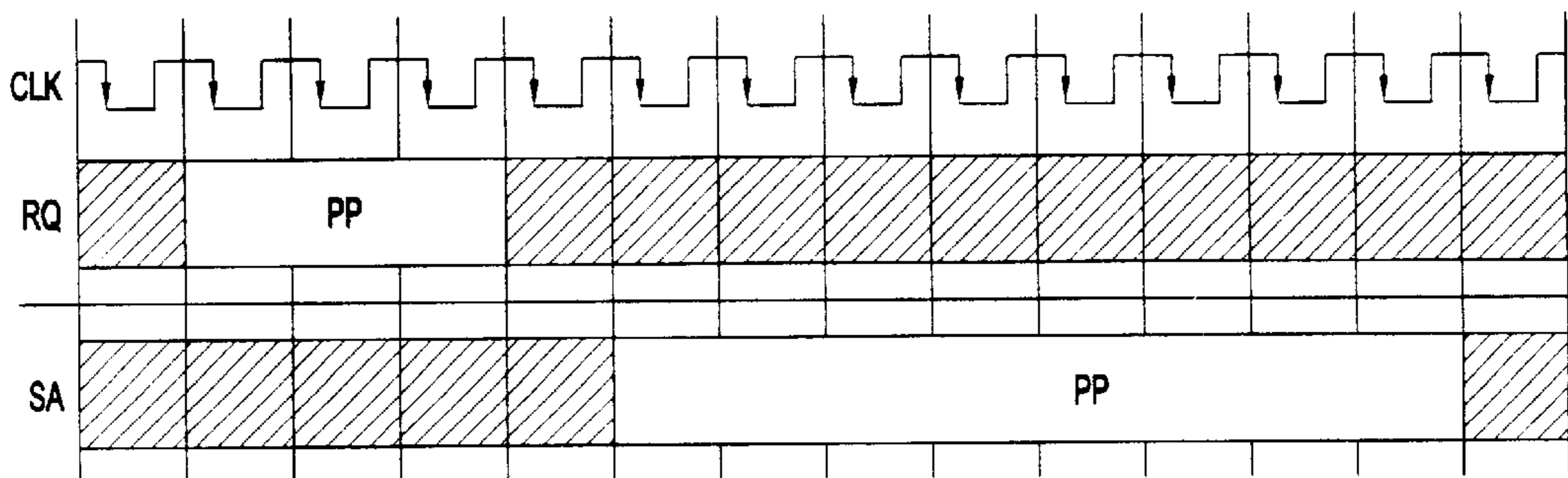
PRECHARGE PAGE
