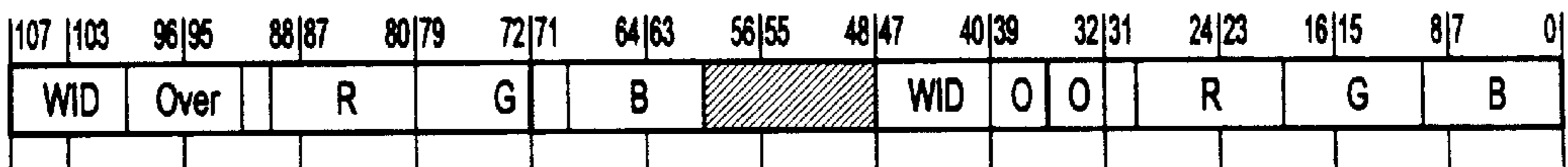
128 bpp Display Refresh 8:32:8:2*(8:10:10:10)
