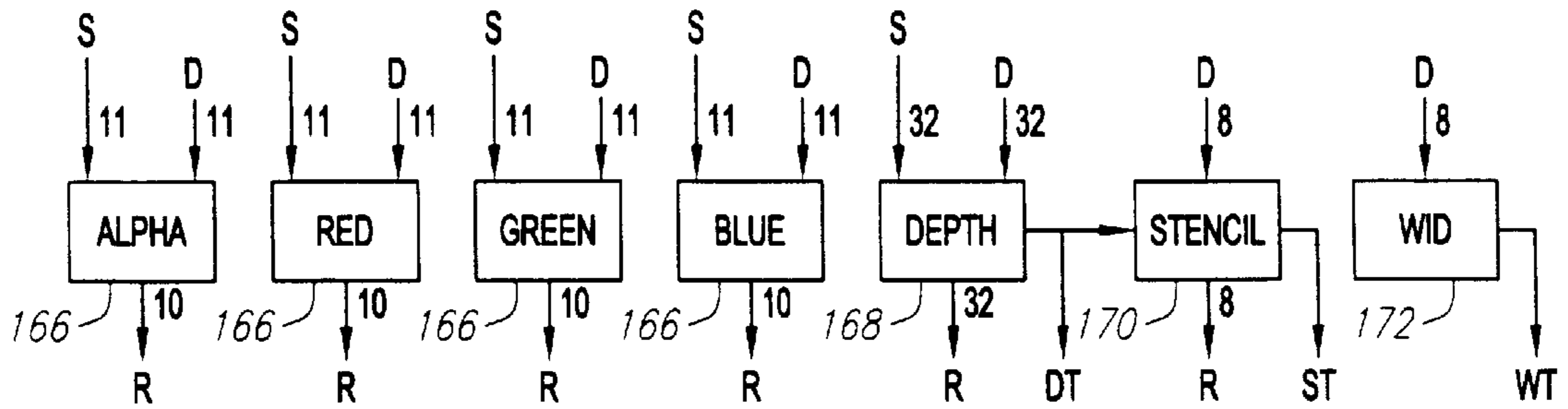
COMPONENTS OF PIXEL ALU
