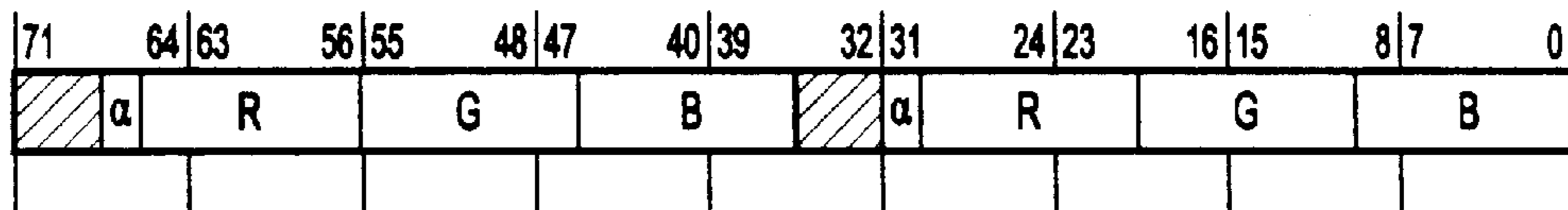
RGB 2:10:10:10 DISPLAY REFRESH
