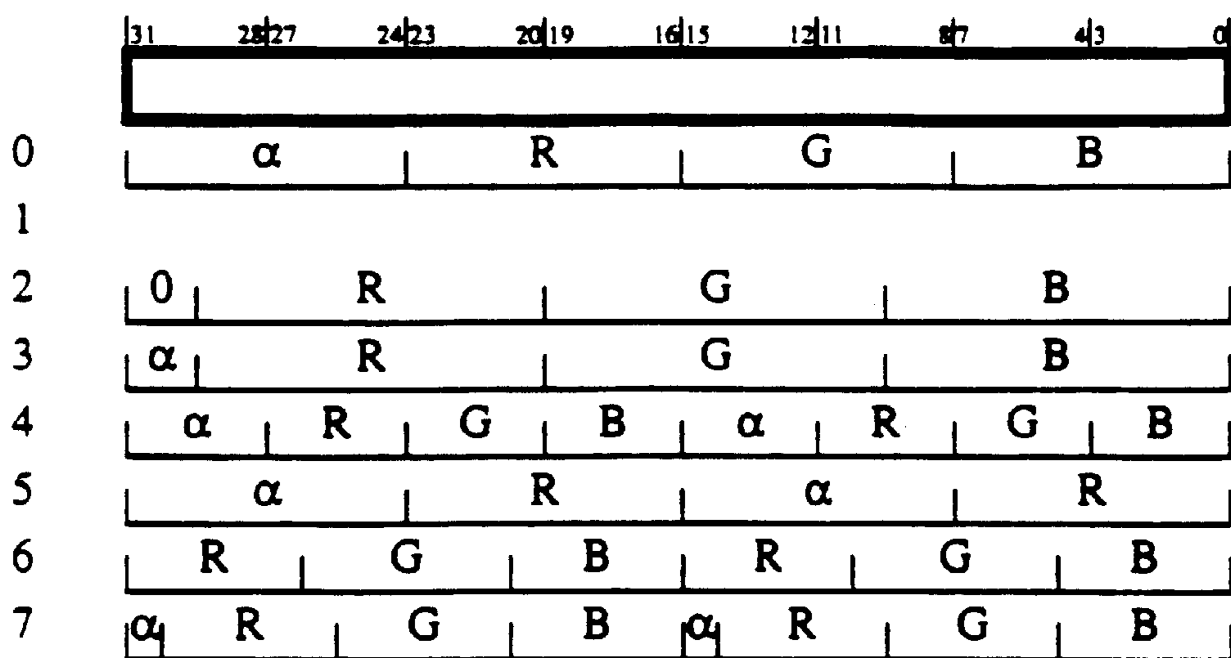
PackColor
