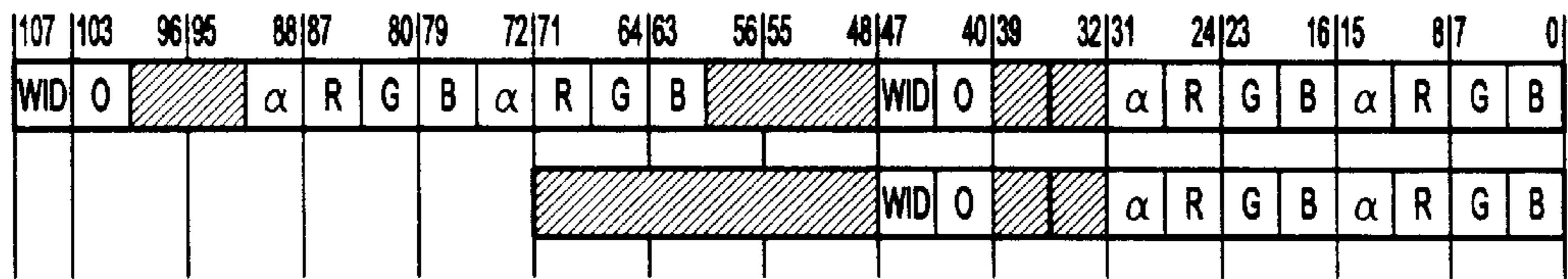
96 bpp Display Refresh 4:4:24:4*(4:4:4:4)
