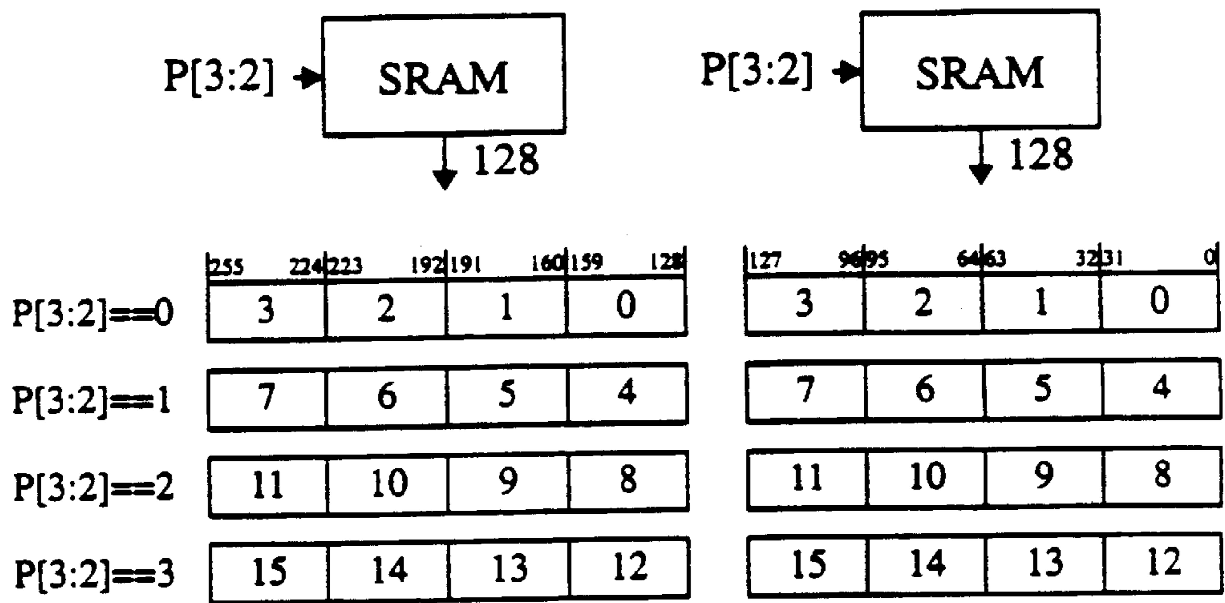
SRAM-to-DQ Routing: RDAT, RPIX Operation
