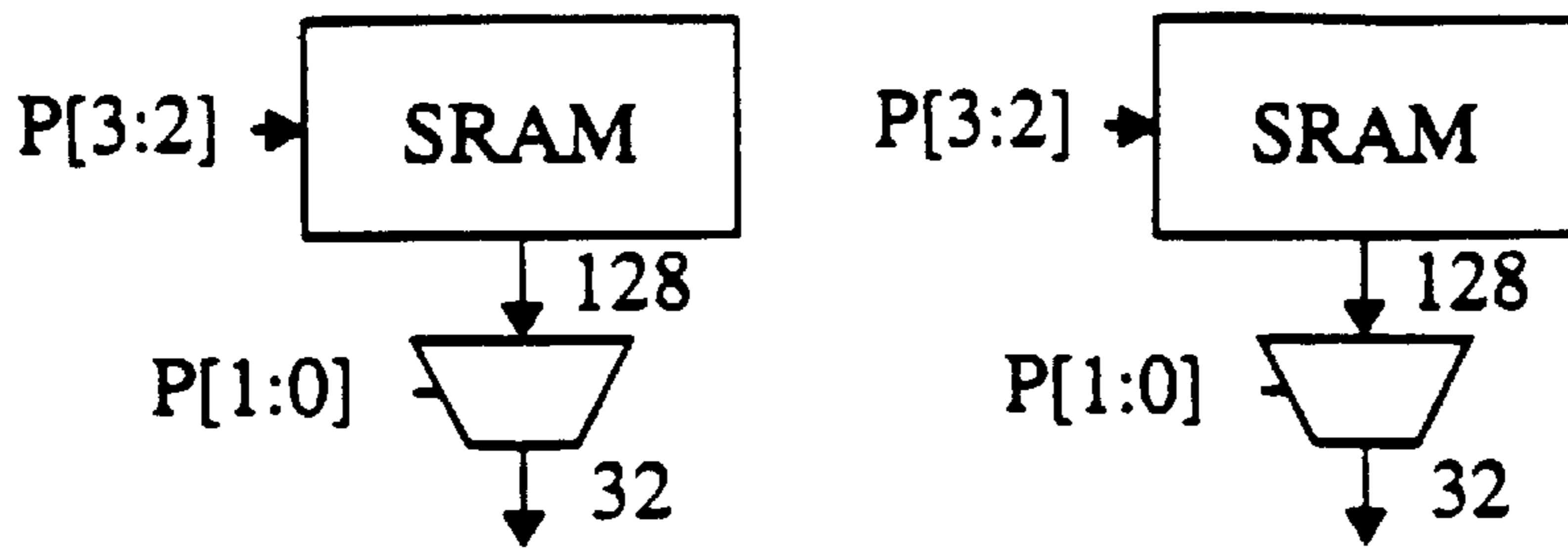
SRAM-to-DQ Routing
