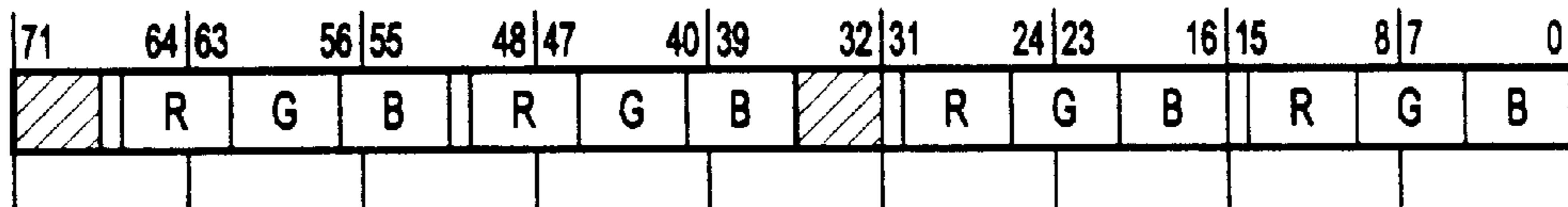
16 BPP DISPLAY REFRESH 1:5:5
