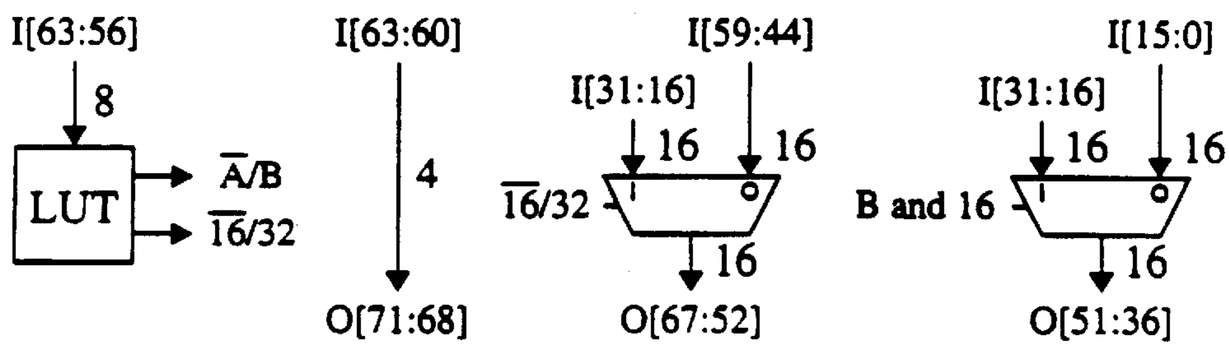
SRAM-to-DQ Routing
