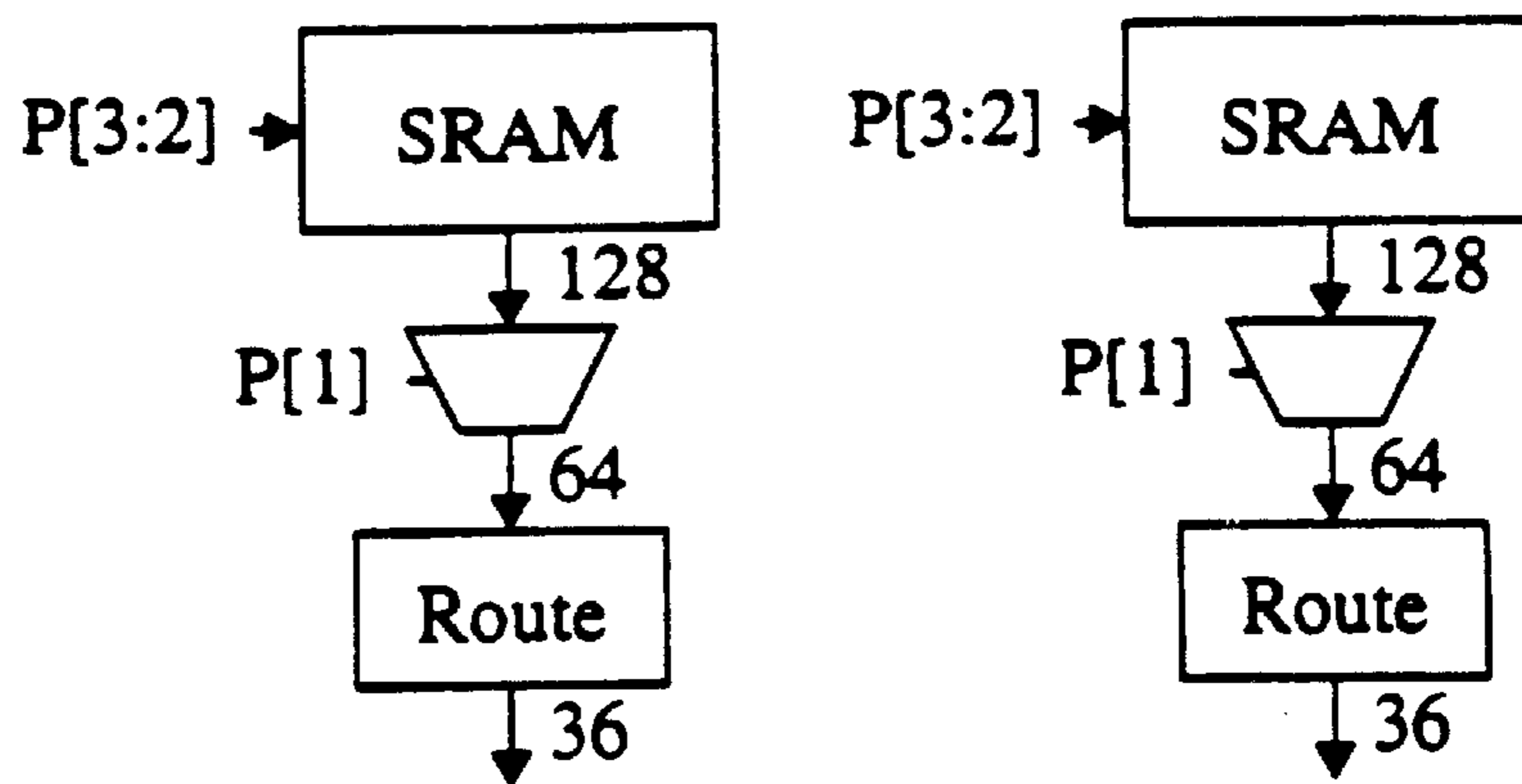
SRAM-to-DQ Routing
