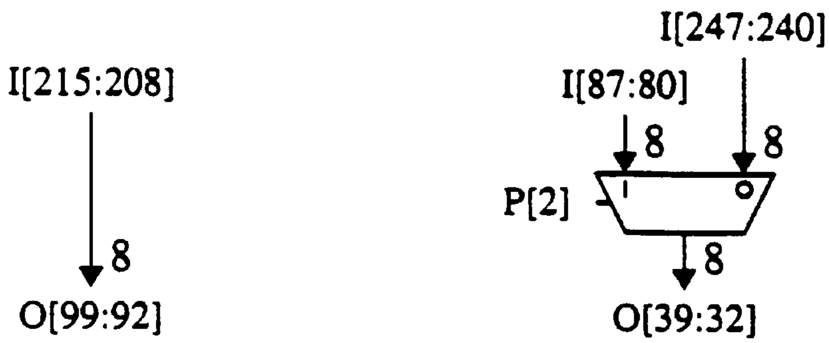
SRAM-to-DQ Routing
