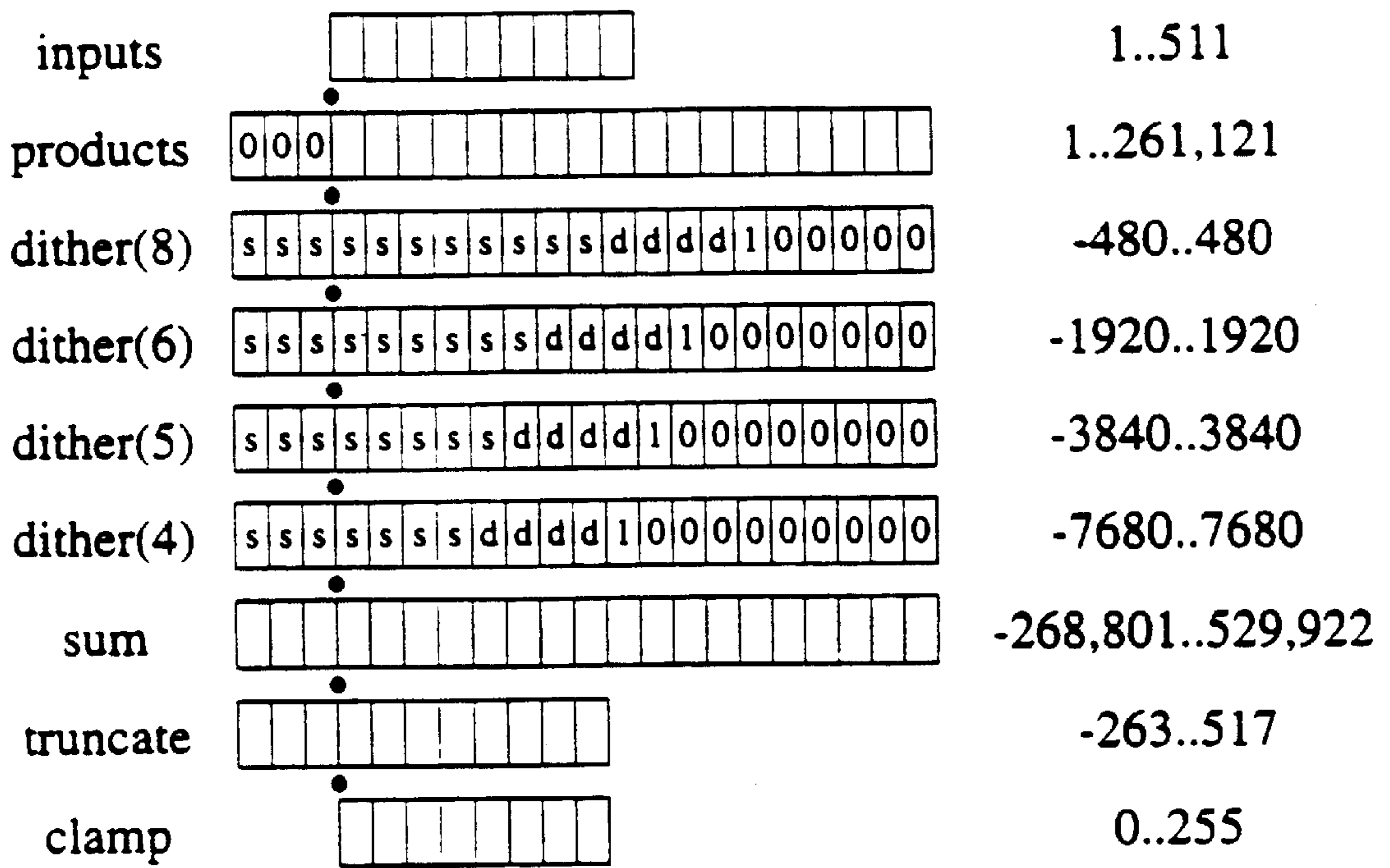
Eight-bit Blend Unit Calculations
