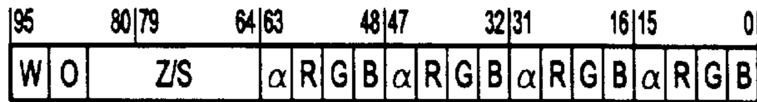
96 bpp Pixel Format 4:4:24:4*(4:4:4:4)
