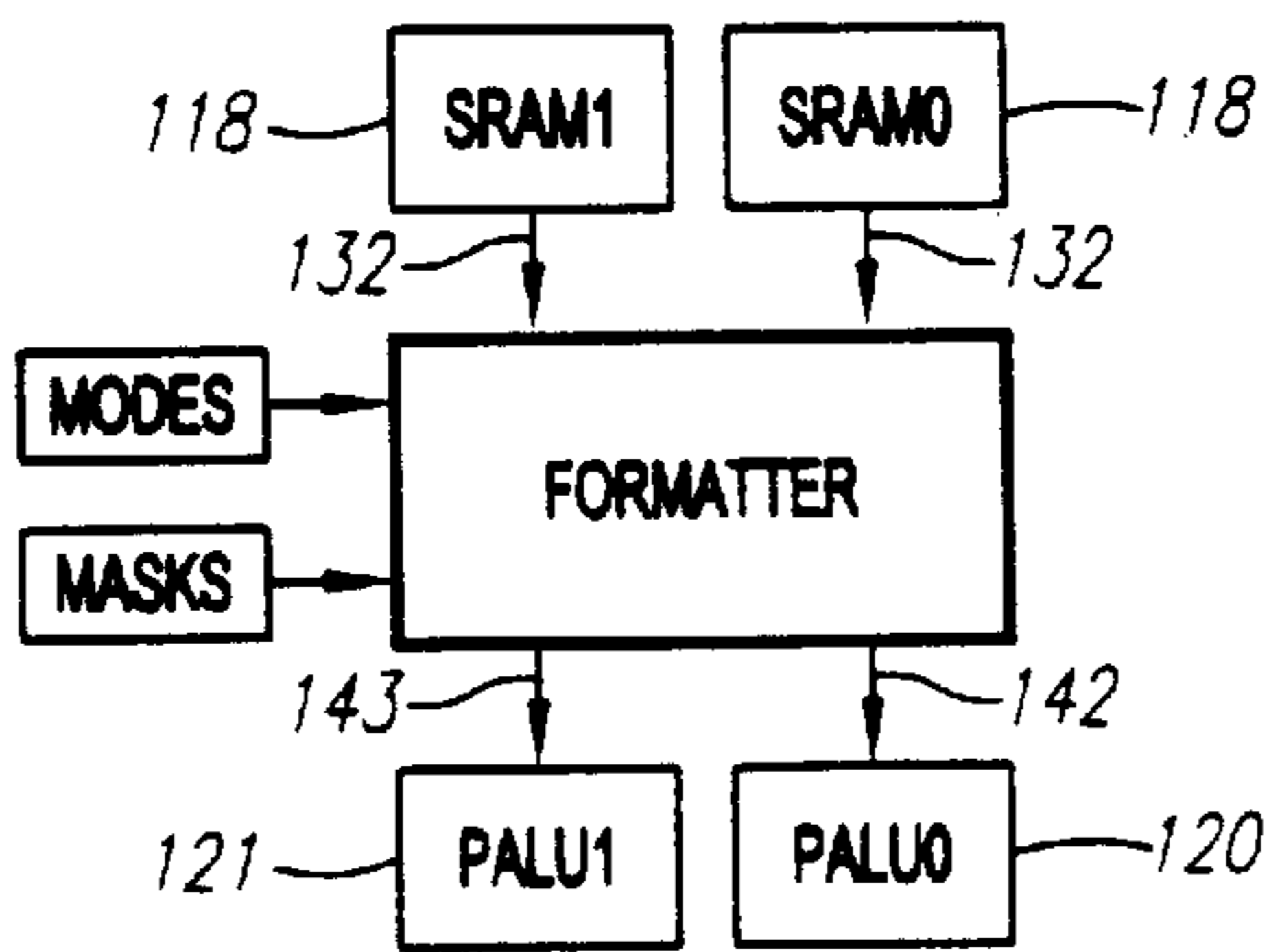
SRAM-TO-PIXEL ALU ROUTING
