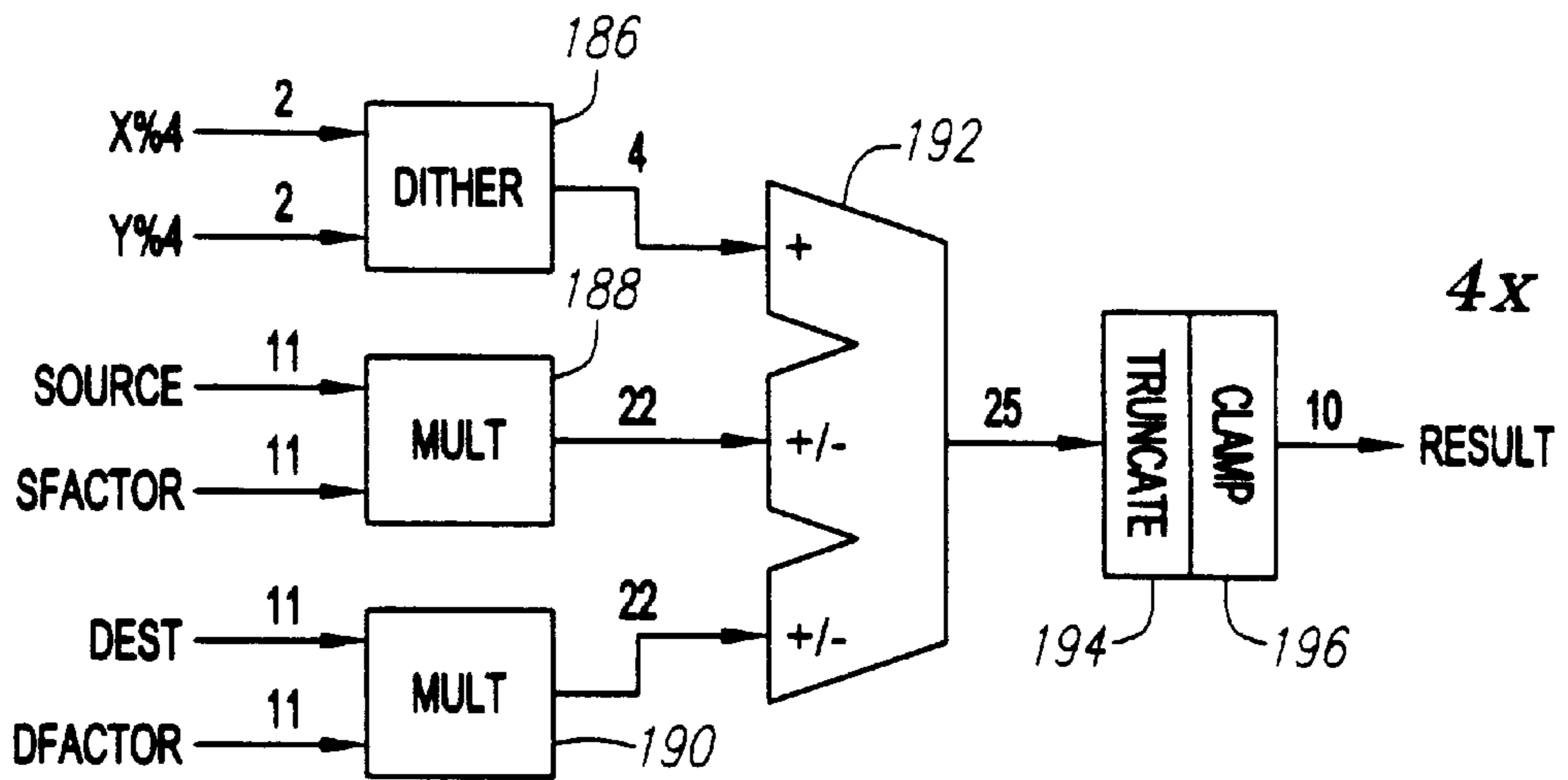
10-BIT BLEND UNIT
