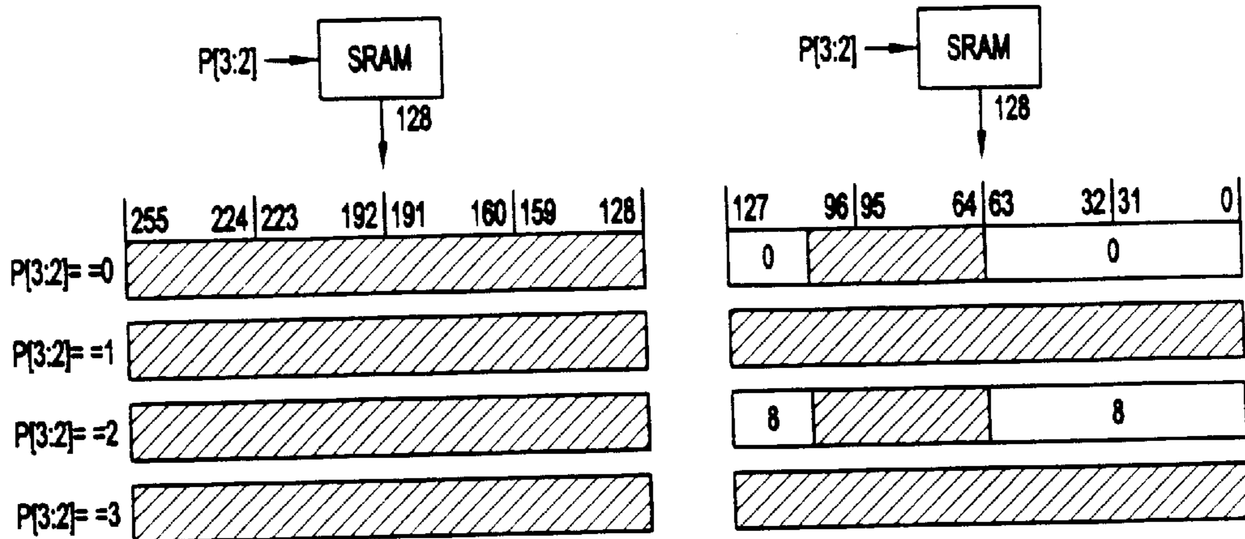
SRAM-TO-DQ ROUTING
