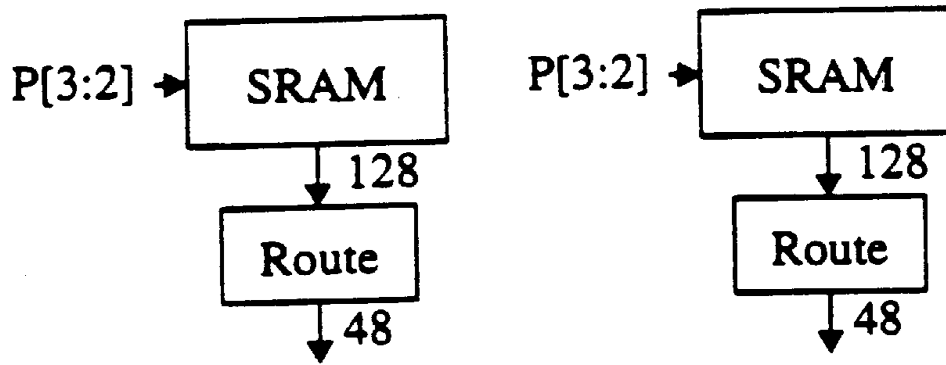
SRAM-to-DQ Routing
