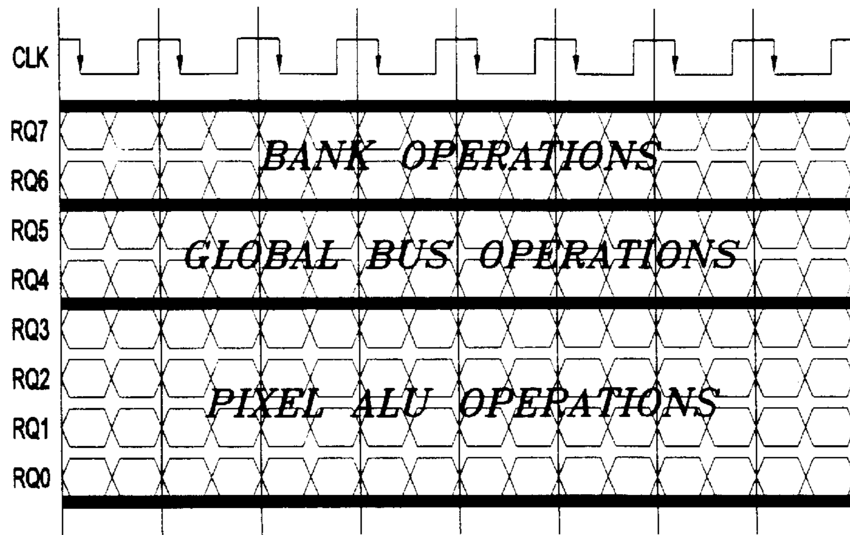
ADDRESS AND CONTROL PROTOCOL
