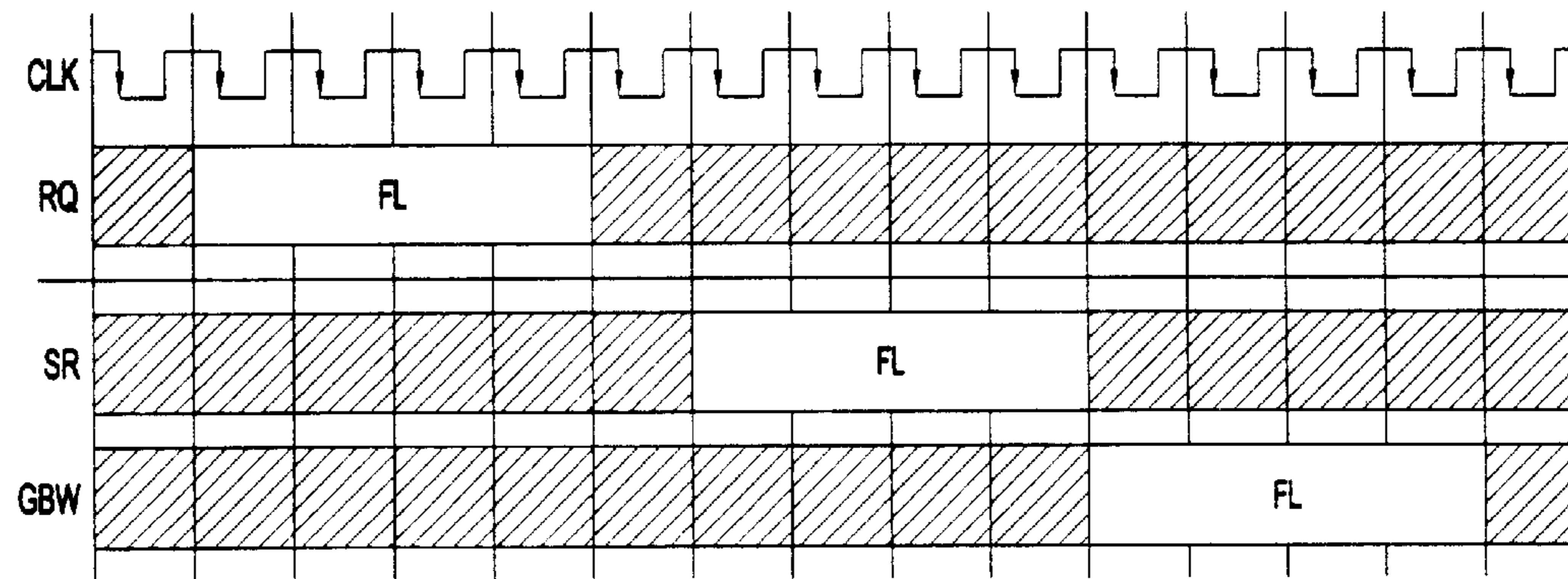
FL OPERATION
