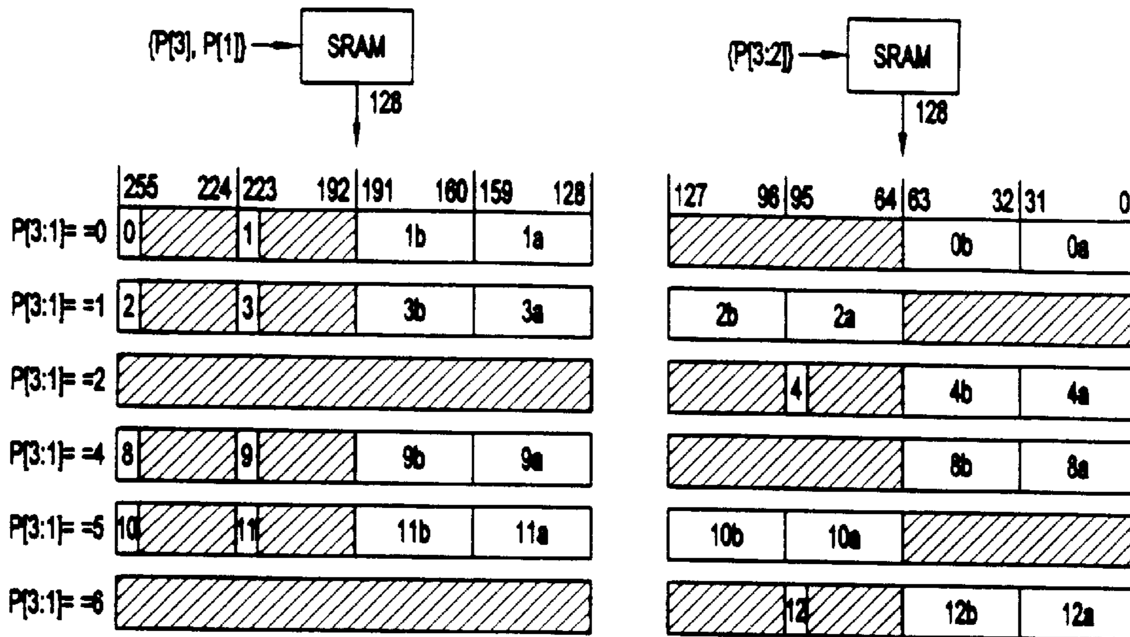
SRAM-TO-DQ ROUTING: 96 BPP
