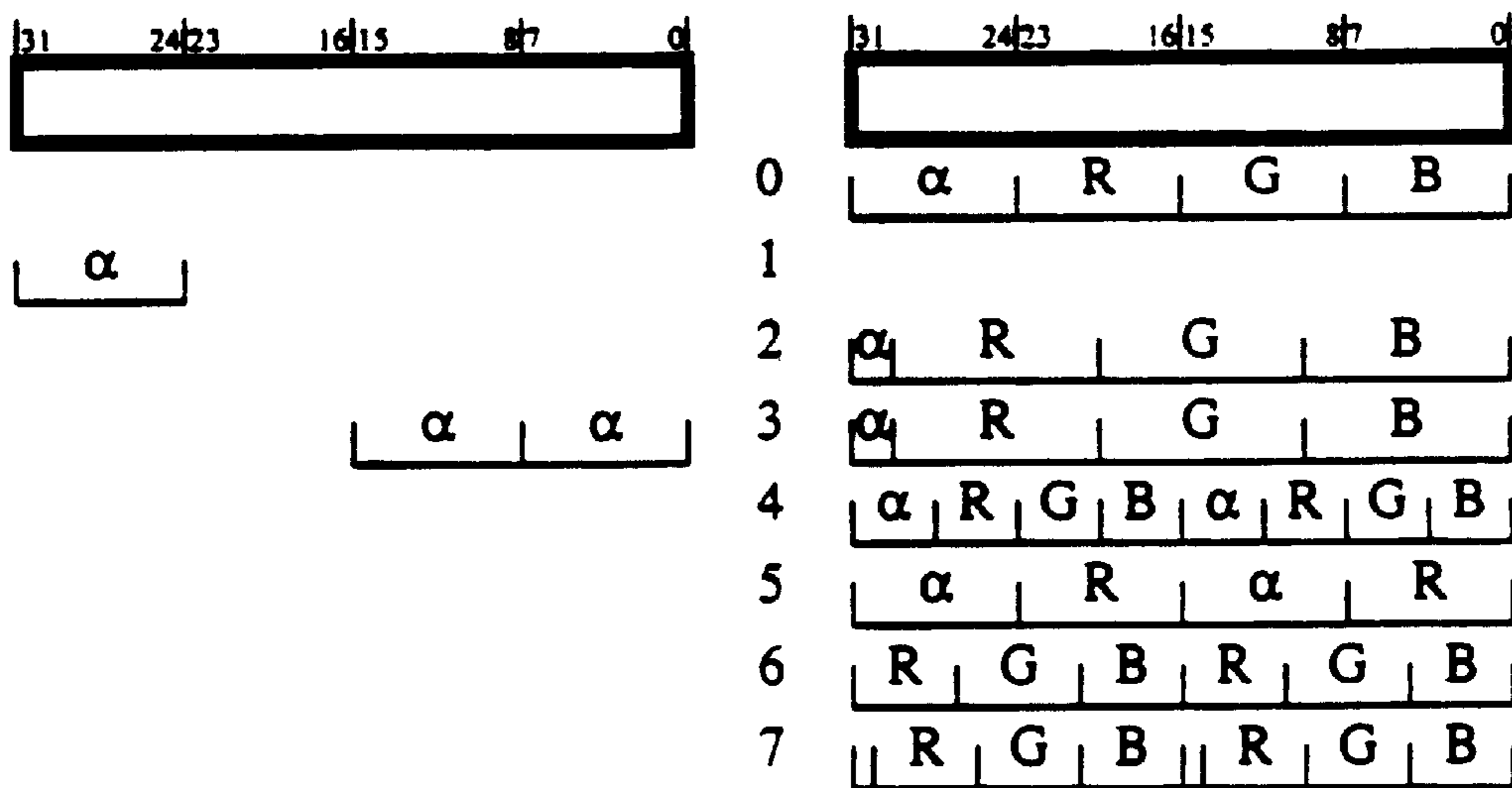
Unpack Functions
