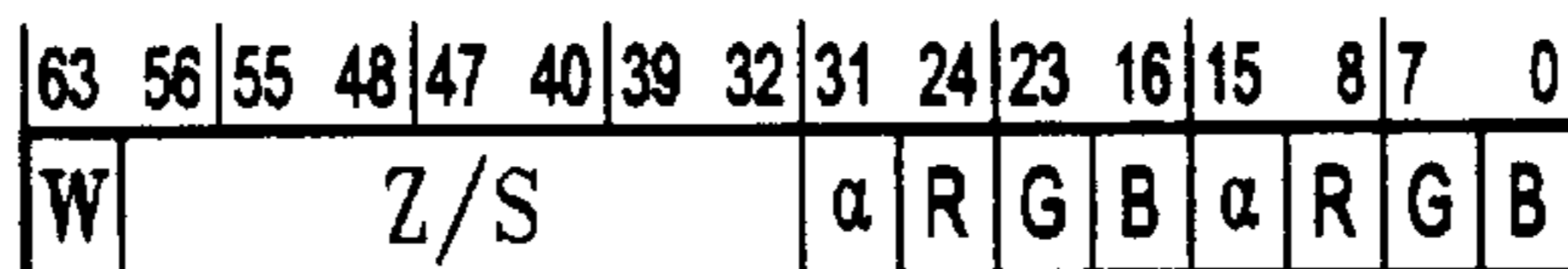
64 BPP PIXEL FORMAT 4:28:2*(4:4:4)
