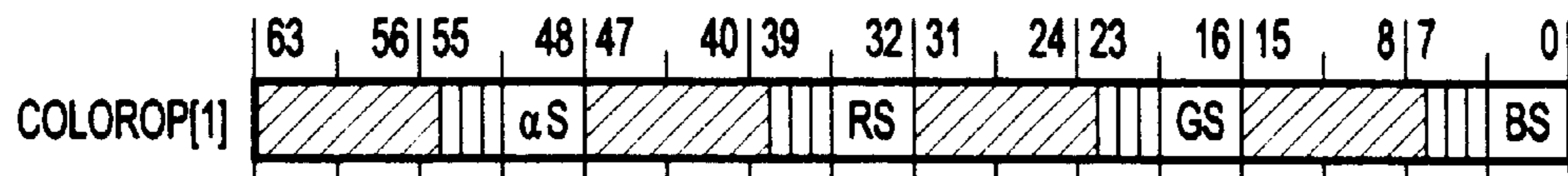
COLOROP[1] REGISTER DATA FORMAT
