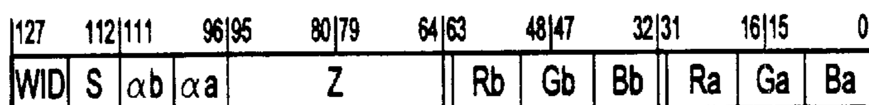
128 bpp Pixel Format 8:8:32:2*(10:10:10:10)
