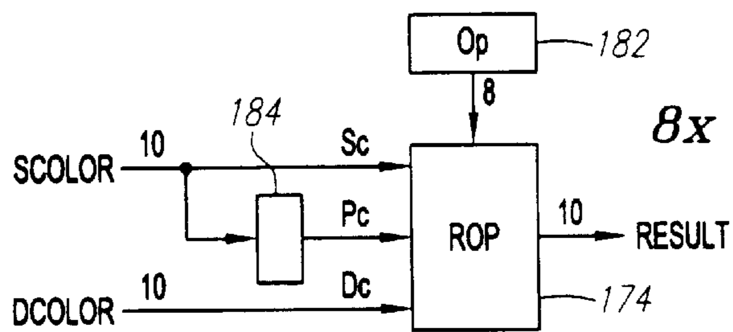
ROP PORTION
