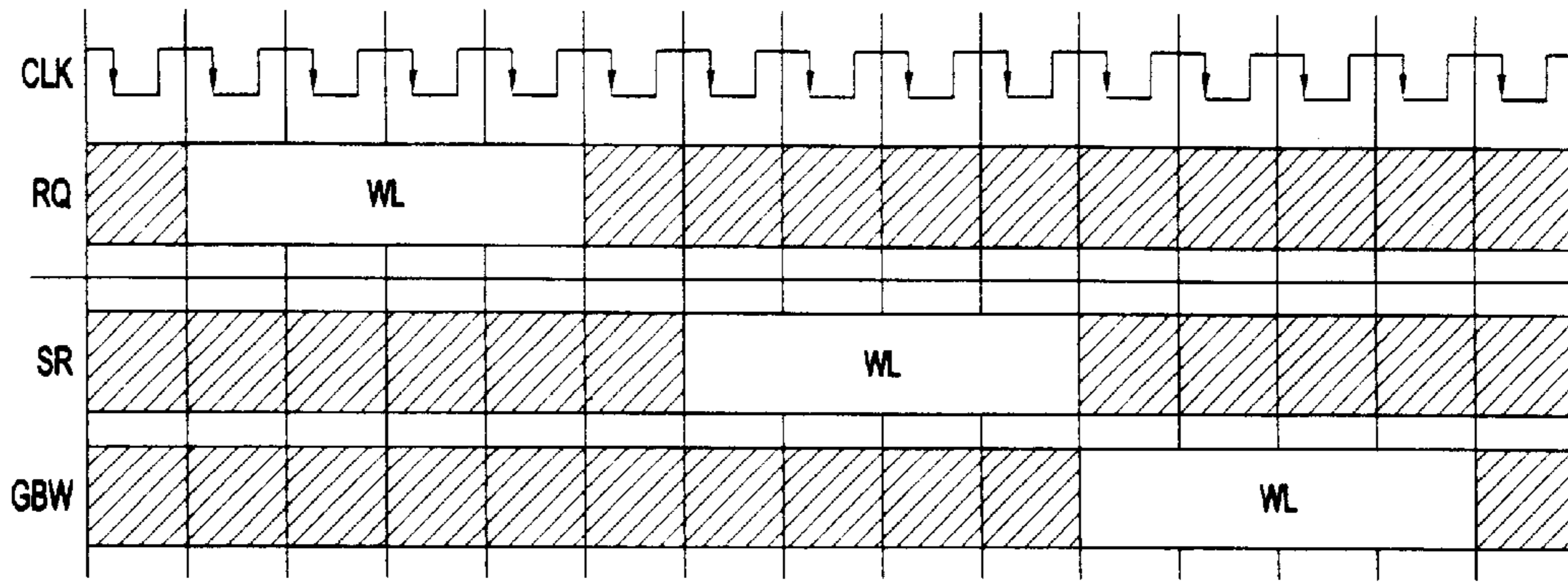
WL OPERATION
