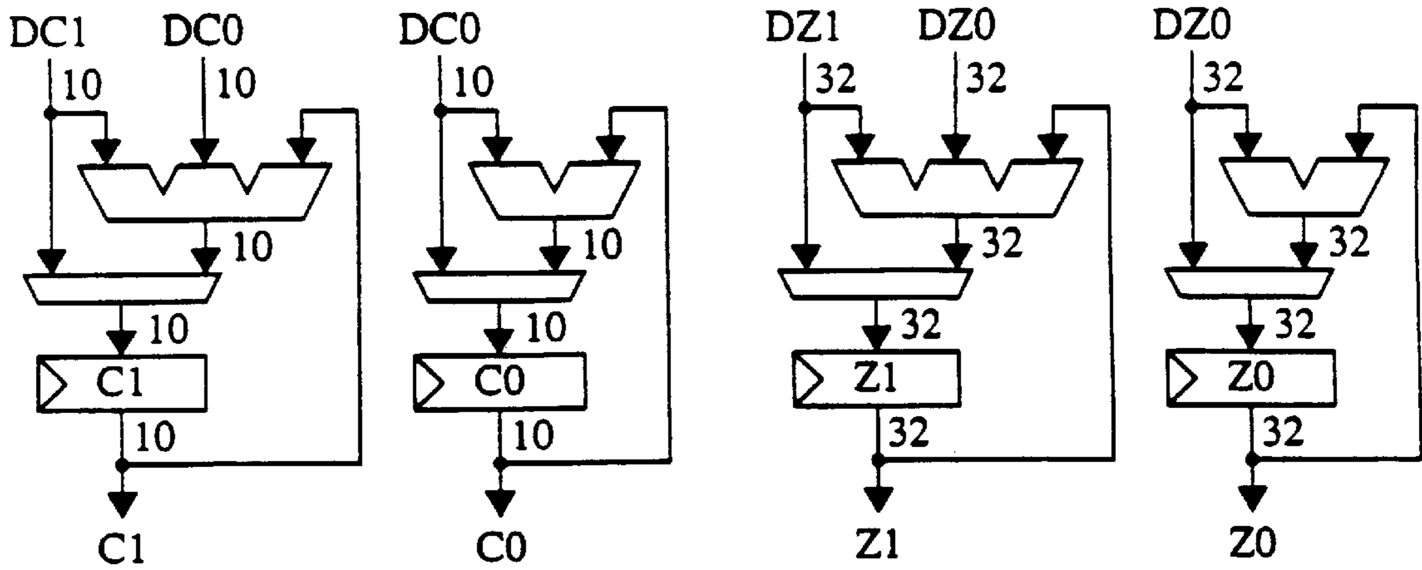
Color and Depth Accumulators
