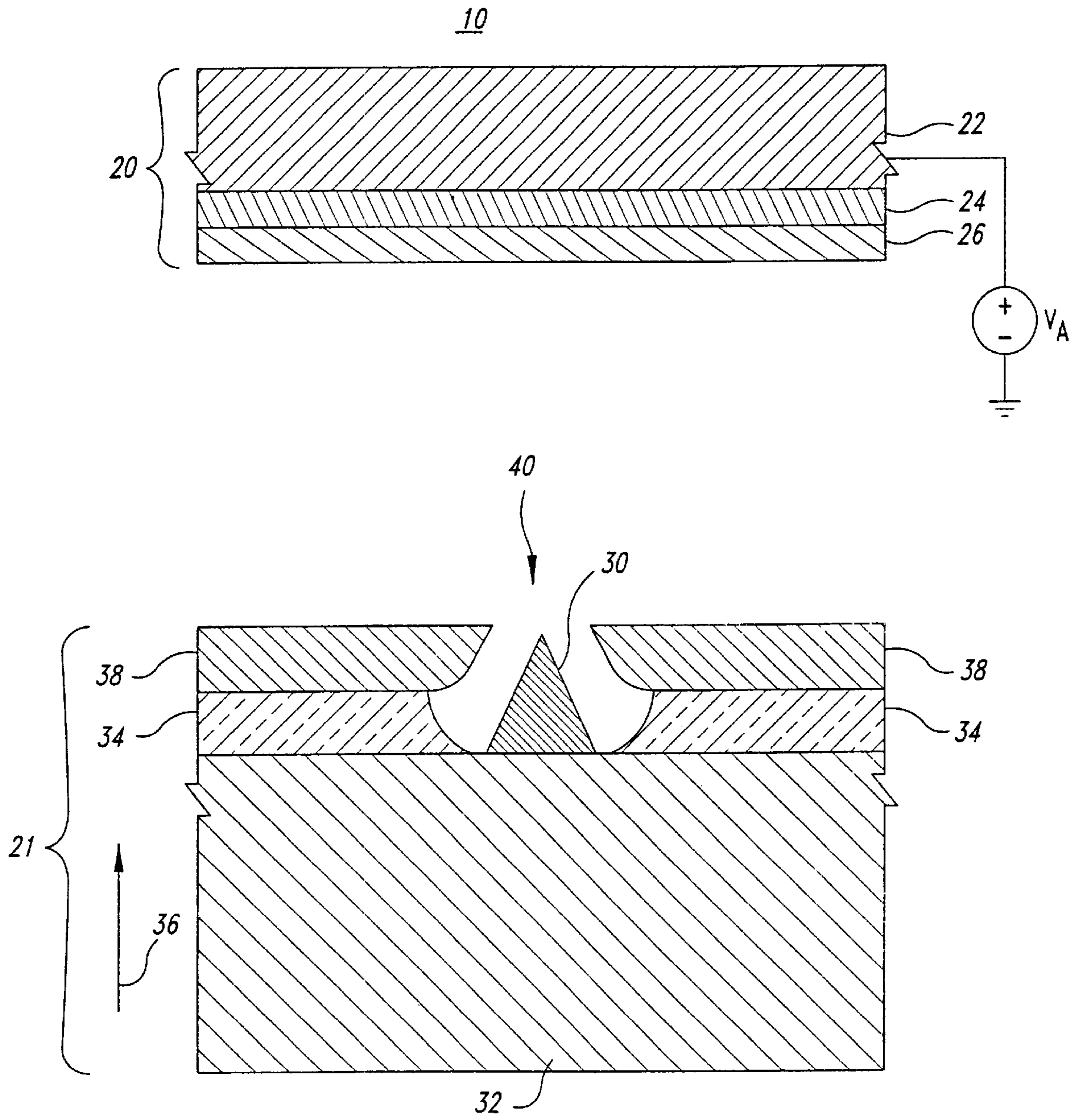
Fig. 1 (PRIOR ART)
