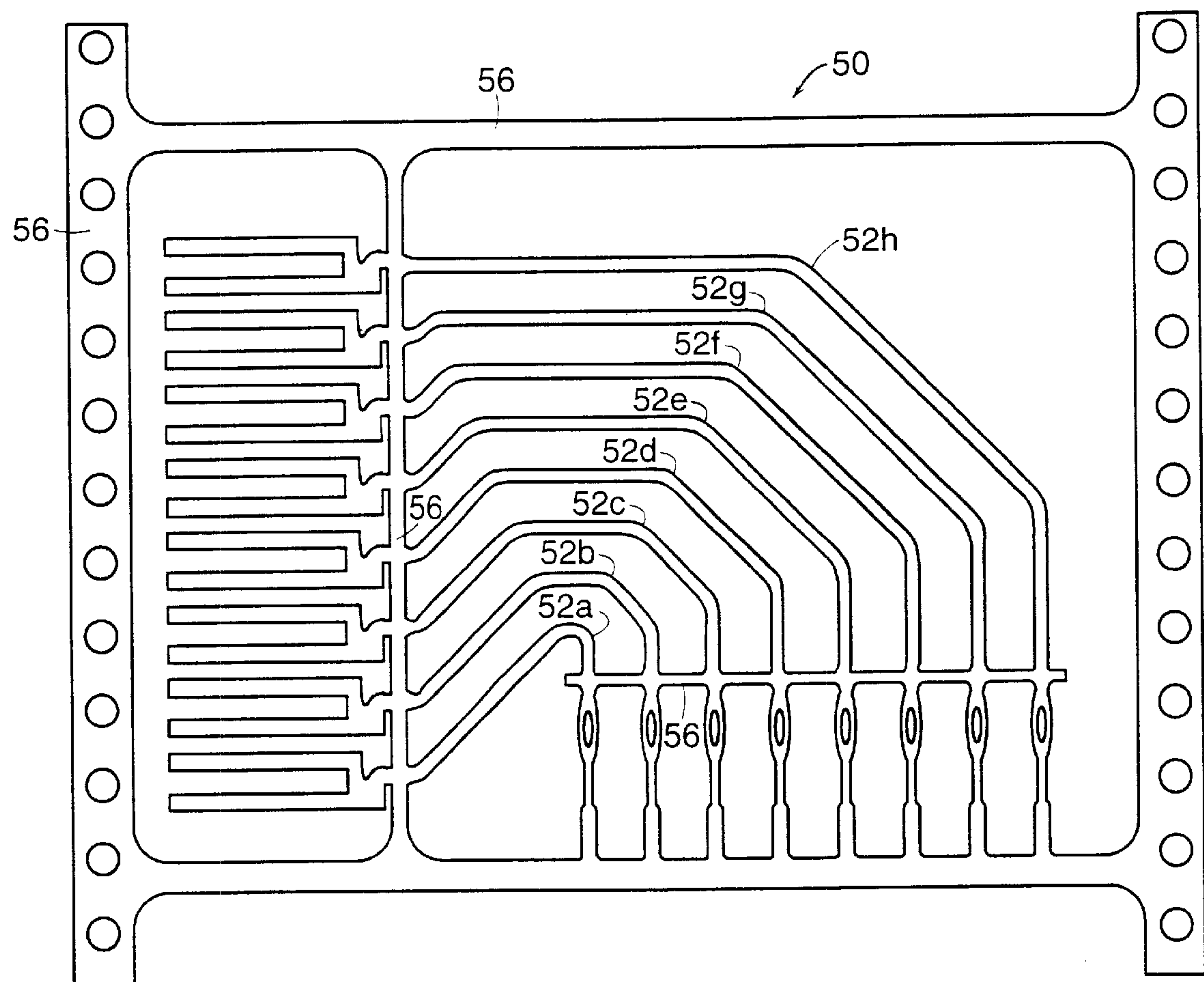
FIG. 2 (PRIOR ART)
