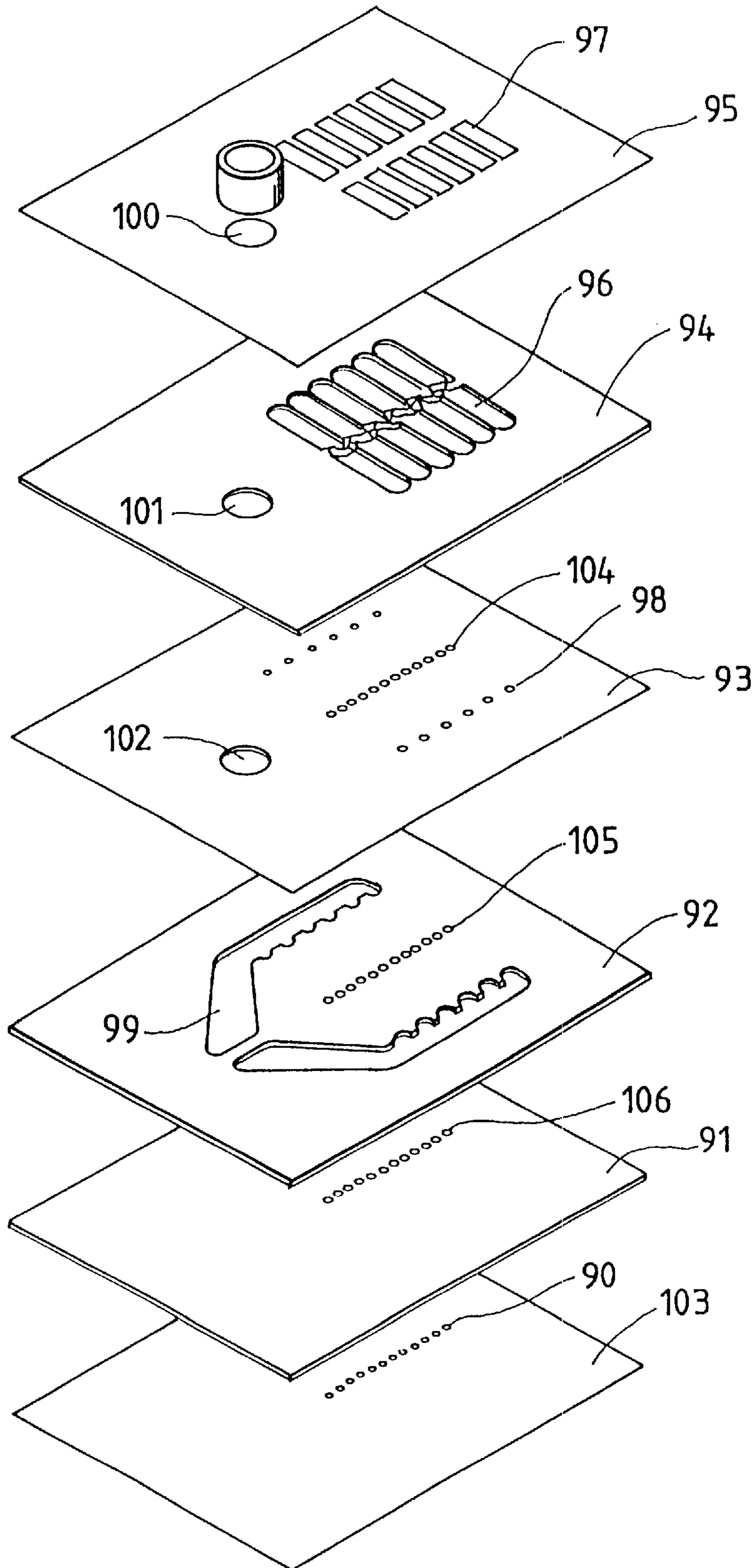
FIG. 13 PRIOR ART
