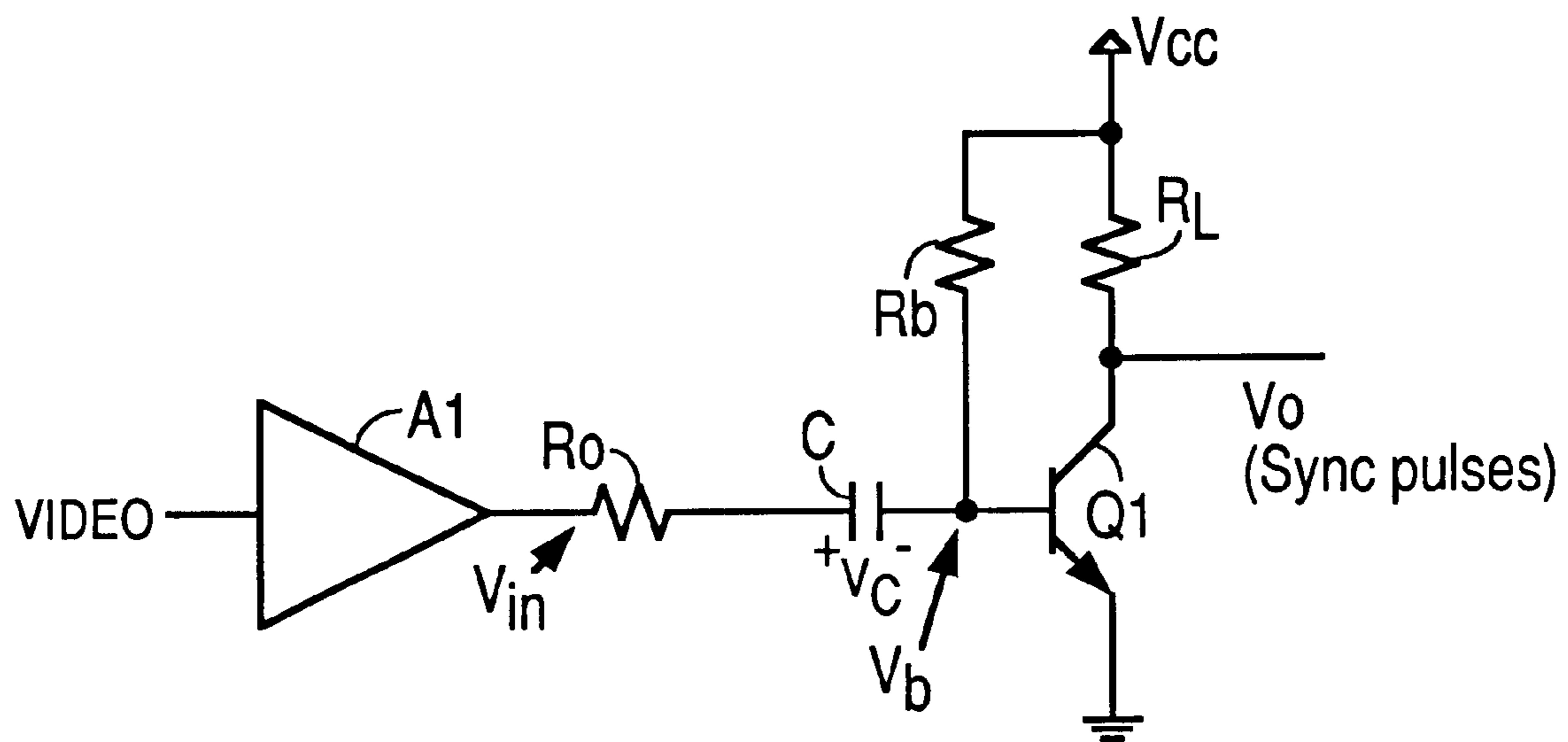
FIG. 10 (PRIOR ART)
