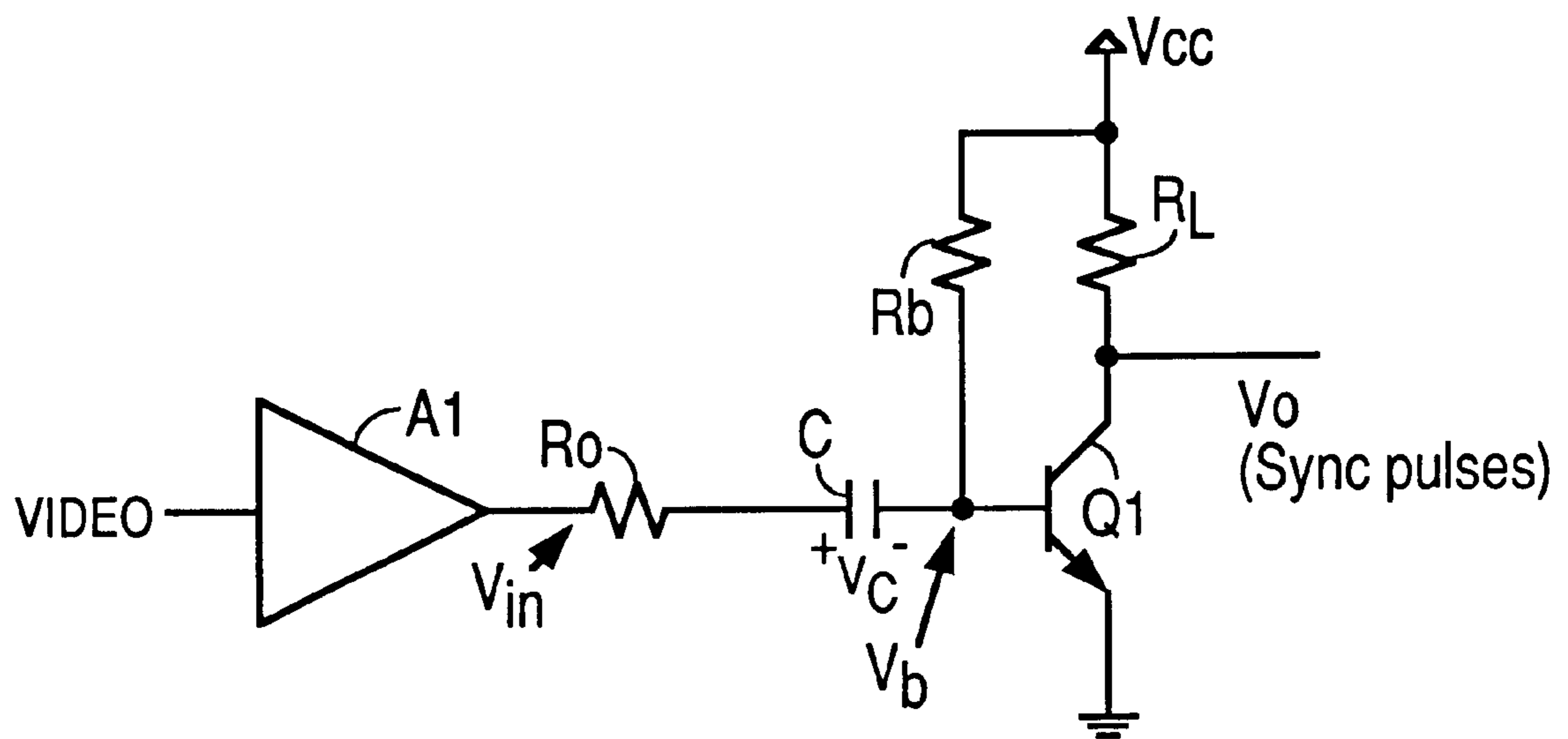
FIG. 10 (PRIOR ART)
