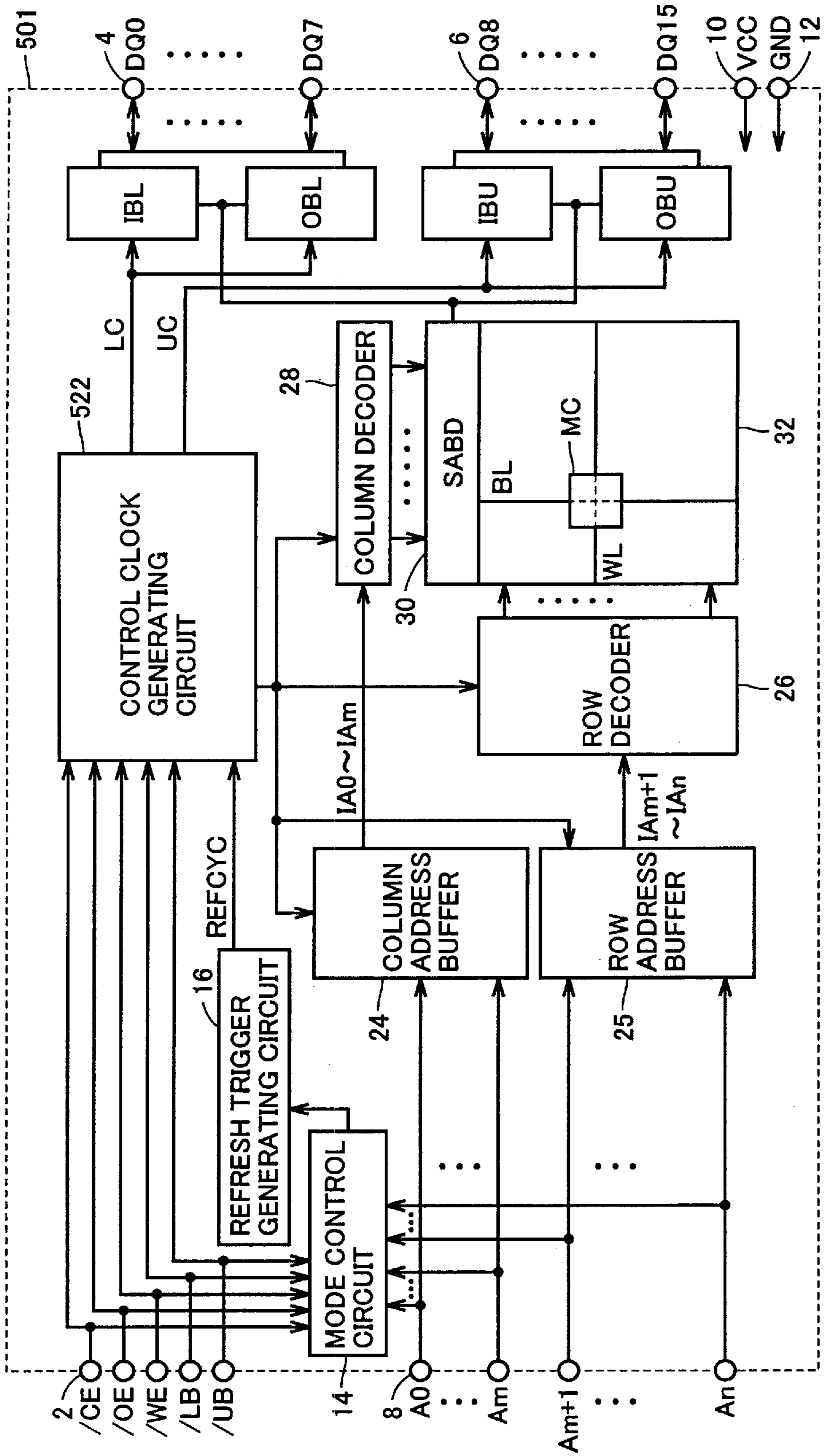
FIG.8 PRIOR ART
