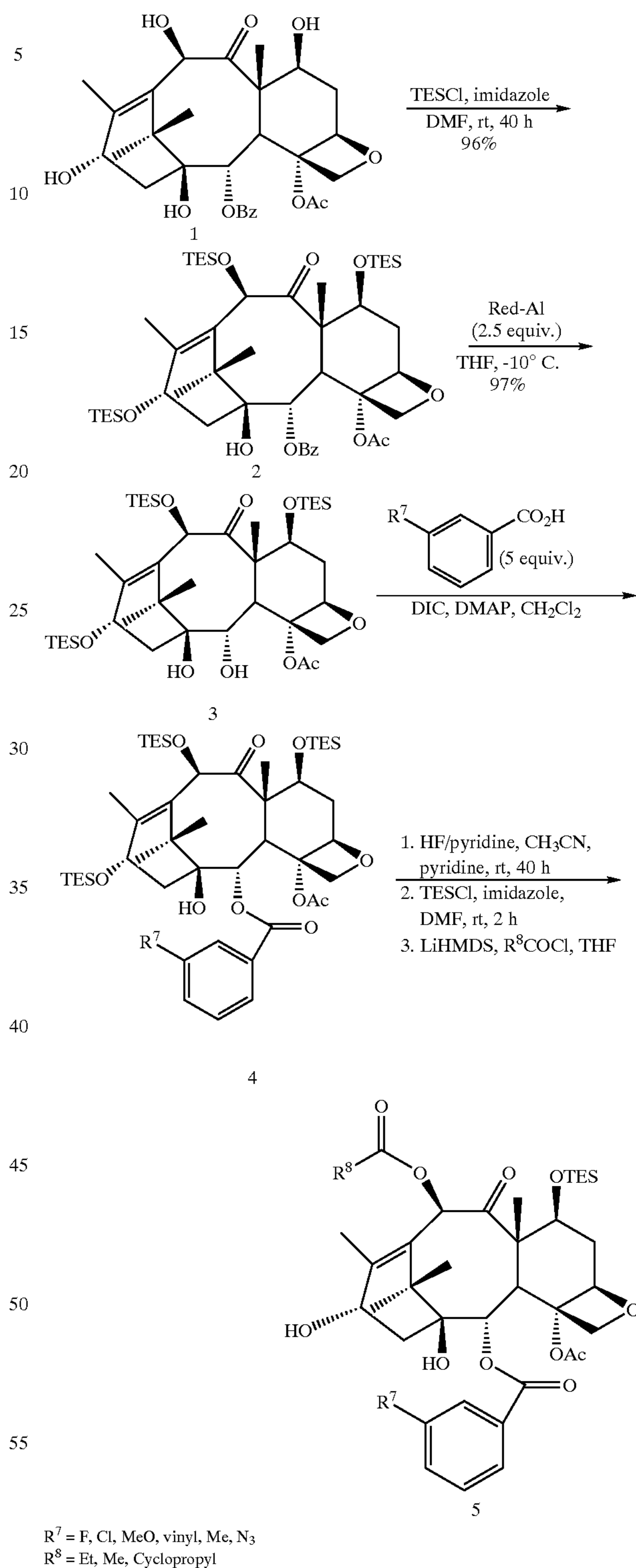
Scheme 1
