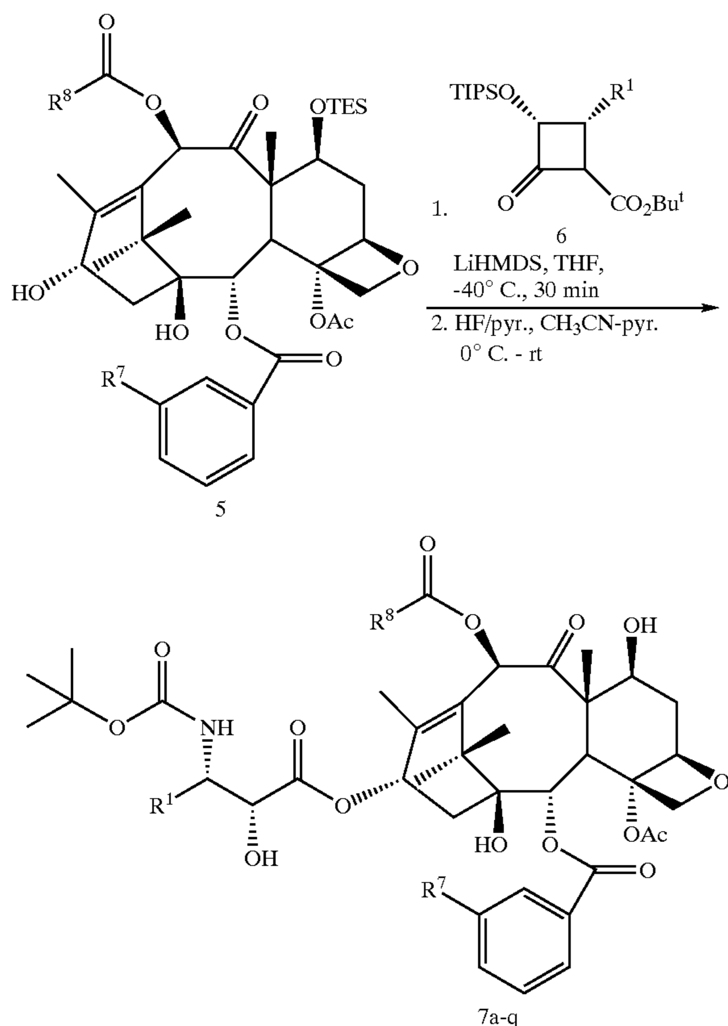
Scheme 2
