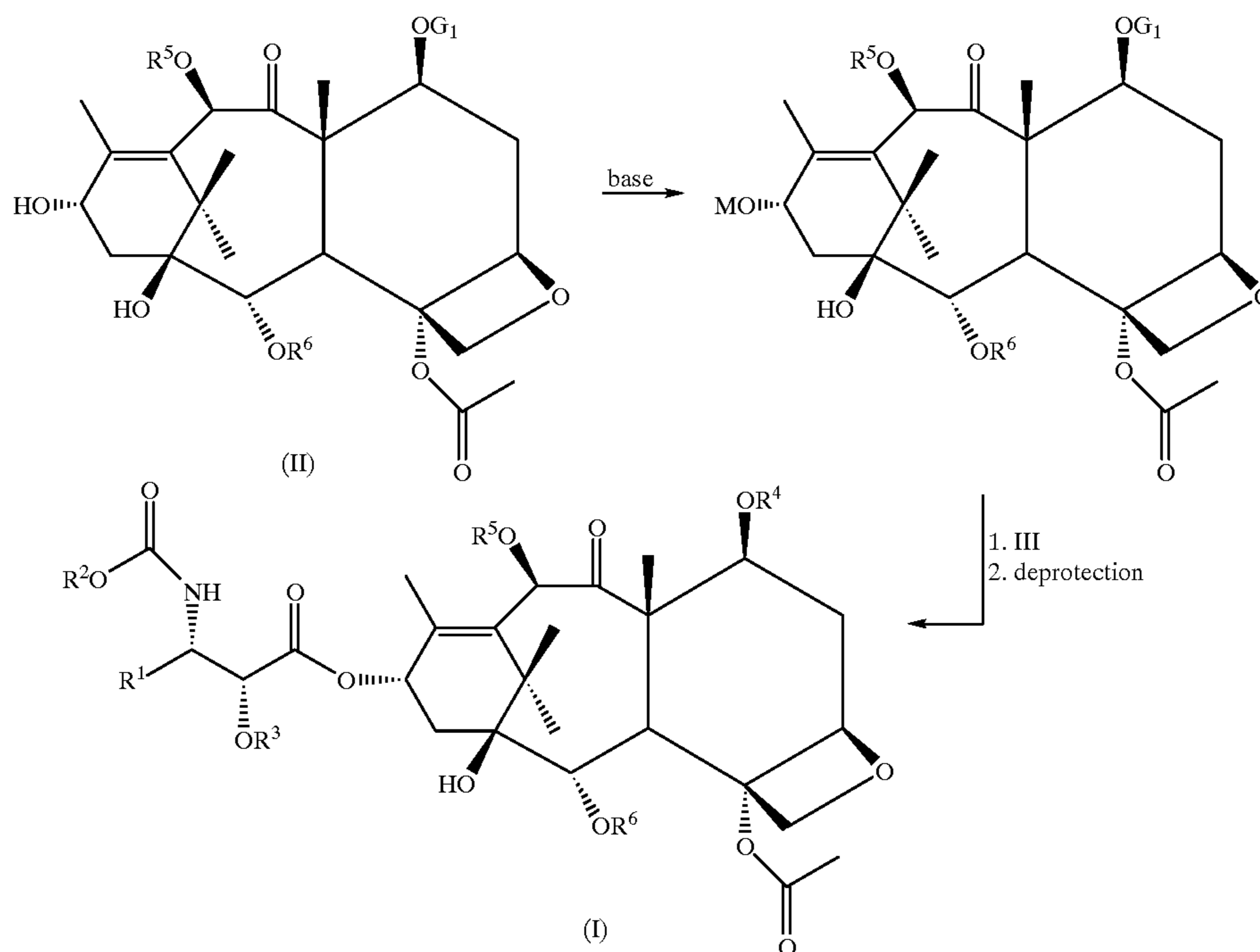
Scheme 3
