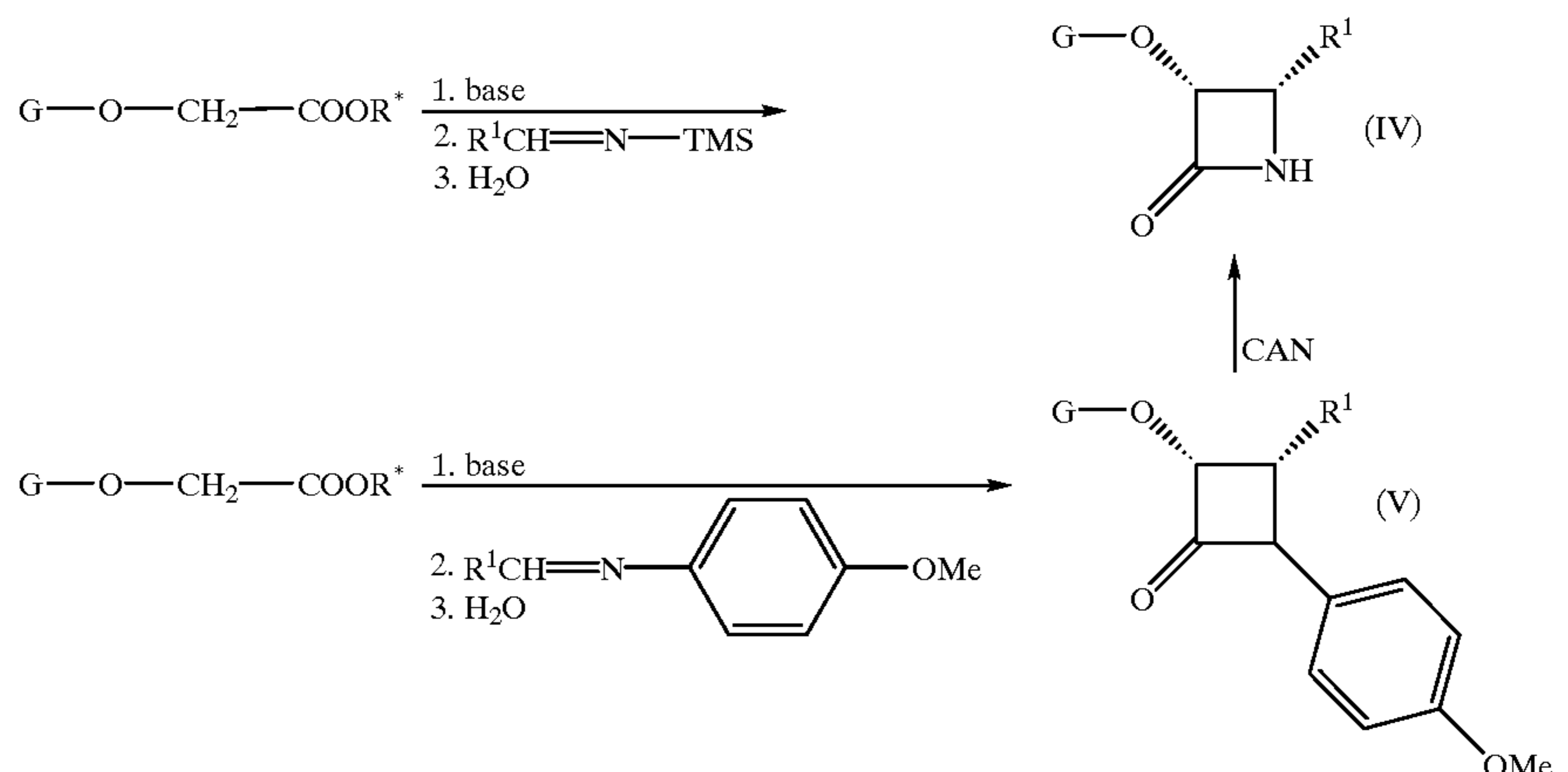
Scheme 1
