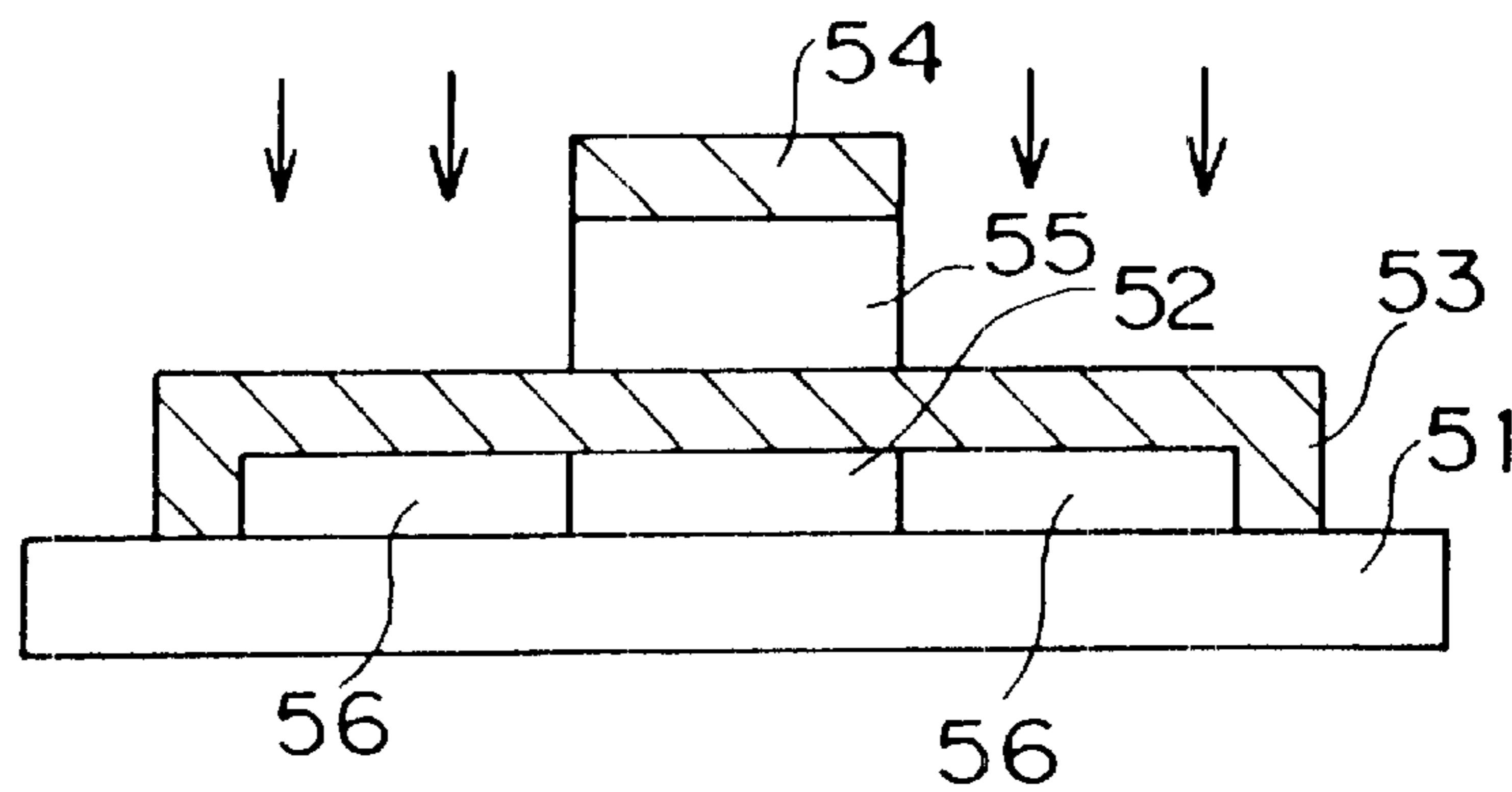
Fig. 32 PRIOR ART
