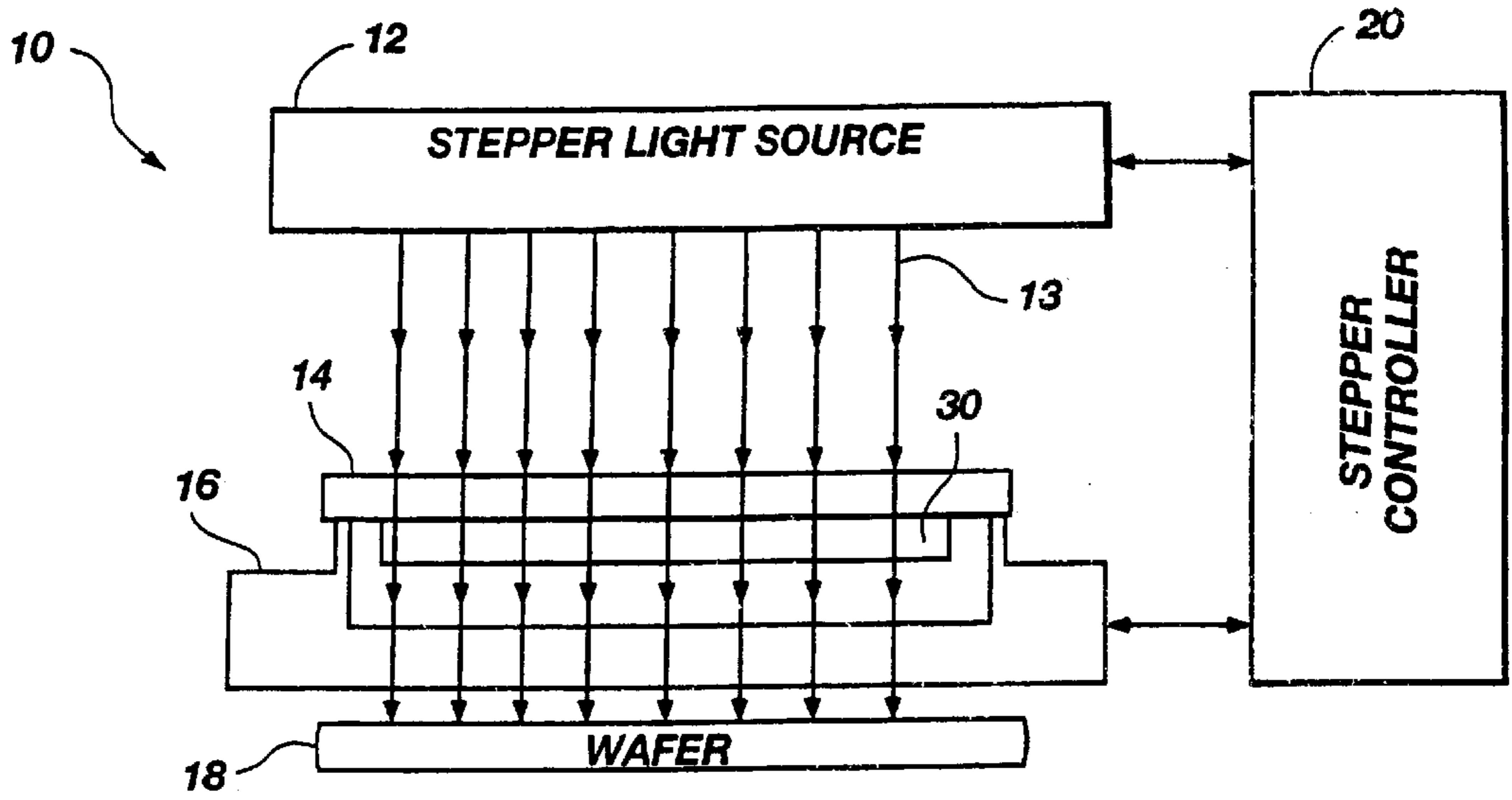
Fig. 1 (PRIOR ART)
