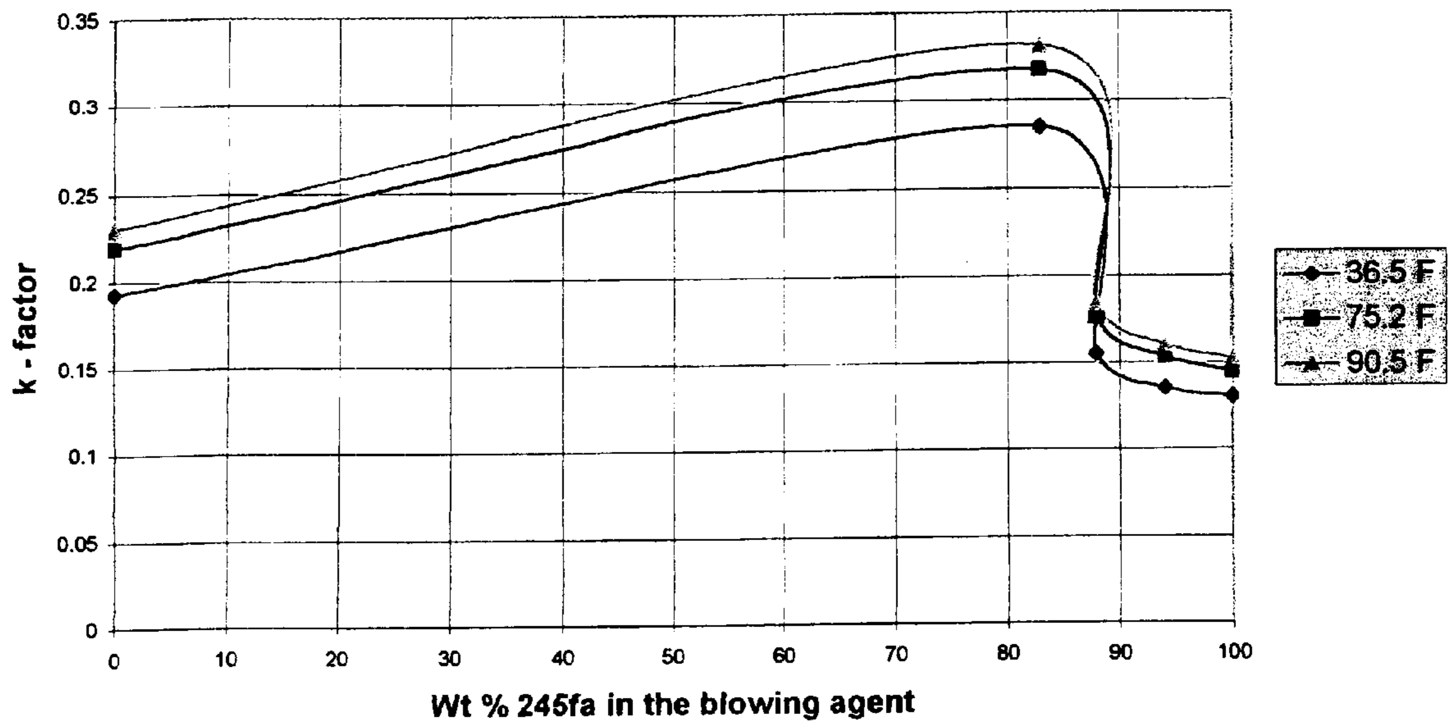
k - factors of foams
