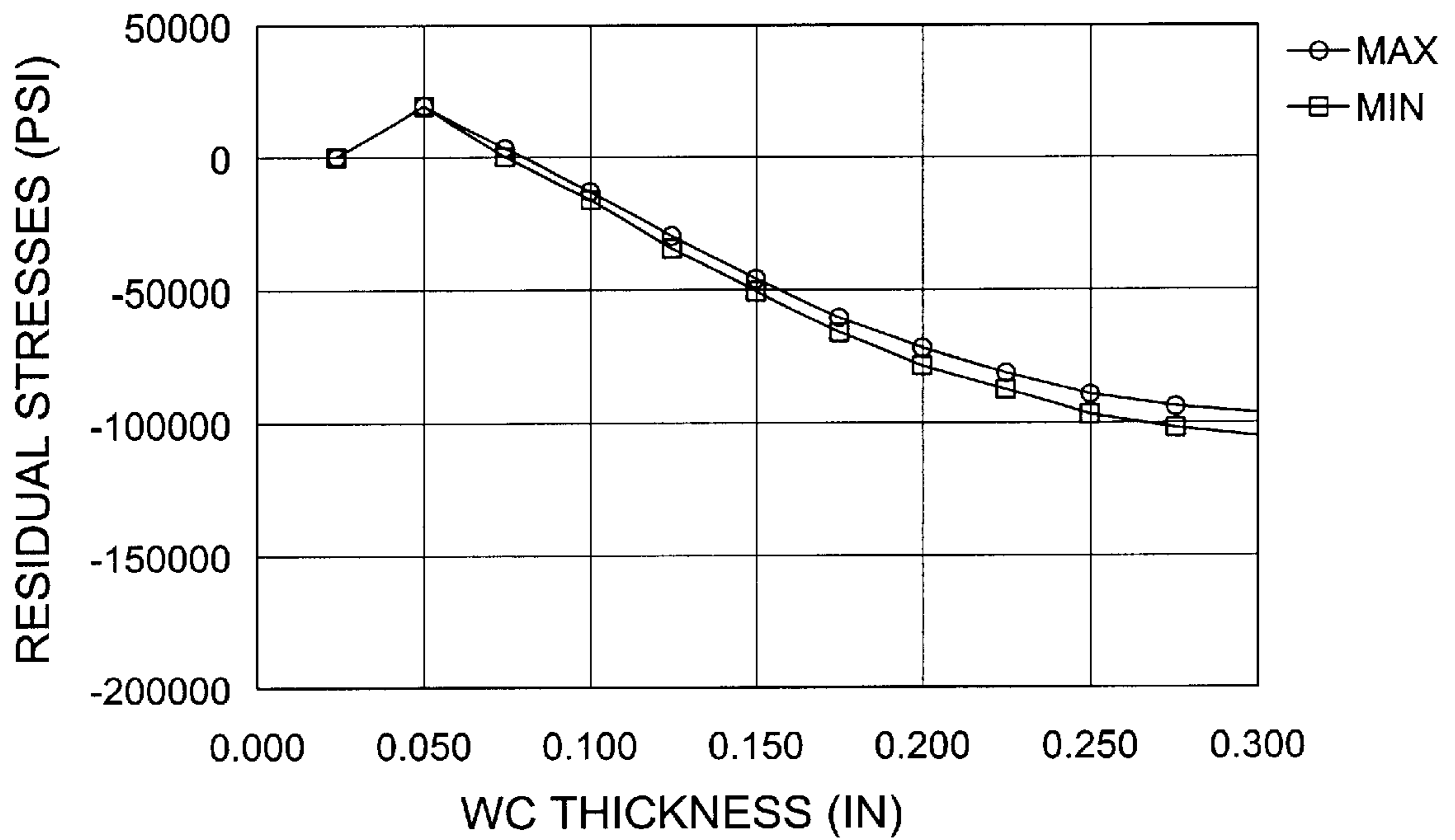
Fig. 4 RESIDUAL STRESSES IN .529 SINGLE LAYER 13% CO
