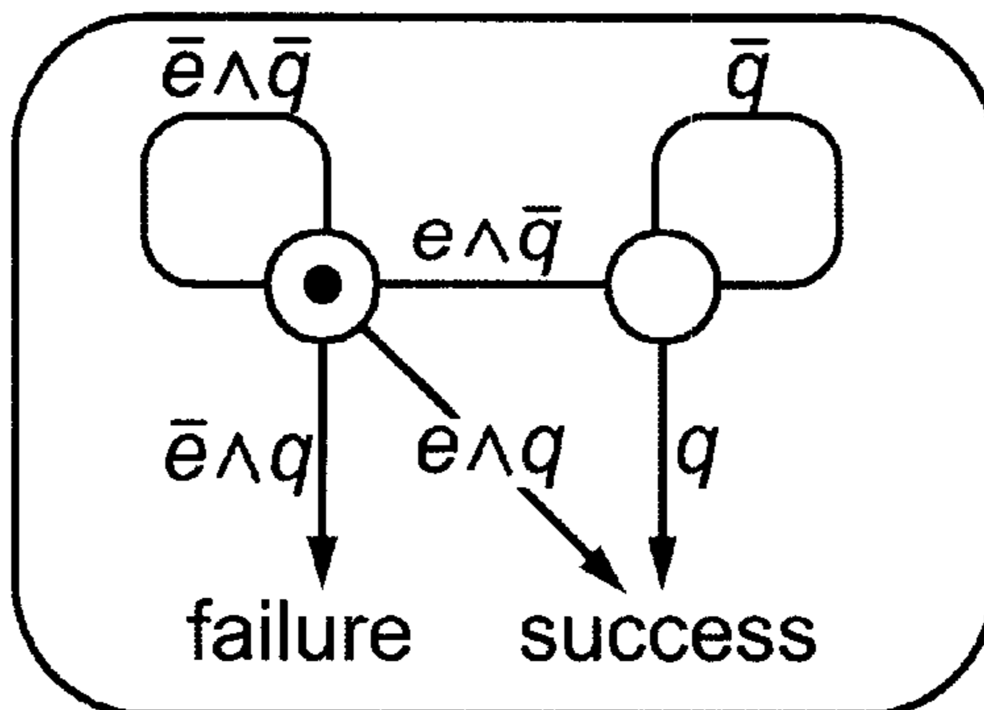
Event e sampled at q
