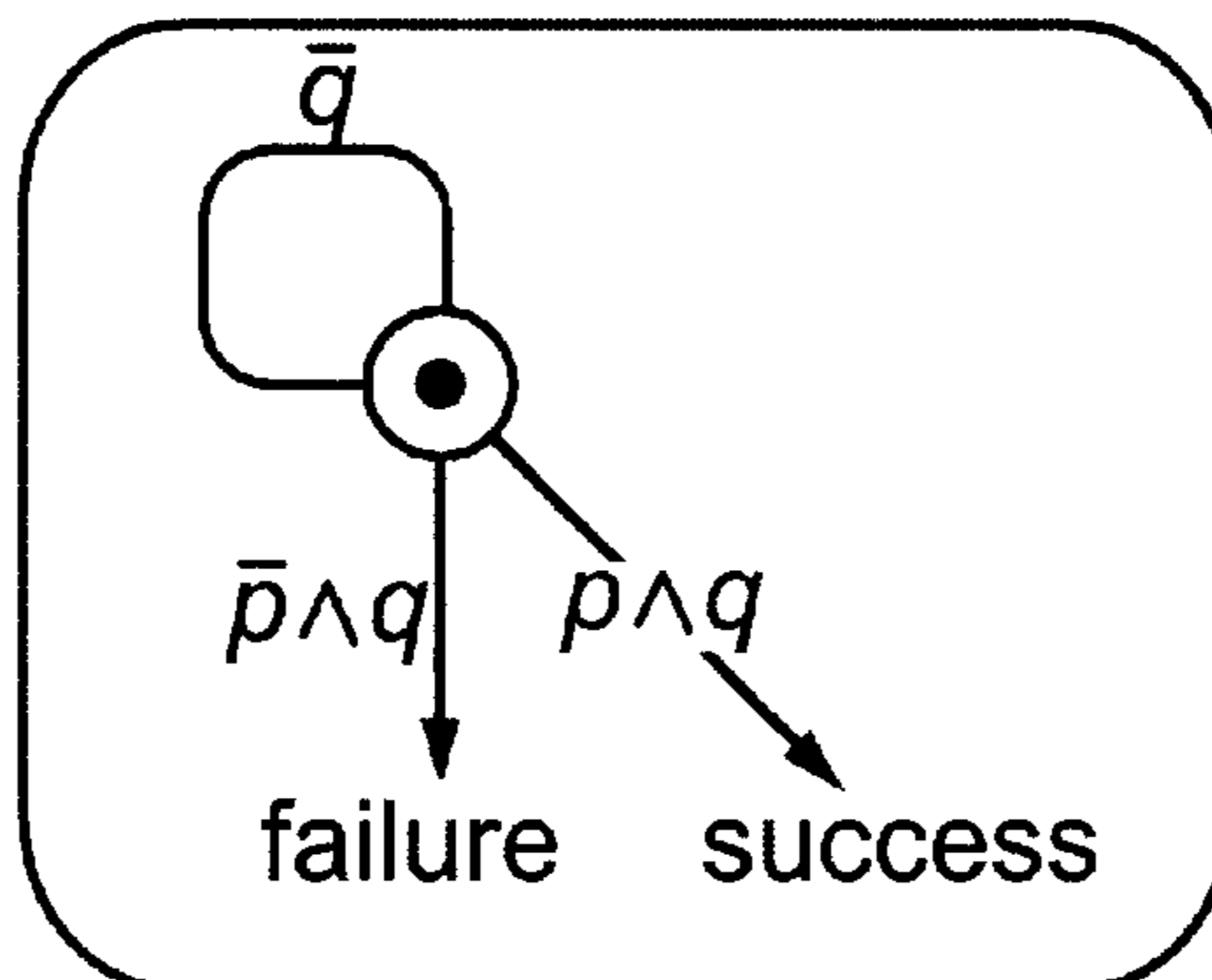
Proposition p sampled at q
