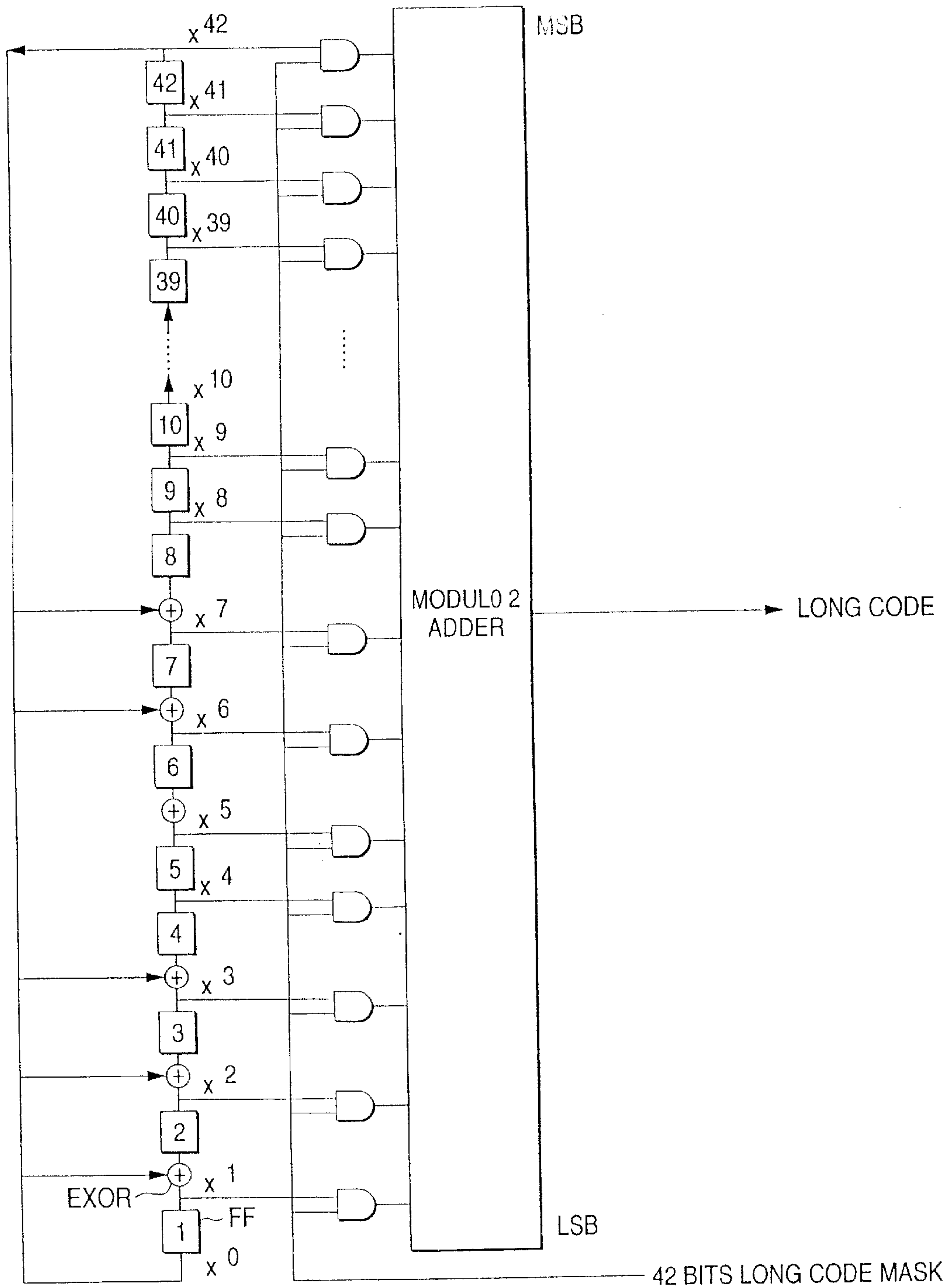
FIG. 7 PRIOR ART
