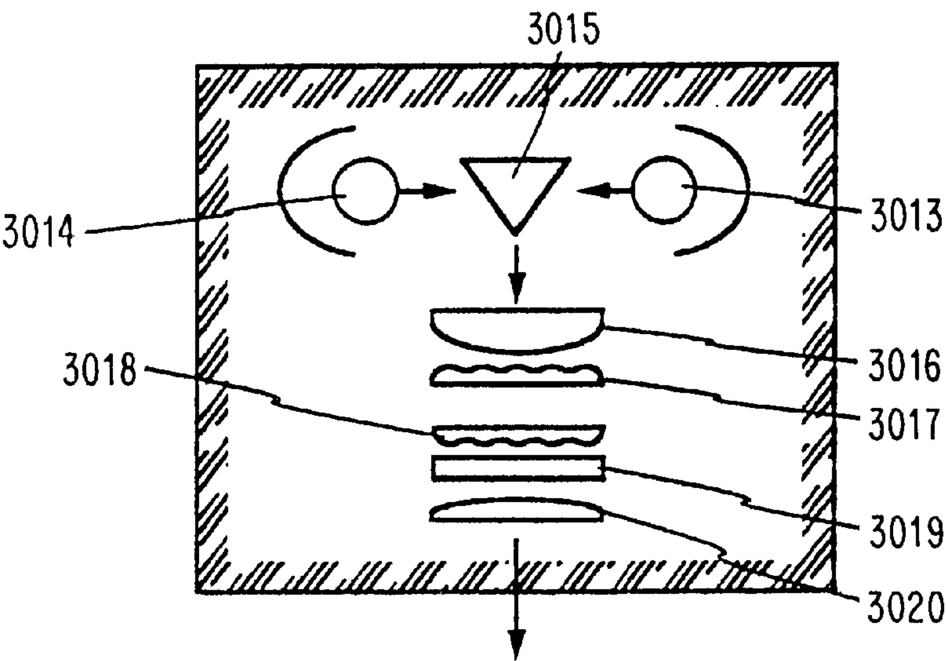
FIG. 27B OPTICAL LIGHT SOURCE SYSTEM
