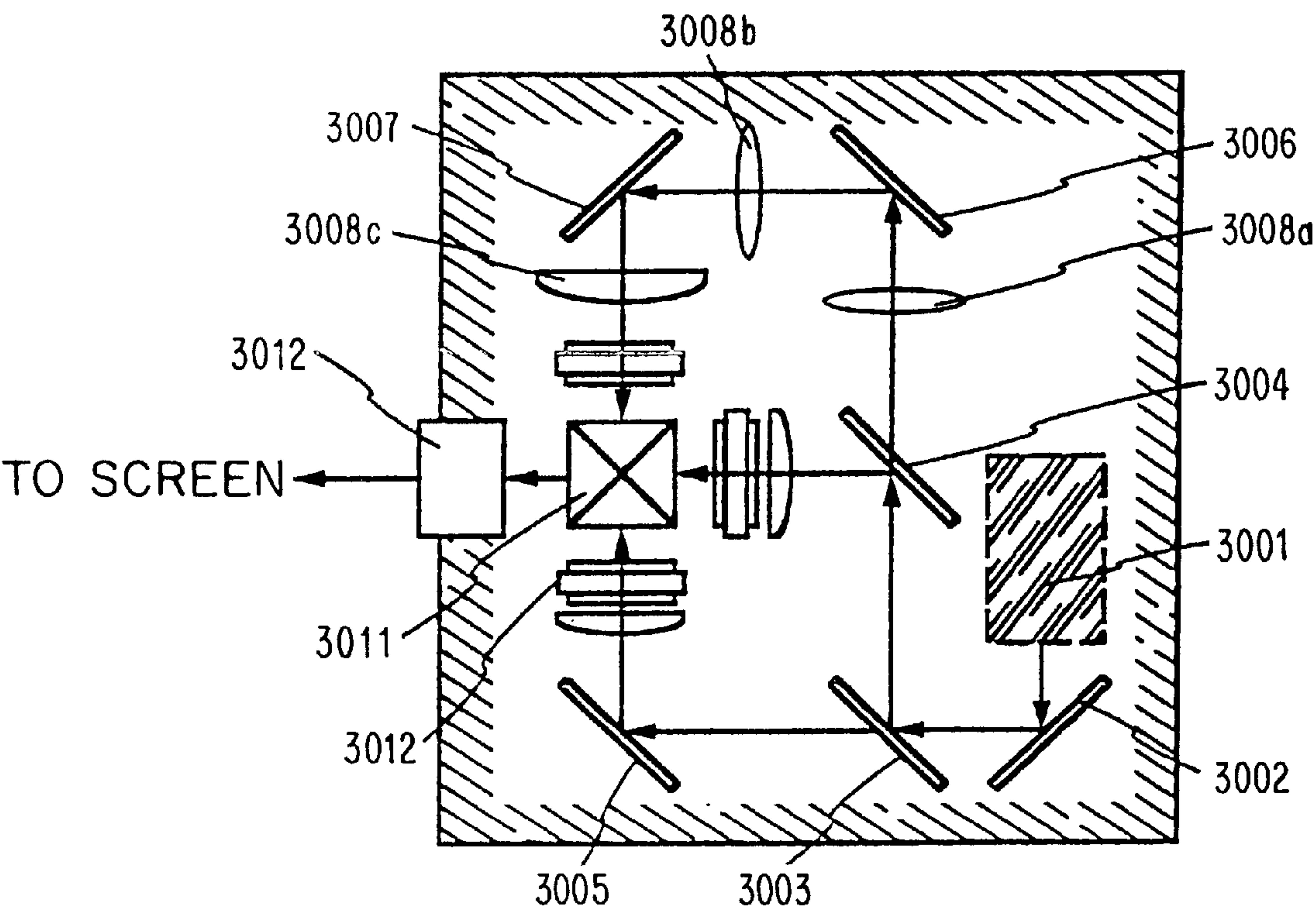
FIG. 27B OPTICAL LIGHT SOURCE SYSTEM
