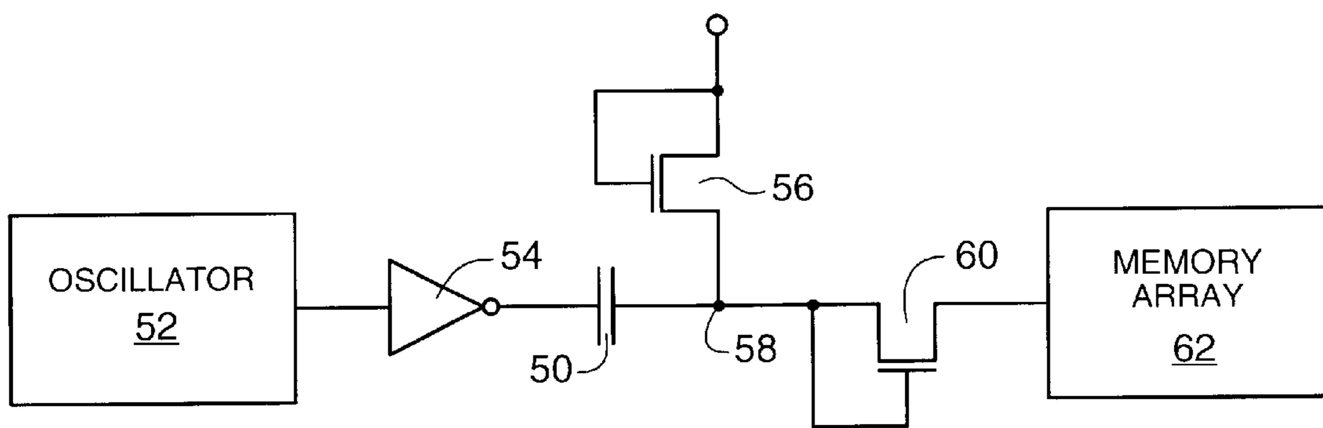
FIG. 5 (PRIOR ART)
