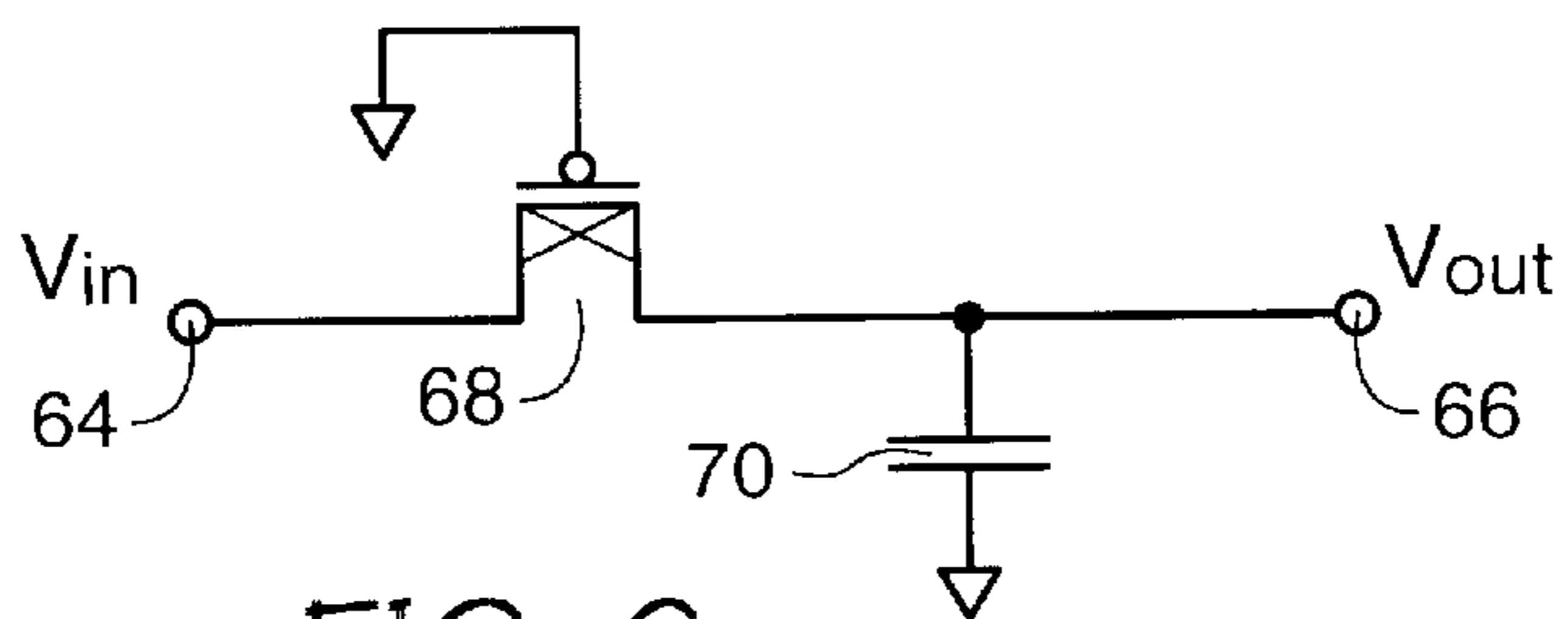
FIG. 6 (PRIOR ART)
