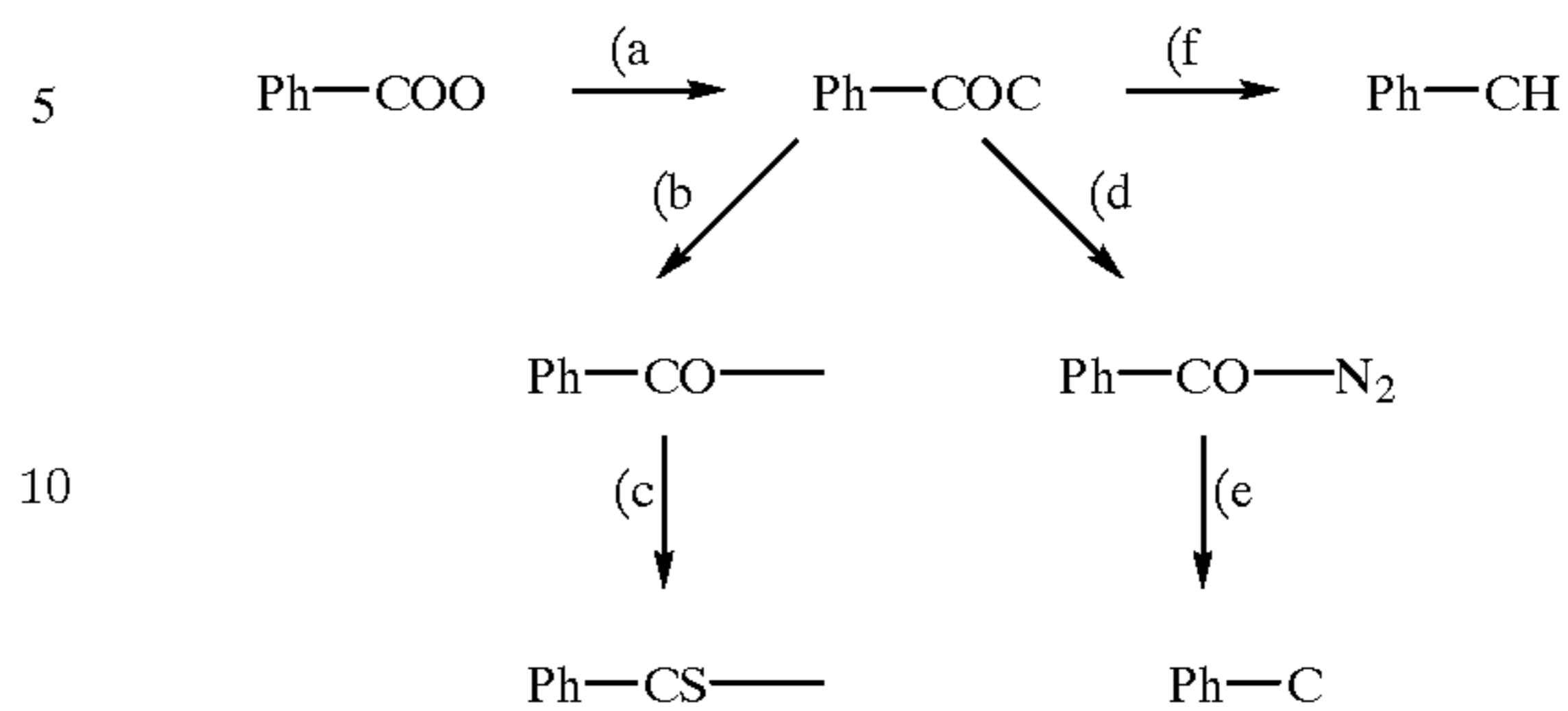
Equation 3: Conversion of the group z
