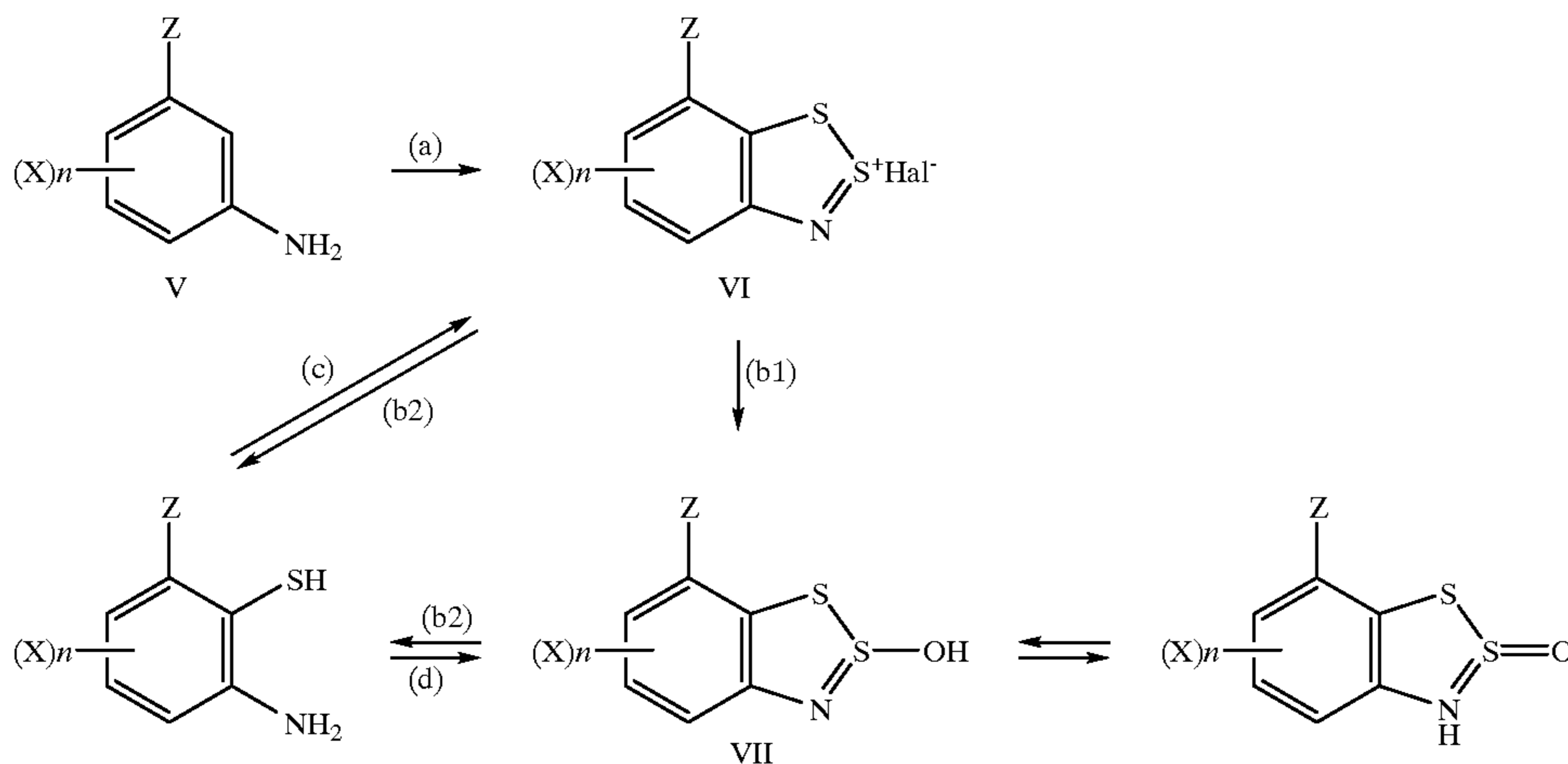
Equation 2
