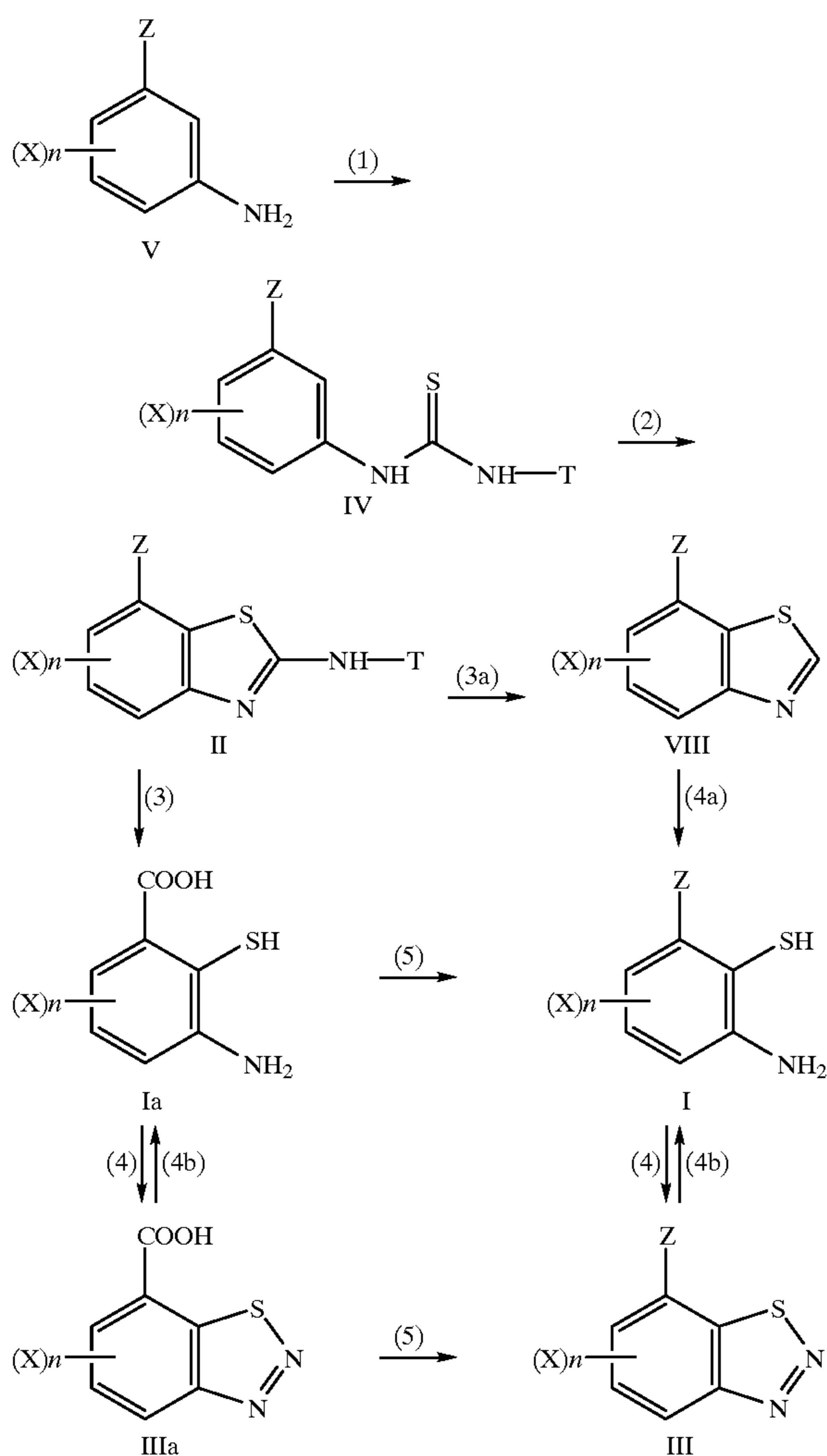
Equation 1
