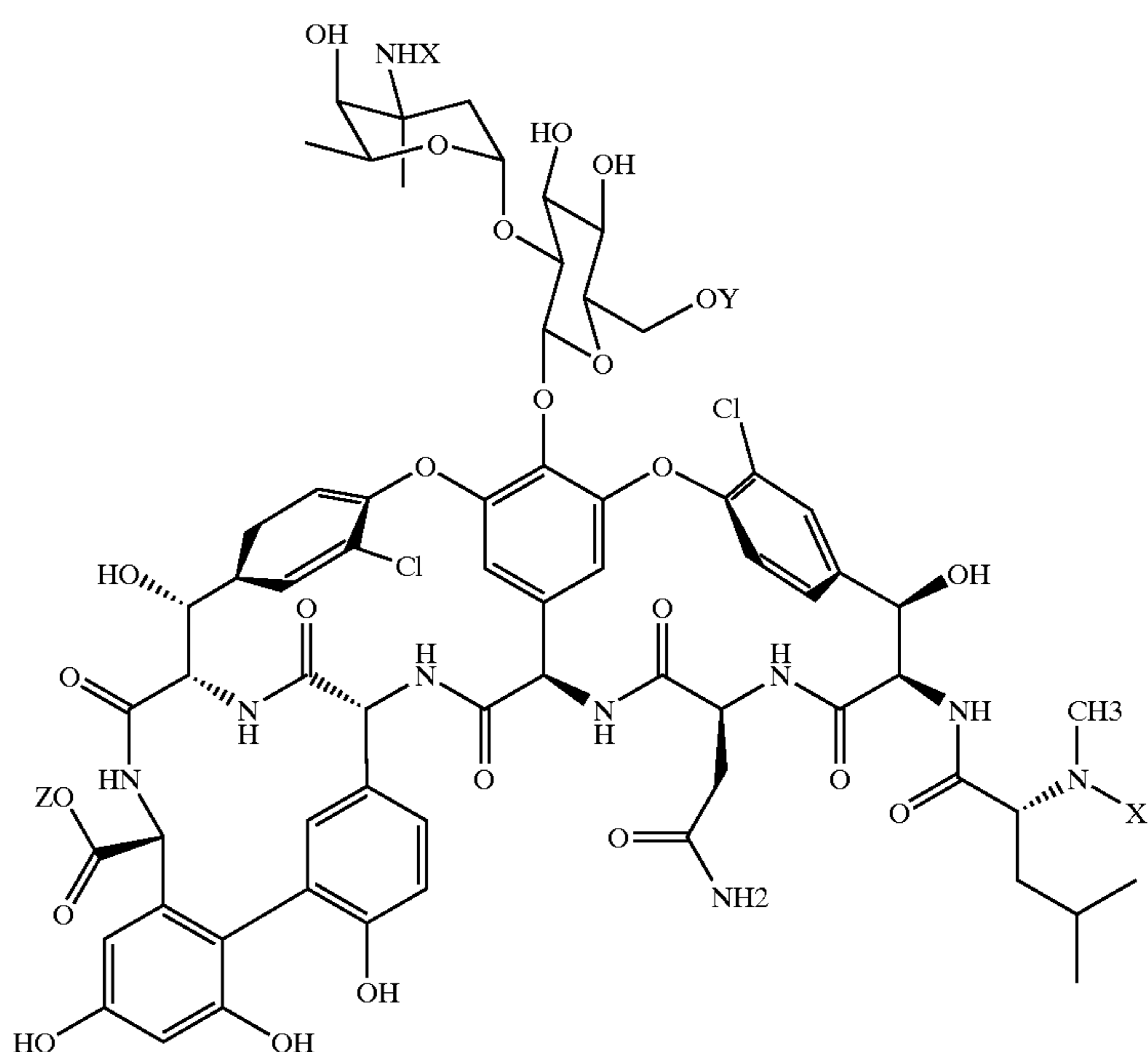
Scheme 1
