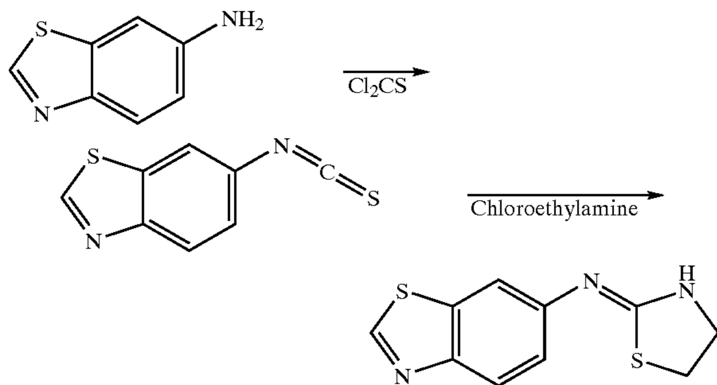
Scheme 6 illustrates schematically the synthesis of a 6-(2-thiazolin-2ylamino) benzothiazole
