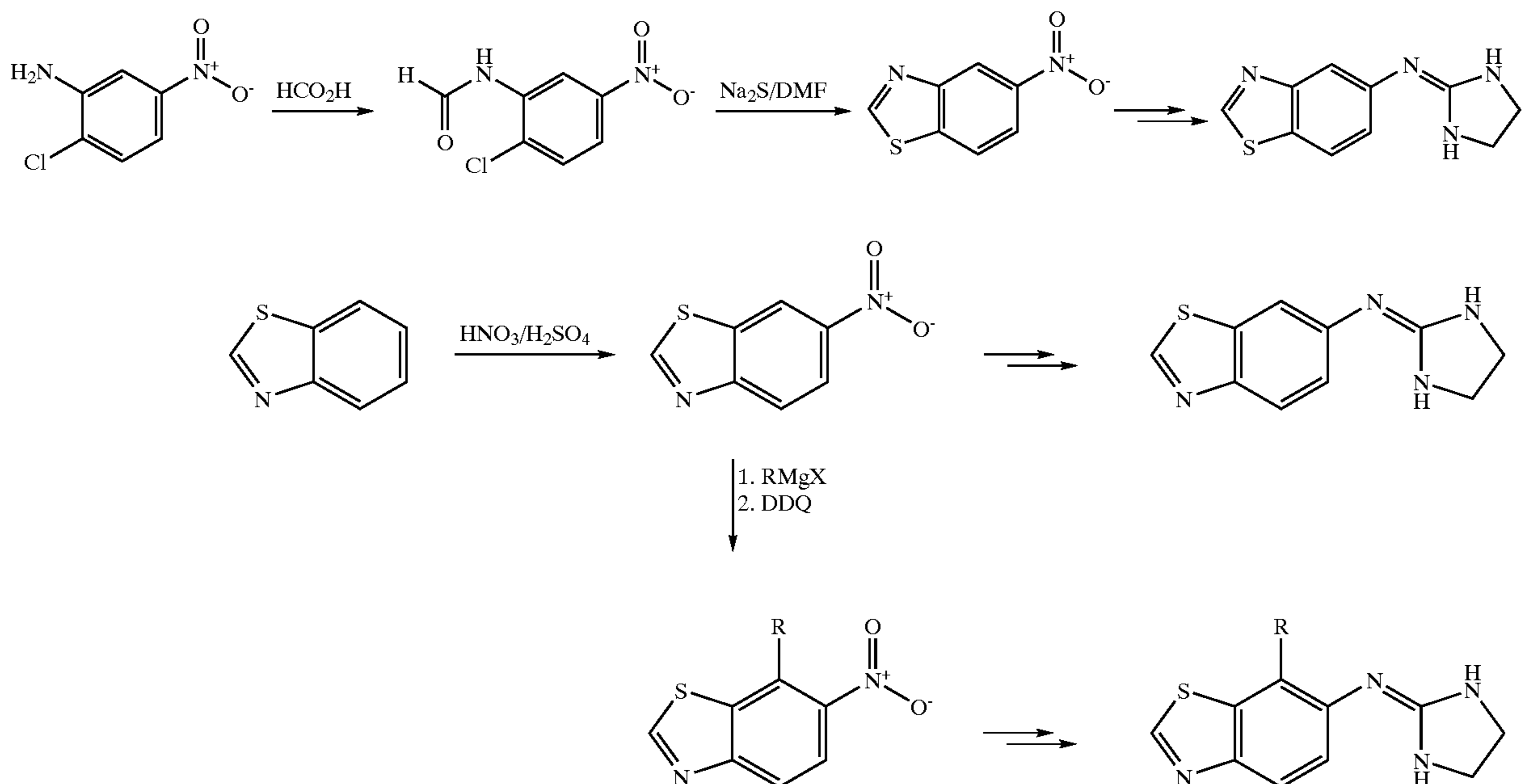
Scheme 4 illustrates schematically the synthesis of a 5-(2-imidazolin-2ylamino) benzothiazole as well as synthesis of 7-substituted derivatives of 6-(2-imidazolin-2ylamino) benzothiazole, where R is alkyl or alkenyl
