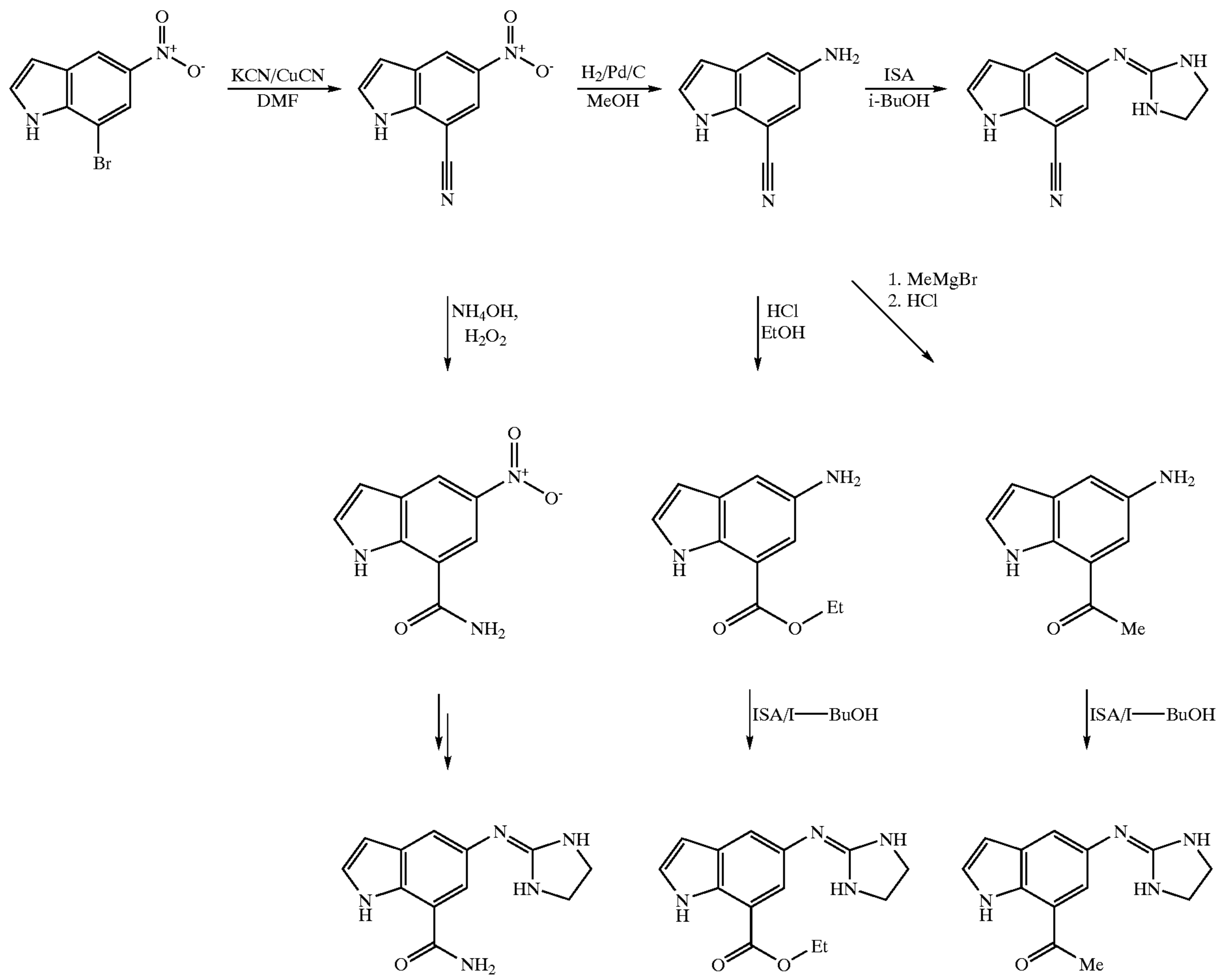
Scheme 2 illustrates schematically the synthesis of 7-substituted derivatives of 5-(2-imidazolin-2-ylamino) indole
