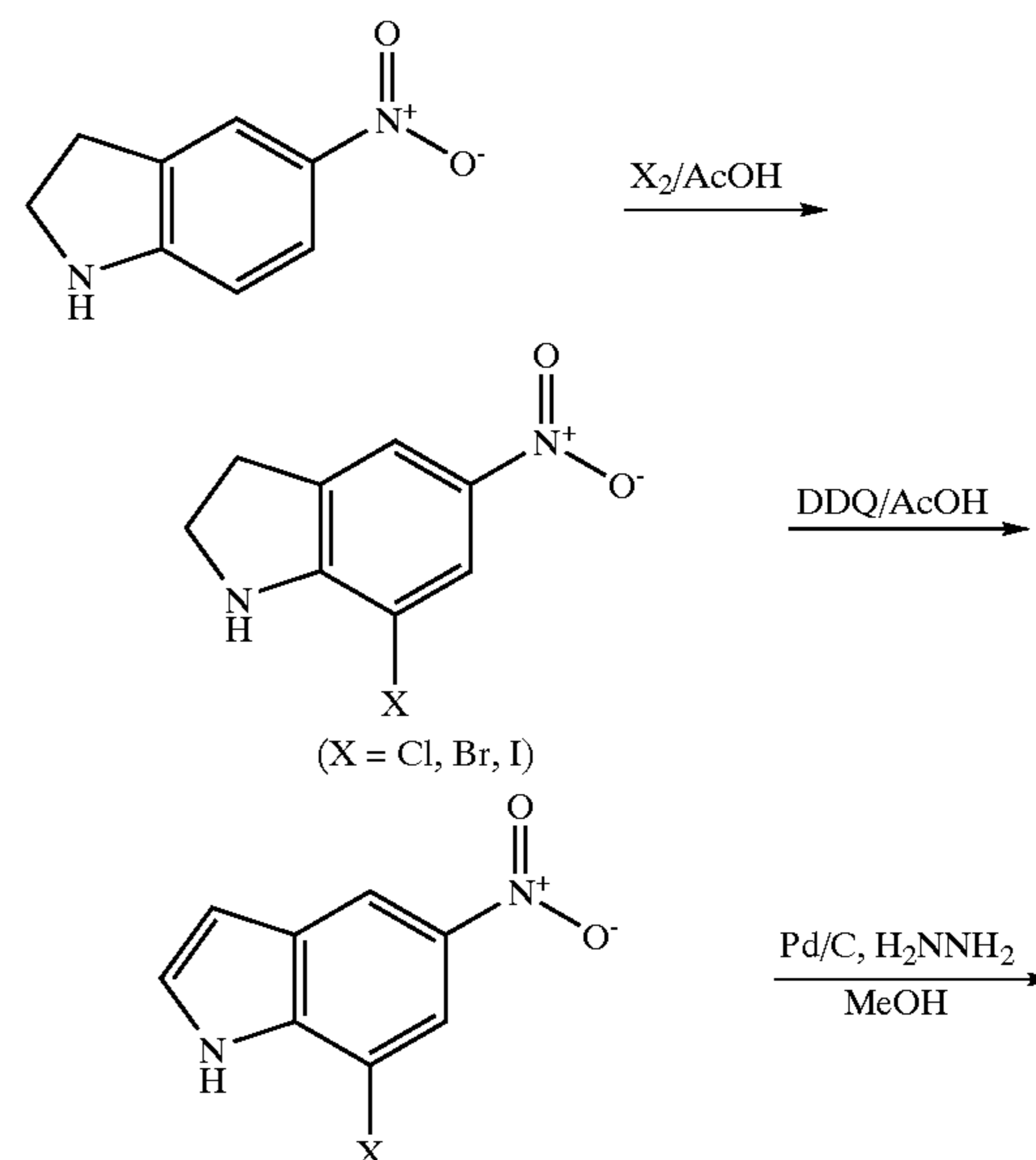
Scheme 1 illustrates schematically the synthesis of 7-substituted derivatives of 5-(2-imidazolin-2ylamino) indole
