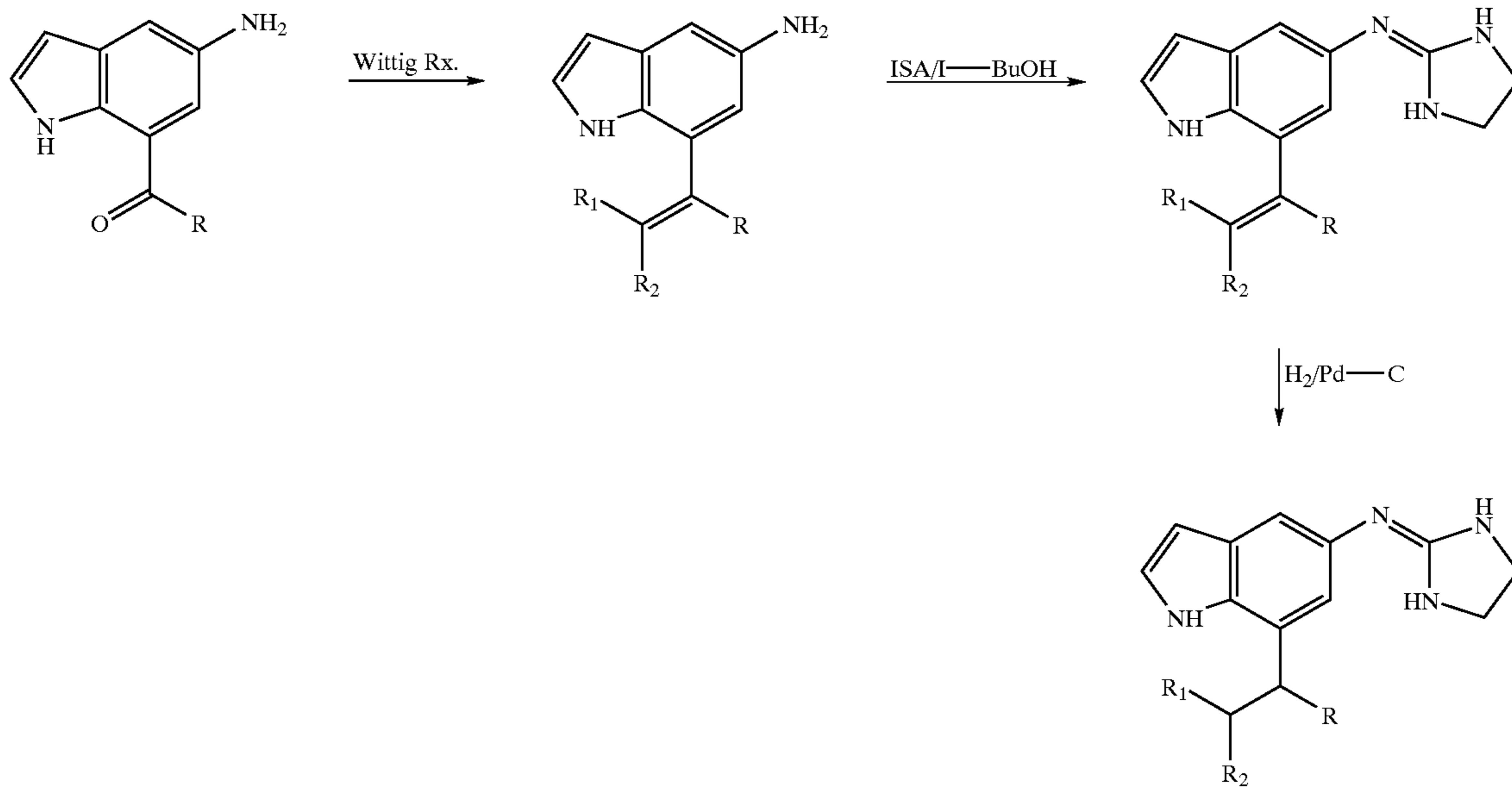
Scheme 3 illustrates schematically the synthesis of 7-substituted branched alkyl/alkenyl derivatives of 5-(2-imidazolin-2ylamino) indole where R_x , R_1 and R_2 are alkyl or alkenyl groups
