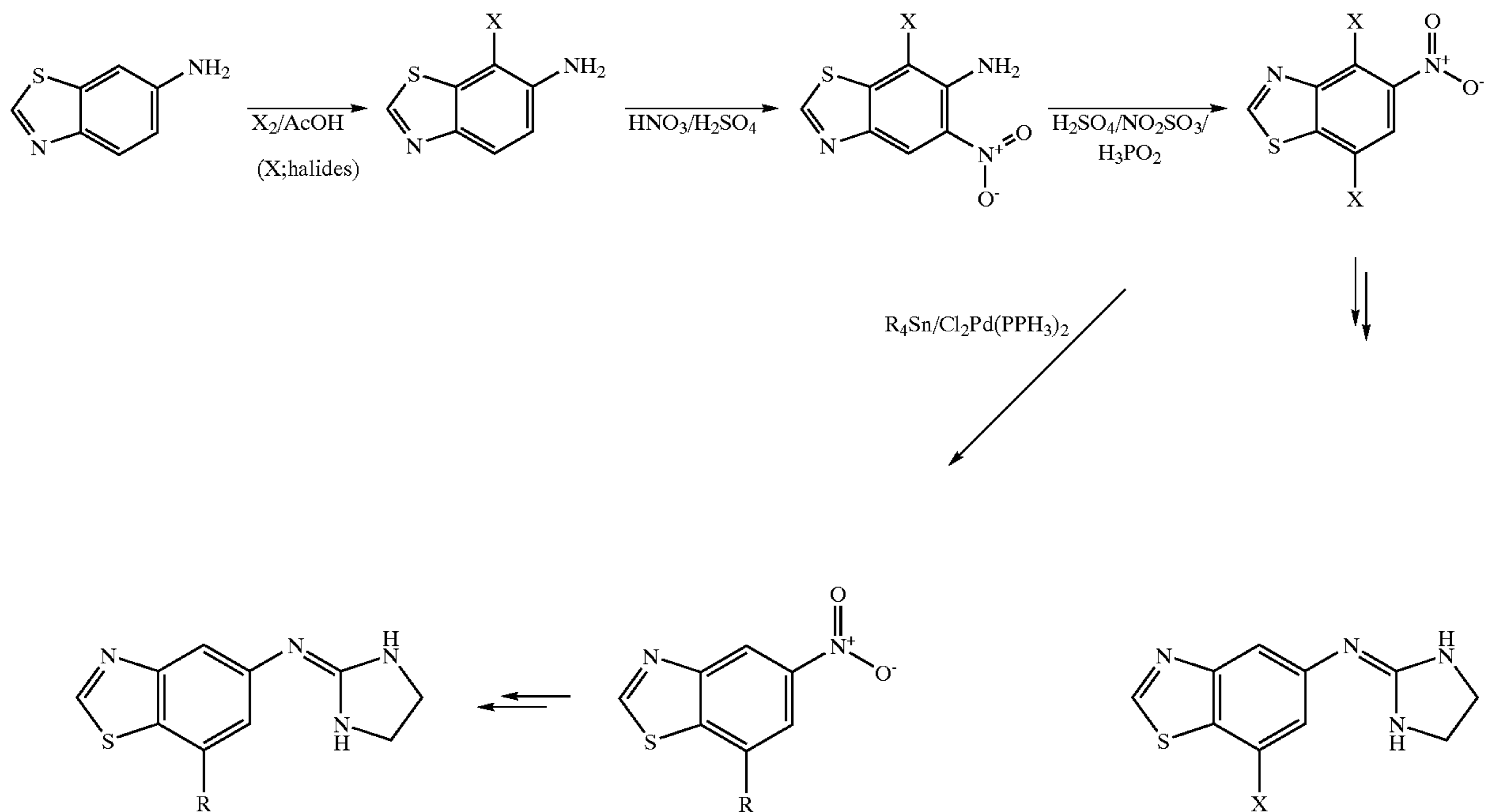
Scheme 5 illustrates schematically the synthesis of 7-substituted derivatives of 5-(2-imidazolin-2ylamino) benzothiazole where R is alkyl or alkenyl
