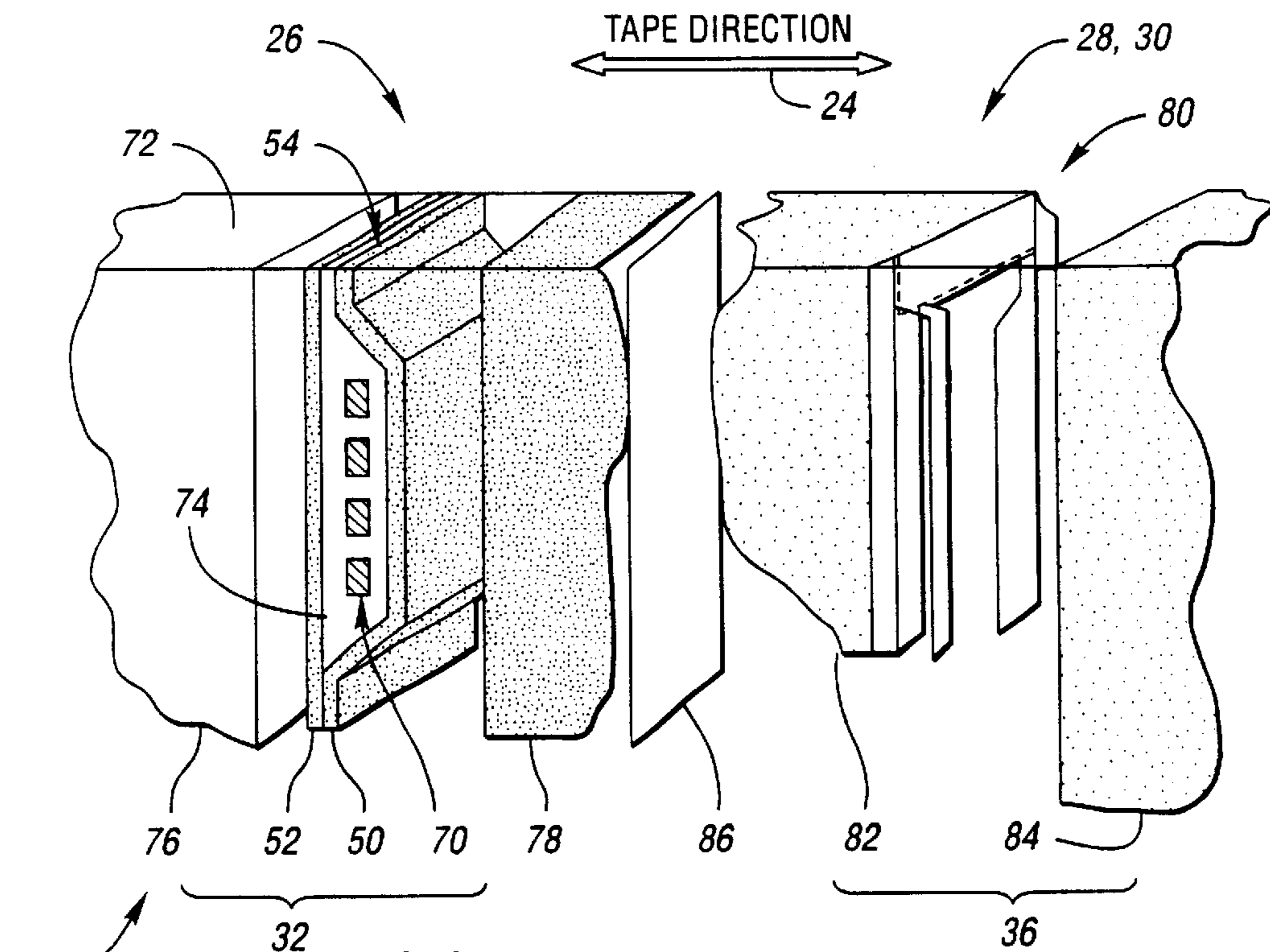
Fig. 3 (PRIOR ART)
