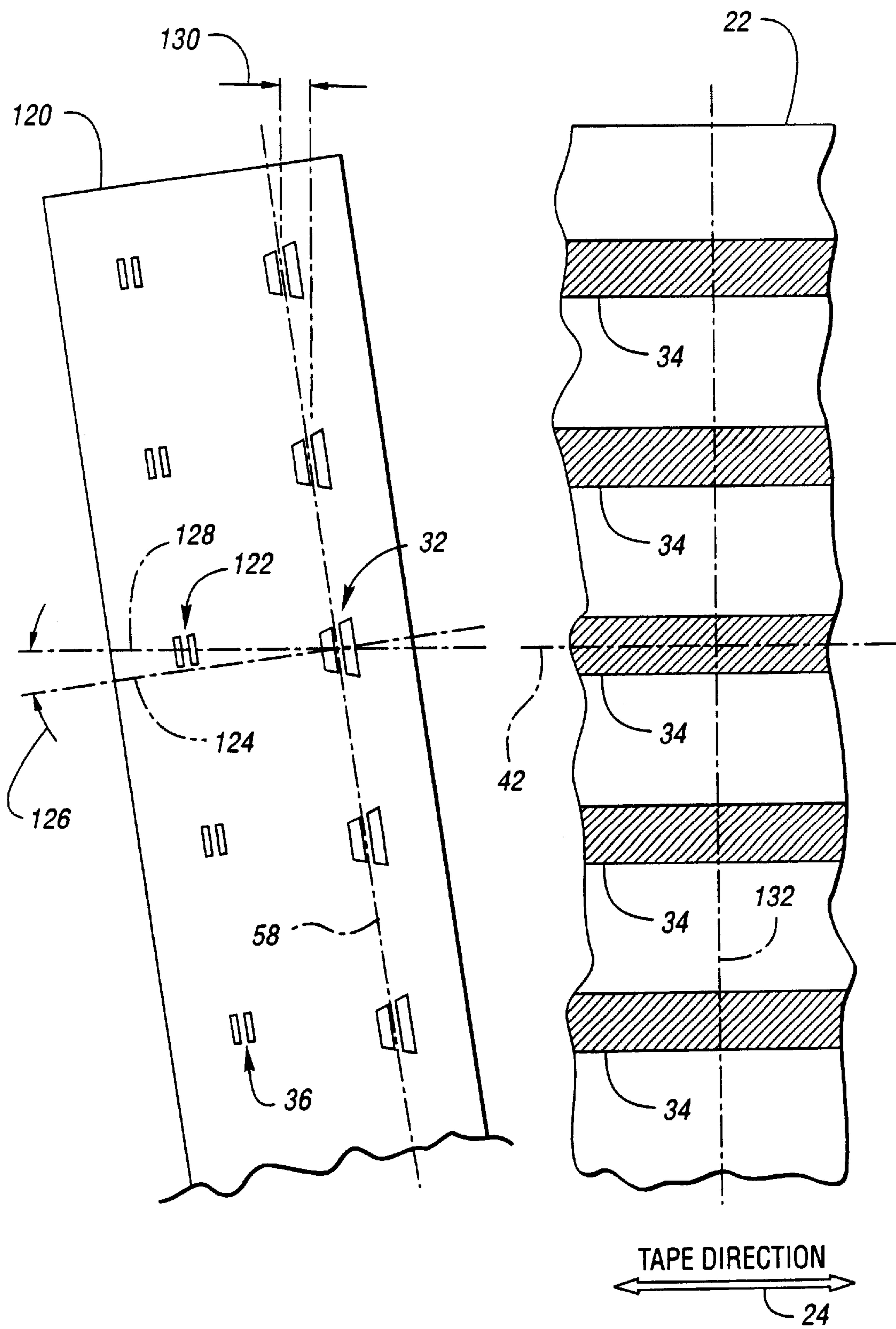
Fig. 6 (PRIOR ART)
