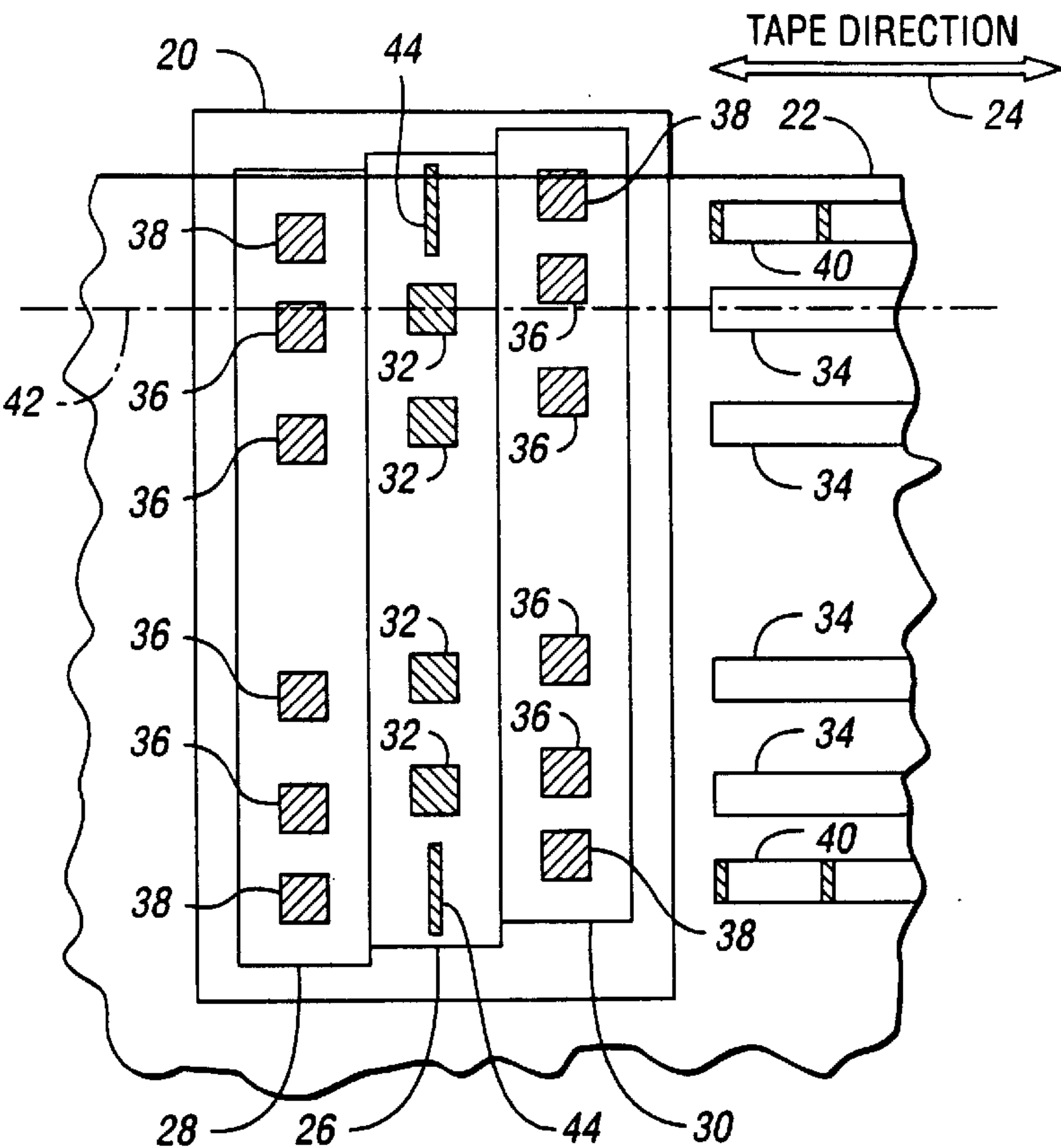
Fig. 1 (PRIOR ART)
