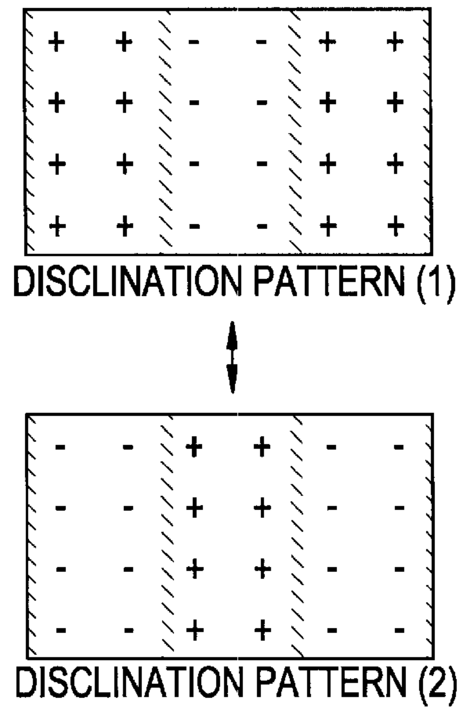
FIG. 17B POLARITY PATTERN OF RESPECTIVE PIXELS IN SOURCE LINE (2 LINES SIMULTANEOUS) INVERSION DRIVING
