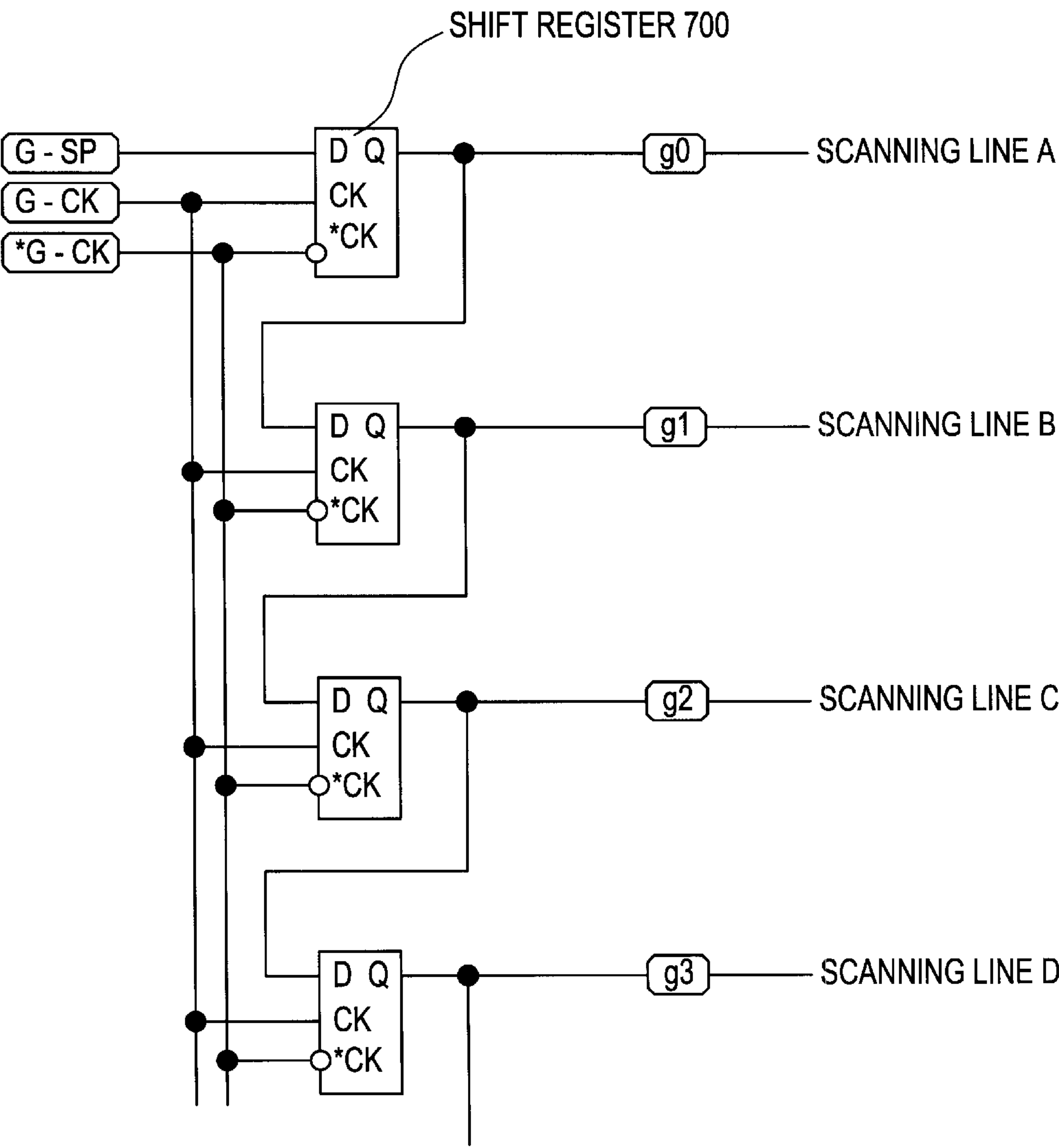
BRIEF VIEW OF PERIPHERY OF GATE DRIVER CIRCUIT
