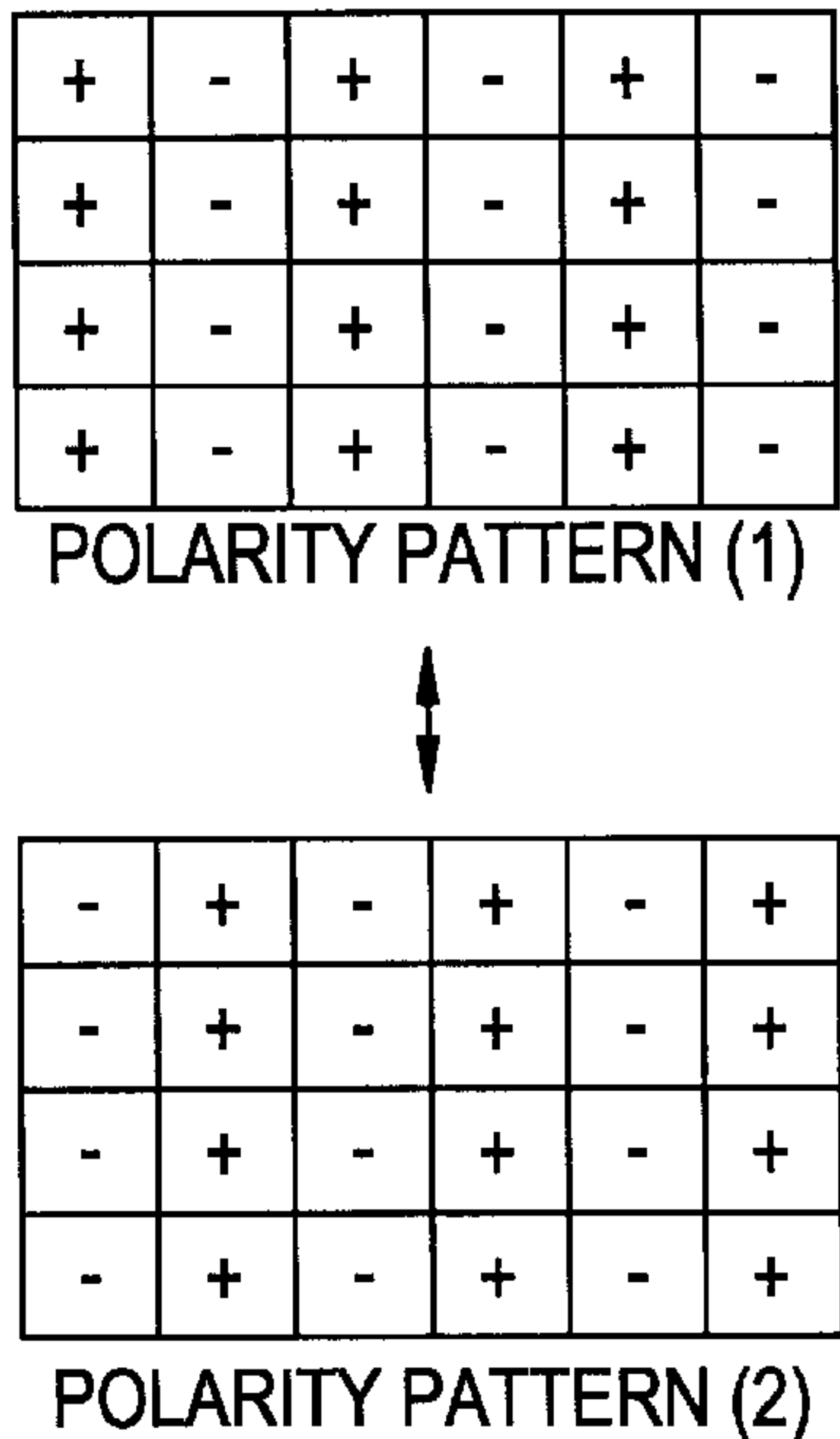
FIG. 17A POLARITY PATTERN OF RESPECTIVE PIXELS IN SOURCE LINE (2 LINES SIMULTANEOUS) INVERSION DRIVING
