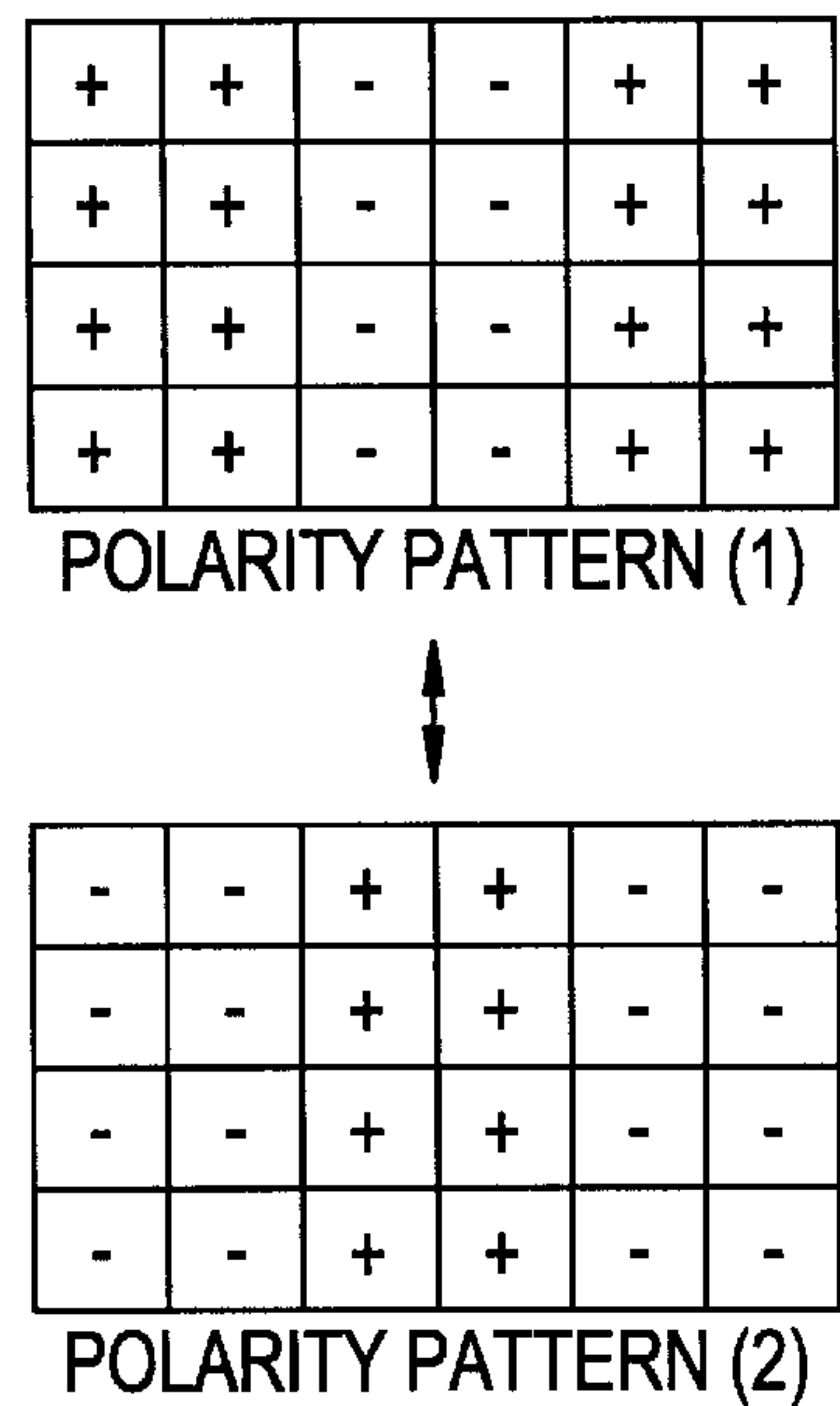
FIG. 17A POLARITY PATTERN OF RESPECTIVE PIXELS IN SOURCE LINE (2 LINES SIMULTANEOUS) INVERSION DRIVING
