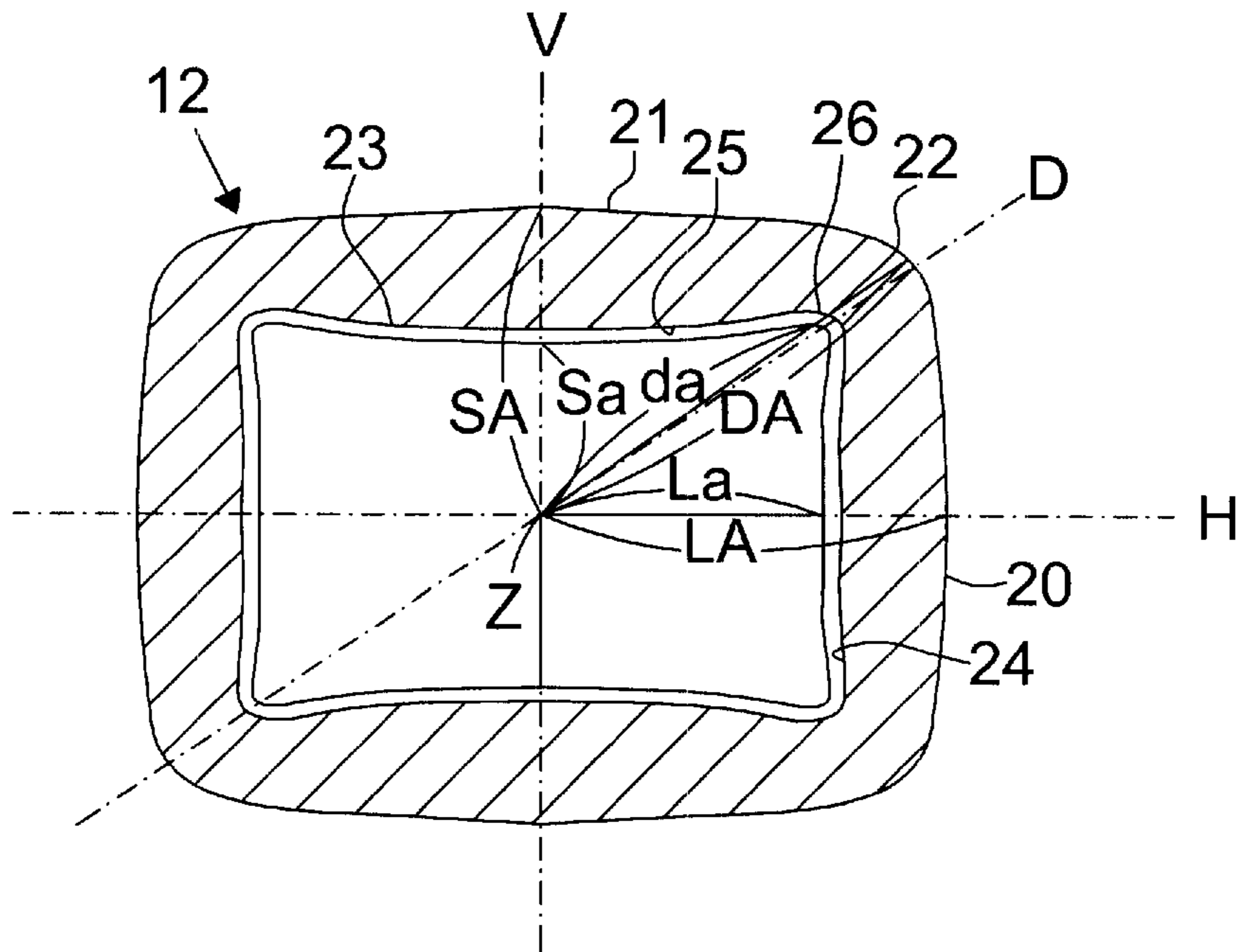
PRIOR ART
