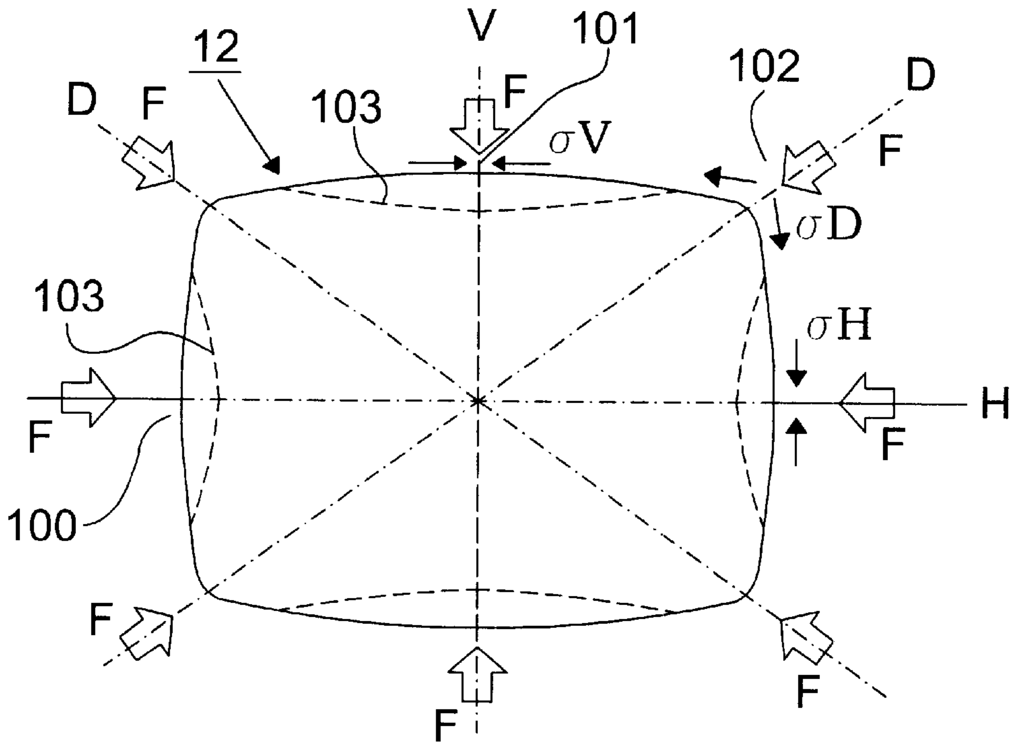
PRIOR ART
