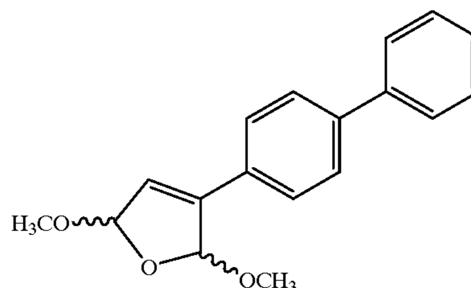
3-(Biphenyl-4-yl)-2,5-dihydro-2,5-dimethoxyfuran
