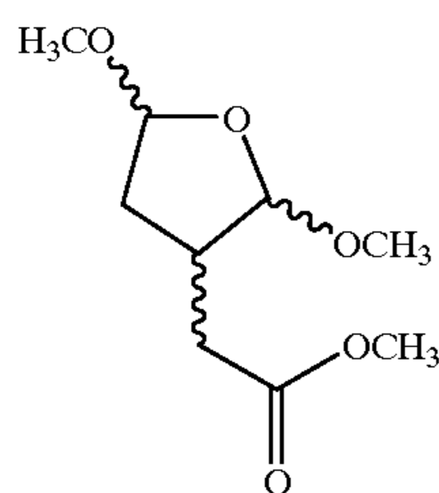
Methyl 2-(2,5-Dimethoxy-tetrahydrofuran-3-yl)-acetate
