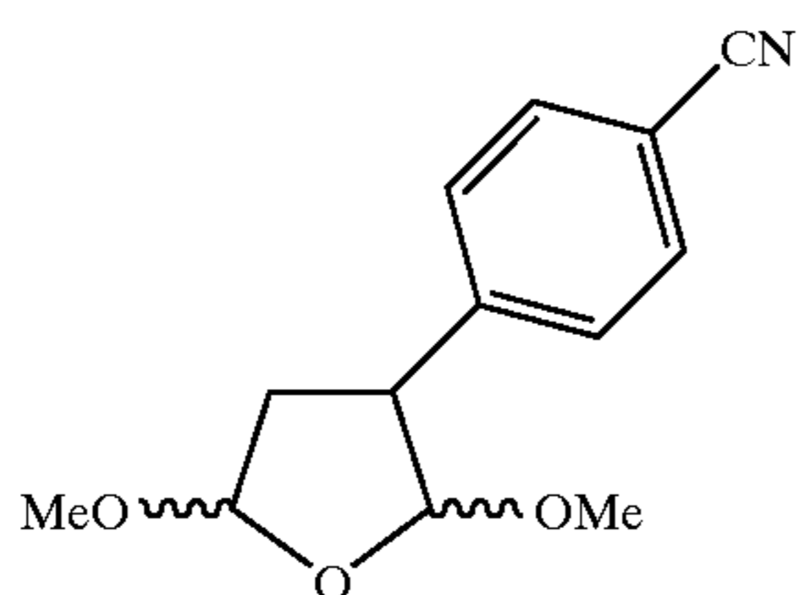
3-(4-Cyanophenyl)-2,5-dimethoxy-tetrahydrofuran
