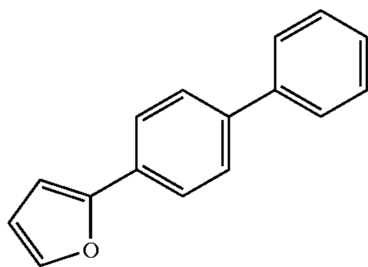
2-Biphenyl-4-yl-furan
