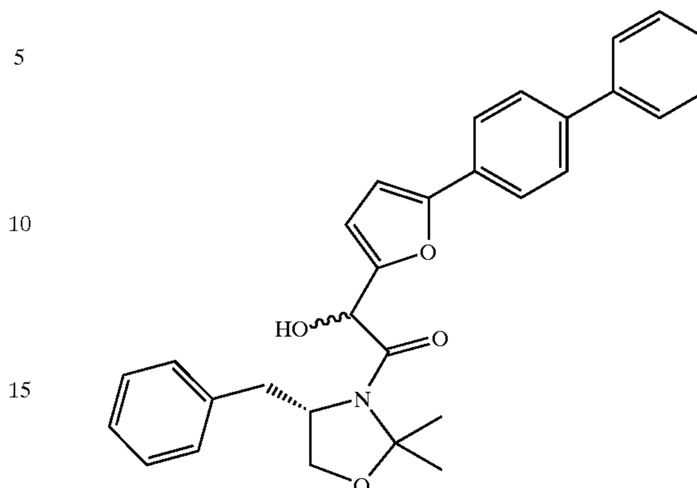
1-(4(S)-Benzyl-2,2-dimethyl-oxazolidin-3-yl)-2-(2-biphenyl-4-yl-furan-5-yl)-2-hydroxy-ethanone
