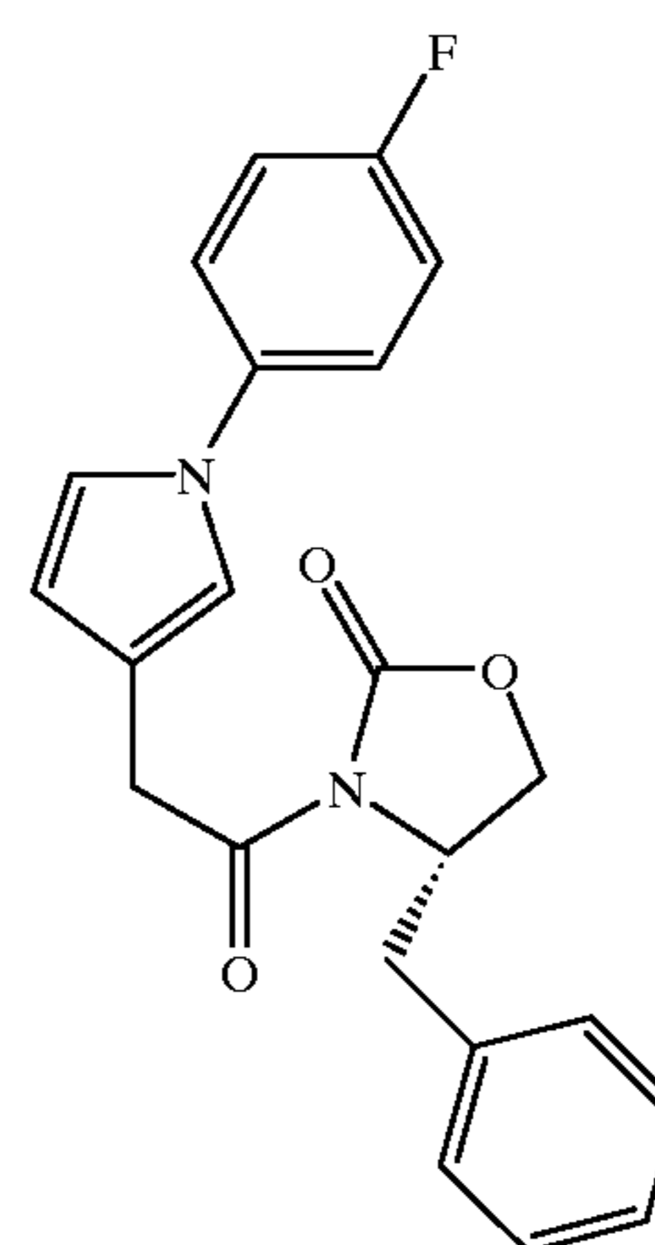
1-(4(S)-Benzyl-oxazolidin-2-on-3-yl)-2-[1-(4-fluorophenyl)-1H-pyrrol-3-yl]-ethanone
