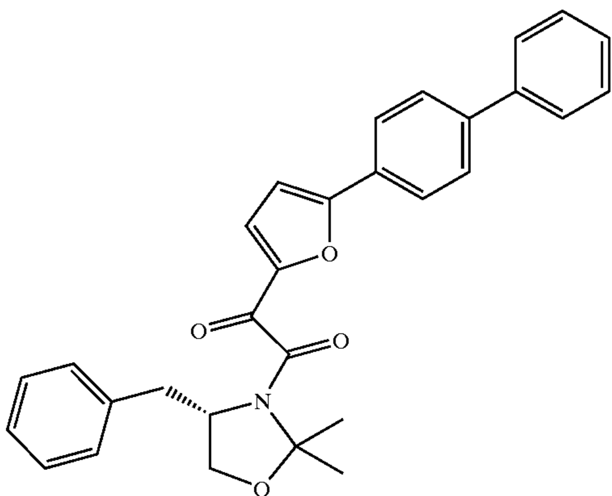
1-(4(S)-Benzyl-2,2-dimethyl-oxazolidin-3-yl)-2-(2-biphenyl-4-yl-furan-5-yl)ethane-1,2-dione
