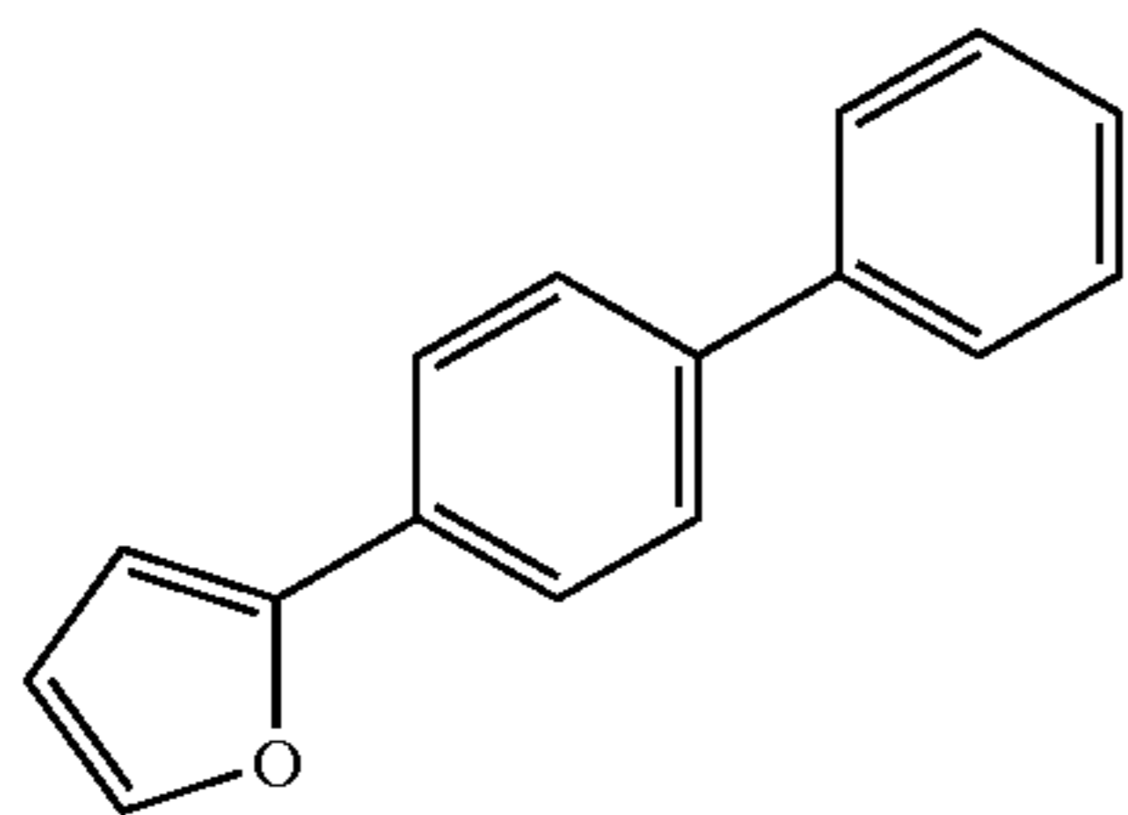
2-Biphenyl-4-yl-furan
