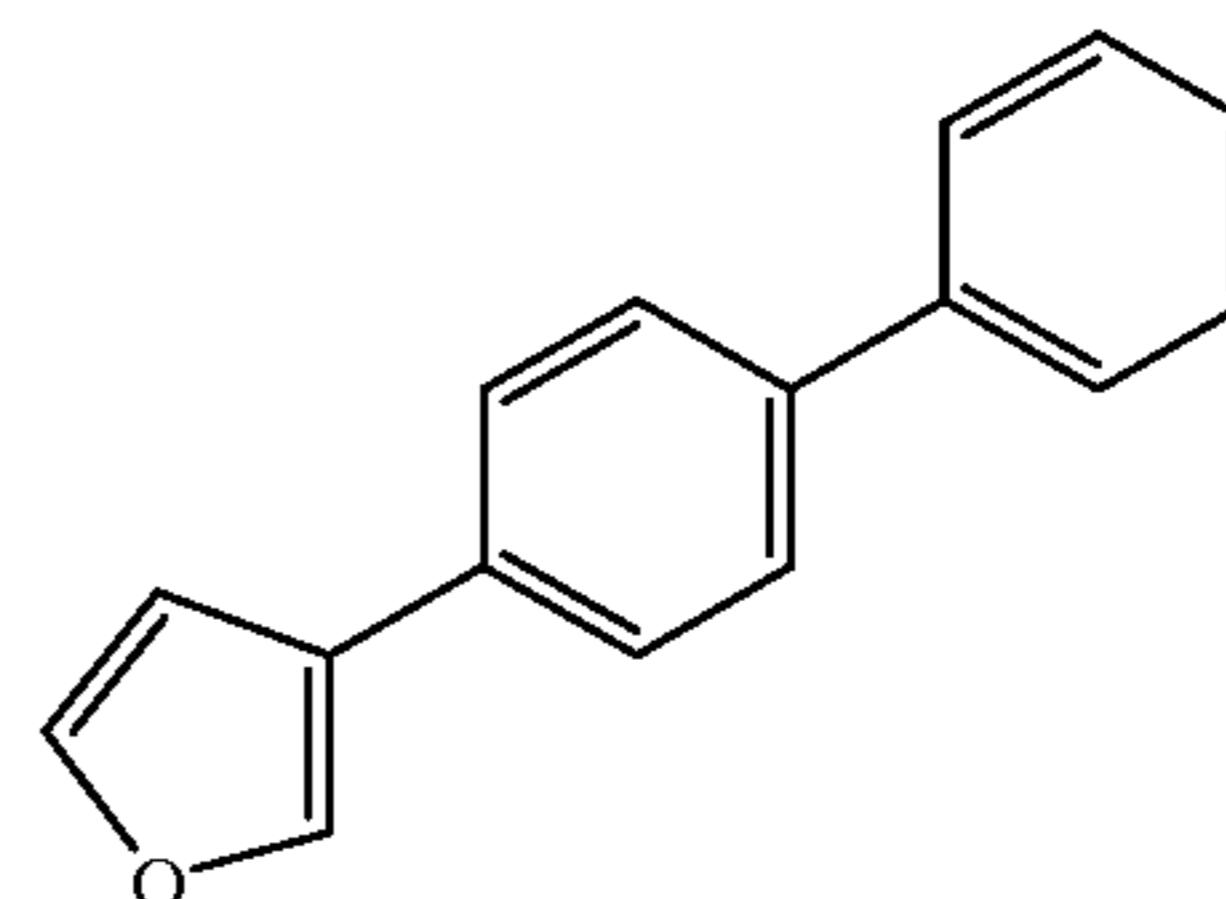
3-(Biphenyl-4-yl)furan
