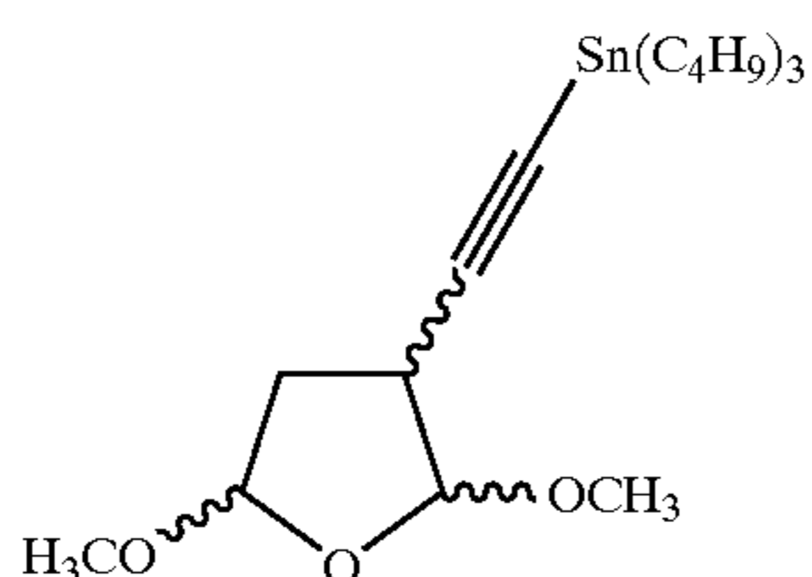
2,5-Dimethoxy-3-(2-tributylstannylethynyl)-tetrahydrofuran
