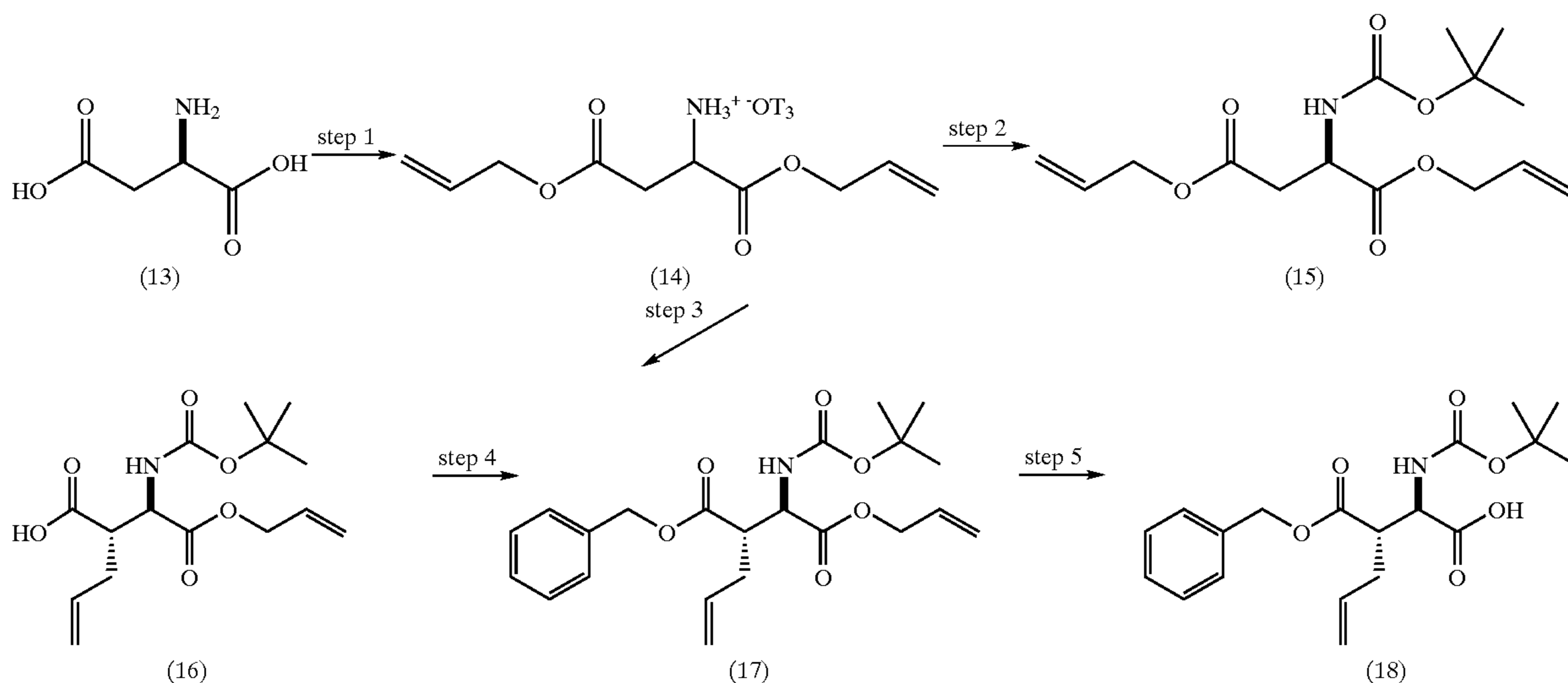
REACTION SCHEME VII
