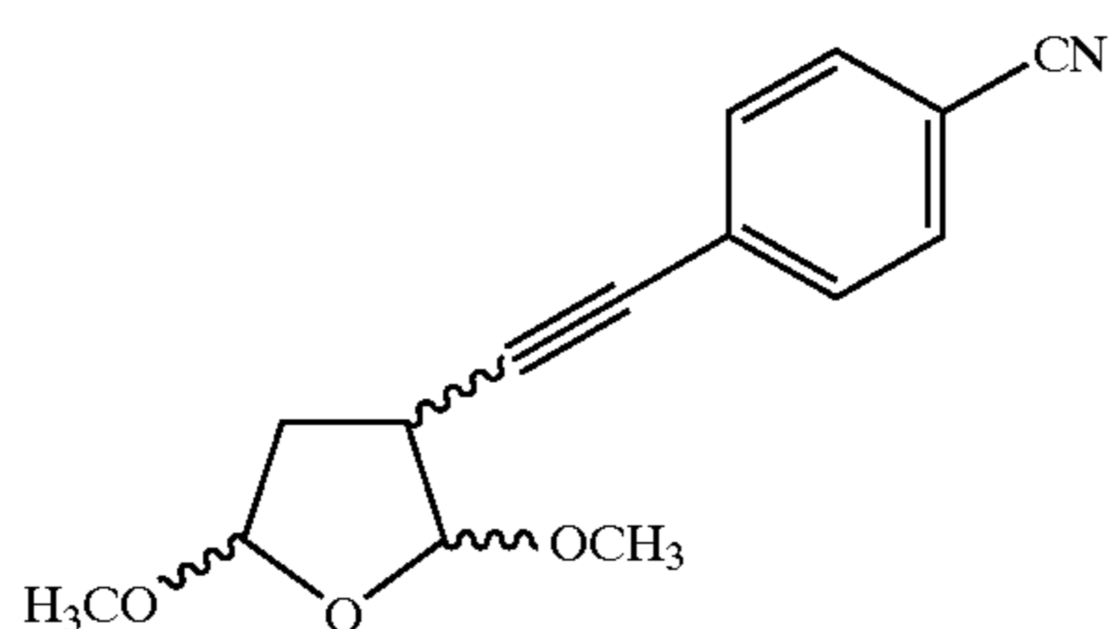
3-[2-(4-Cyanophenyl)-ethynyl]-2,5-dimethoxy-tetrahydrofuran
