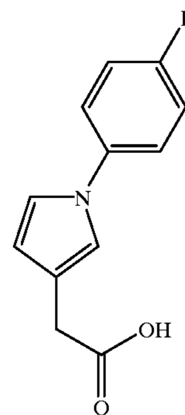
2-[1-(4-Fluorophenyl)-1H-pyrrol-3-yl]-acetic Acid
