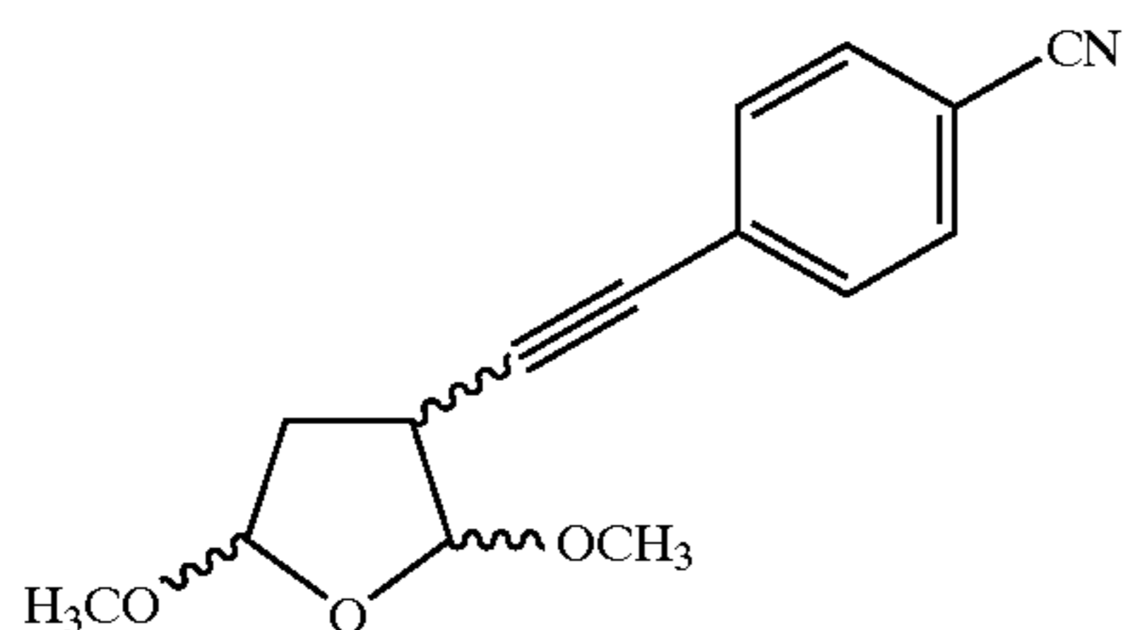
3-[2-(4-Cyanophenyl)-ethynyl]-2,5-dimethoxy-tetrahydrofuran
