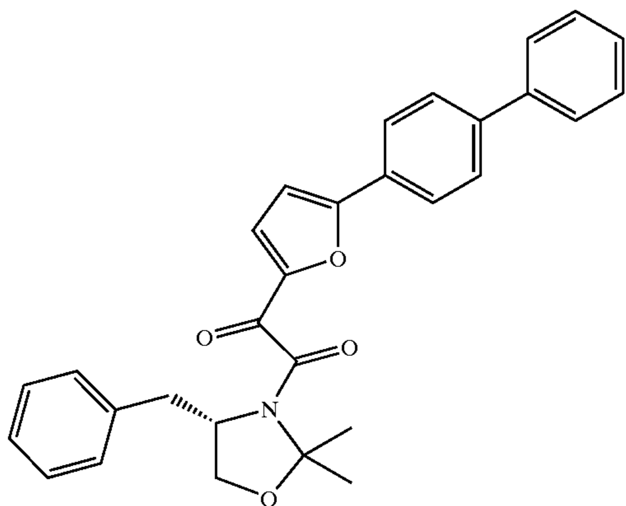
1-(4(S)-Benzyl-2,2-dimethyl-oxazolidin-3-yl)-2-(2-biphenyl-4-yl-furan-5-yl)ethane-1,2-dione
