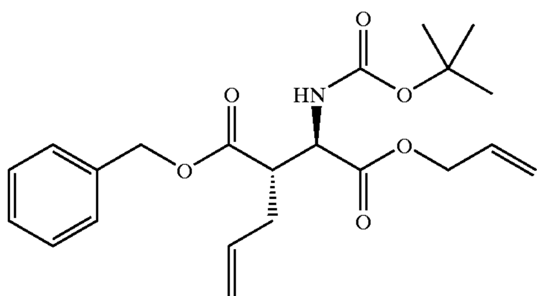
\alpha -Allyl, \beta -Benzyl 3(R)-Allyl-t-butoxycarbonyl-D-aspartate
