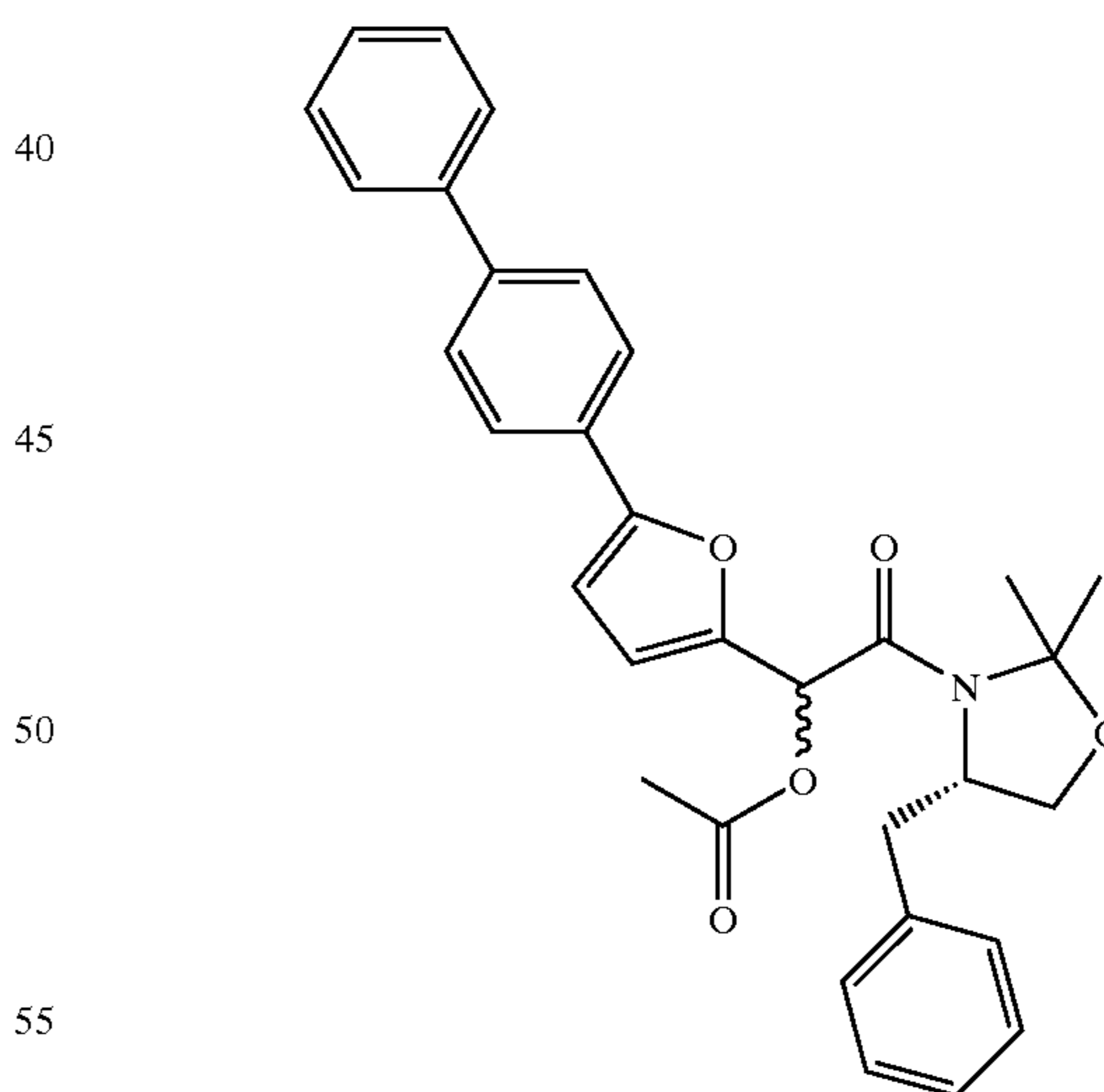
2-Acetoxy-1-(4(S)-benzyl-2,2-dimethyl-oxazolidin-3-yl)-2-(2-biphenyl-4-yl-furan-5-yl)-ethanone
