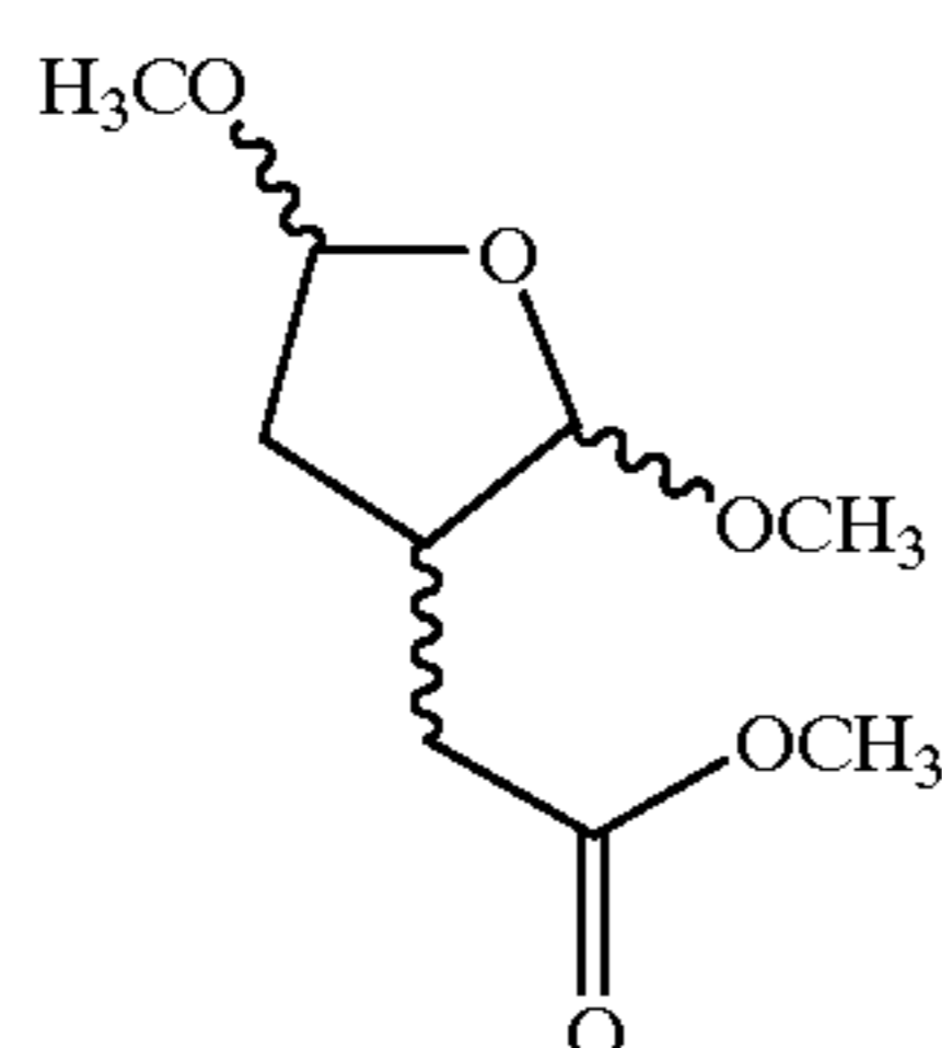
Methyl 2-(2,5-Dimethoxy-tetrahydrofuran-3-yl)-acetate
