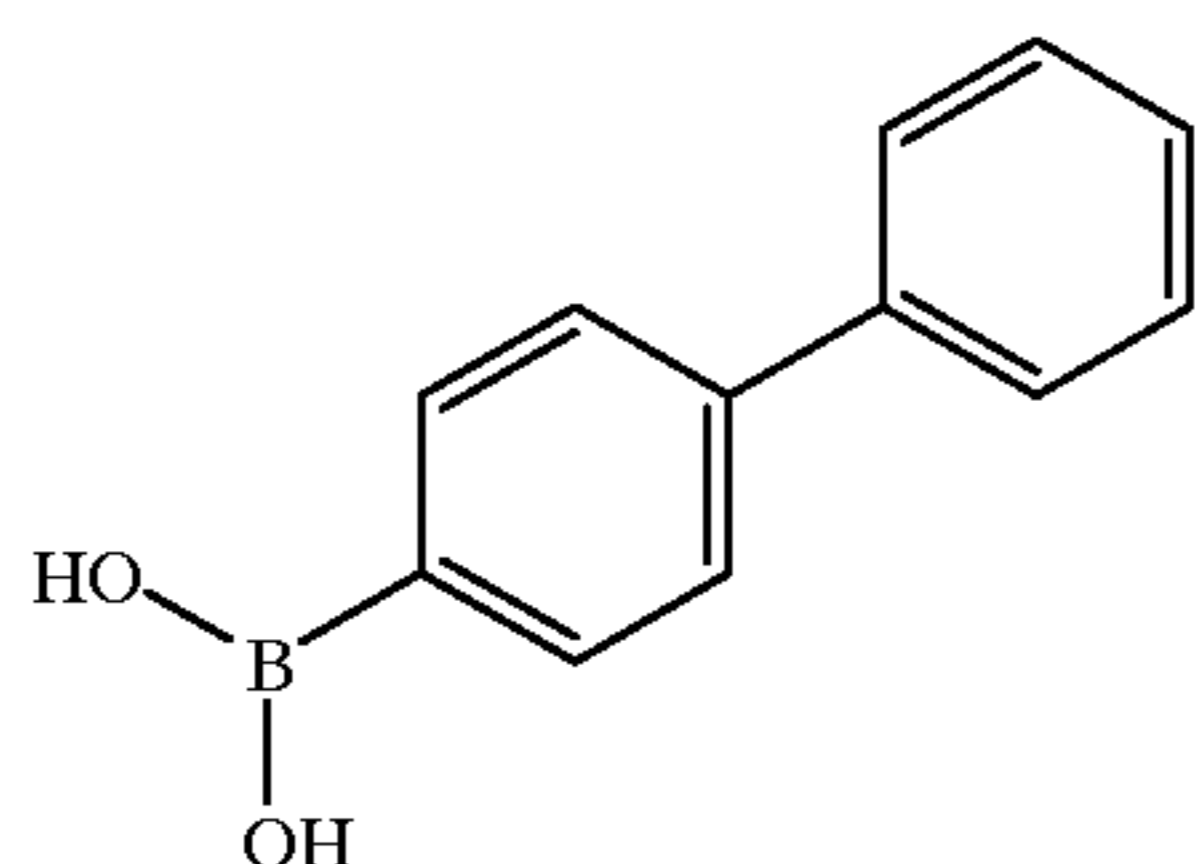
4-Biphenylboronic Acid
