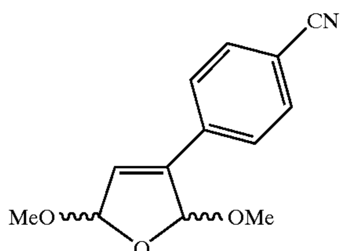
3-(4-Cyanophenyl)-2,5-dihydro-2,5-dimethoxyfuran
