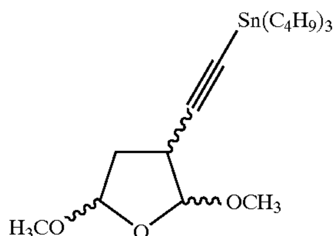
2,5-Dimethoxy-3-(2-tributylstannylethynyl)-tetrahydrofuran
