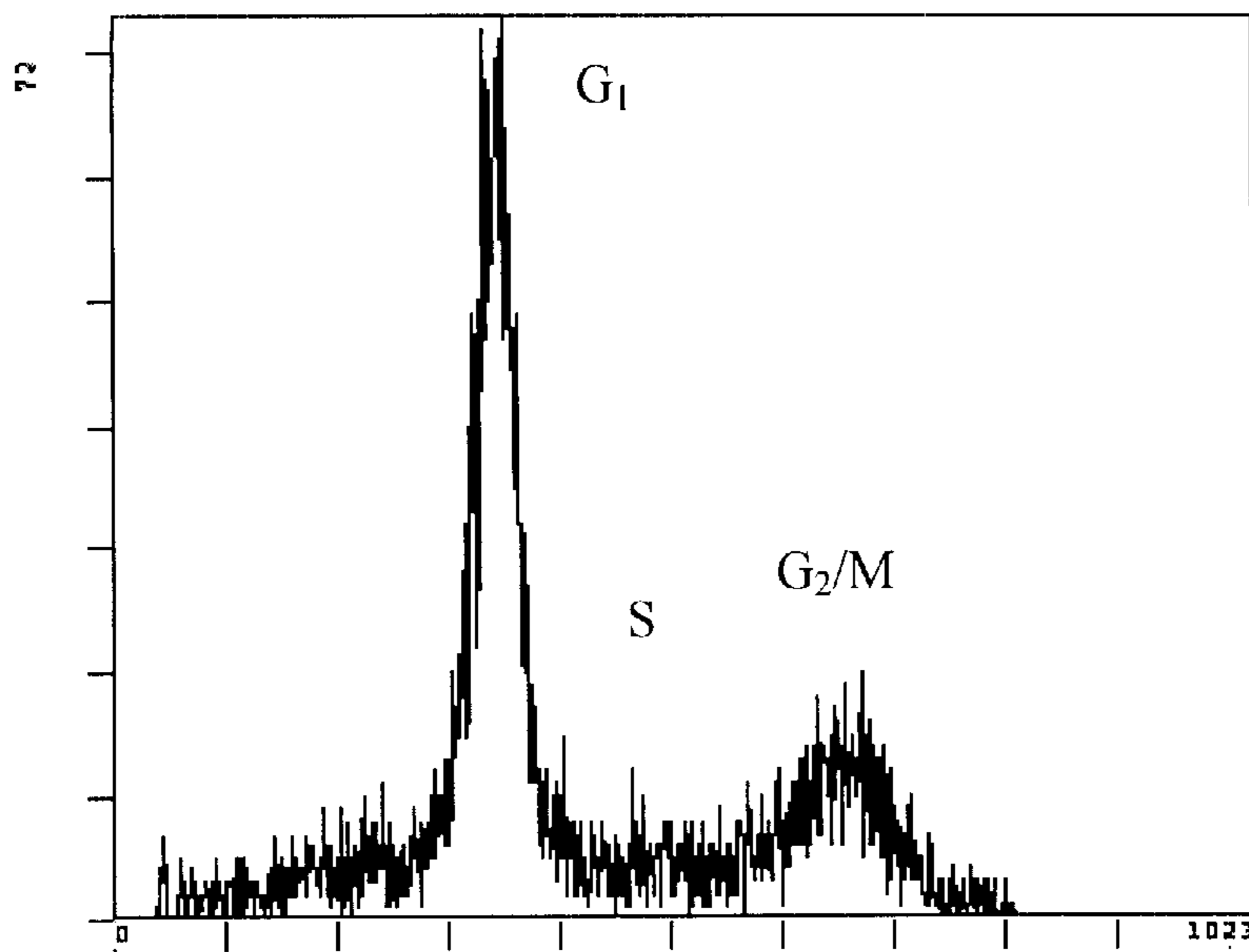
8,21,23-Hexahydro-discodermolide(100 nM)
