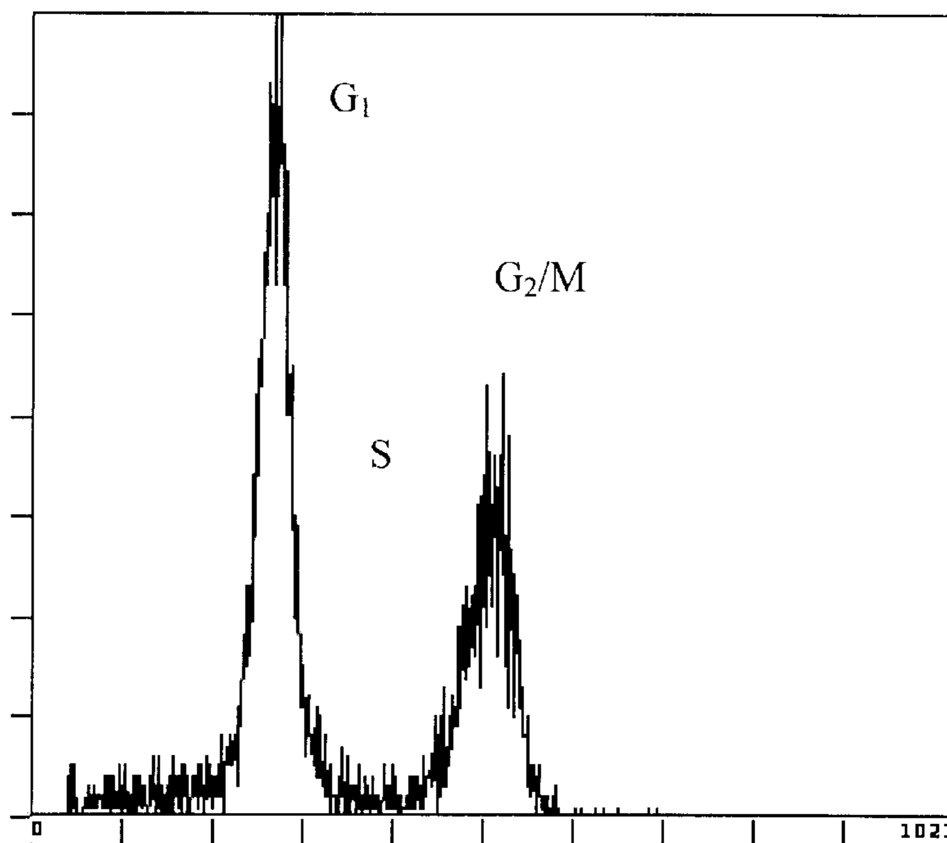
7-Deoxy-8,21,23 hexahydrodiscodermolide (1000 nM)
