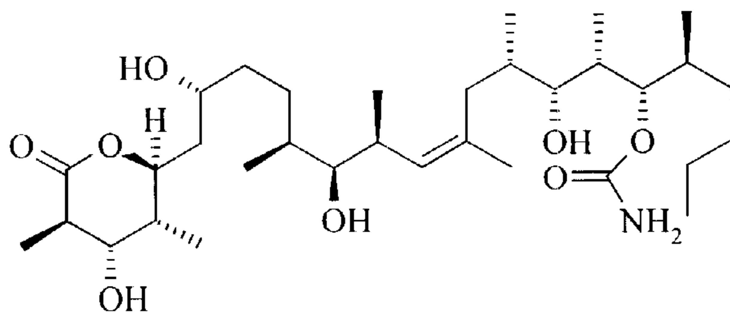
8,21,23-Hexahydrodiscodermolide (XII)
