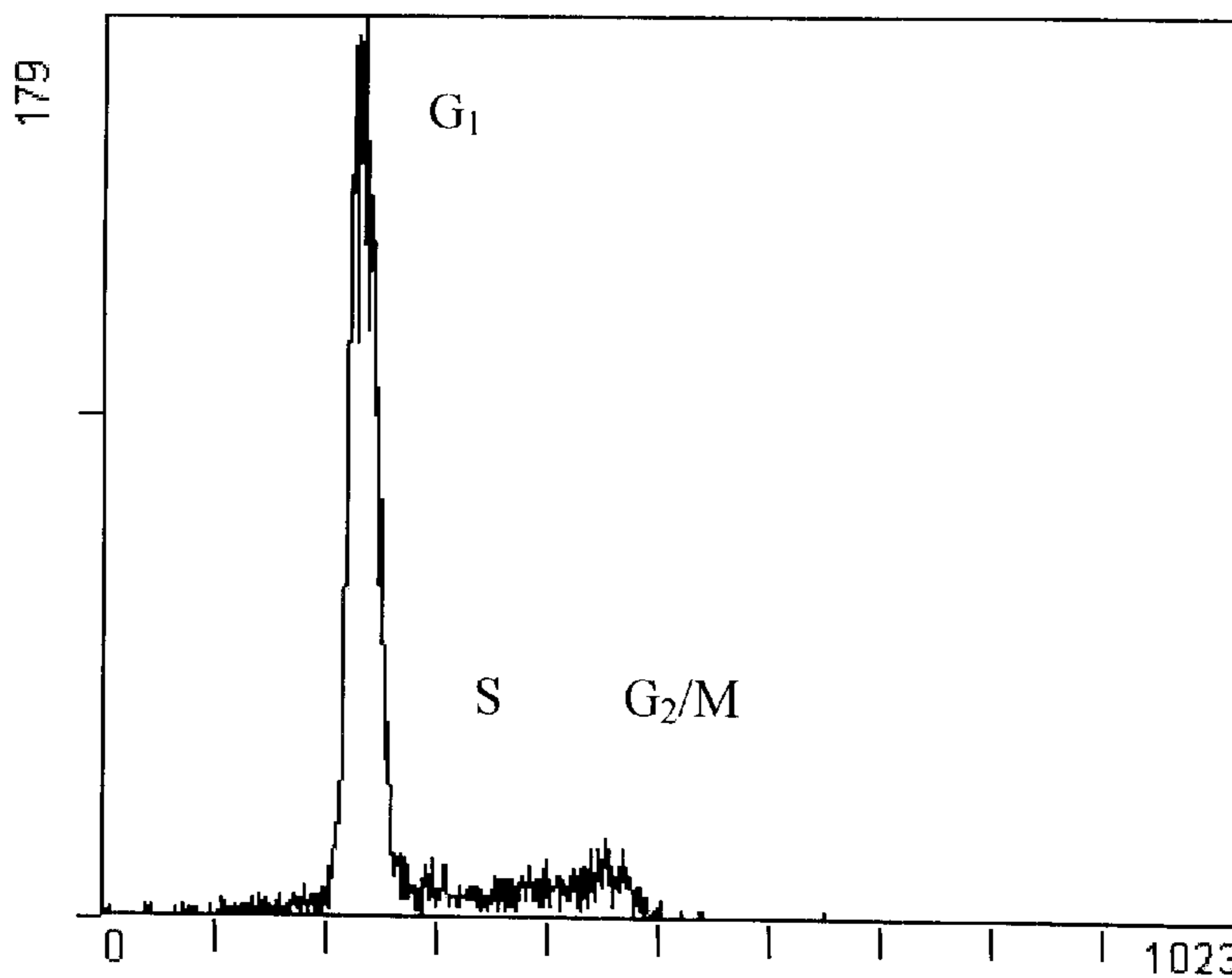
7-Deoxy-8,21,23-hexahydrodiscodermolide- 3,11,17-triacetate (1000 nM)
