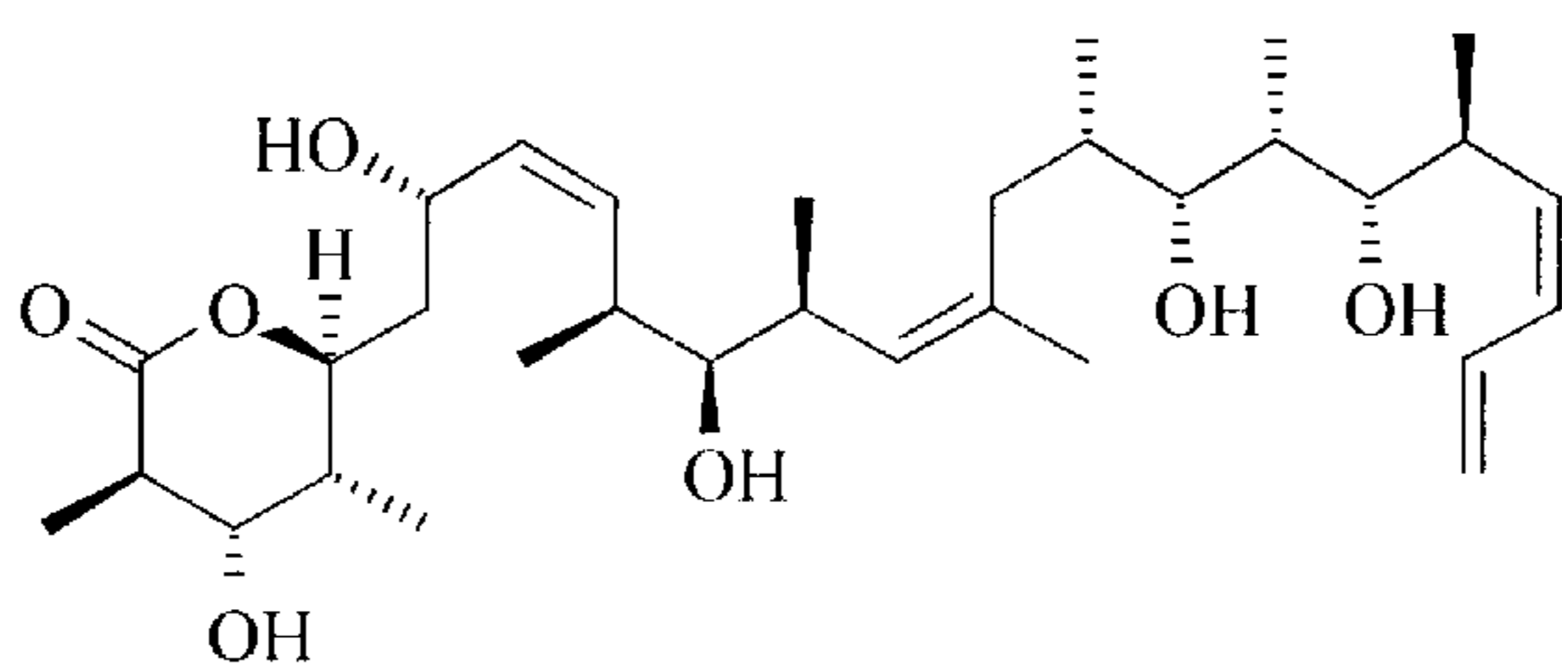
19-Desaminocarbonyldiscodermolide (III)
