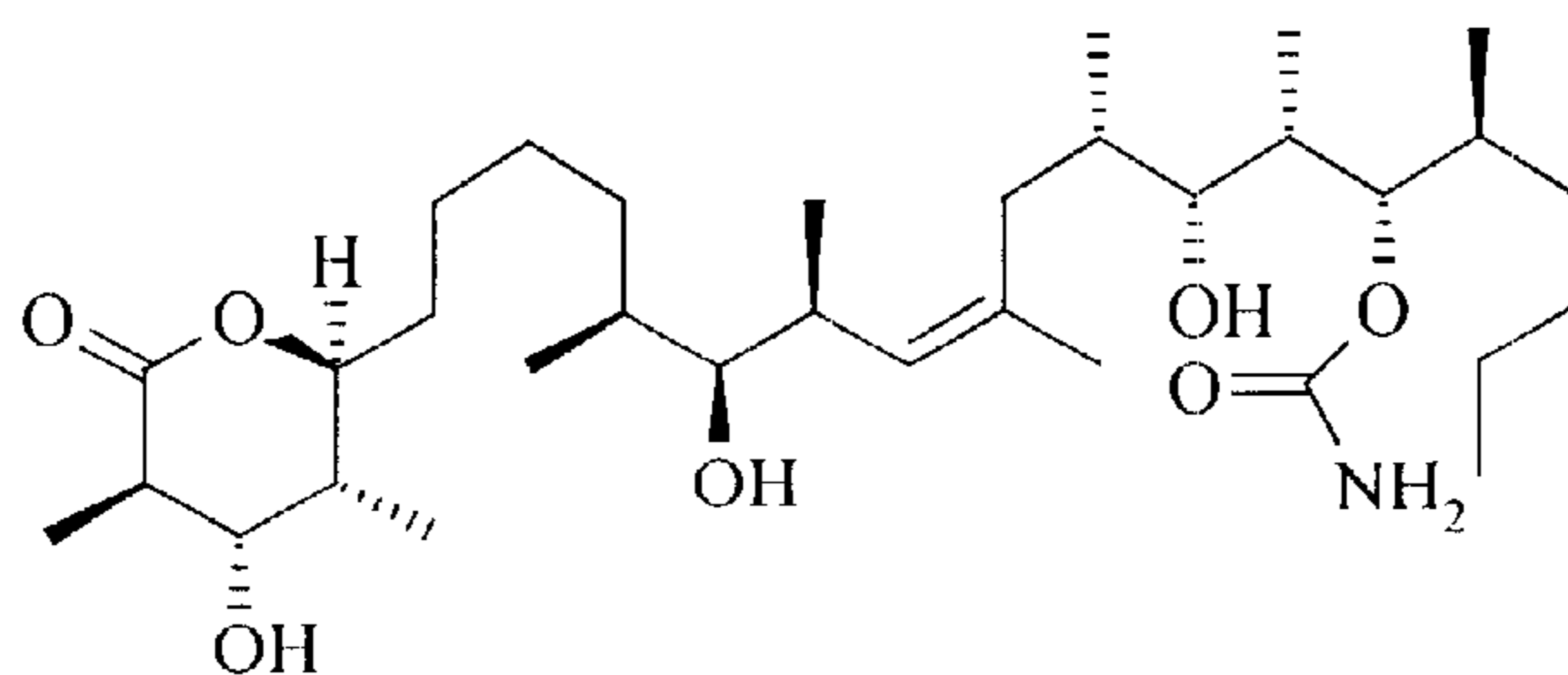
8,21,23-Hexahydrodiscodermolide (XII)
