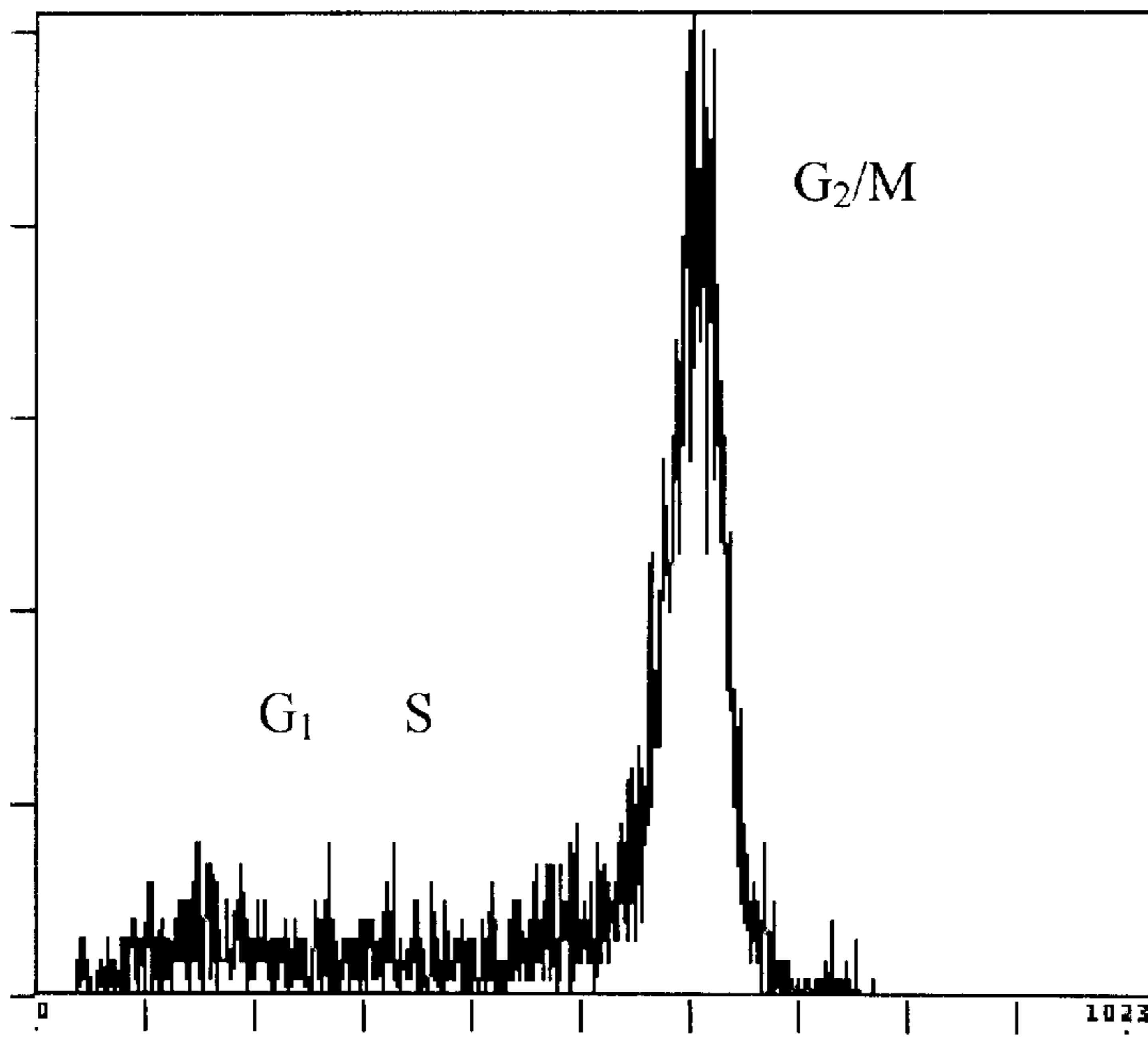
Discodermolide (100 nM)
