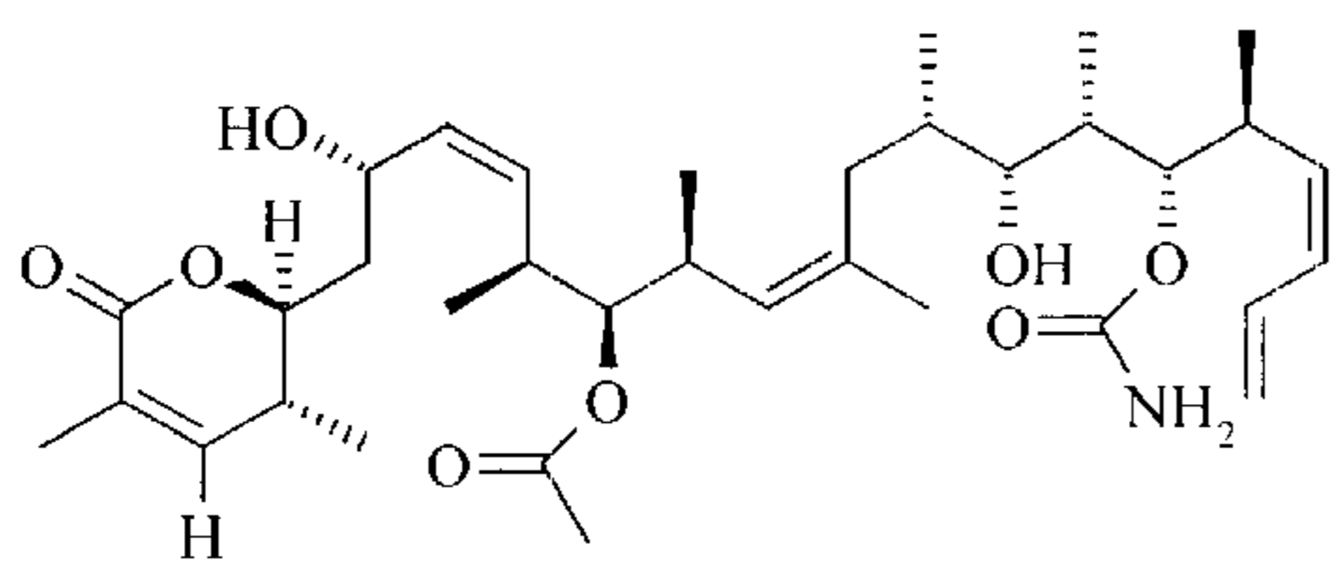
3-Deoxy-2 \Delta -discodermolide-11-acetate (X)
