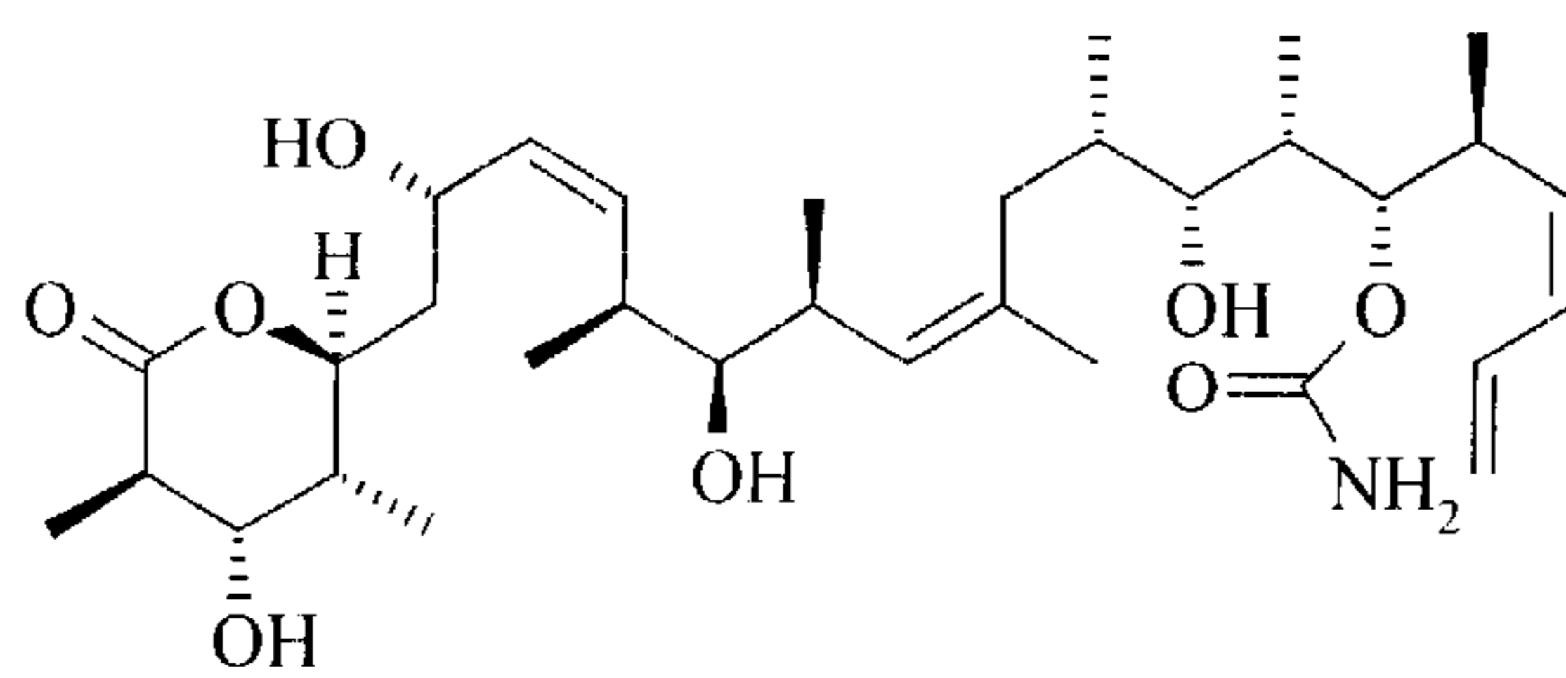
Discodermolide (I)
