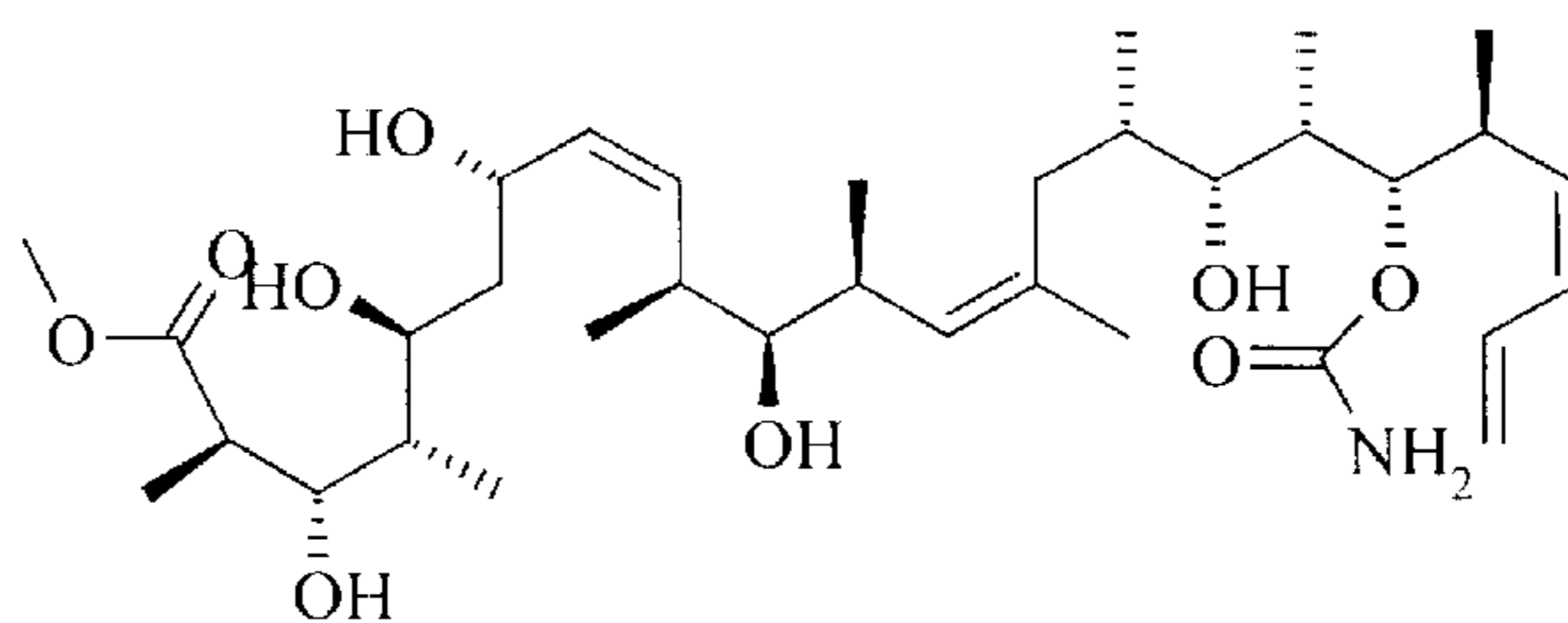
Methyldiscodermolate (V)
