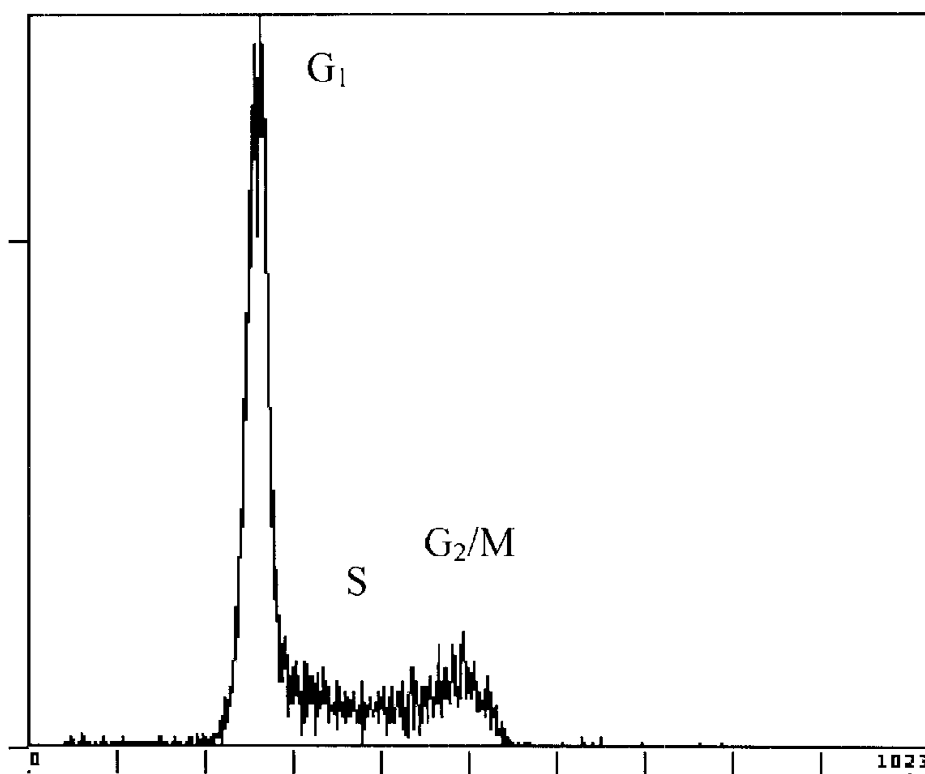
7-Deoxy-8,21,23-hexahydrodiscodermolide (100nM)
