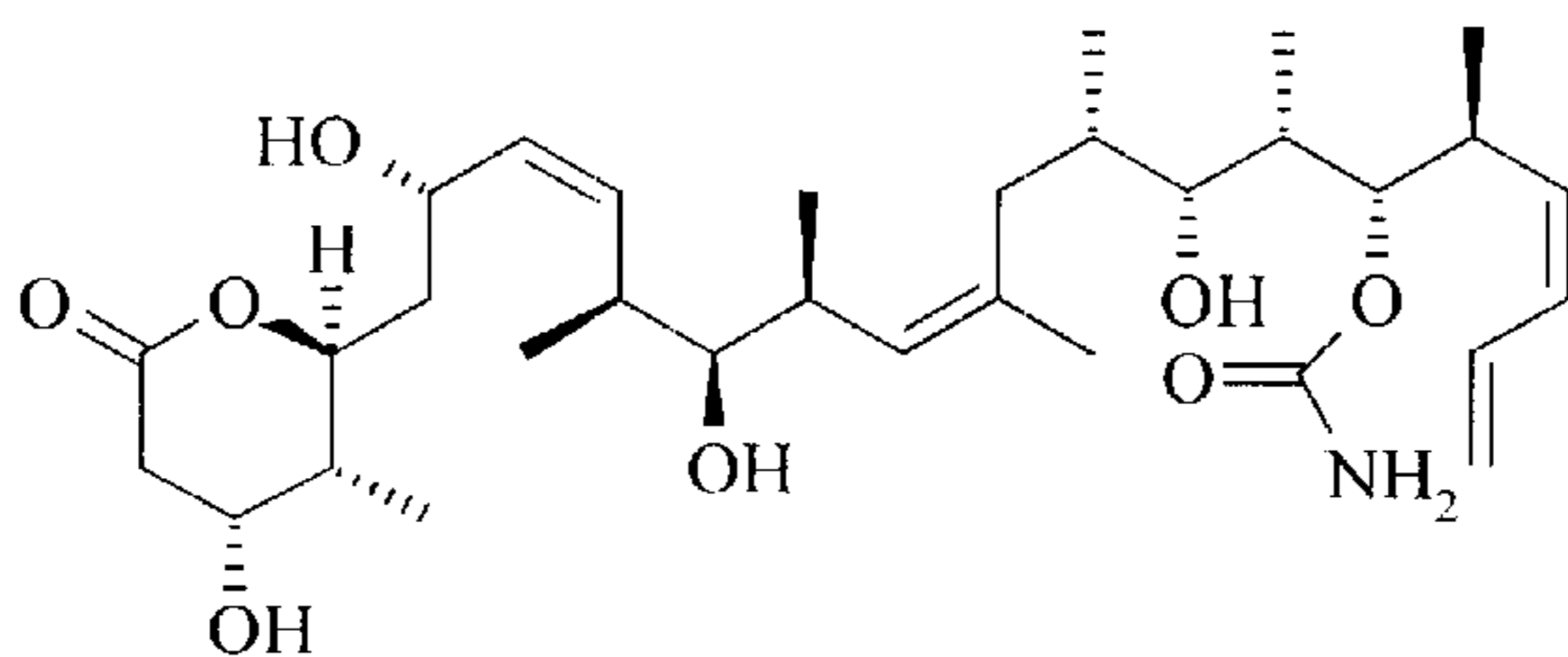
2-Desmethyldiscodermolide (II)
