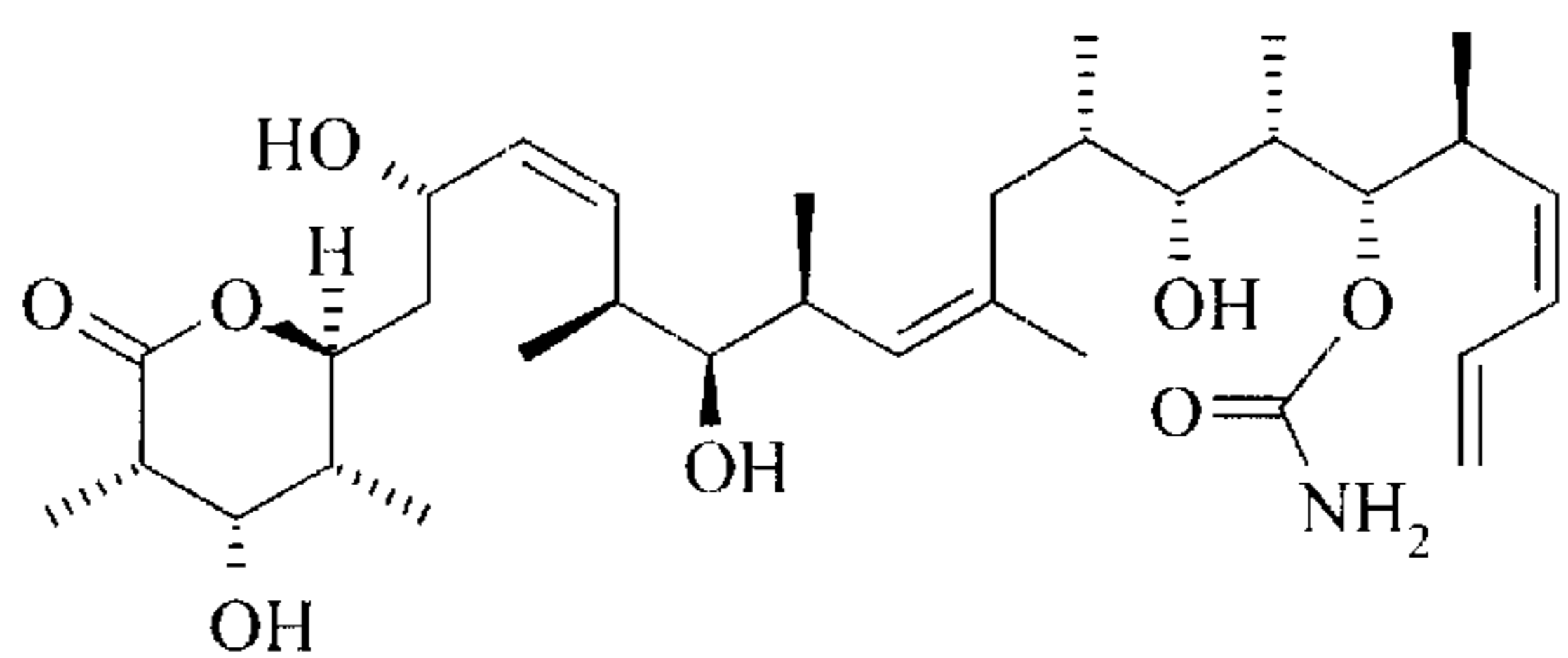
2-Epidiscodermolide (IV)
