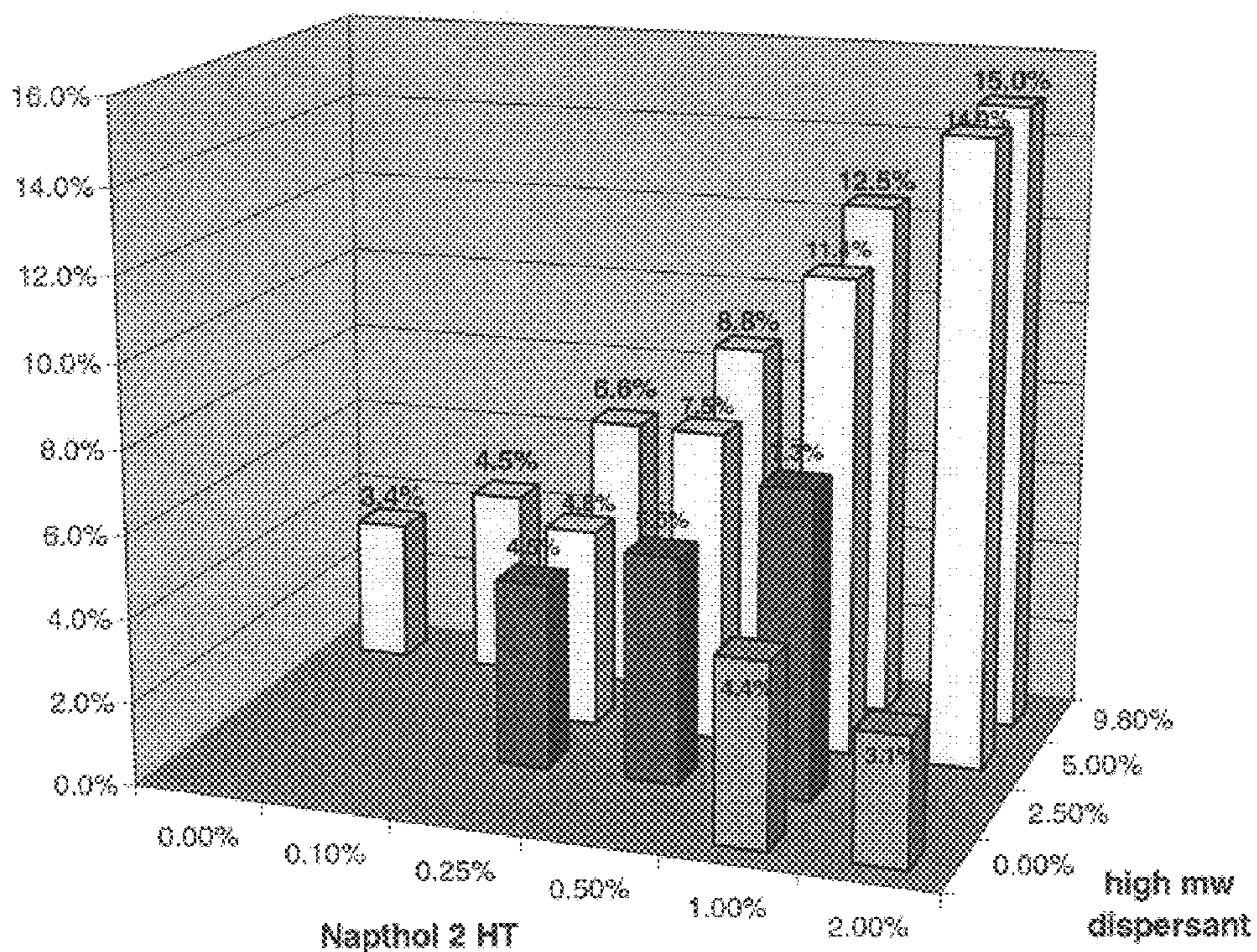
Percent Carbon Black to 200 cSt
