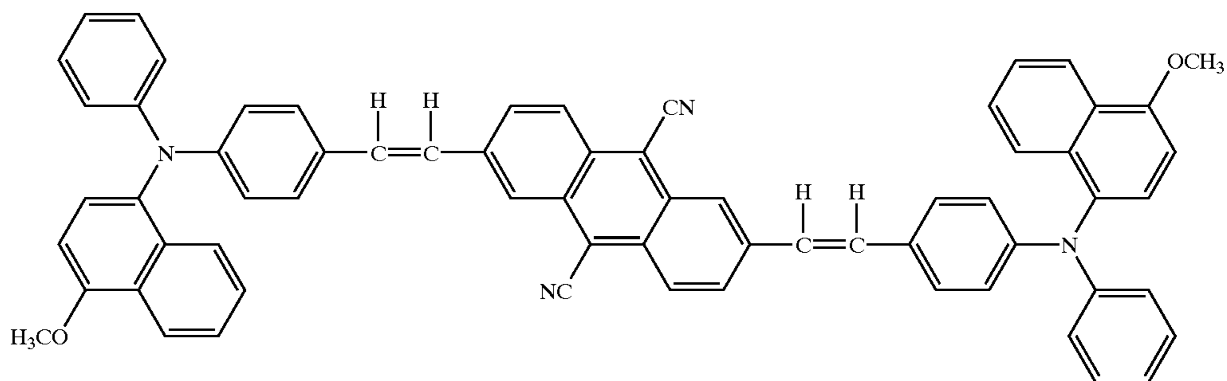
Structural Formula (7)-2:
