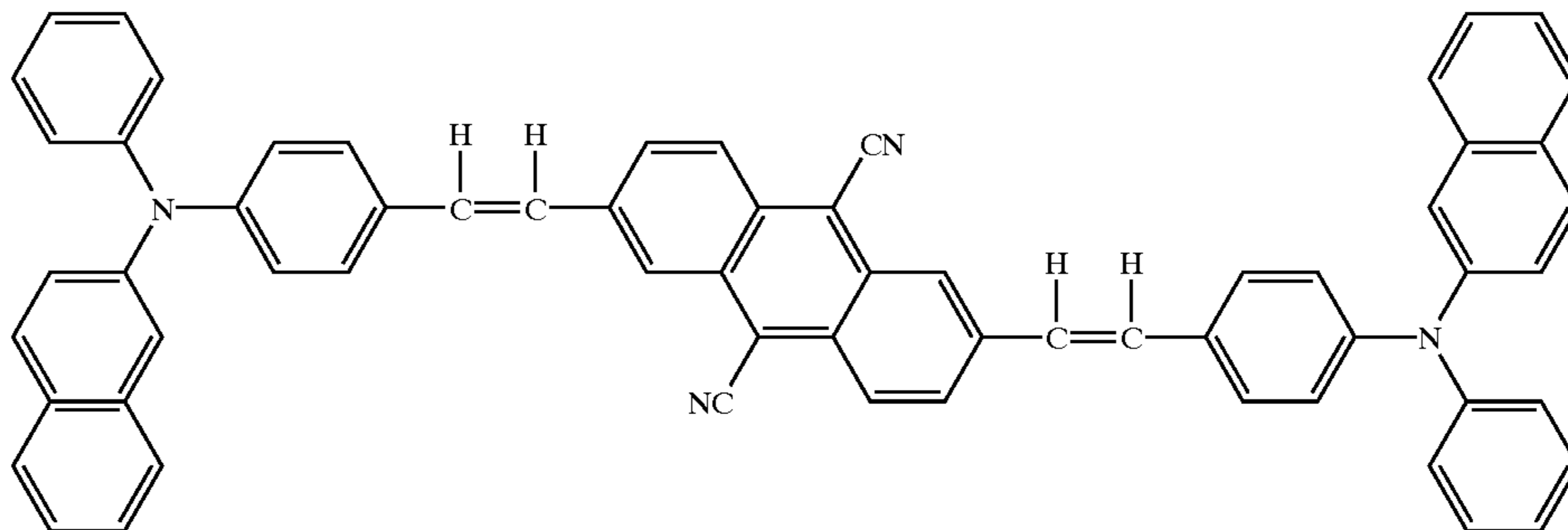
Structural Formula (7)-3:
