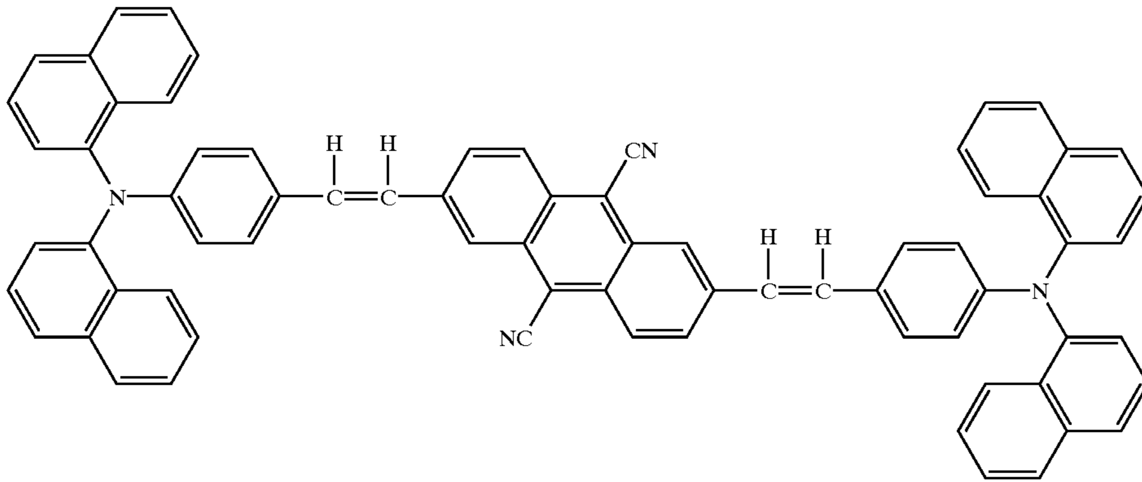
Structural Formula (7)-6:
