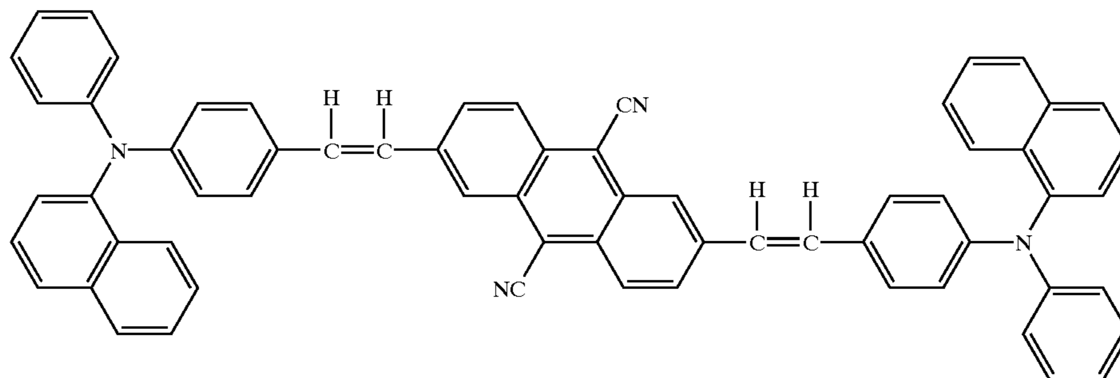
Structural Formula (7)-1:
