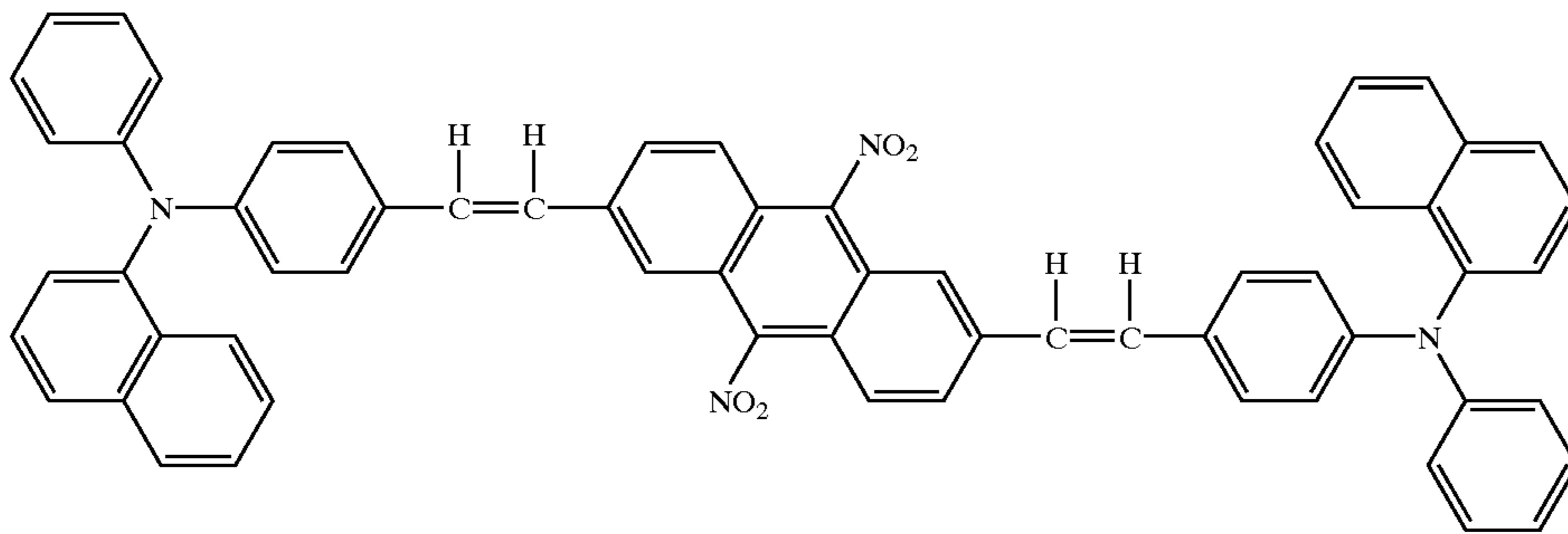
Structural Formula (7)-5:
