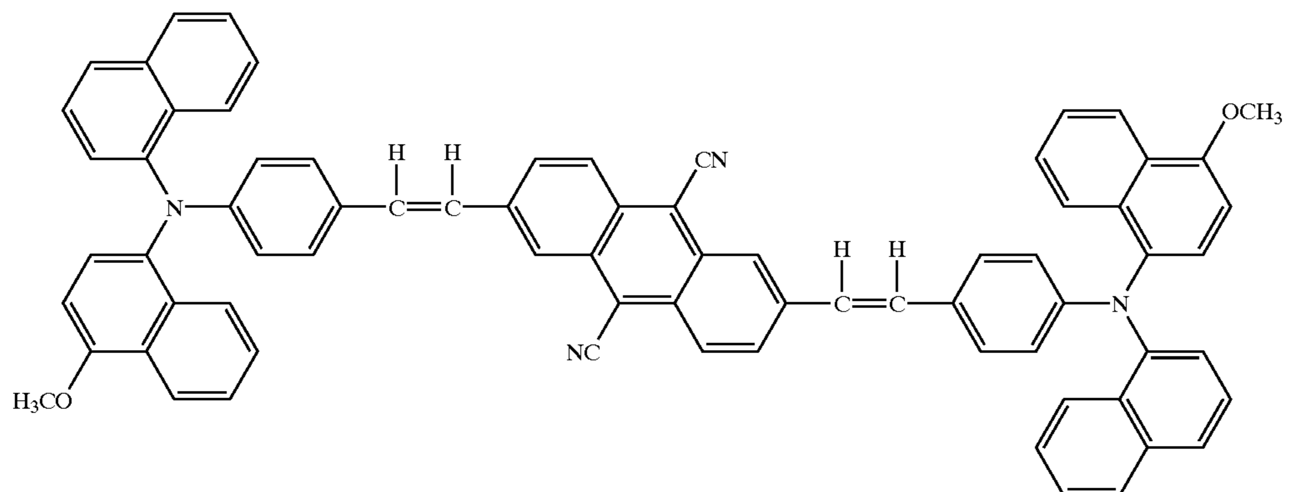
Structural Formula (7)-7:
