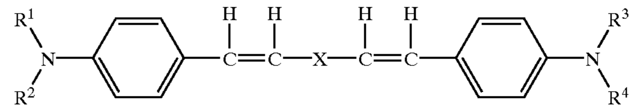
General Formula (1)
