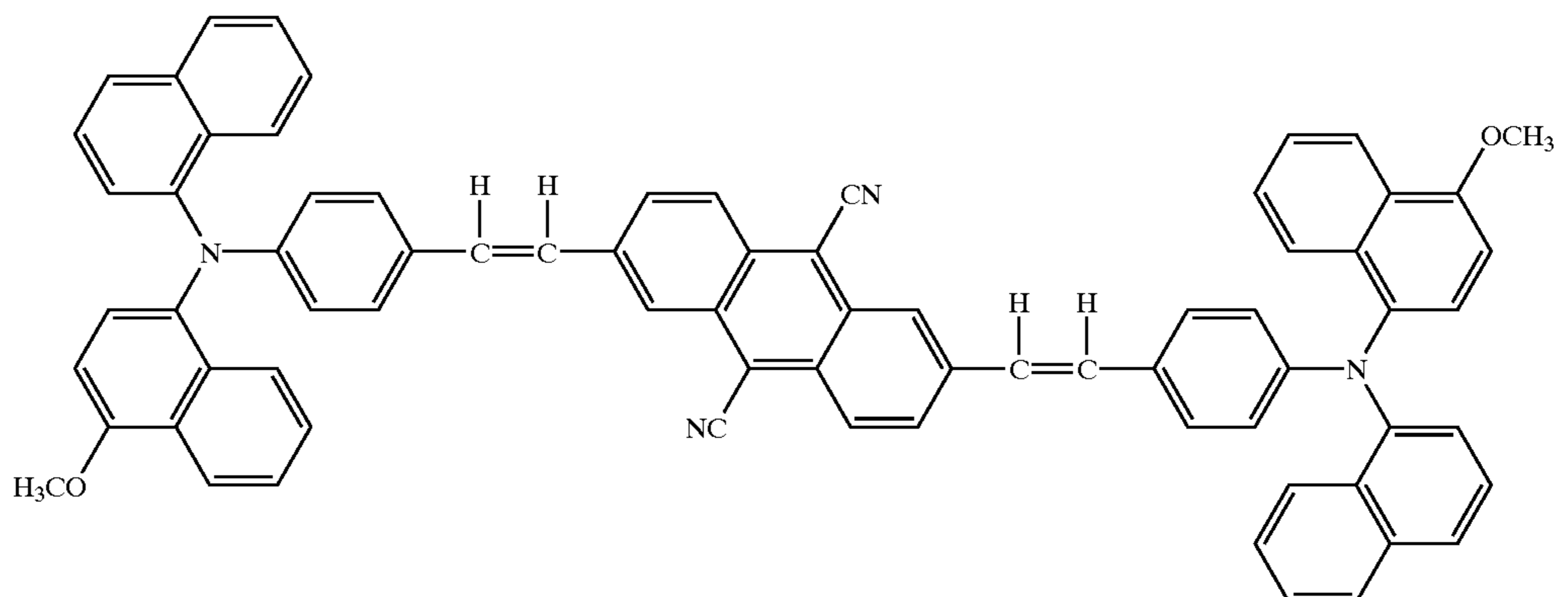
Structural Formula (7)-7:
