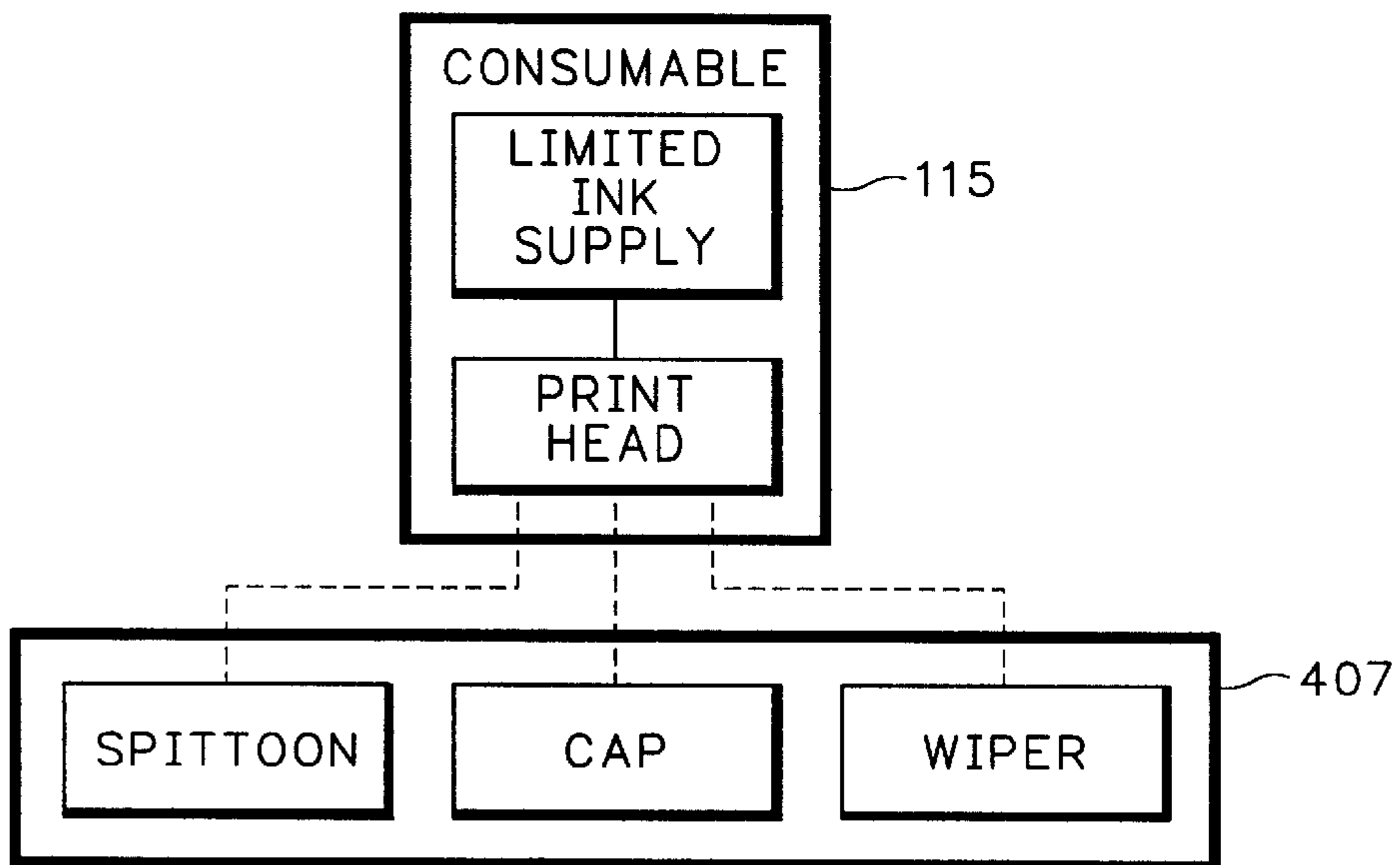
DISPOSABLE PRINT CARTRIDGE FLUIDIC BLOCK DIAGRAM
