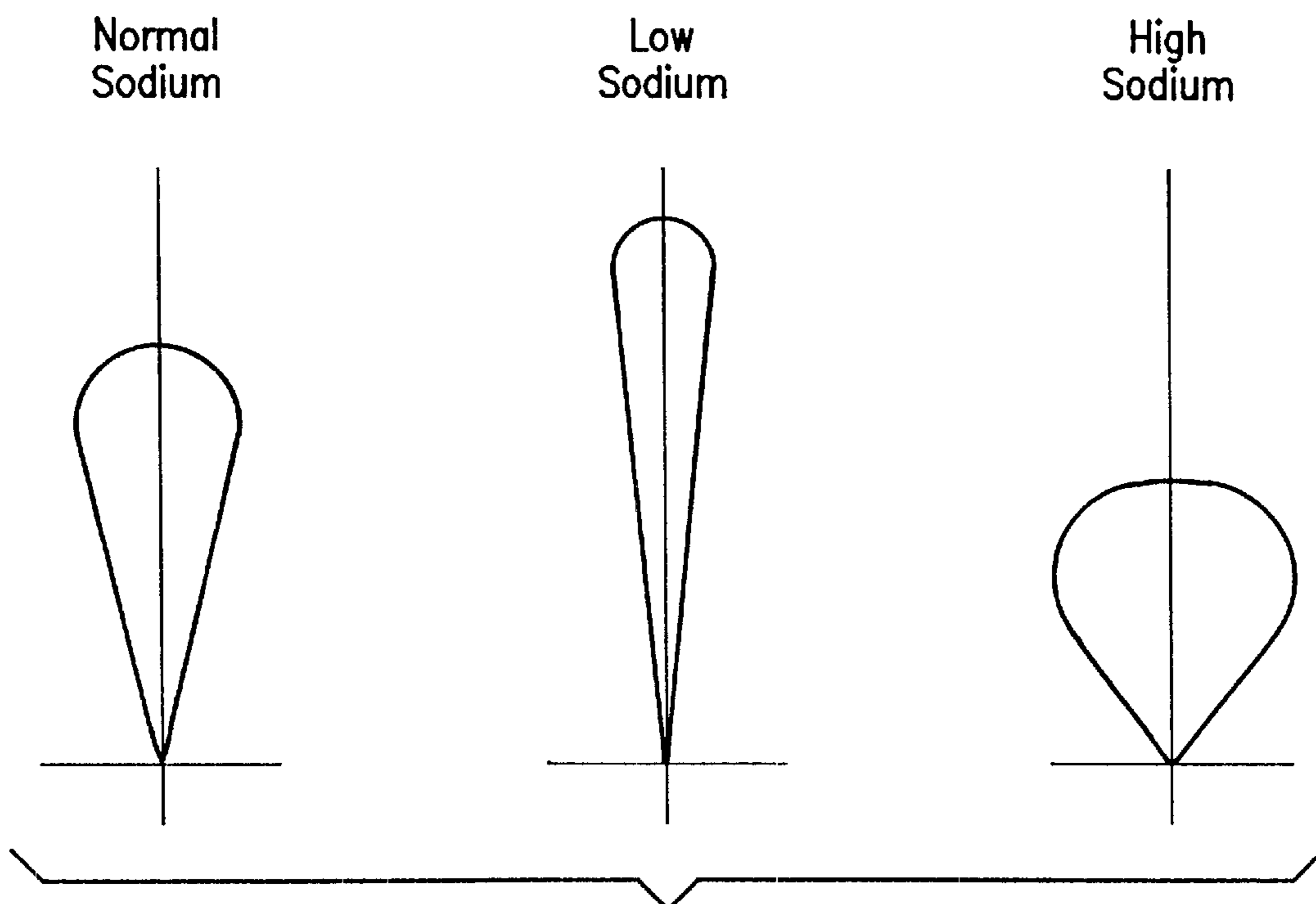
Scatter Diagrams
