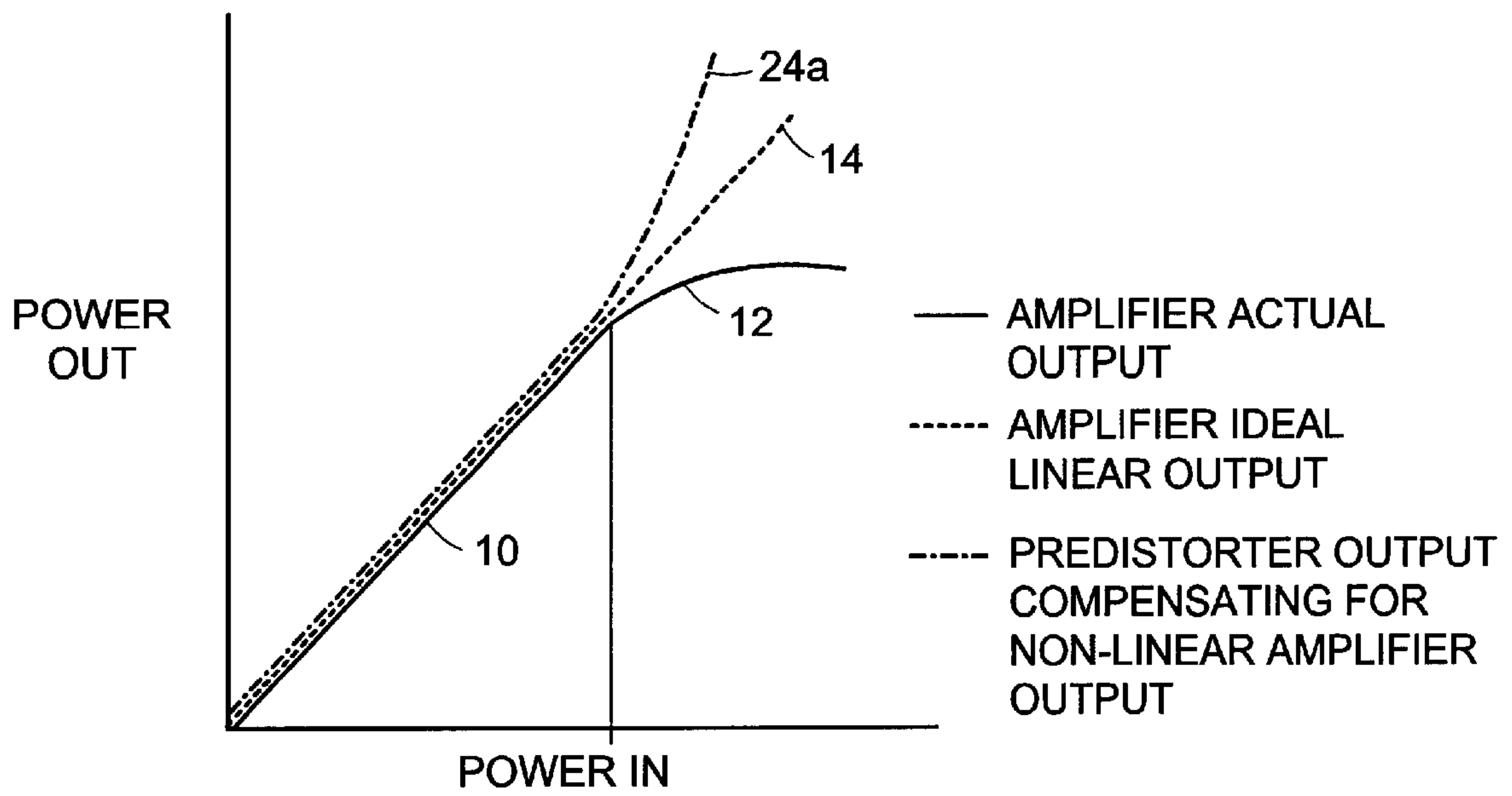
FIG. 1 (PRIOR ART)
