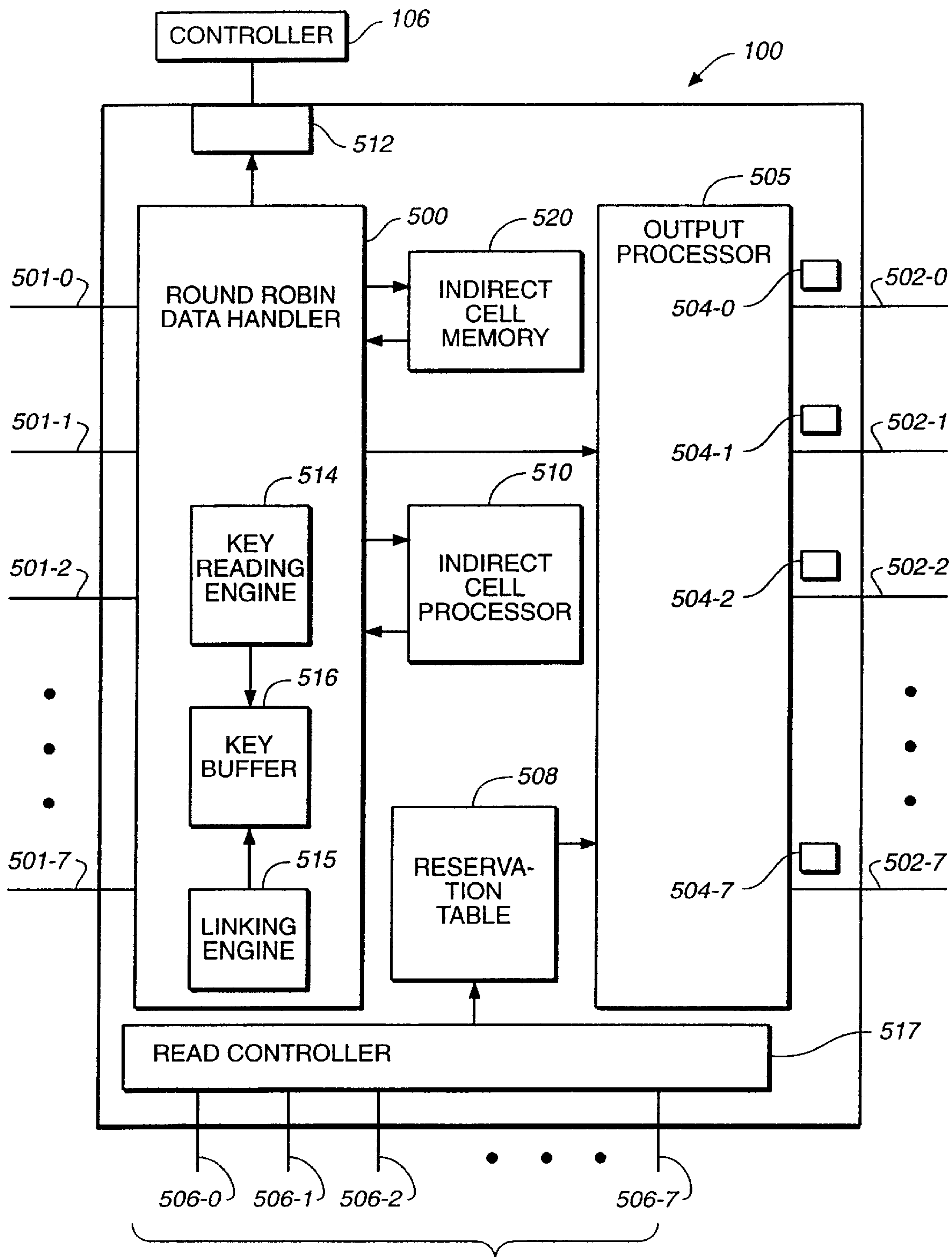
FIG. 5A READ REQUEST INPUTS FROM MULTI-FUNCTION MULTIPORTS 150
