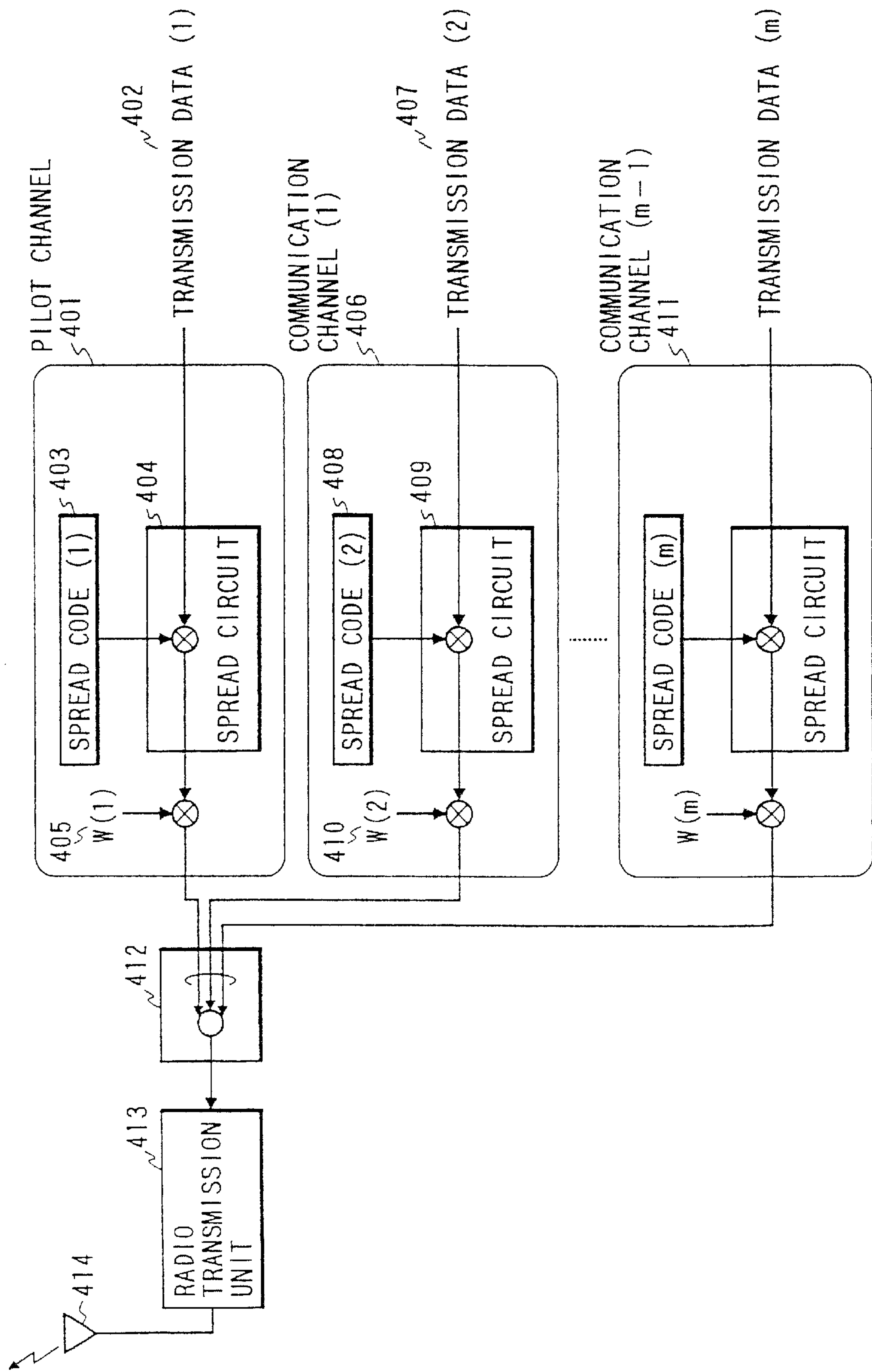
FIG. 4 PRIOR ART
