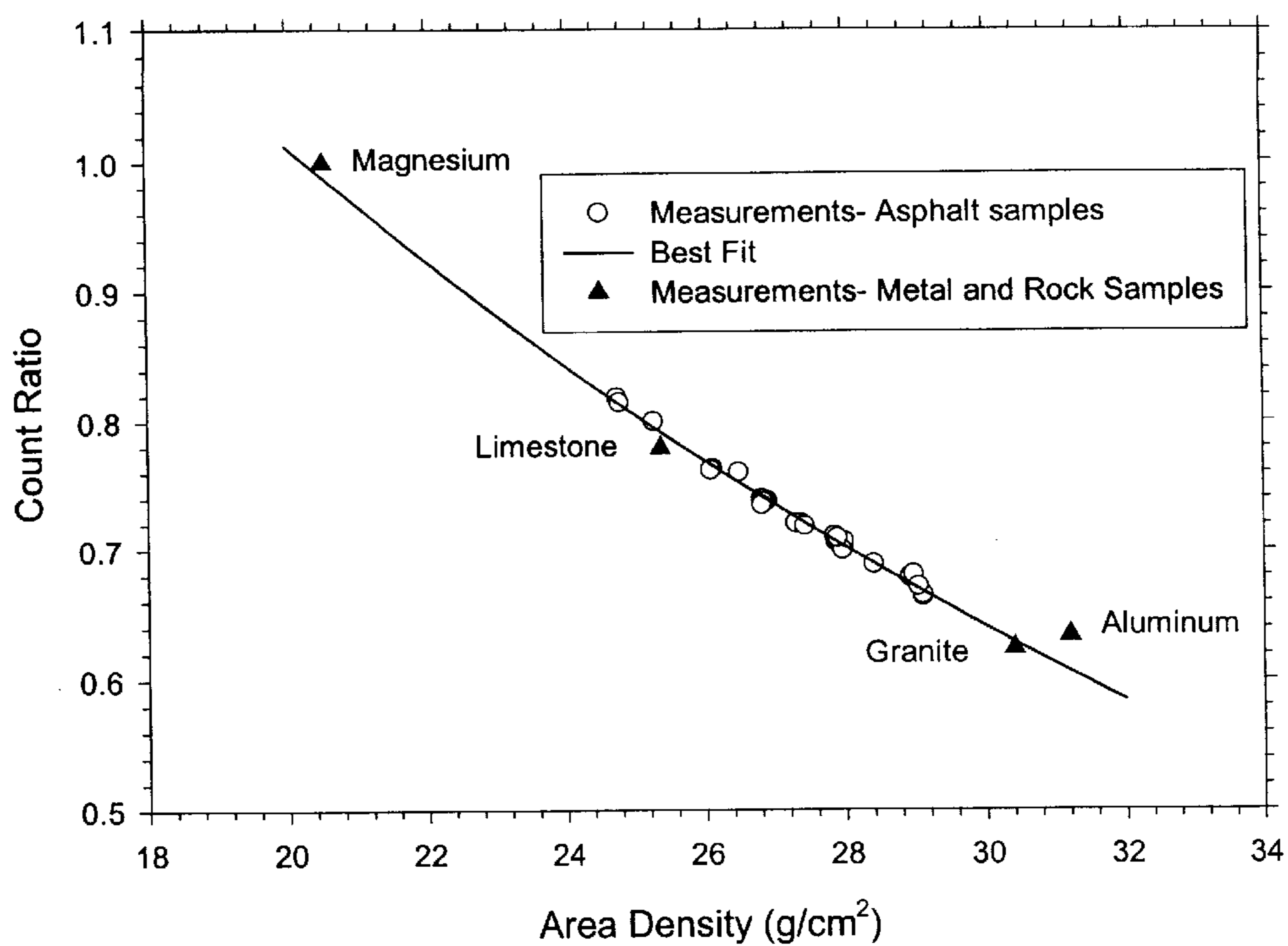
Figure 7 Asphalt Equivalent Normalization Factors for Metal and Rock Samples
