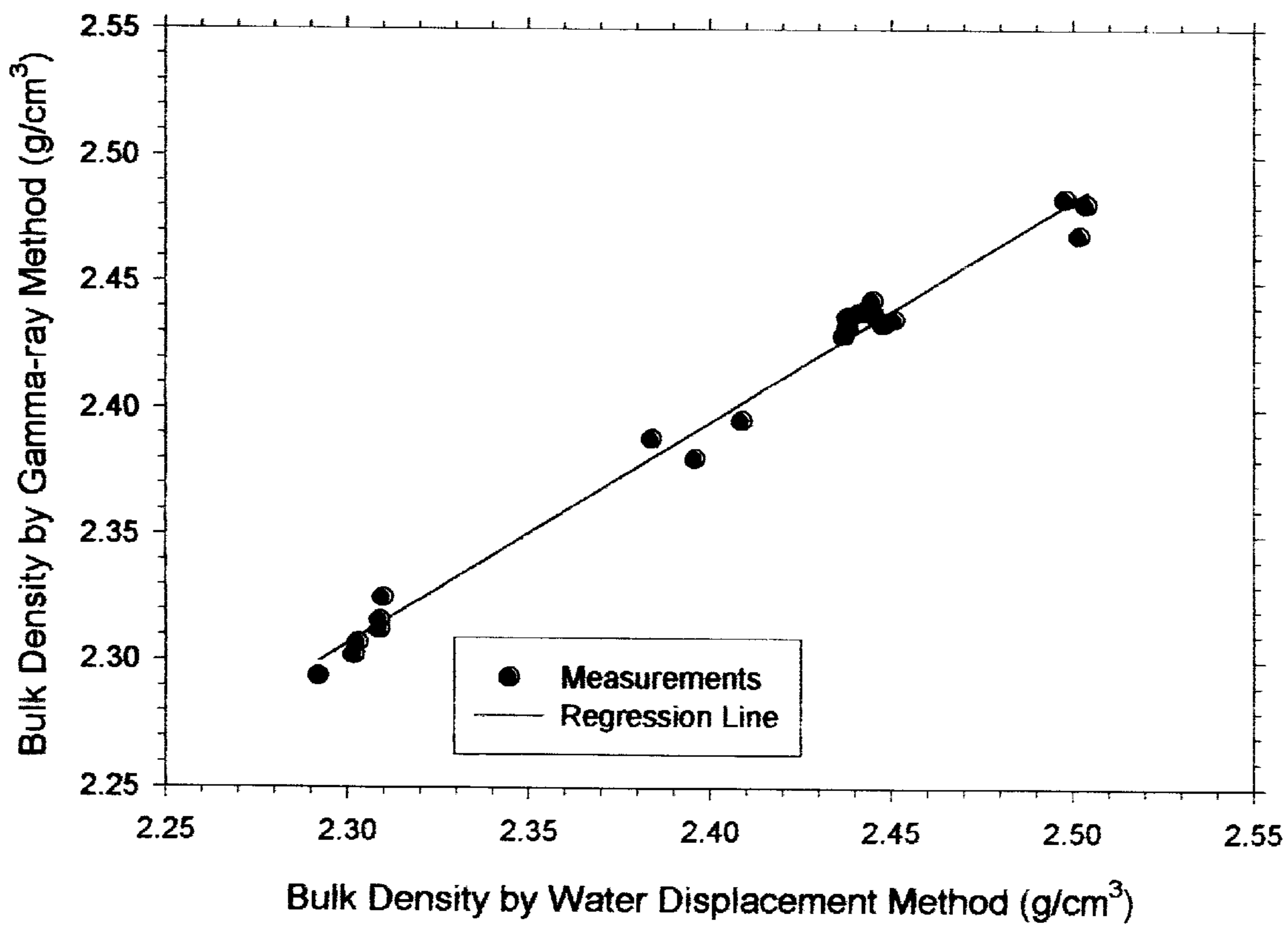
Figure 6 Bulk Density of Unknown Samples
