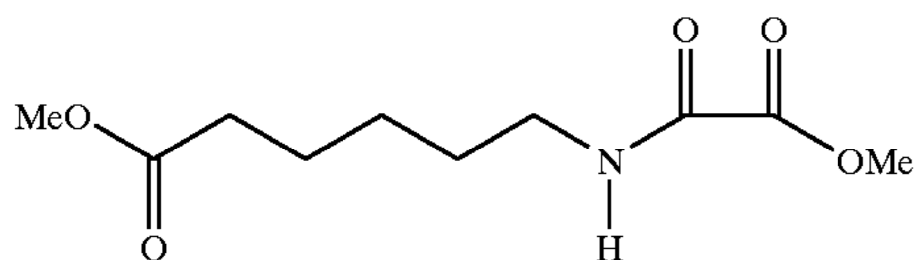
Compound B (n=11, R=Butyl)
