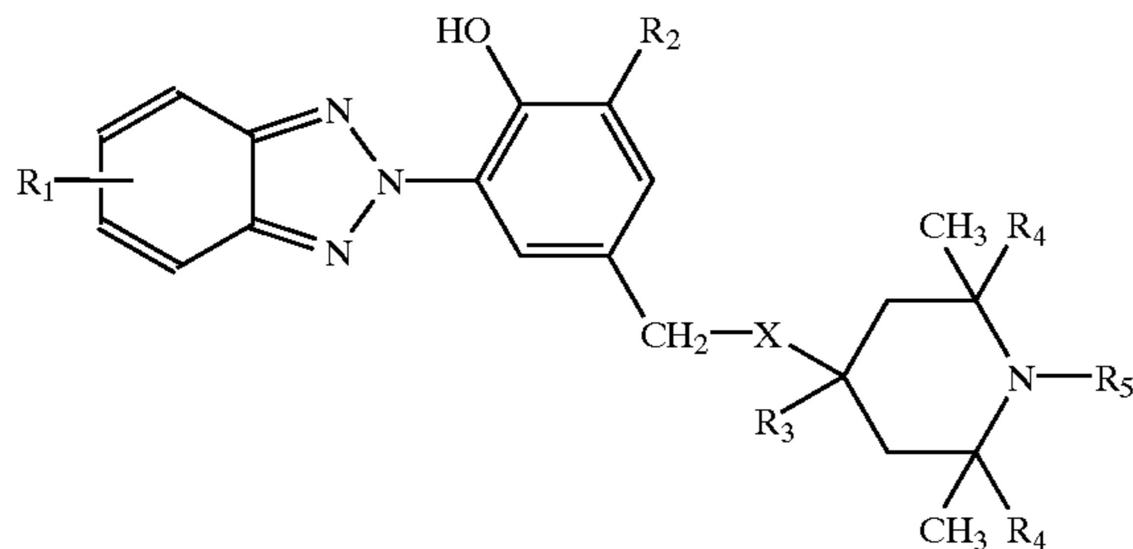
Formula (I)
