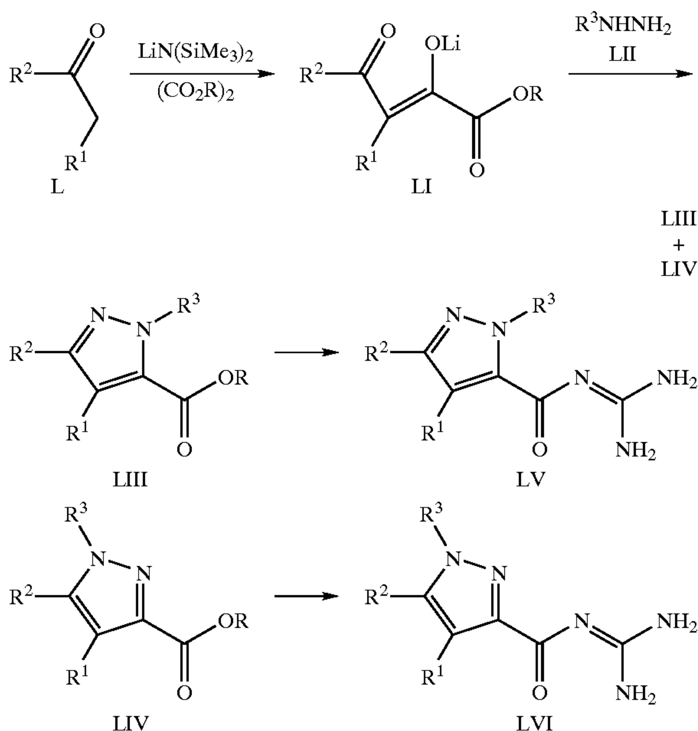
SCHEME VIII
