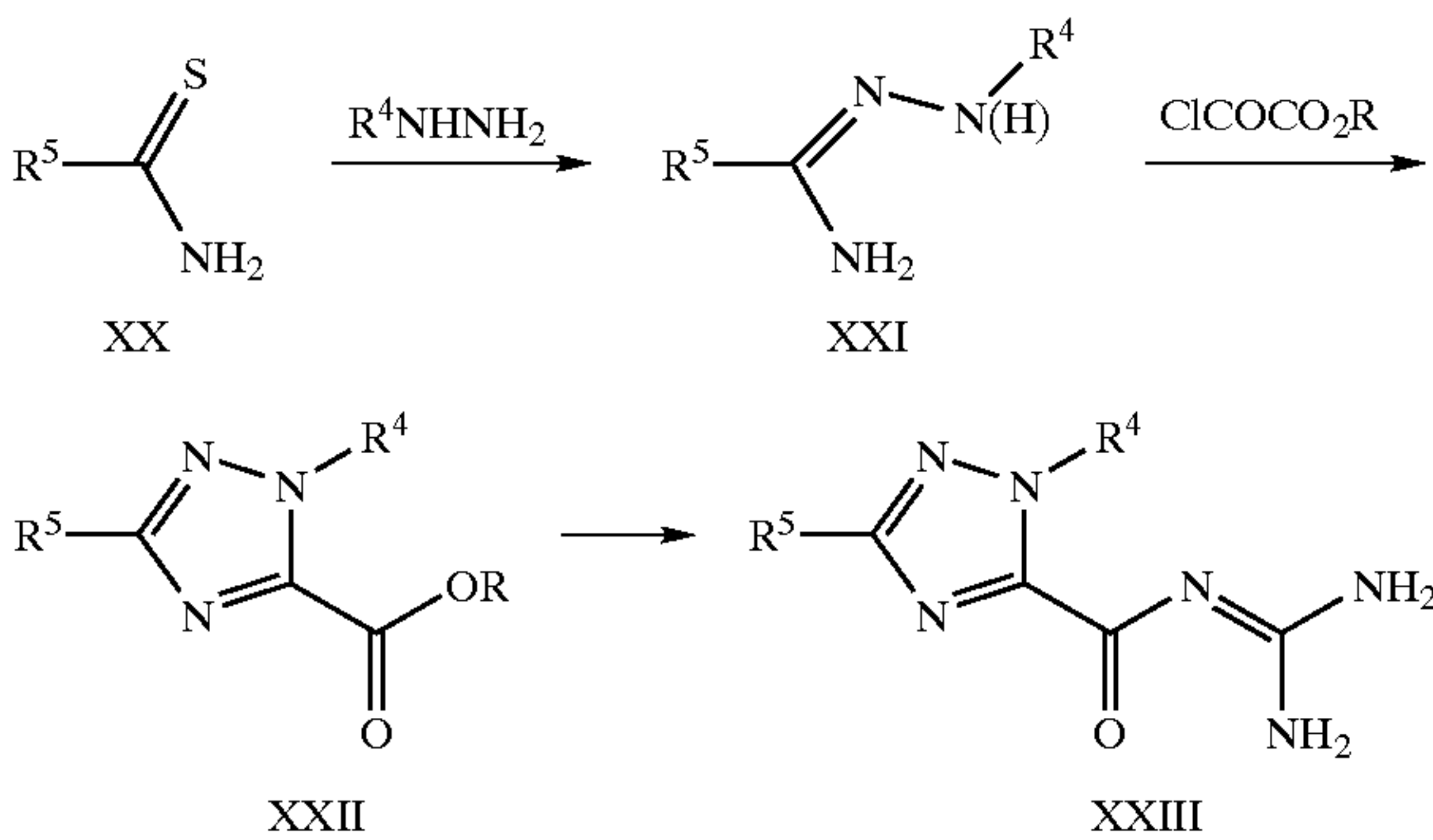
SCHEME IV
