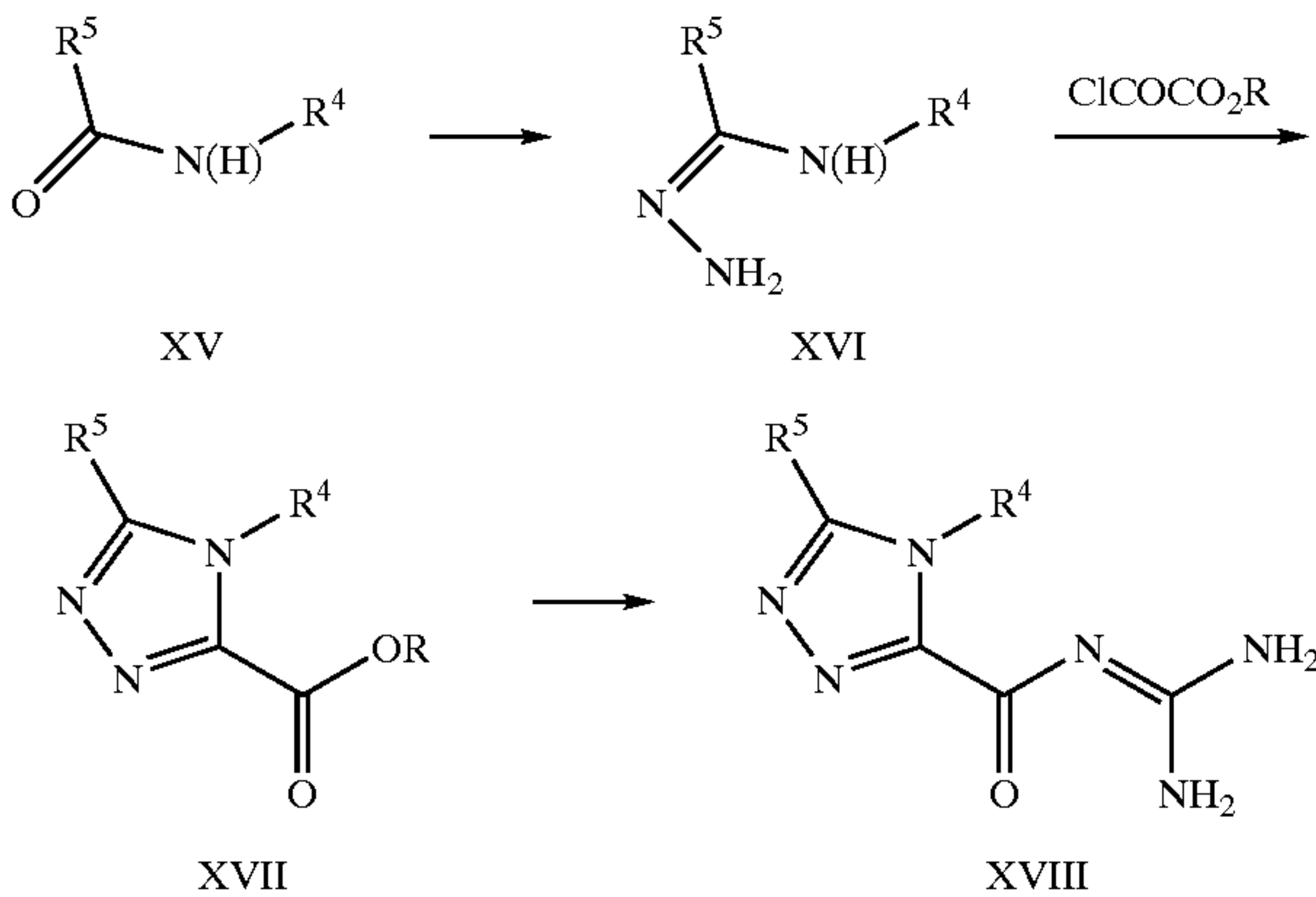
SCHEME III
