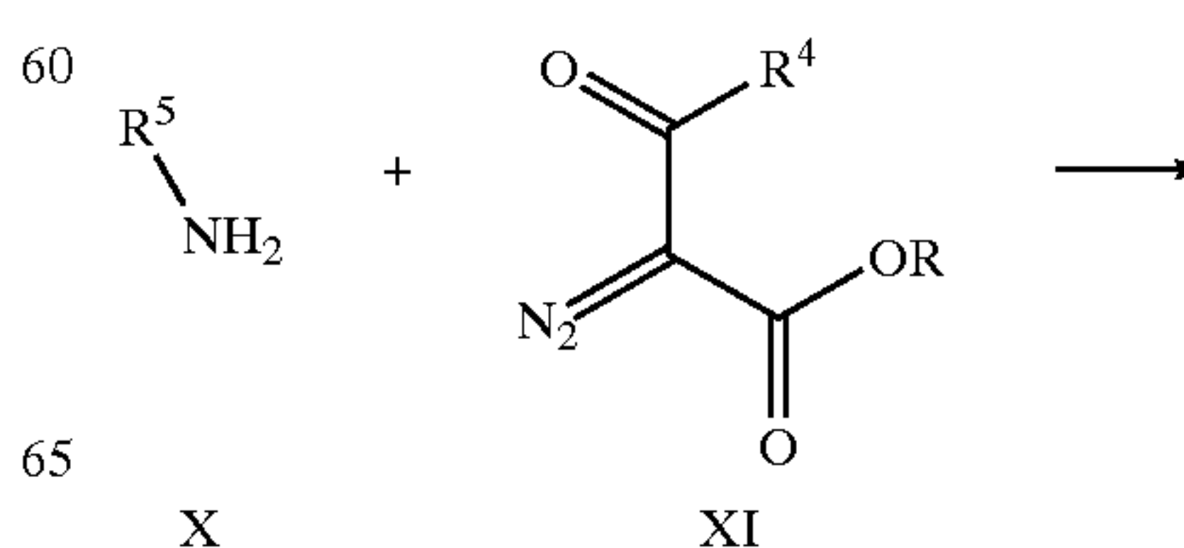
SCHEME II
