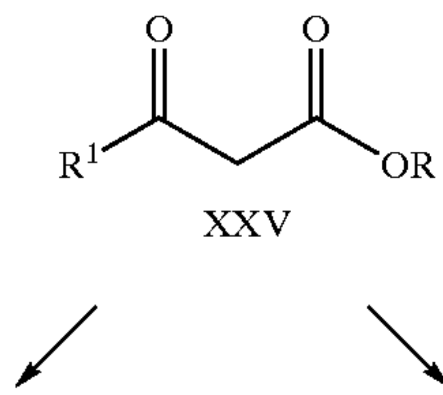
SCHEME V
