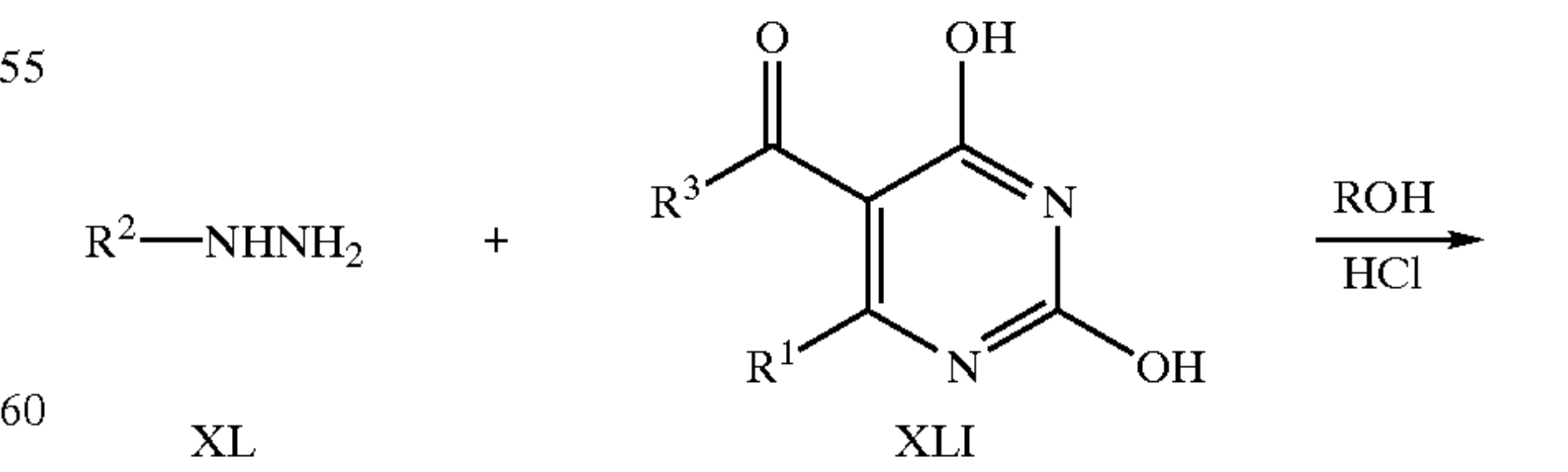
SCHEME VII
