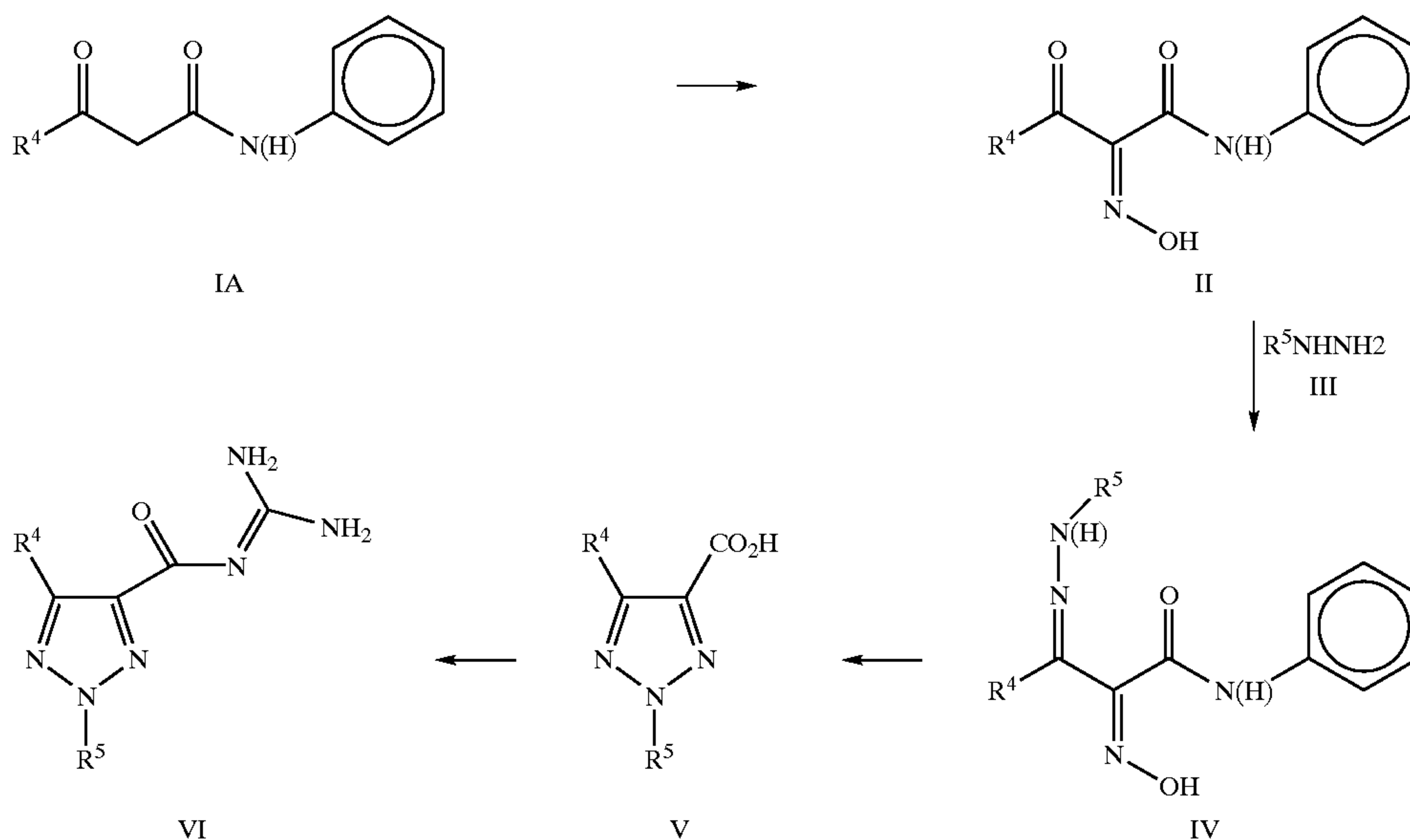
SCHEME I
