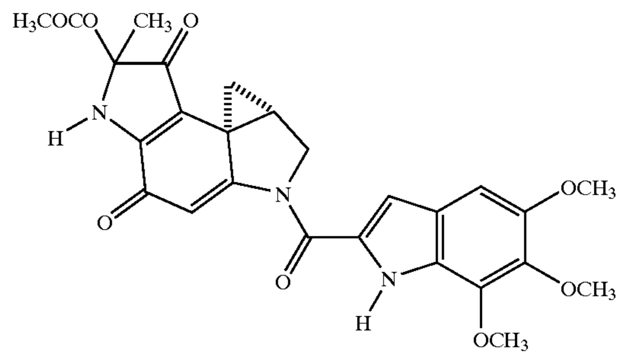
Duocarmycin A
