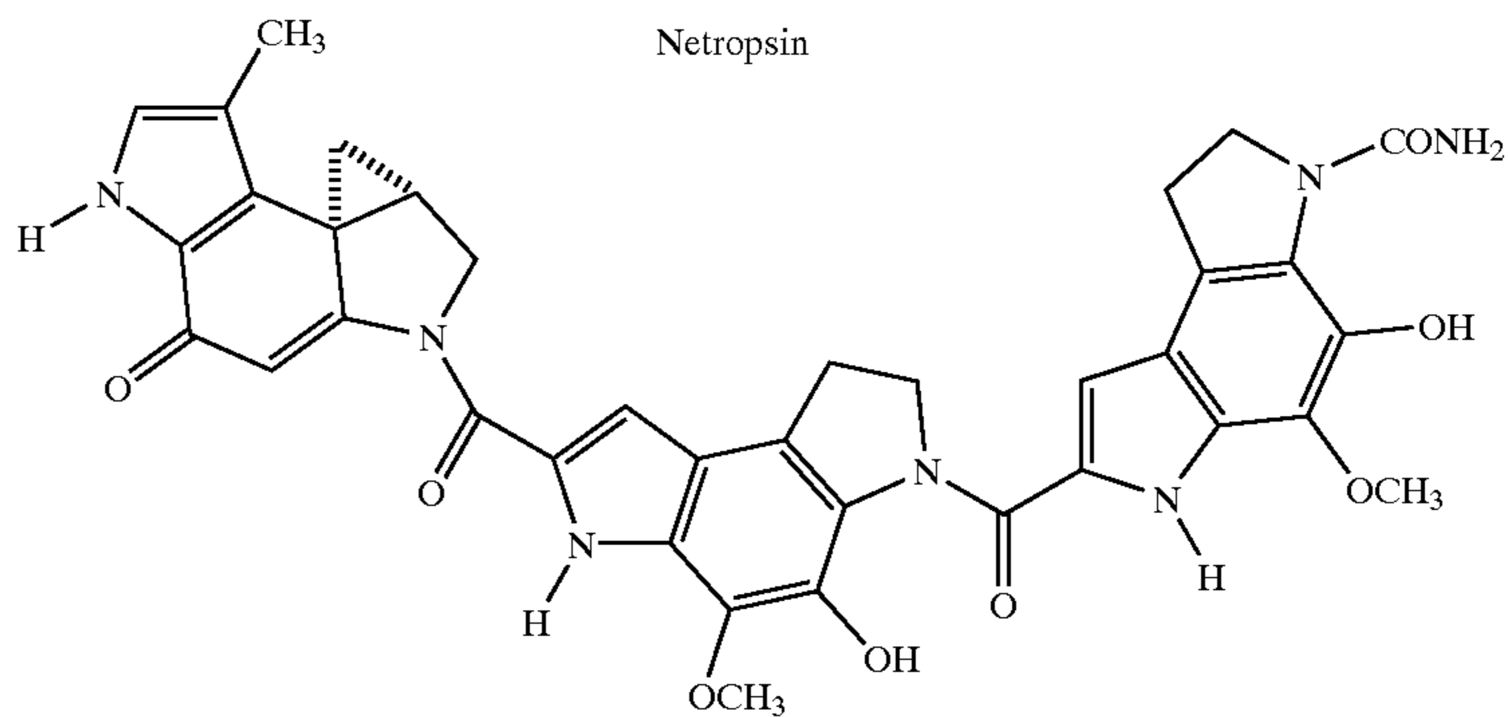
CC-1065
