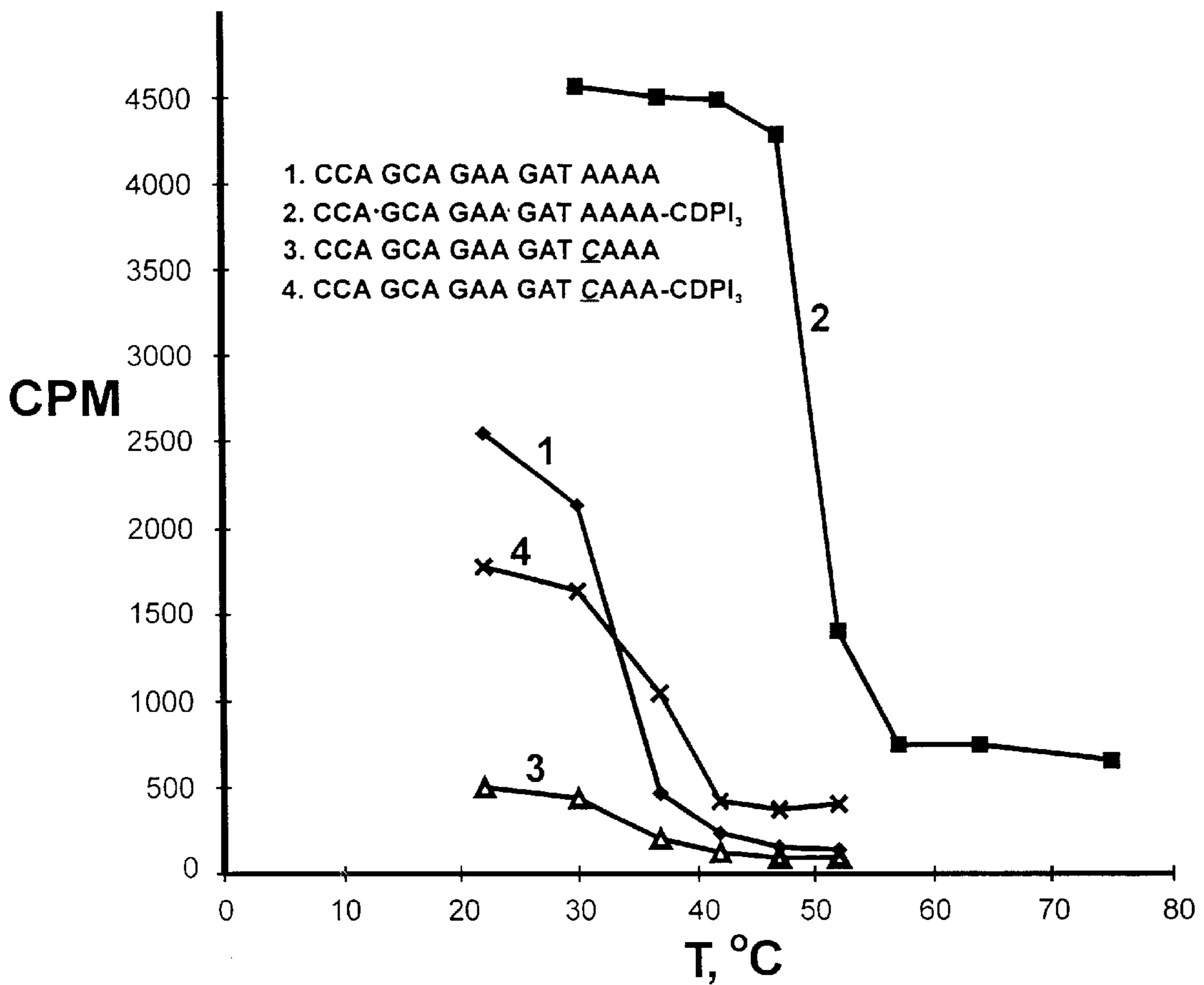
Figure 1: Slot blot hybridization of unmodified ODN or 3'-ODN-CDPI 3 conjugates to M13mp19 (+) strand DNA. Underlined nucleotides represent mismatches with the targeted plasmid sequence.
