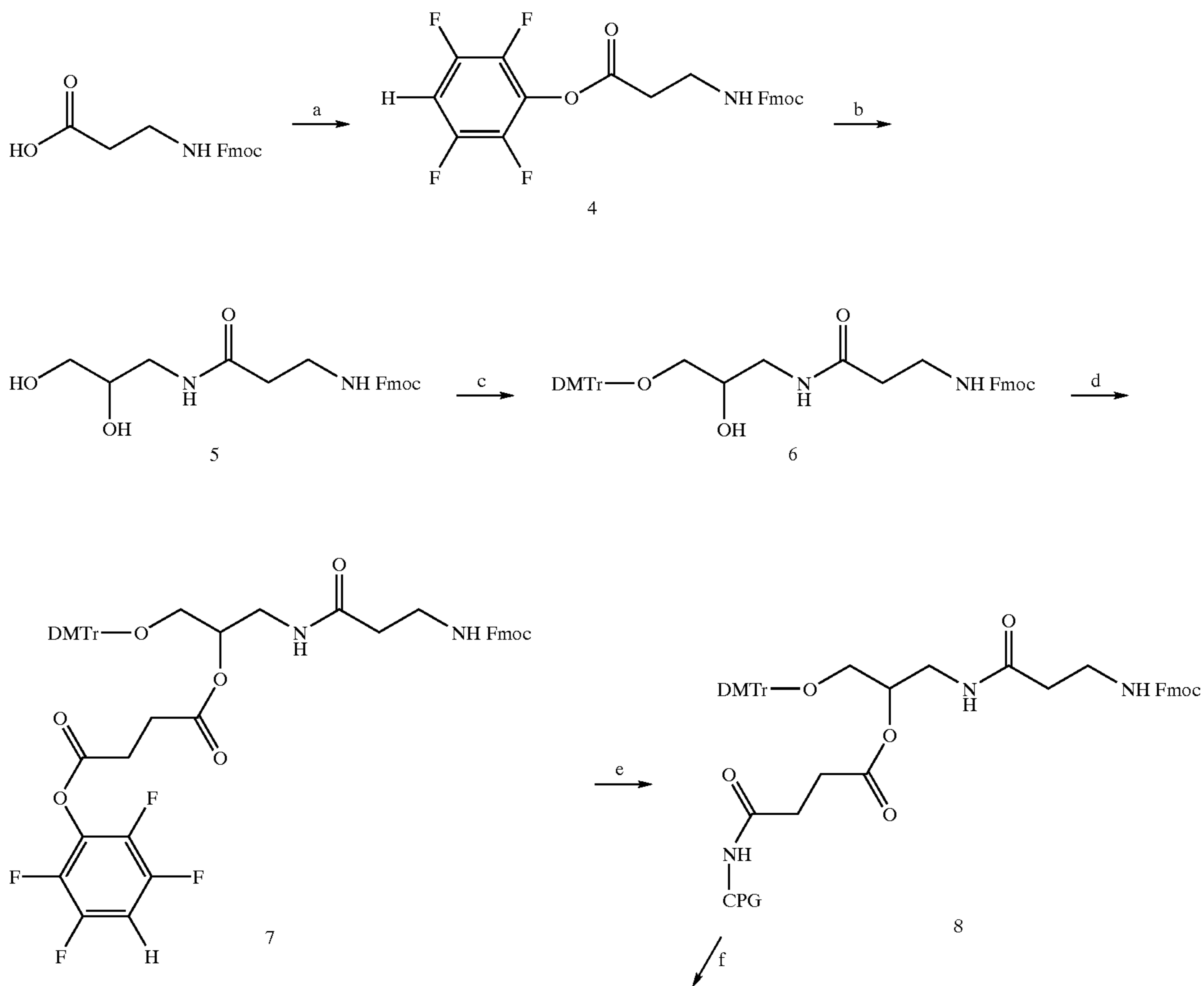
Reaction Scheme 5
