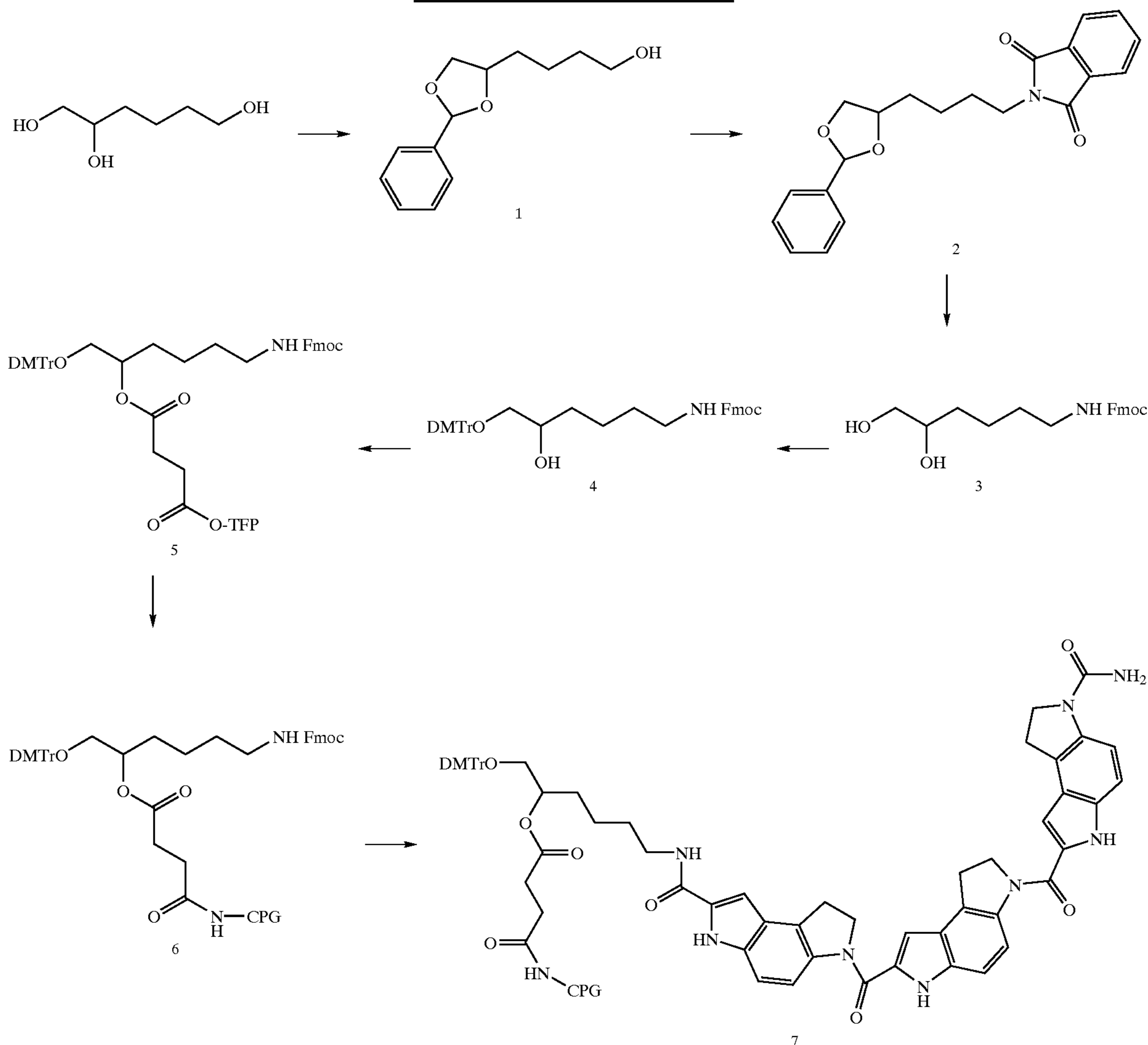
Scheme 6 Preparation of \text{CDPI}_3 -CPG support (below)
