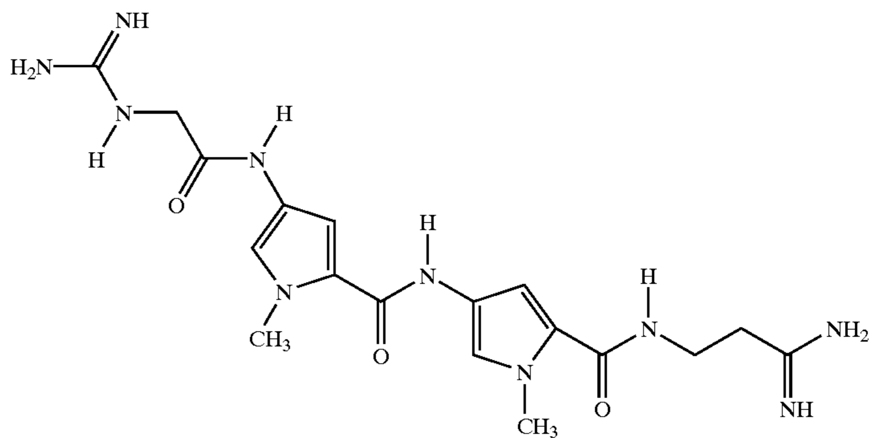
Netropsin
