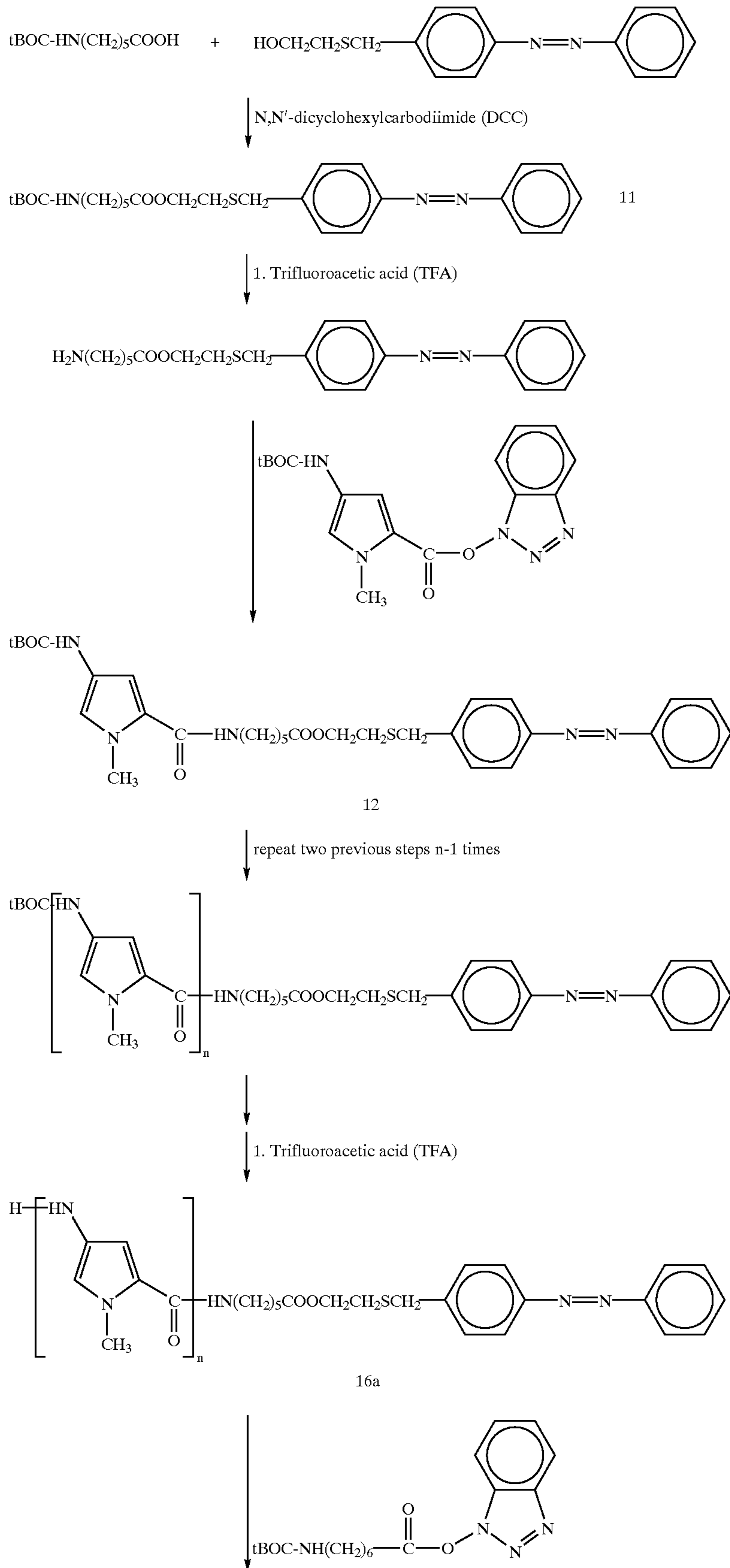
Reaction Scheme 2
