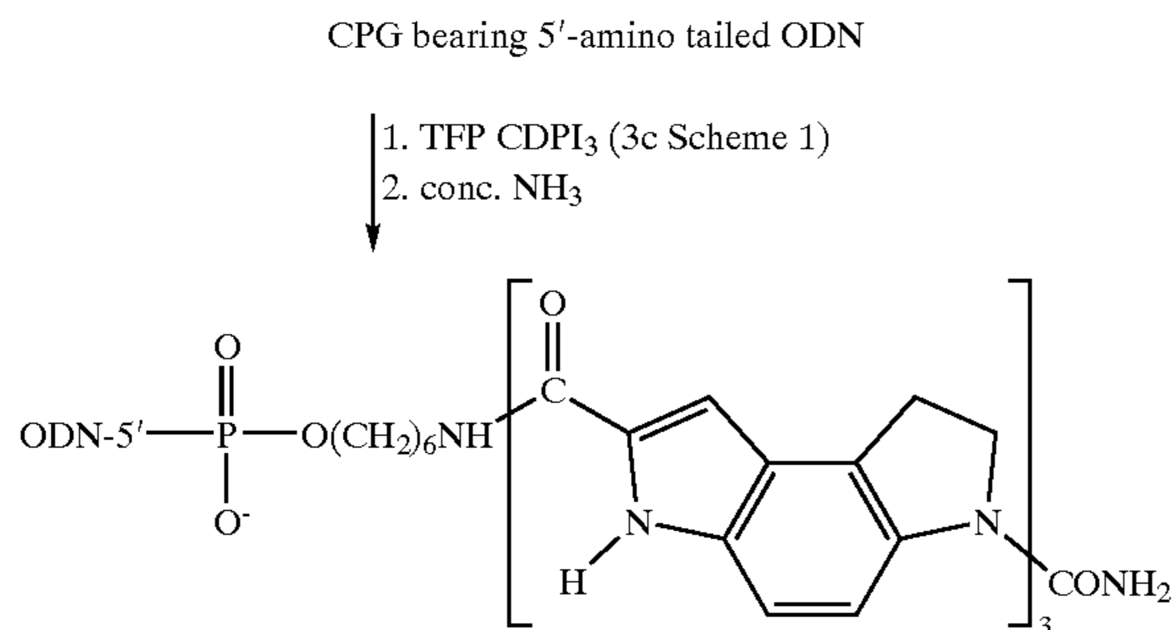
Reaction Scheme 4
