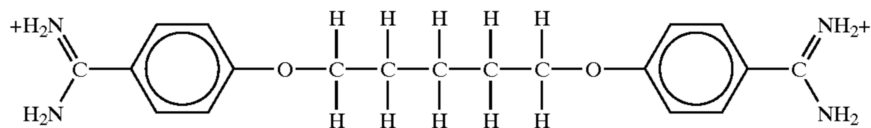
Pentamidine
