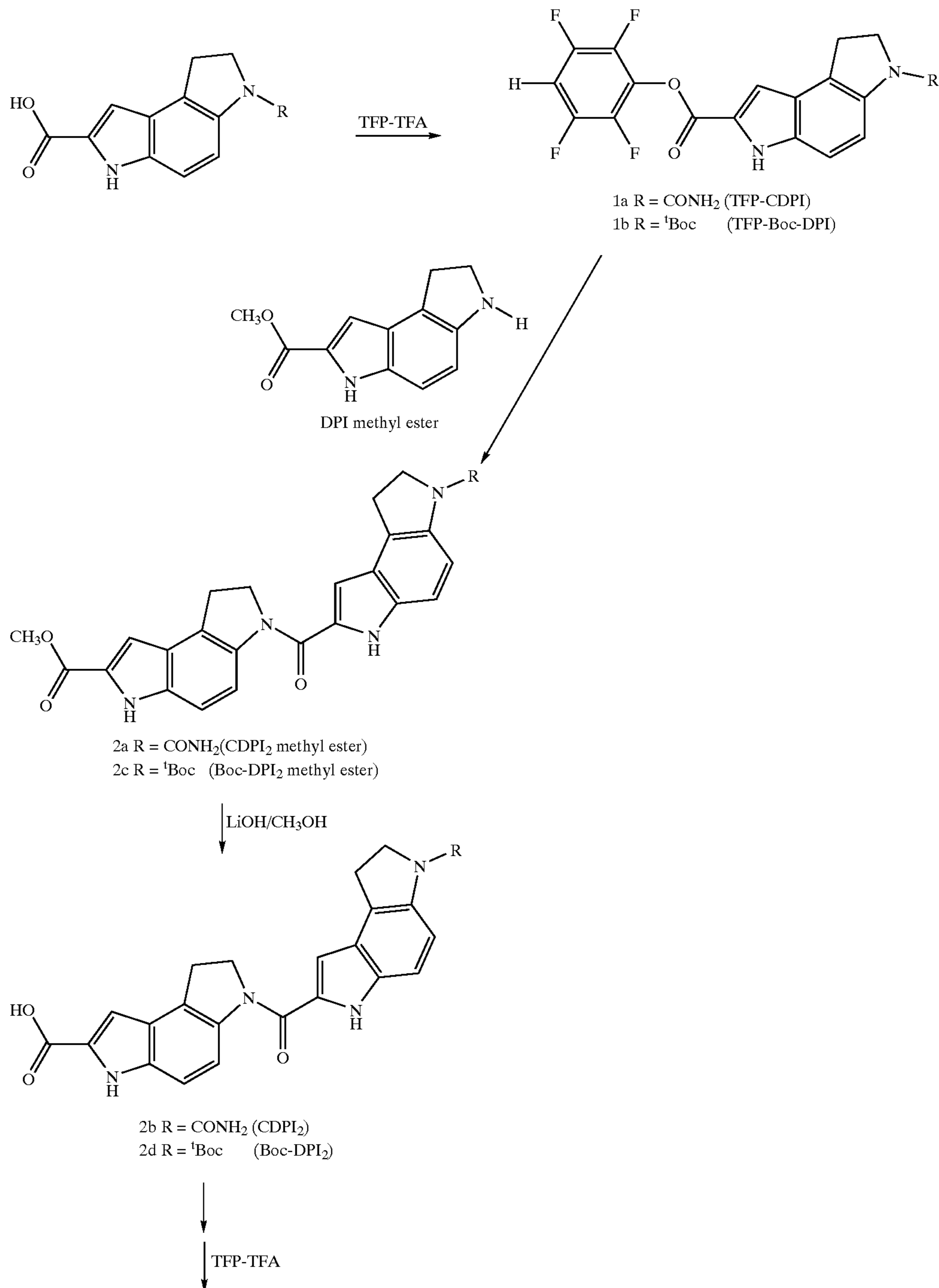
Reaction Scheme 1
