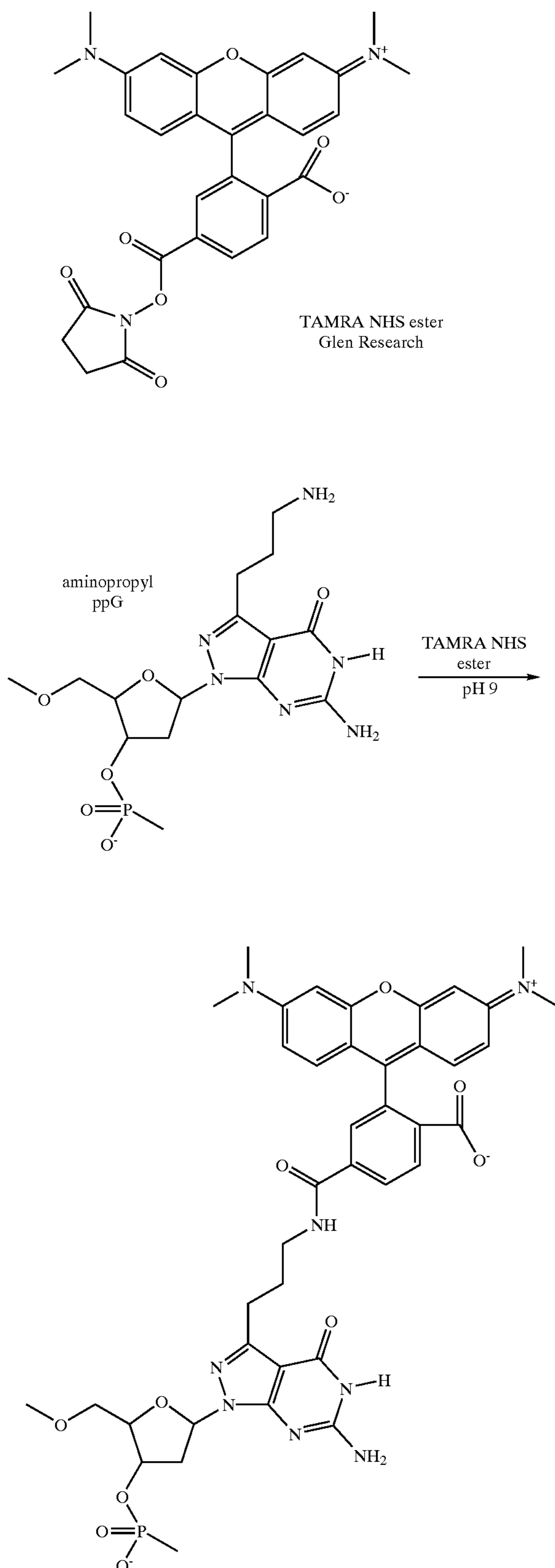
Scheme 9 Postsynthesis introduction of TAMRA quencher at the internal ppG or ppA residues (below)
