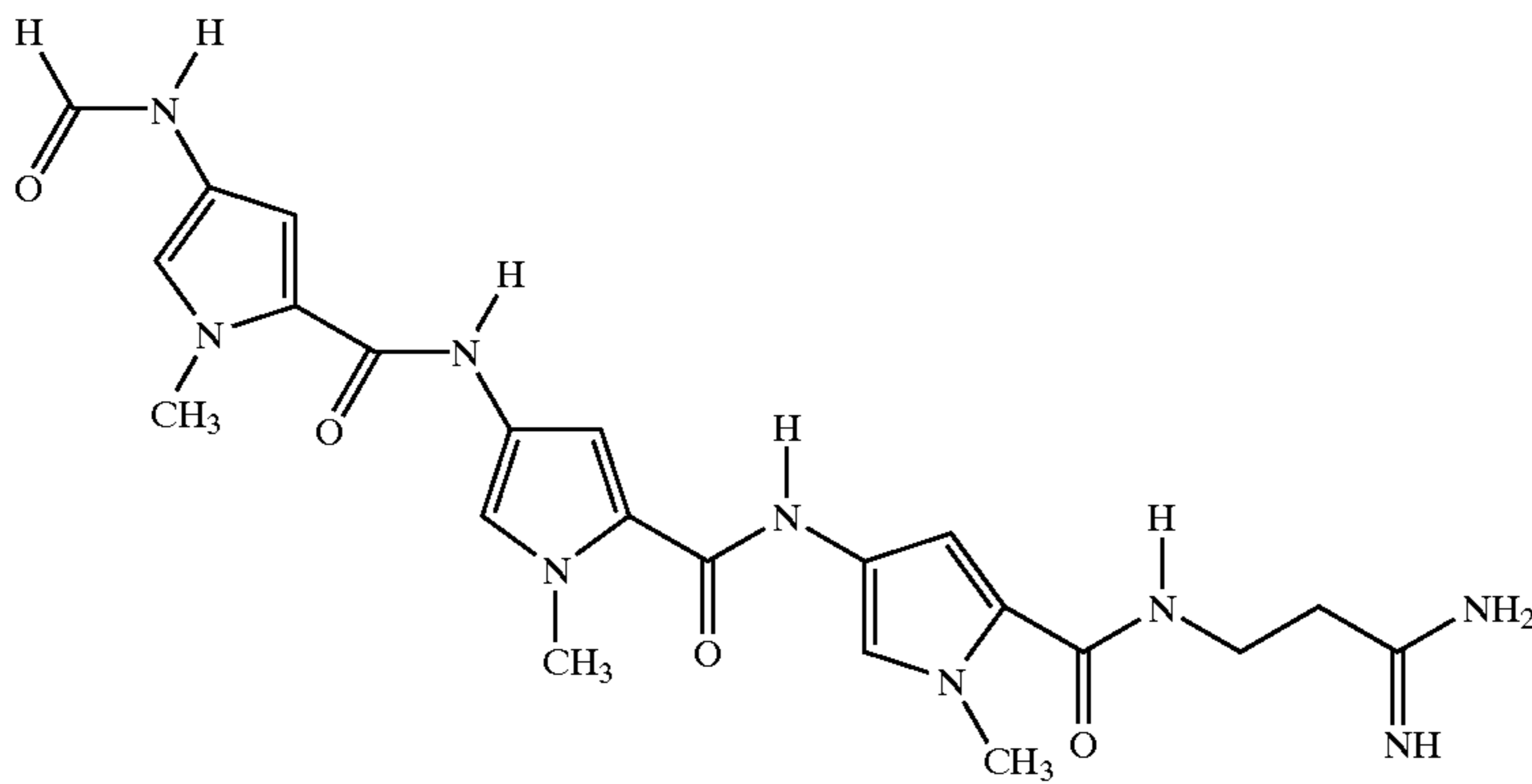
Distamycin
