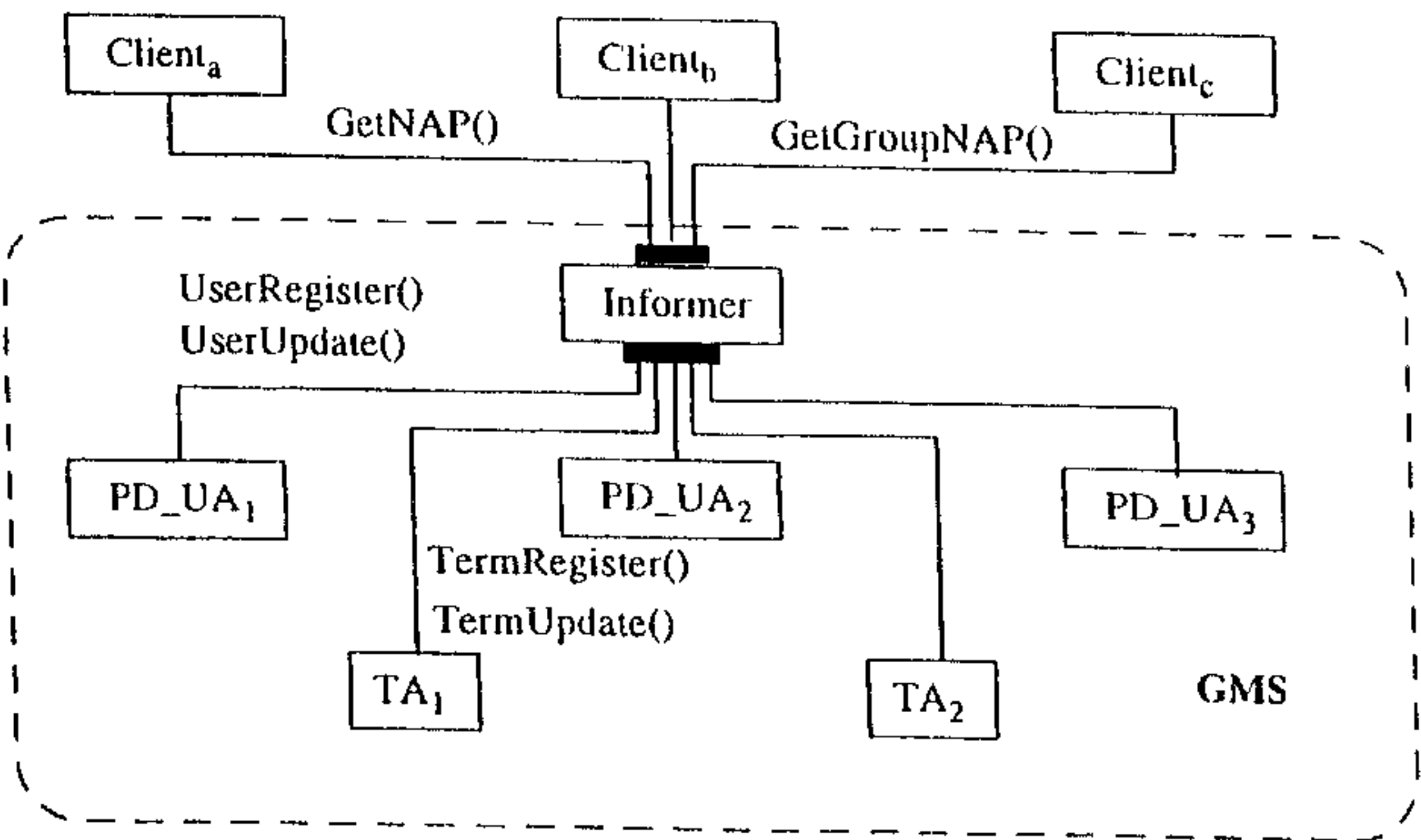
The Informer object provides location information service to the applications
