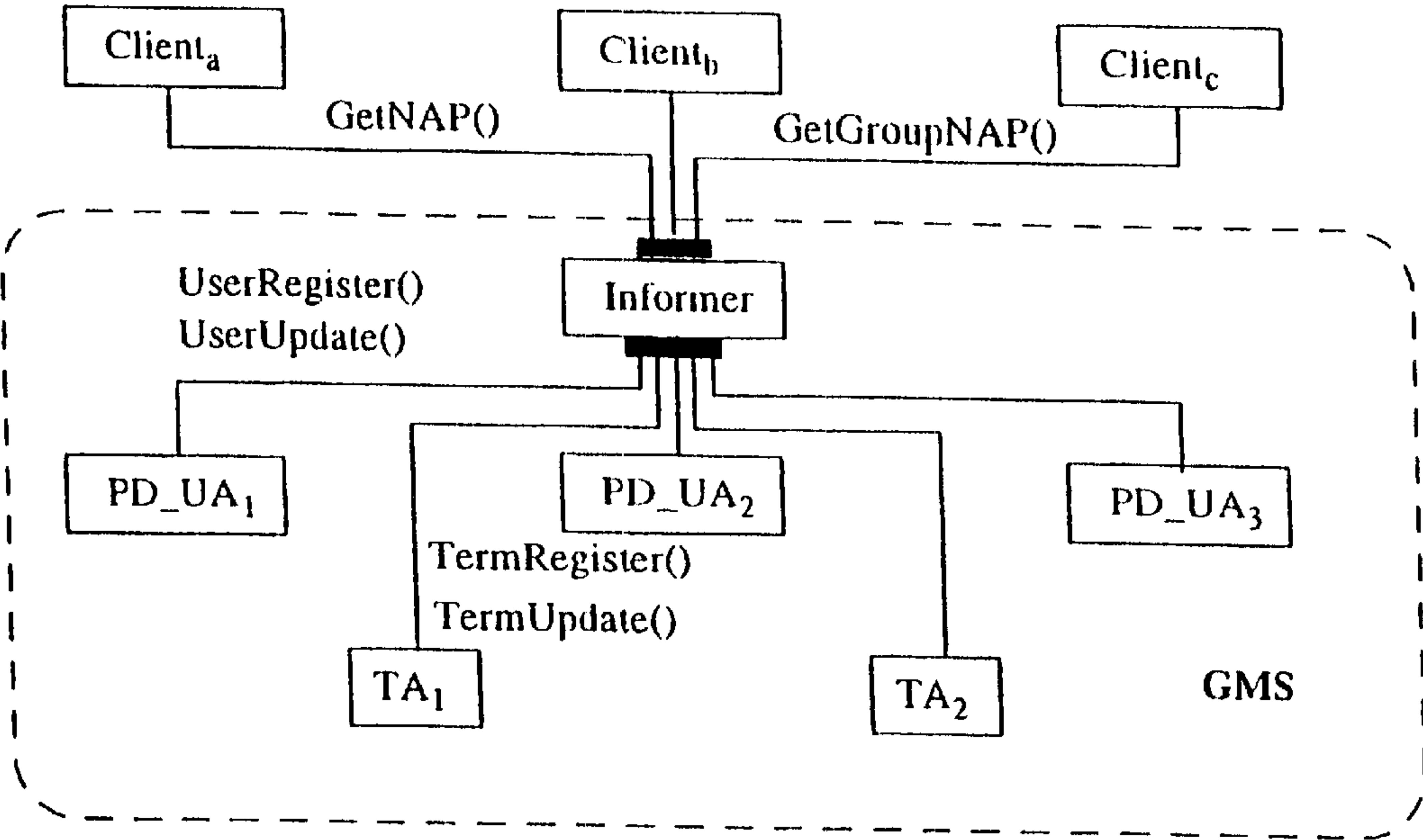
Figure 1 The Informer object provides location information service to the applications
