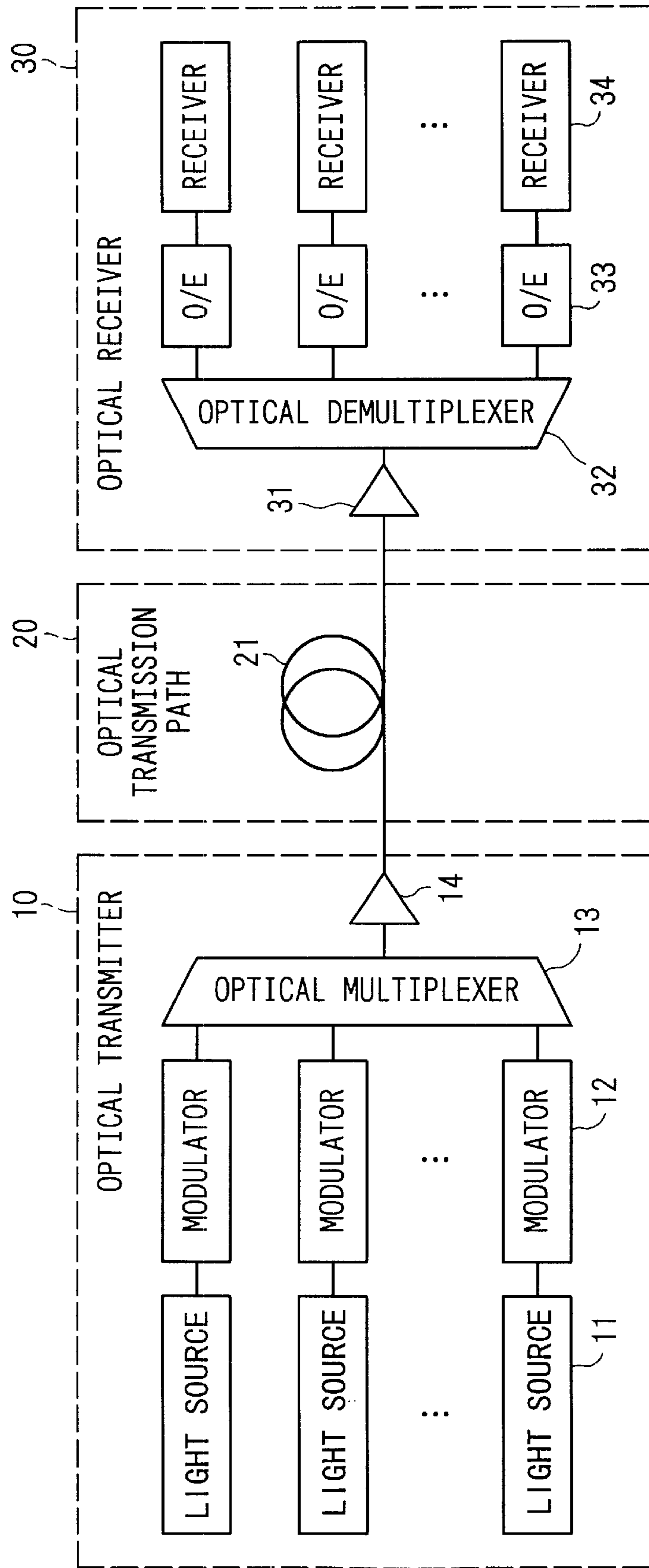
FIG.1 STRUCTURE OF THE FIRST EMBODIMENT OF THE PRESENT INVENTION
