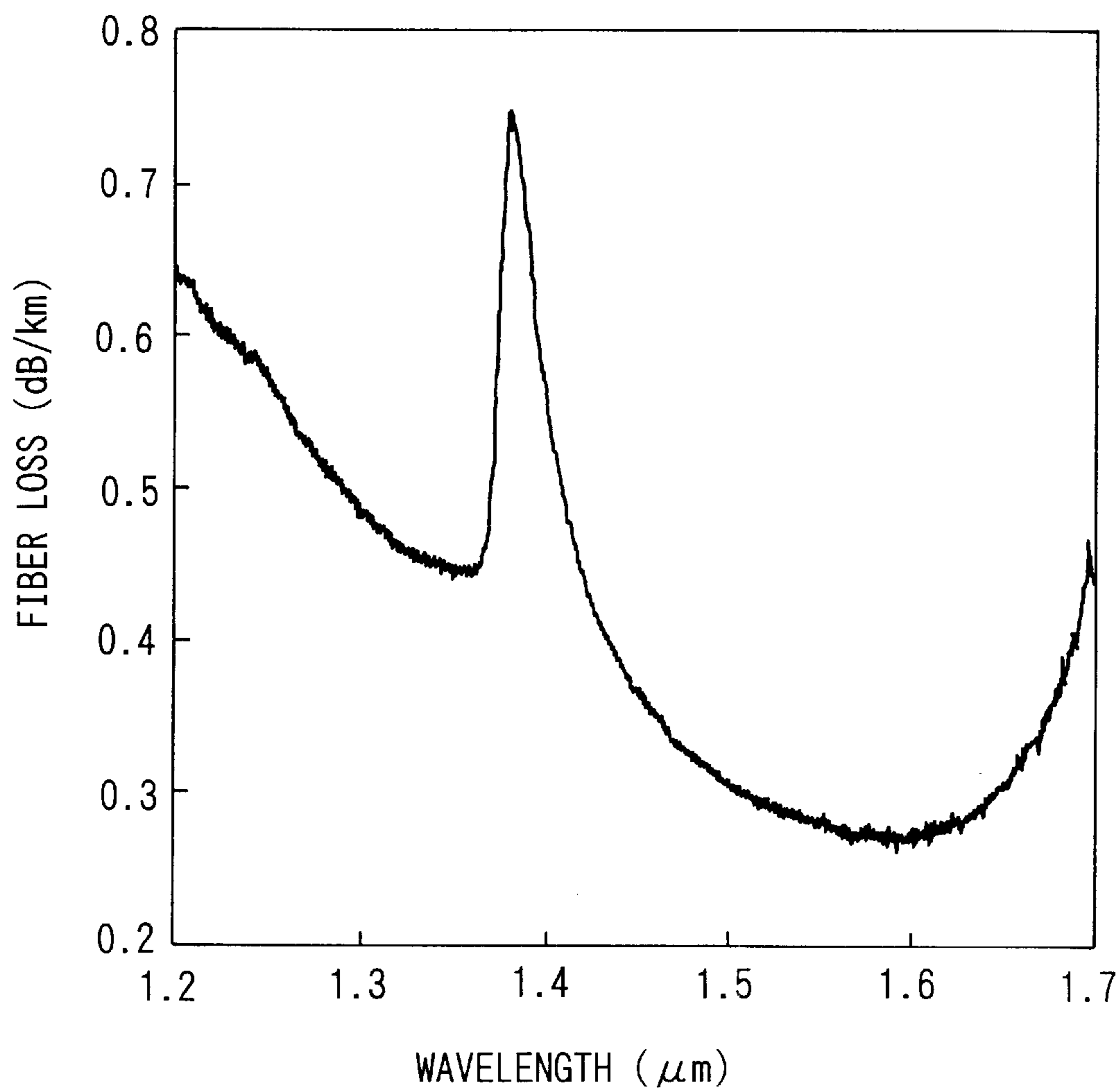
LOSS CHARACTERISTICS OF AN ON-SITE OPTICAL FIBER FOR COMMUNICATION
