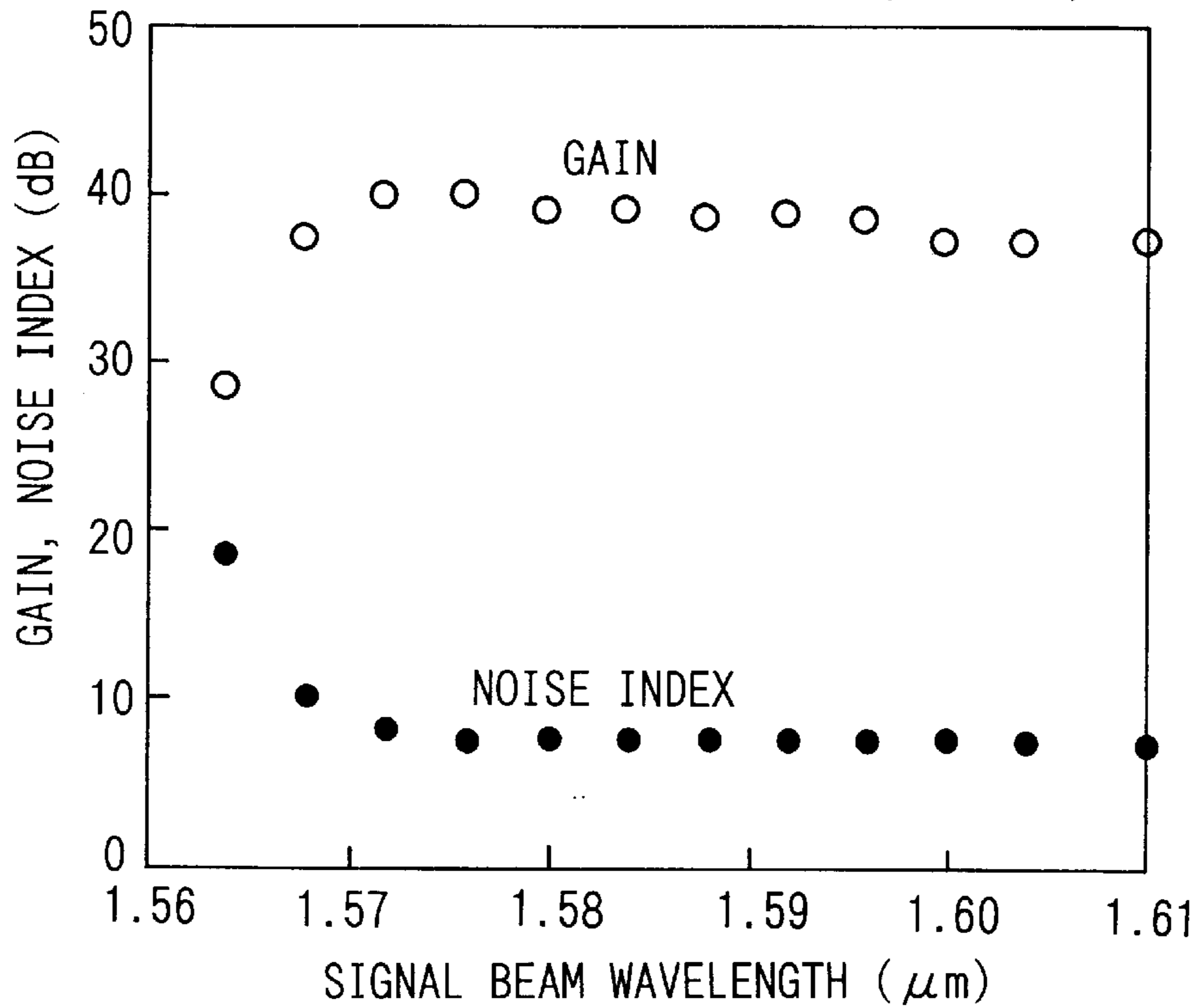
GAIN CHARACTERISTICS OF A Er-DOPED OPTICAL FIBER AMPLIFIER (GS-EDFA)
