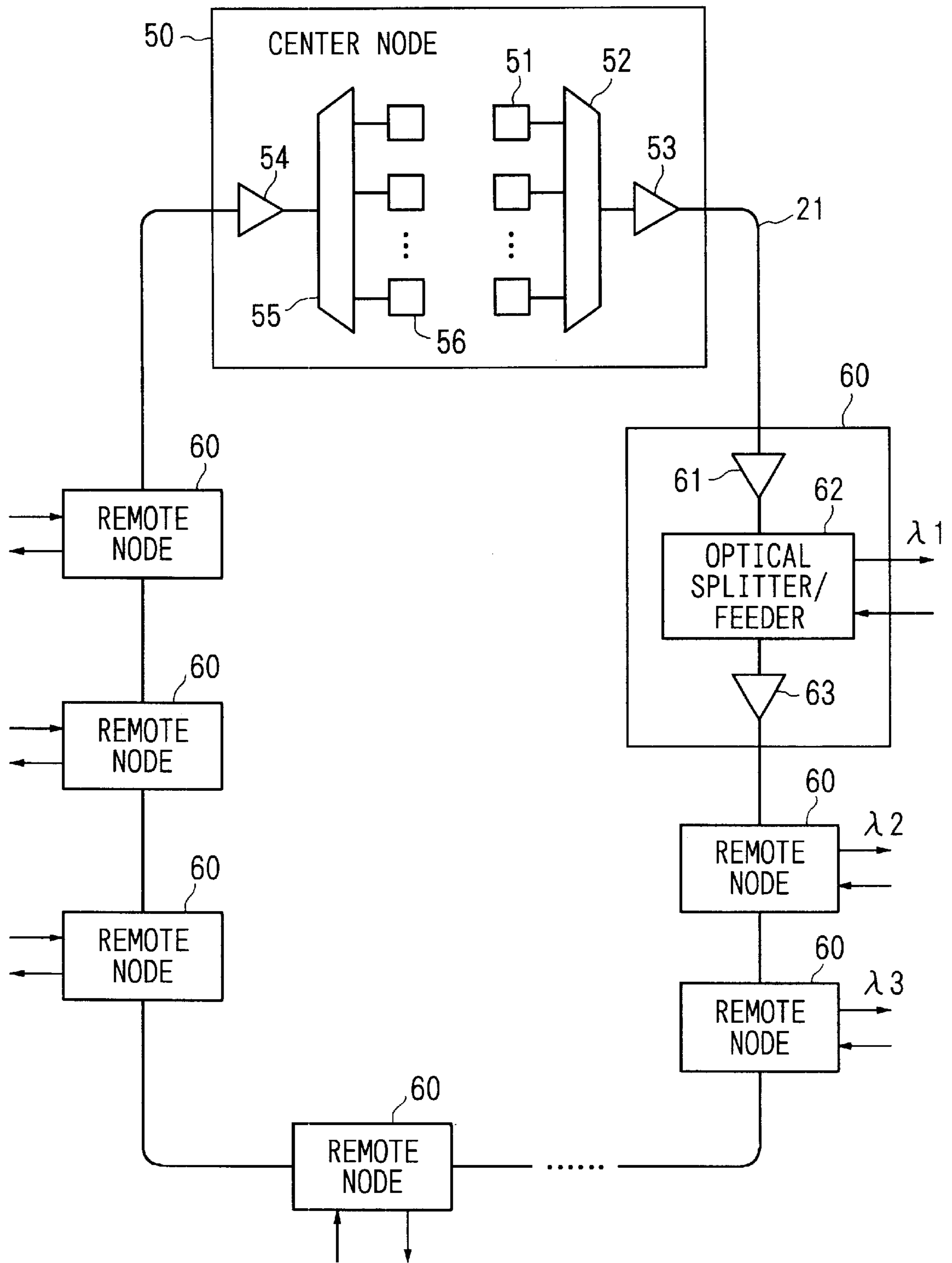
STRUCTURE OF THE FORTH EMBODIMENT OF THE PRESENT INVENTION
