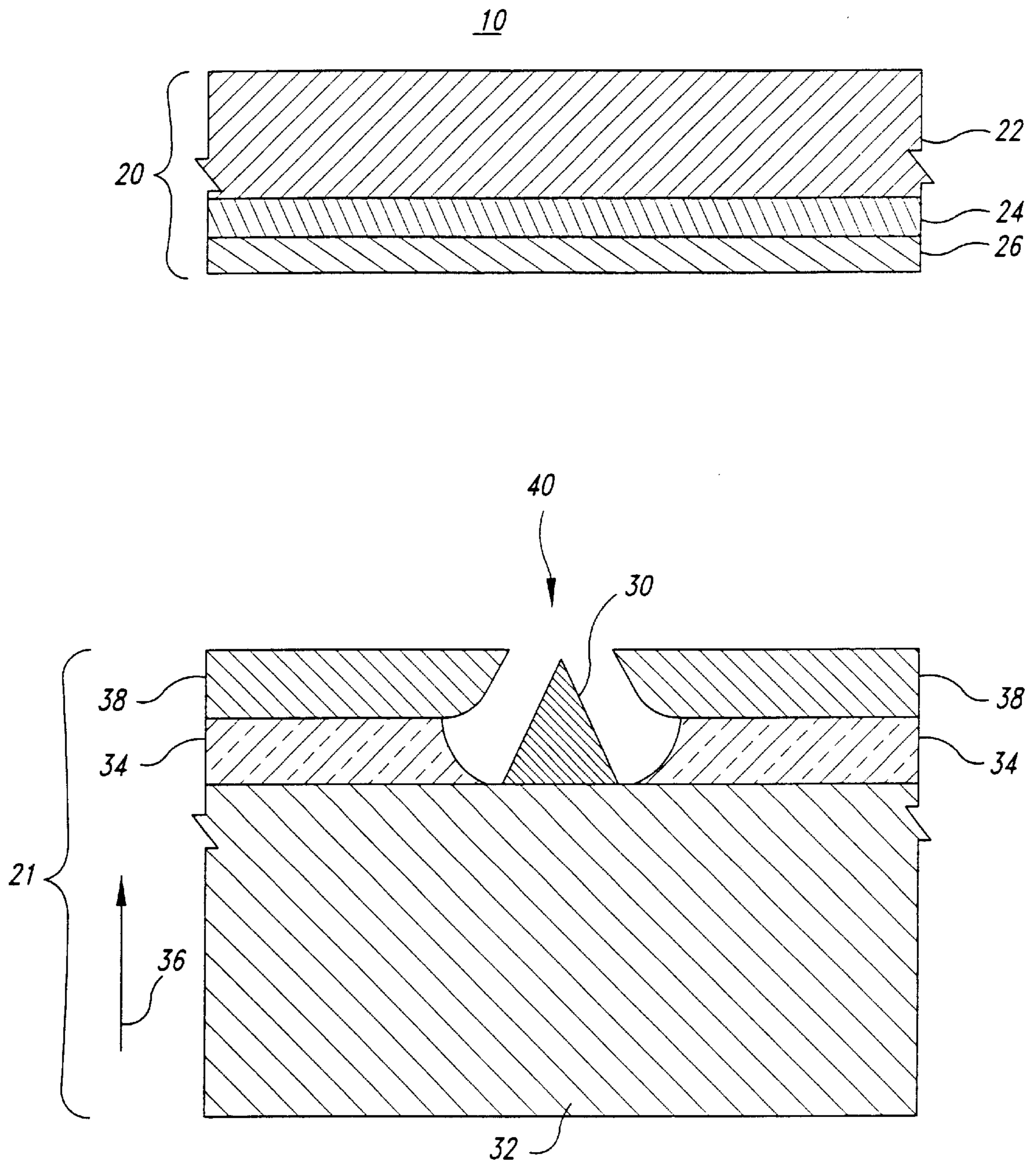
Fig. 1 (PRIOR ART)
