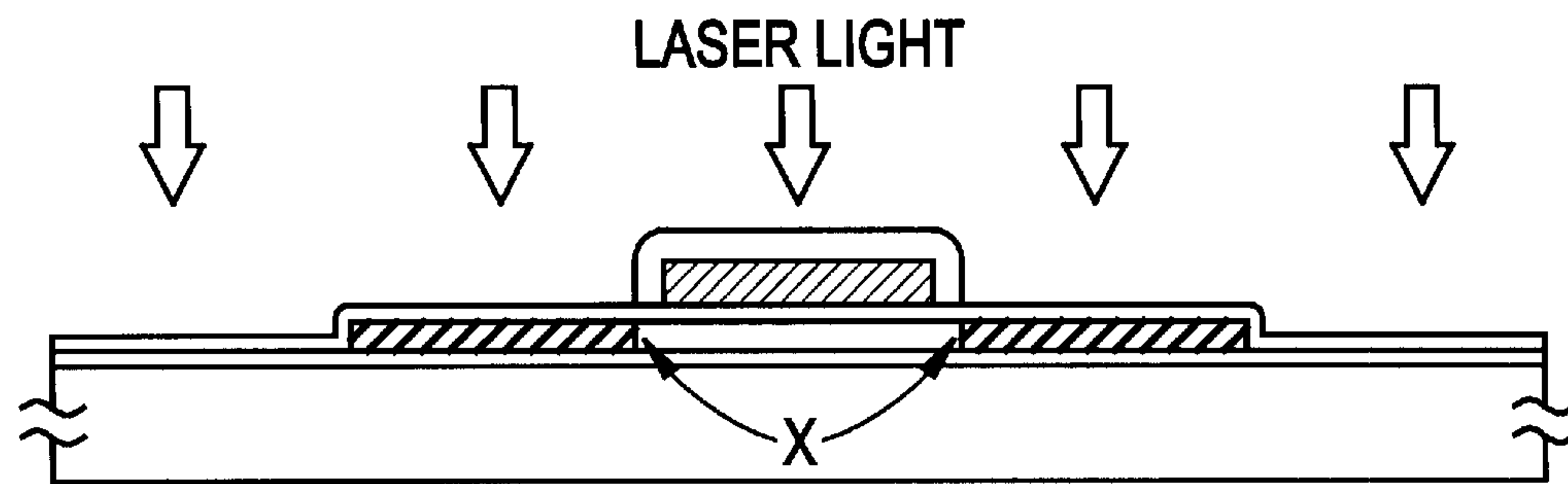
FIG. 2C PRIOR ART
