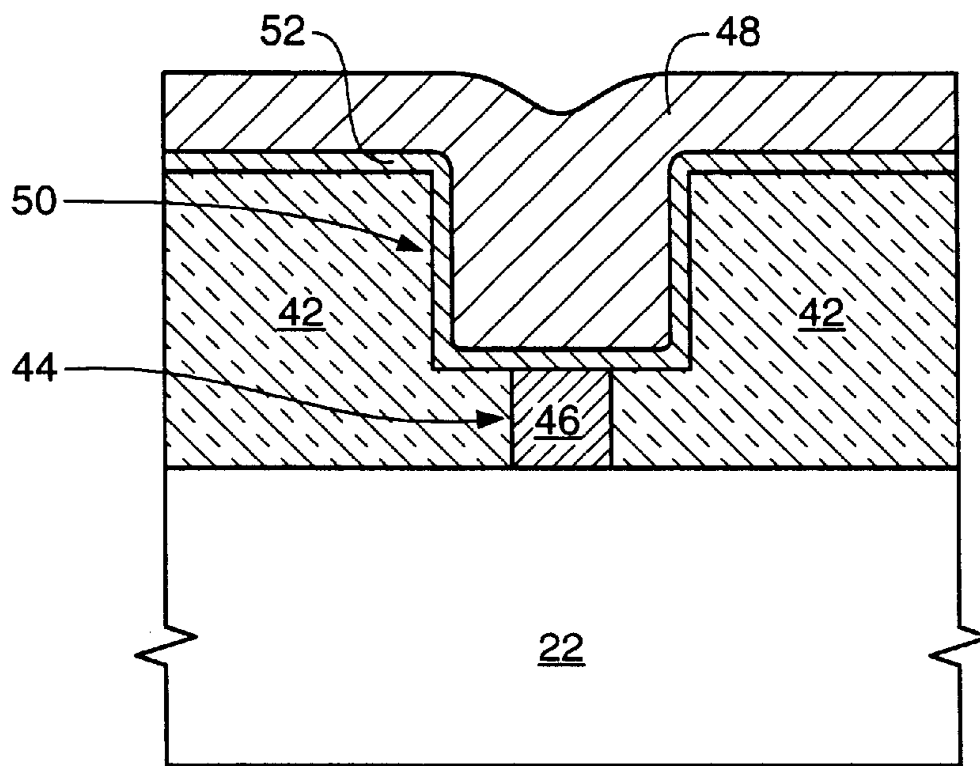
FIG. 7 (PRIOR ART)
