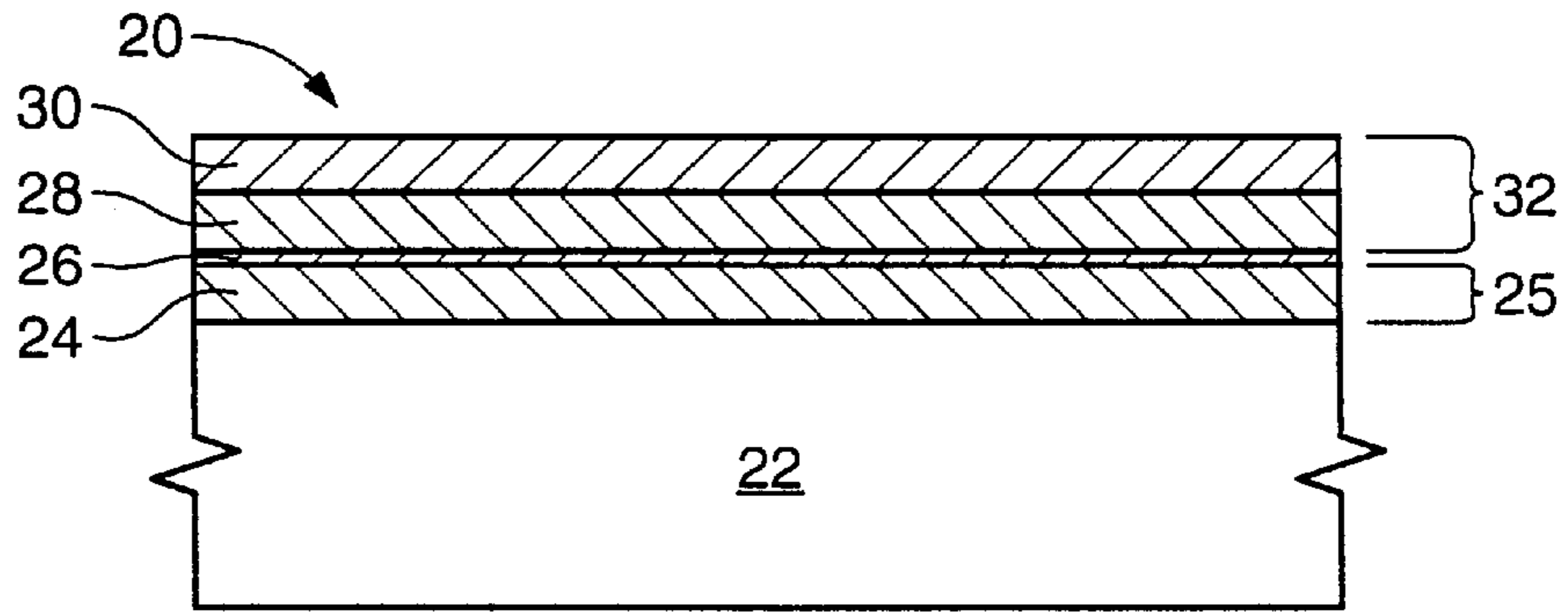
FIG. 2 (PRIOR ART)
