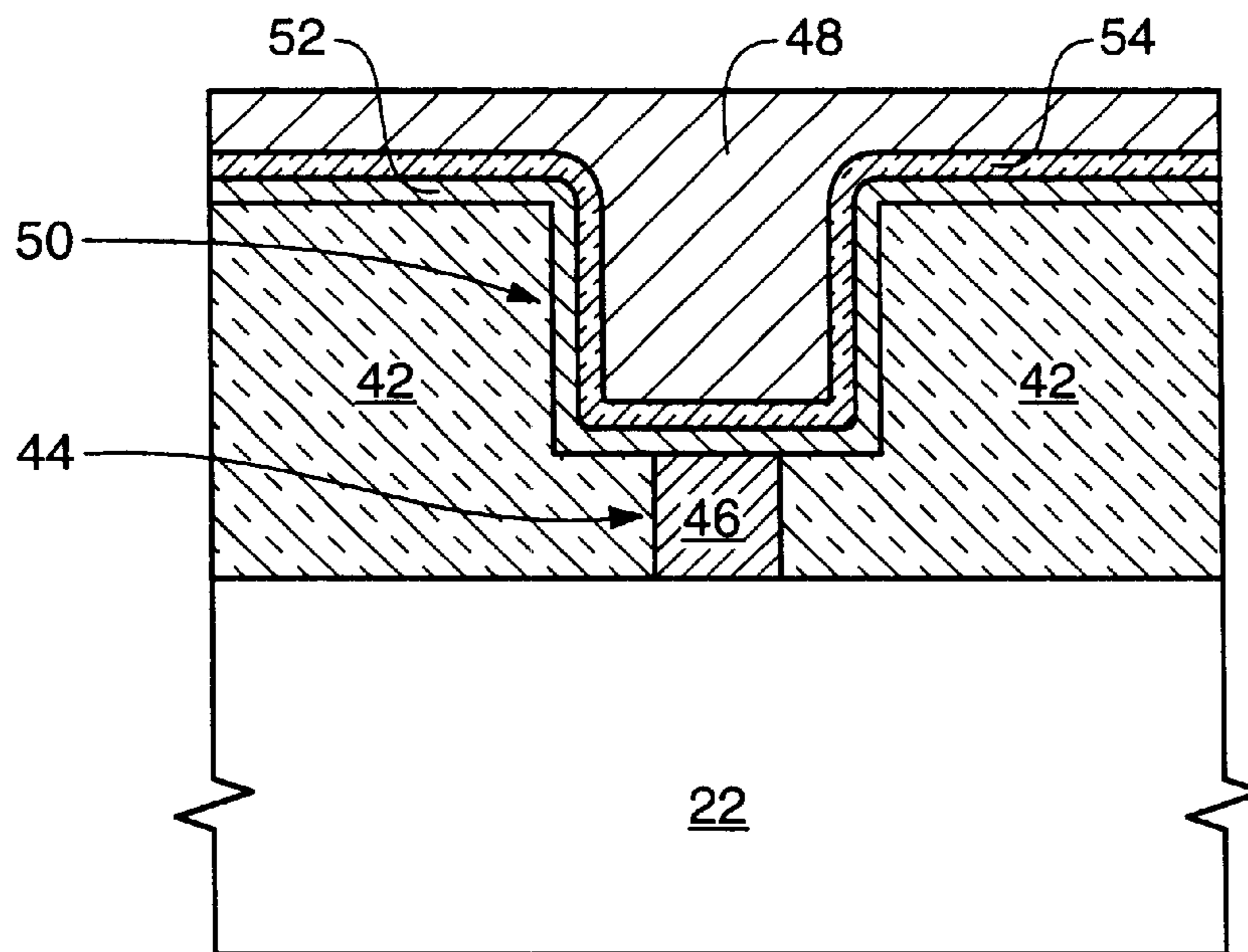
FIG. 8 (PRIOR ART)
